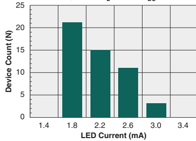
Typical I F for Switch Operation (N=50, I L =200mA DC )
