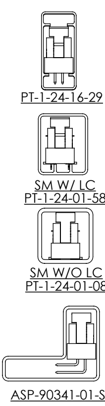
FIG 7 PACKAGING VIEWS
