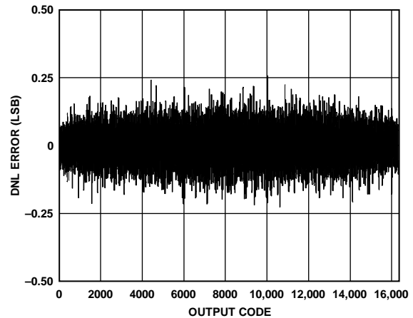
Figure 17. AD9255-80 DNL with f_{IN} = 12.5 MHz
