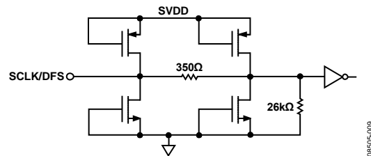
Figure 59. Equivalent SCLK/DFS Input Circuit
