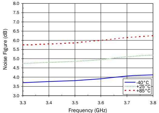
Noise Figure (NF) versus Frequency
