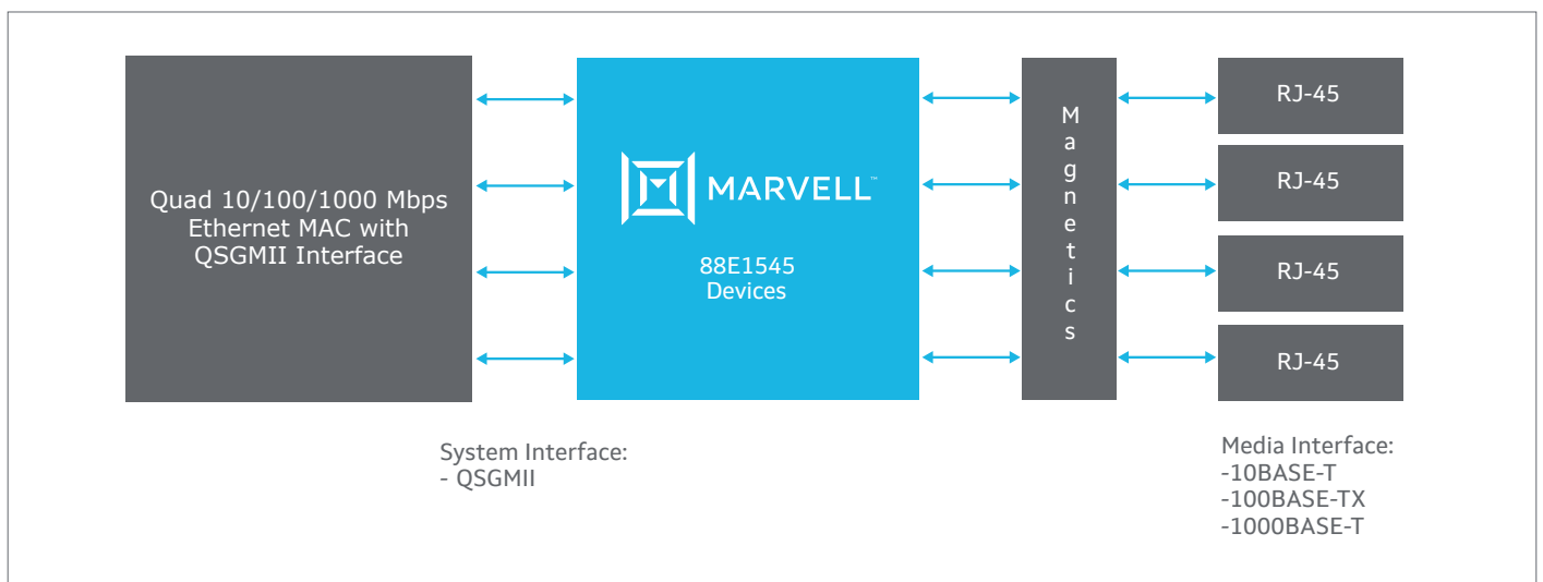
Figure 1. QSGMII to Copper Application
