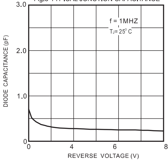
Fig.3-TYPICAL JUNCTION CAPACITANCE
