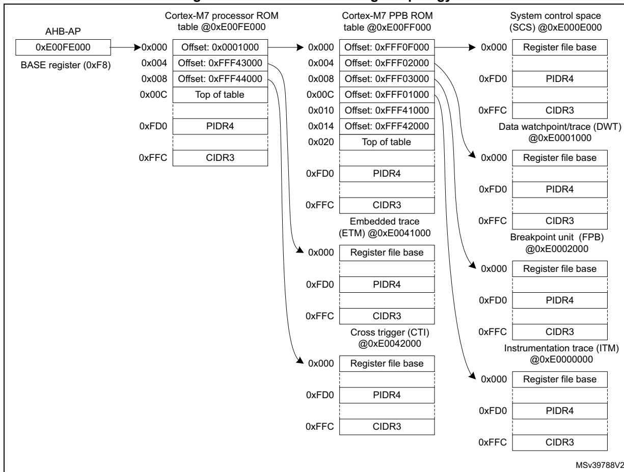
Figure 871. Cortex-M7 CoreSight topology
