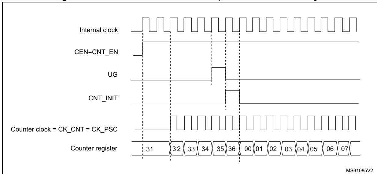
Figure 409. Control circuit in normal mode, internal clock divided by 1
