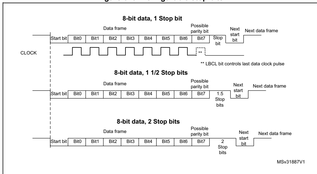
Figure 613. Configurable stop bits
