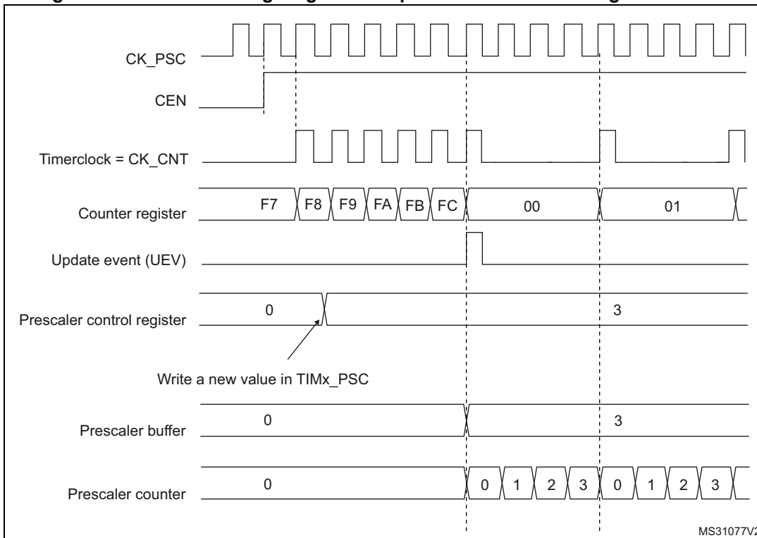
Figure 498. Counter timing diagram with prescaler division change from 1 to 4
