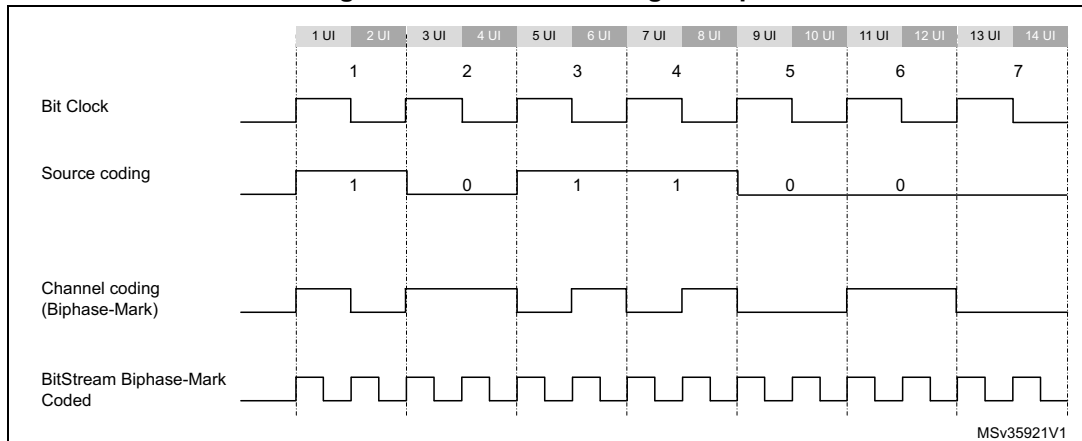
Figure 712. Channel coding example
