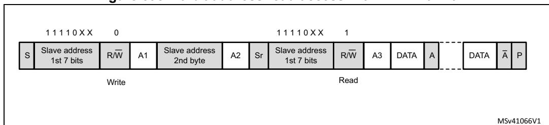
Figure 595. 10-bit address read access with HEAD10R=0
