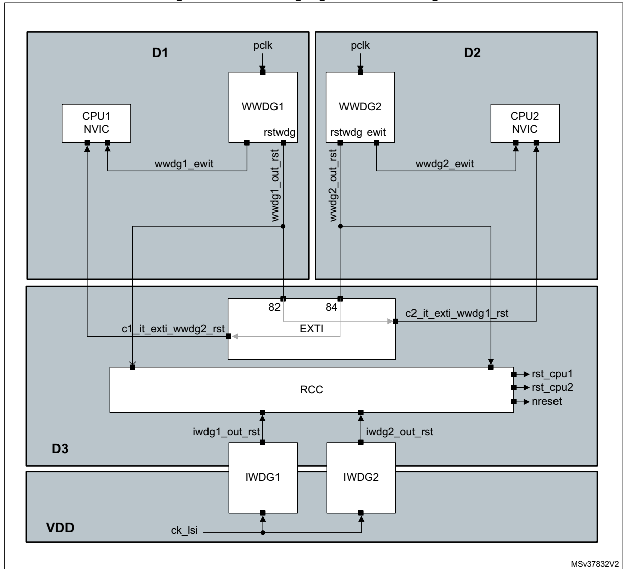
Figure 573. Watchdog high-level block diagram
