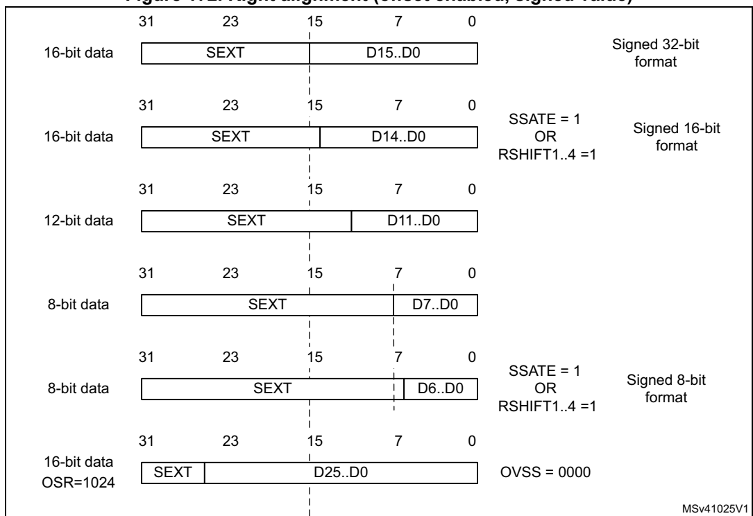
Figure 172. Right alignment (offset enabled, signed value)
