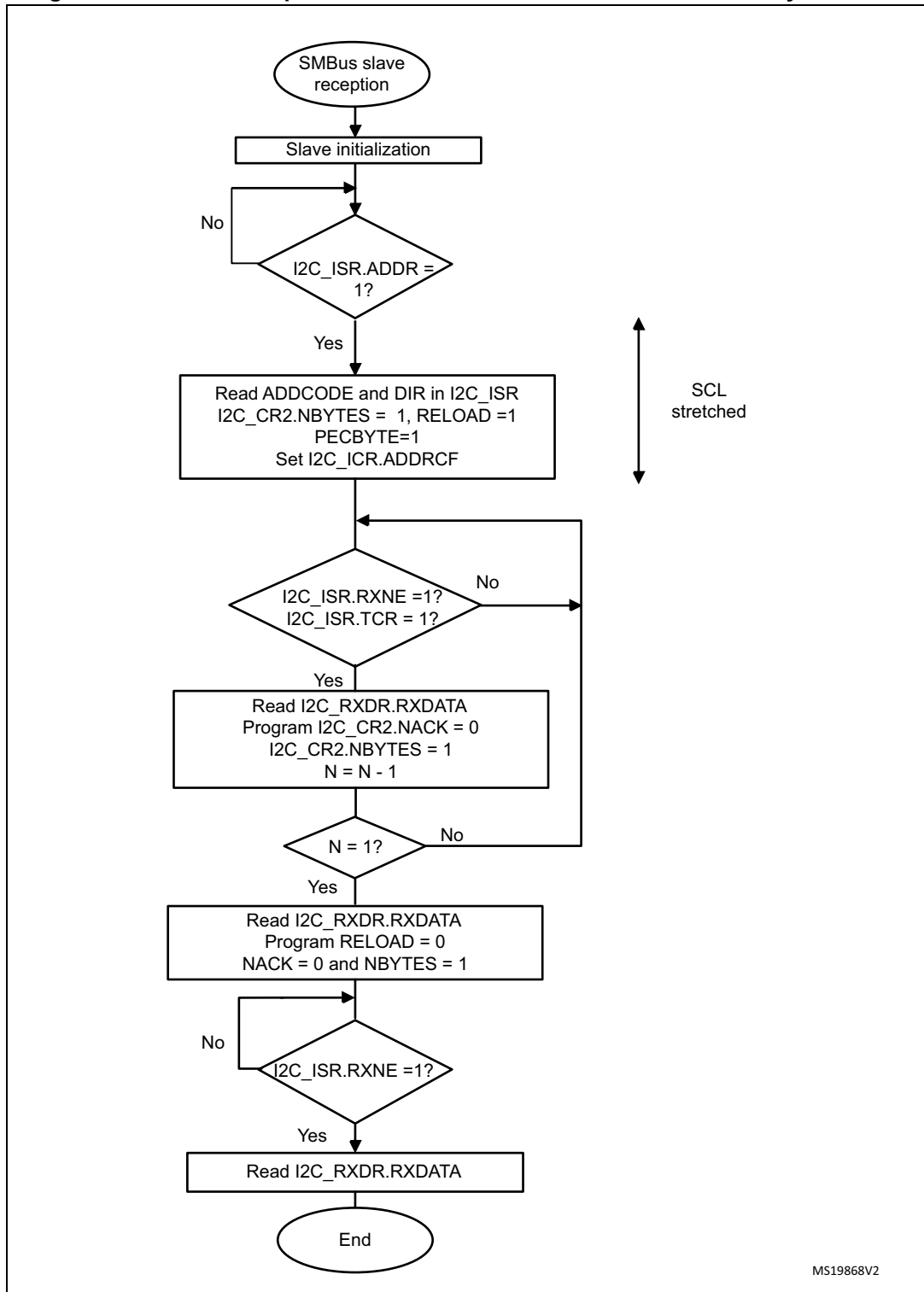
Figure 606. Transfer sequence flowchart for SMBus slave receiver N Bytes + PEC
