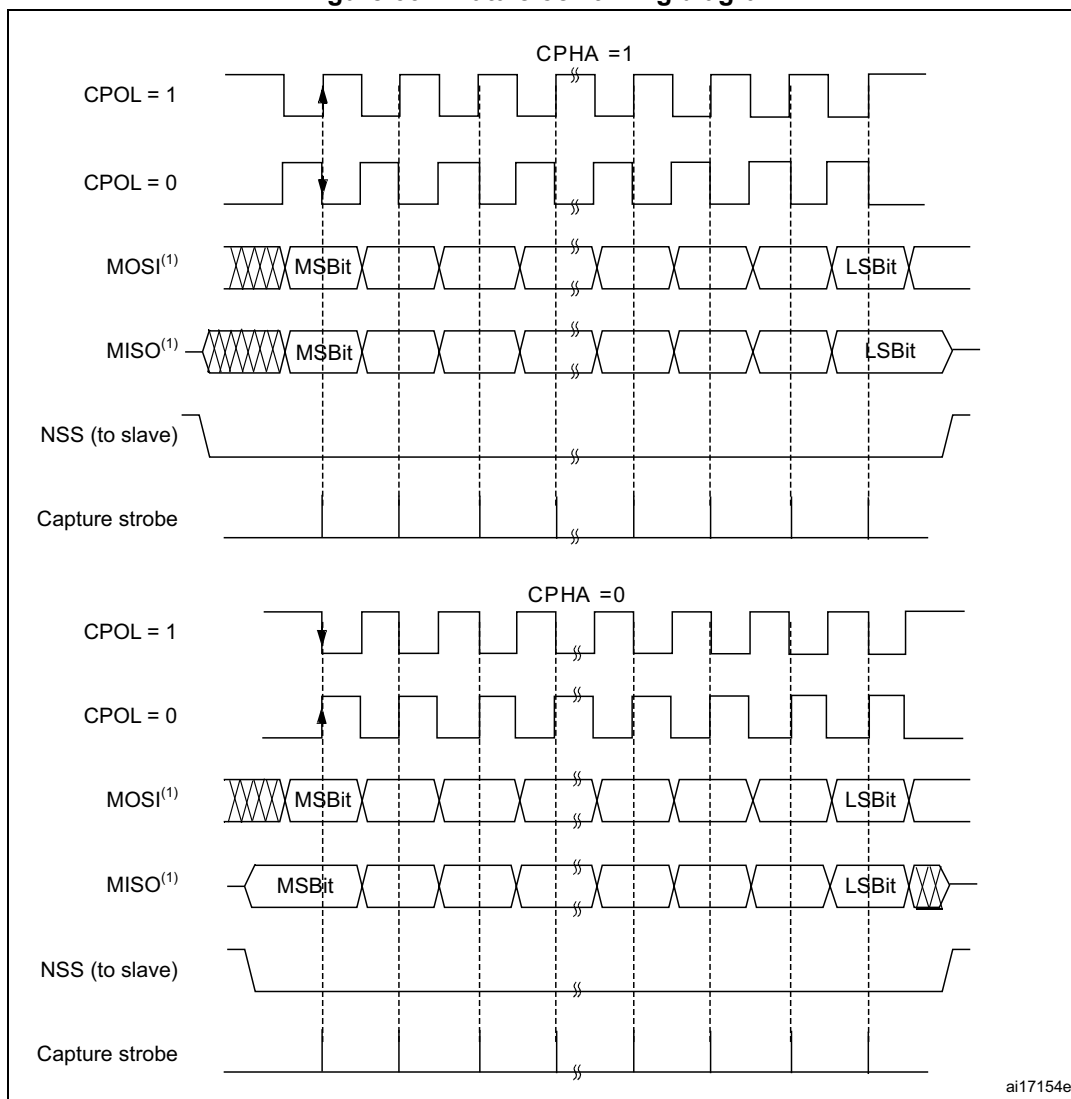
Figure 662. Data clock timing diagram
