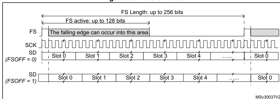
Figure 687. Audio frame
