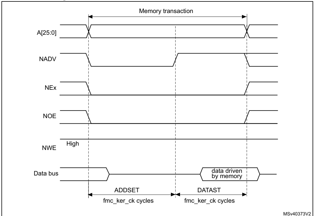
Figure 109. Mode 2 and mode B read access waveforms
