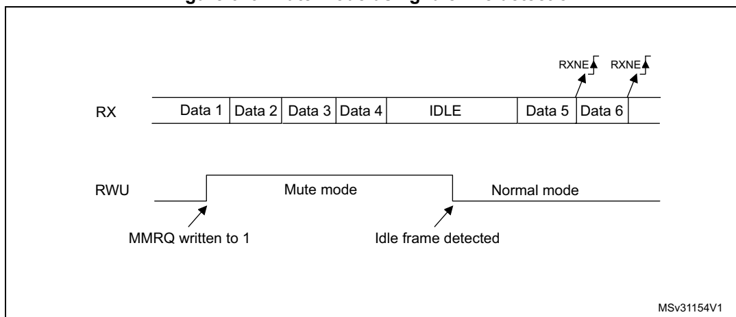
Figure 619. Mute mode using Idle line detection
