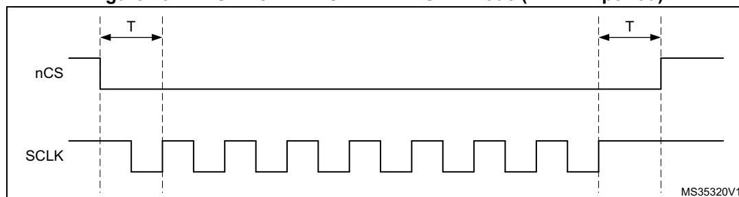
Figure 137. nCS when CKMODE = 1 in SDR mode (T = CLK period)
