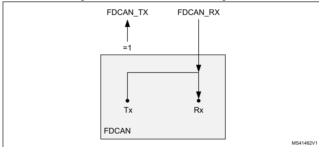
Figure 776. Pin control in bus monitoring mode
