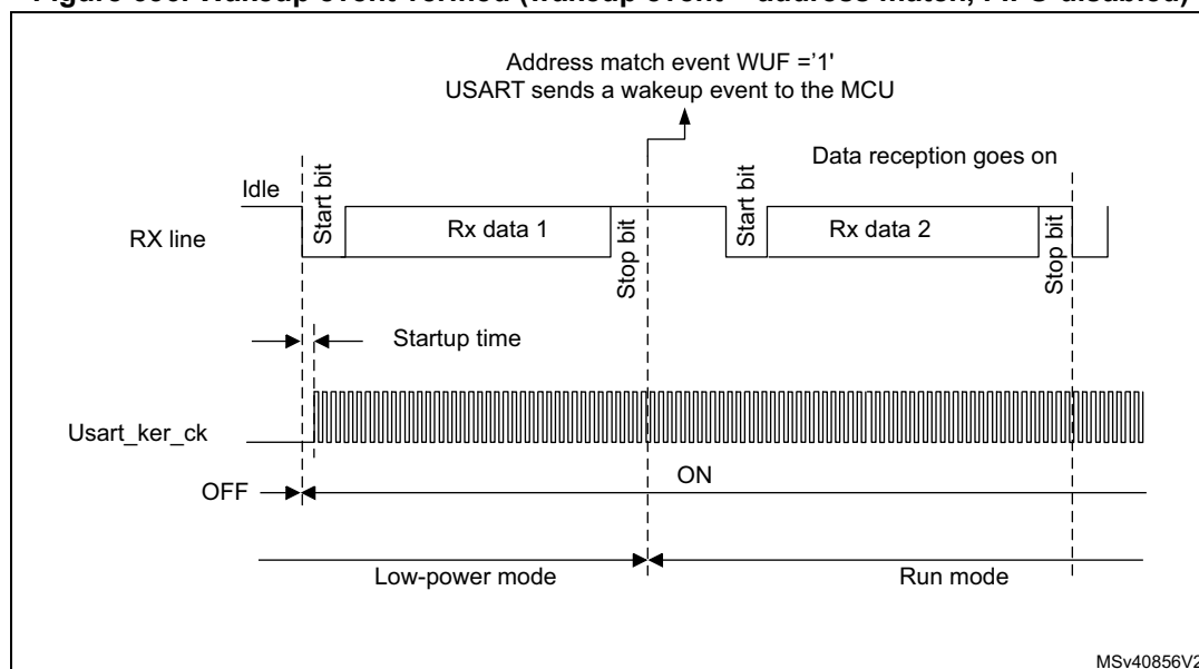
Figure 636. Wakeup event verified (wakeup event = address match, FIFO disabled)
