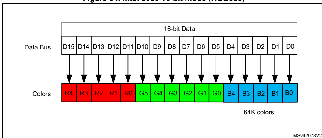
Figure 94. Intel 8080 16-bit mode (RGB565)
