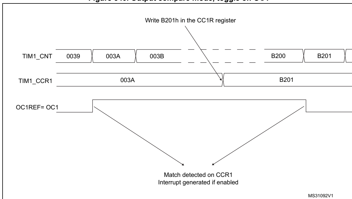
Figure 540. Output compare mode, toggle on OC1
