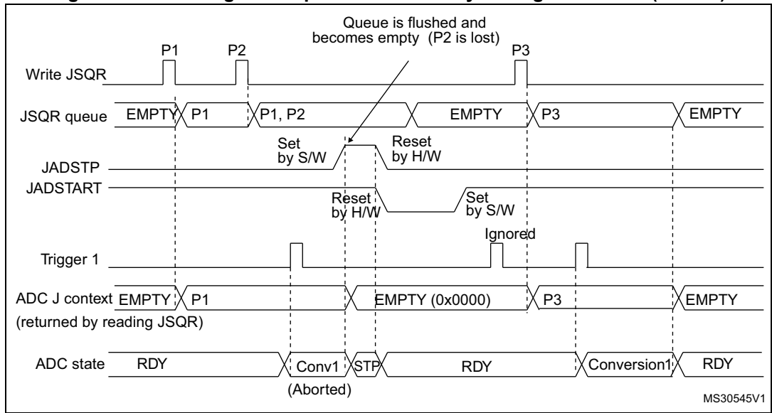
Figure 164. Flushing JSQR queue of context by setting JADSTP=1 (JQM=1)
