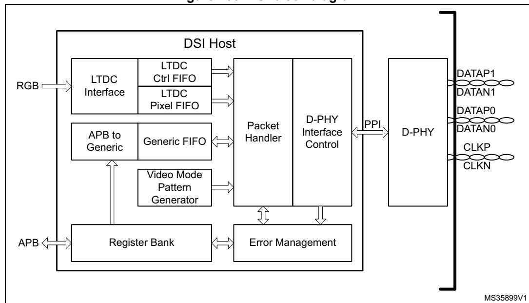
Figure 255. DSI block diagram
