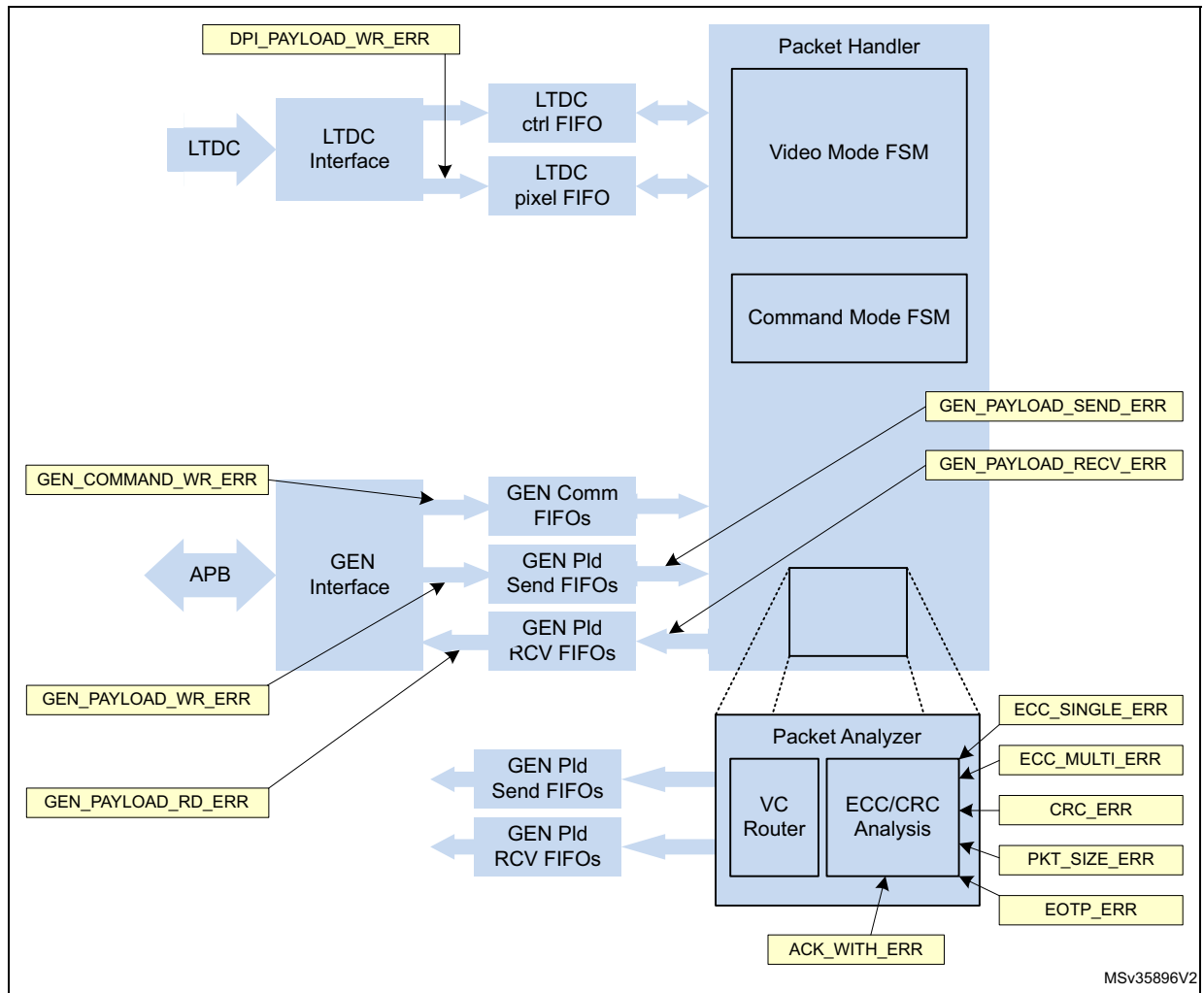
Figure 288. Error sources
