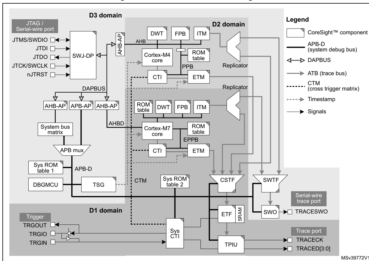
Figure 860. Power domains of debug infrastructure
