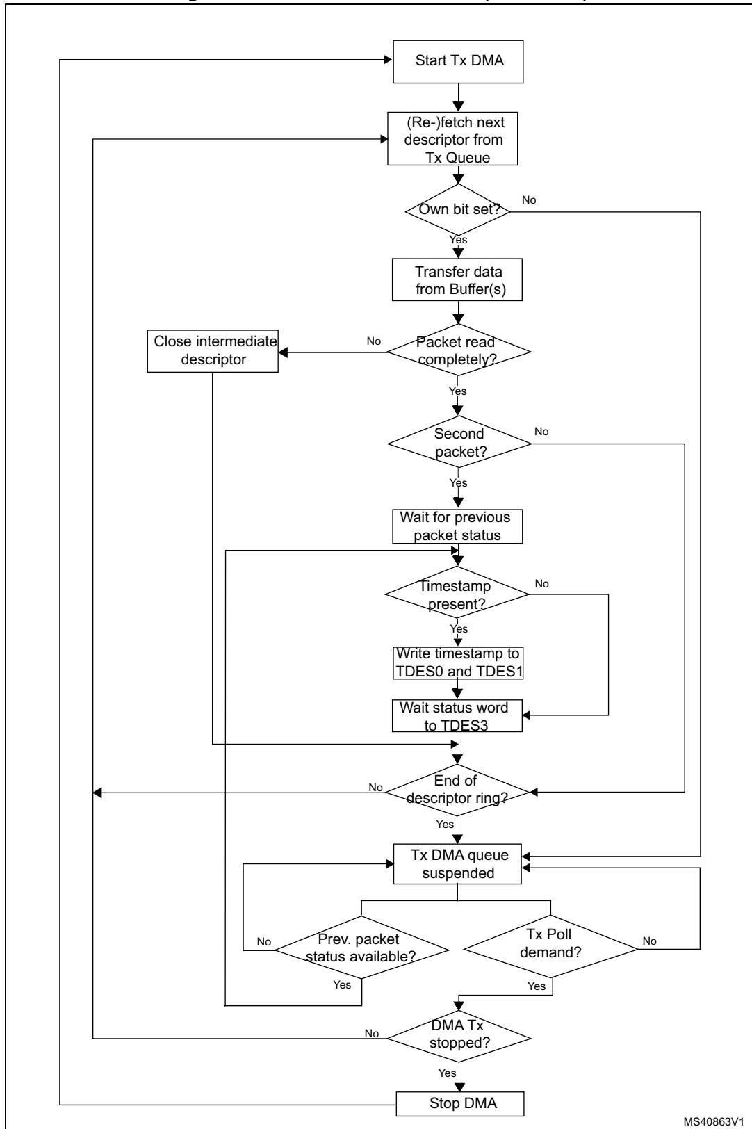
Figure 821. DMA transmission flow (OSP mode)
