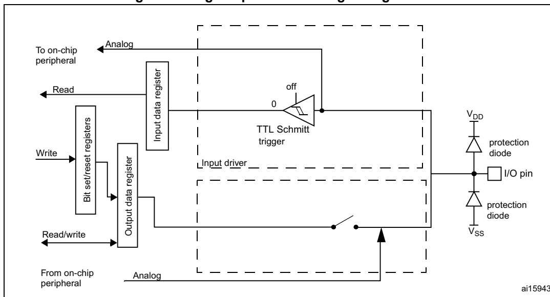
Figure 81. High impedance-analog configuration
