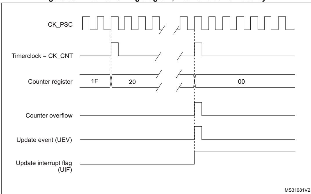
Figure 502. Counter timing diagram, internal clock divided by N
