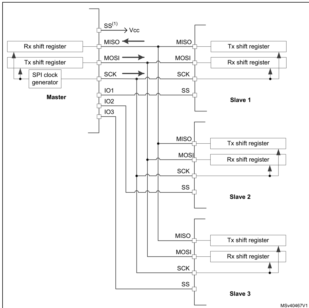
Figure 656. Master and three independent slaves at star topology
