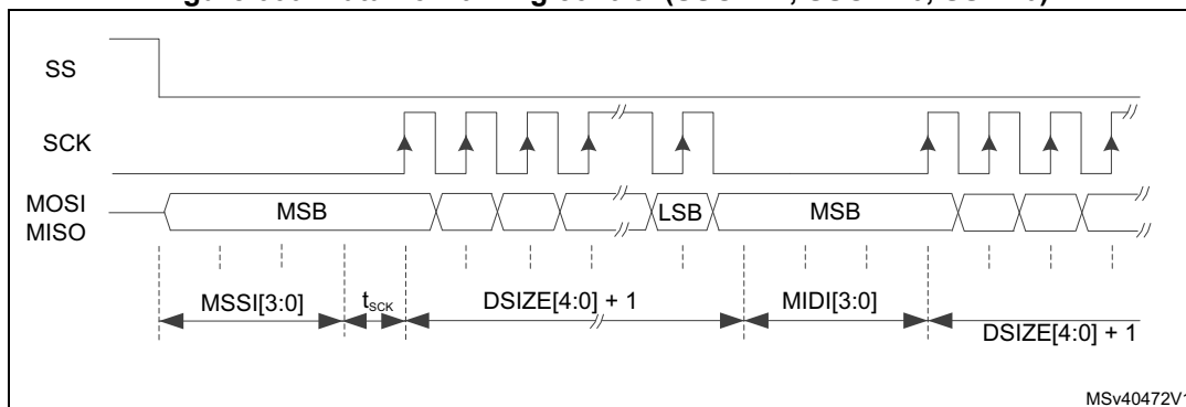
Figure 660. Data flow timing control (SSOE=1, SSOM=0, SSM=0)
