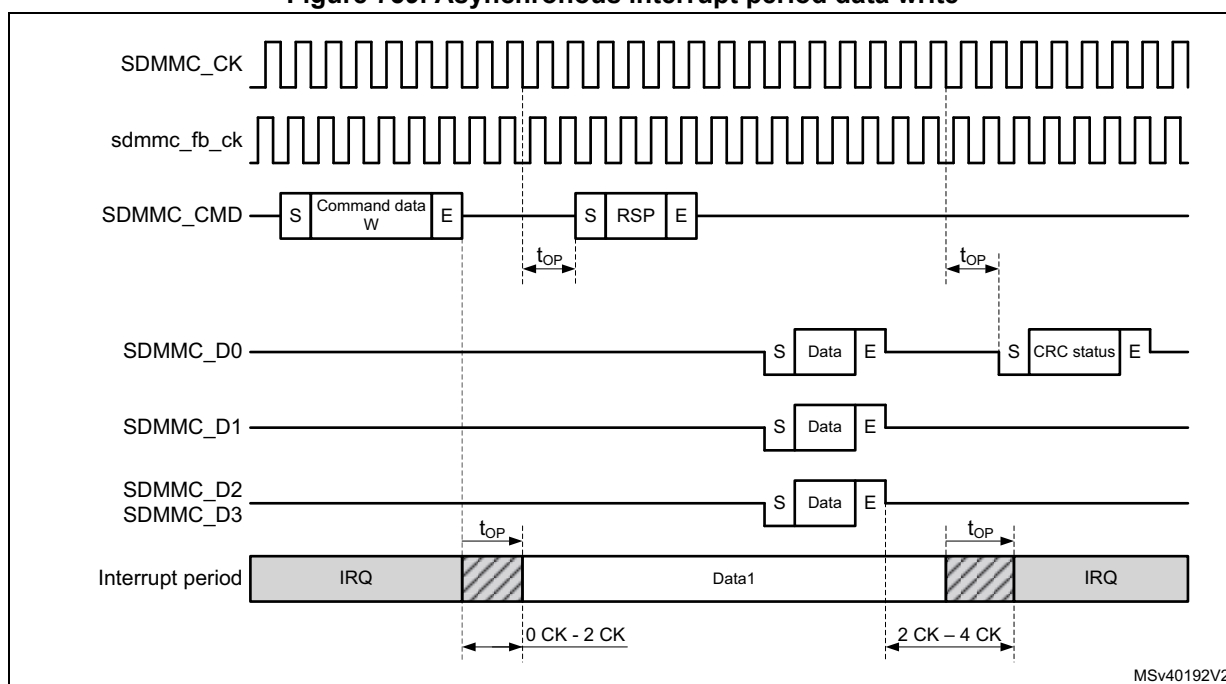
Figure 759. Asynchronous interrupt period data write
