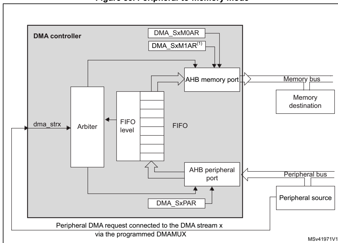
Figure 85. Peripheral-to-memory mode
