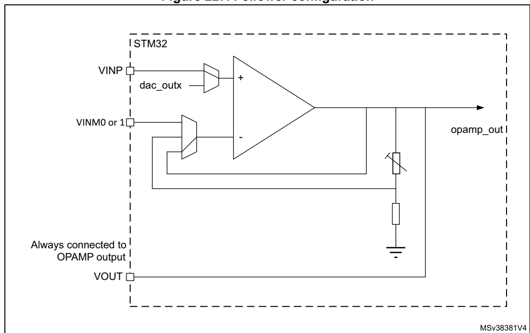
Figure 227. Follower configuration
