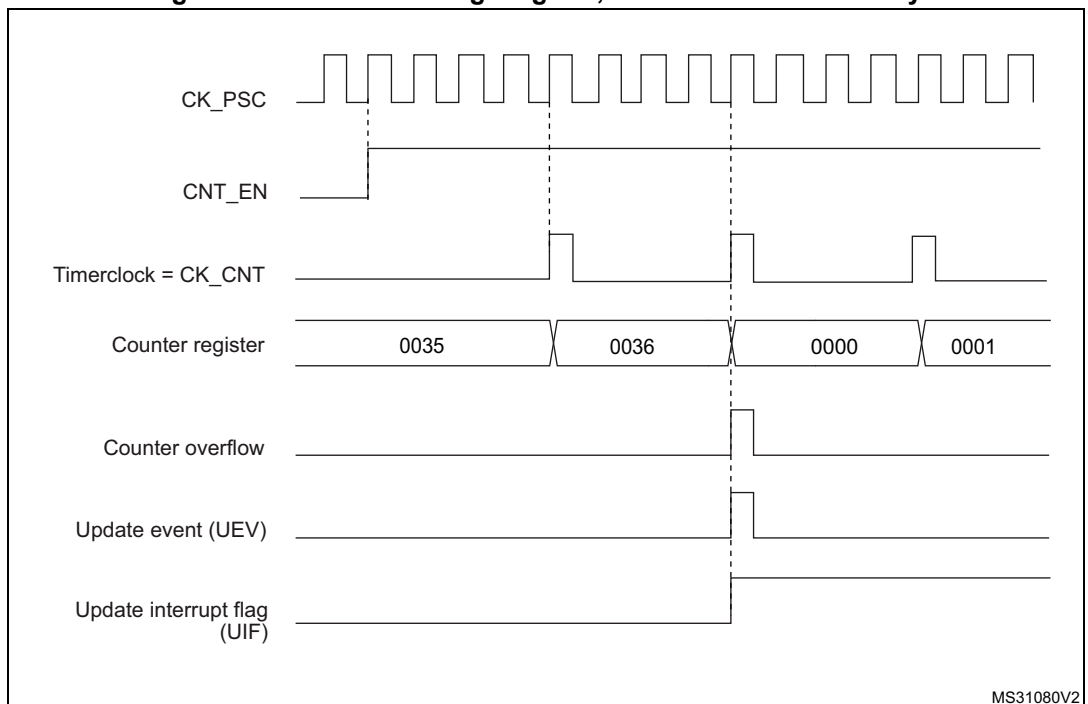
Figure 501. Counter timing diagram, internal clock divided by 4
