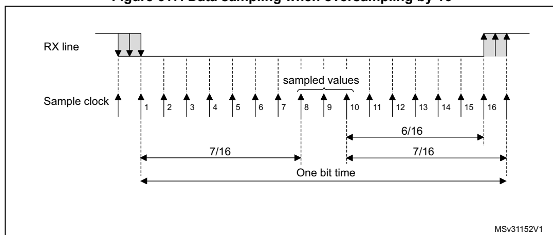
Figure 617. Data sampling when oversampling by 16
