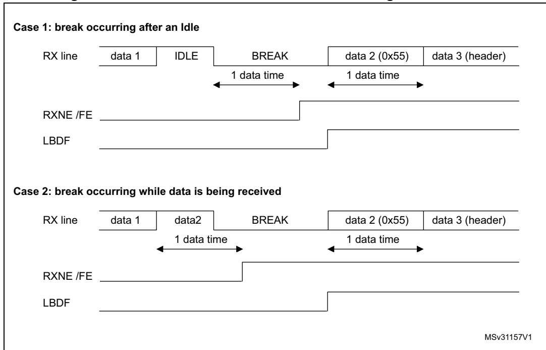
Figure 622. Break detection in LIN mode vs. Framing error detection
