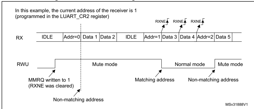
Figure 644. Mute mode using address mark detection
