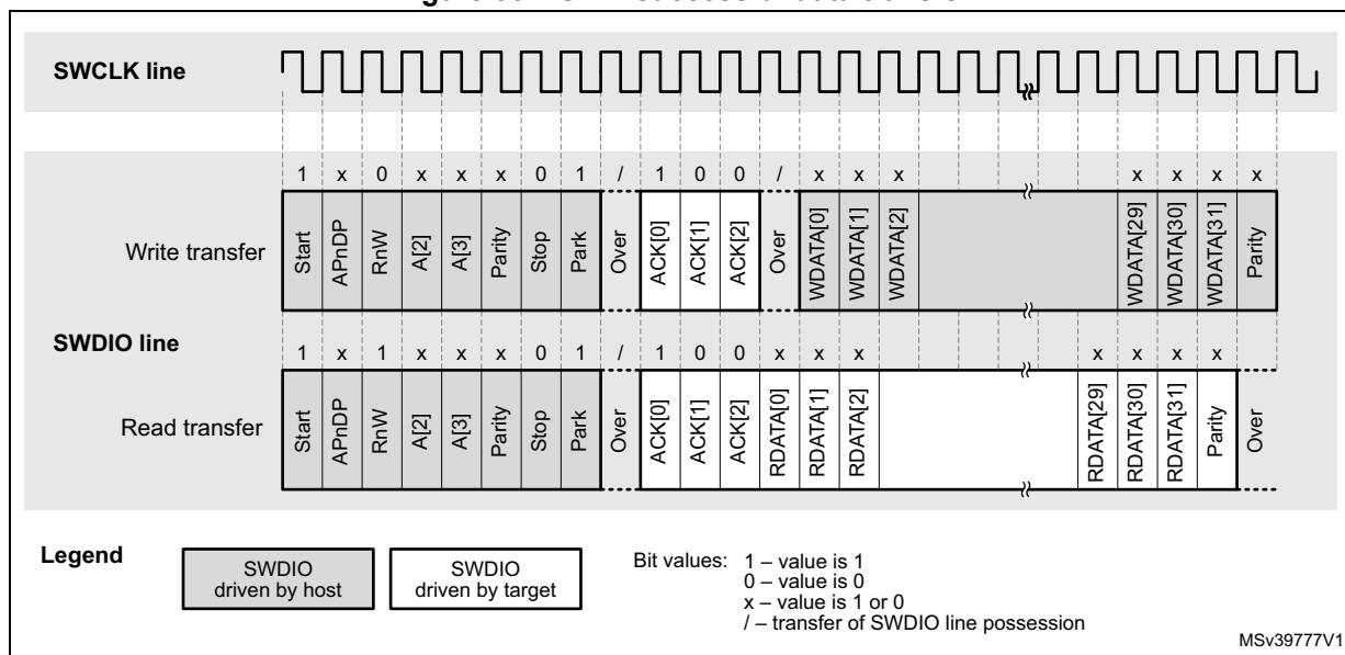
Figure 862. SWD successful data transfer
