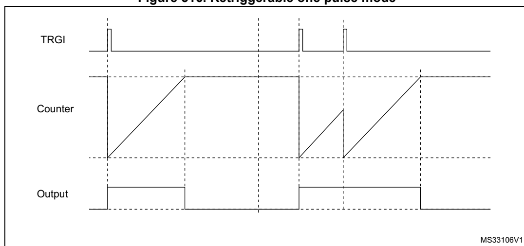
Figure 516. Retriggerable one pulse mode
