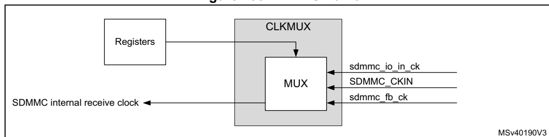
Figure 753. CLKMUX unit
