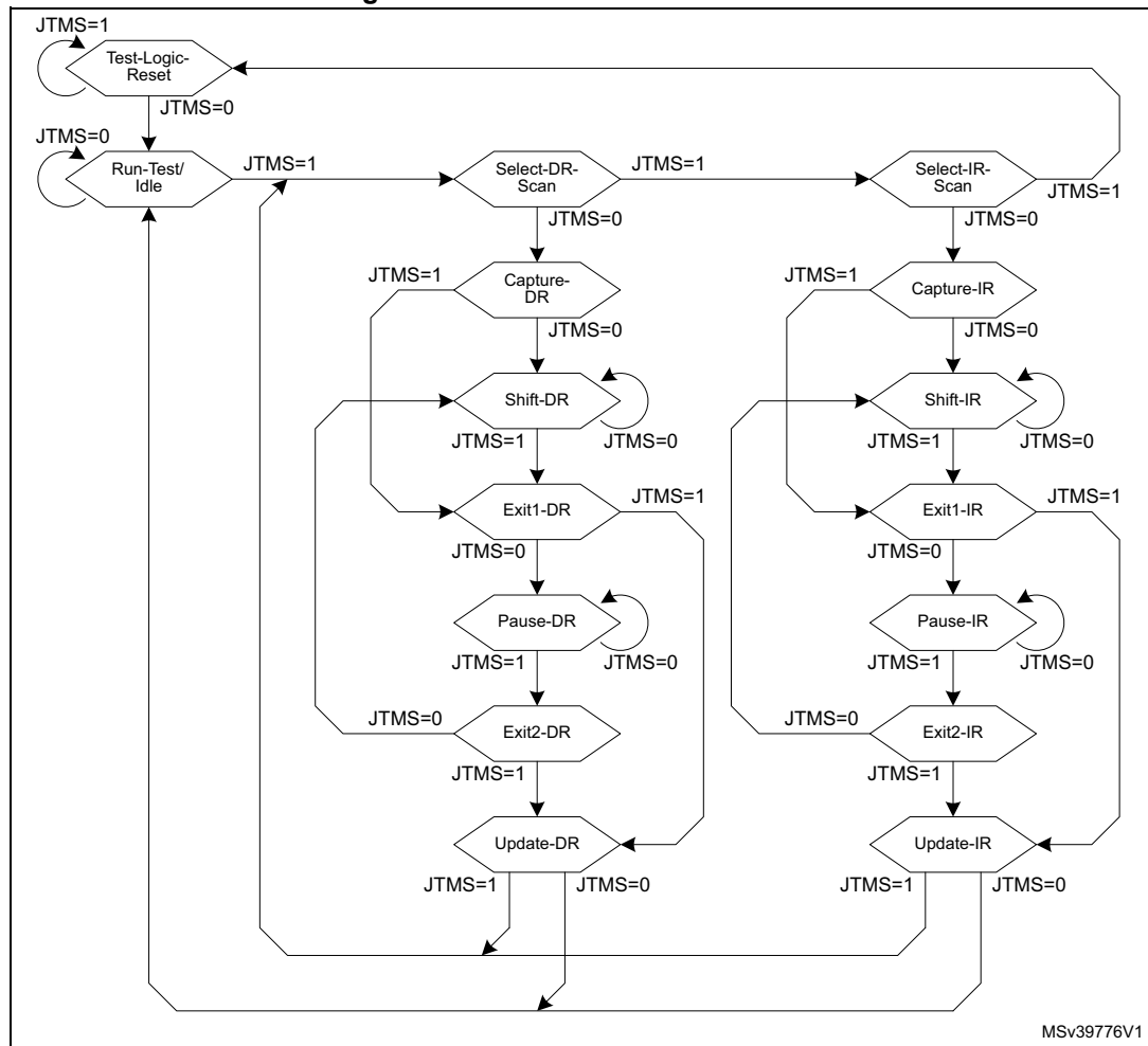
Figure 863. JTAG TAP state machine
