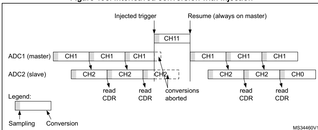
Figure 198. Interleaved conversion with injection
