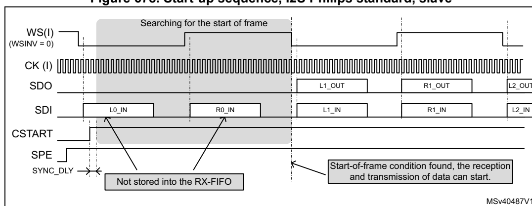
Figure 678. Start-up sequence, I2S Philips standard, slave
