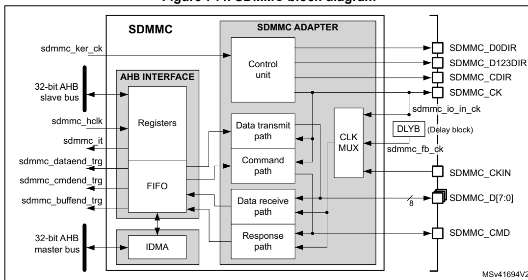
Figure 744. SDMMC block diagram
