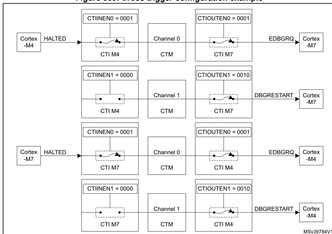
Figure 869. Cross trigger configuration example
