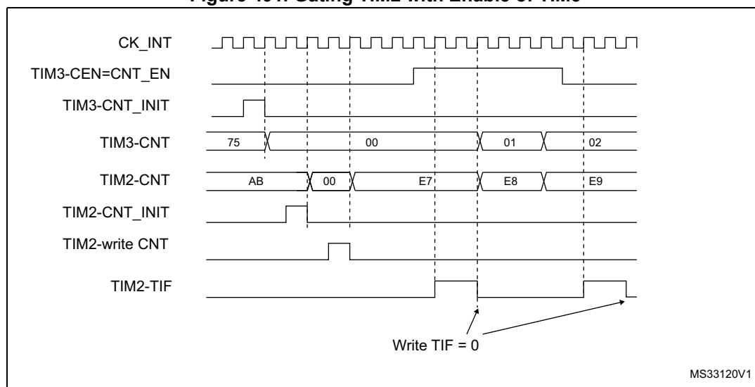
Figure 491. Gating TIM2 with Enable of TIM3
