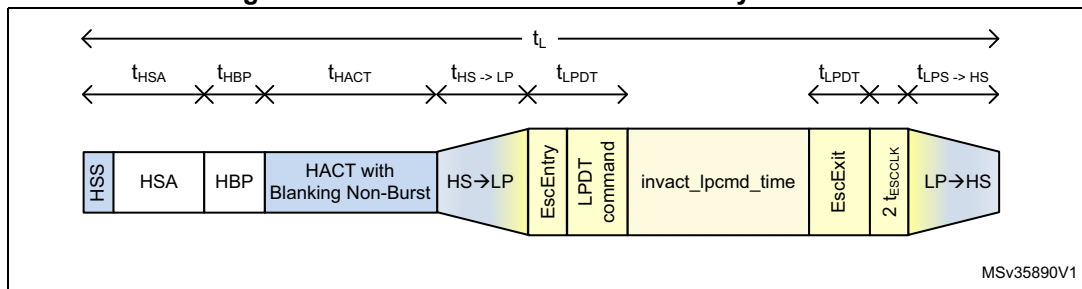
Figure 275. VLPSIZE for non-burst with sync events
