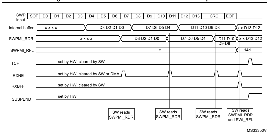
Figure 732. SWPMI No software buffer mode reception
