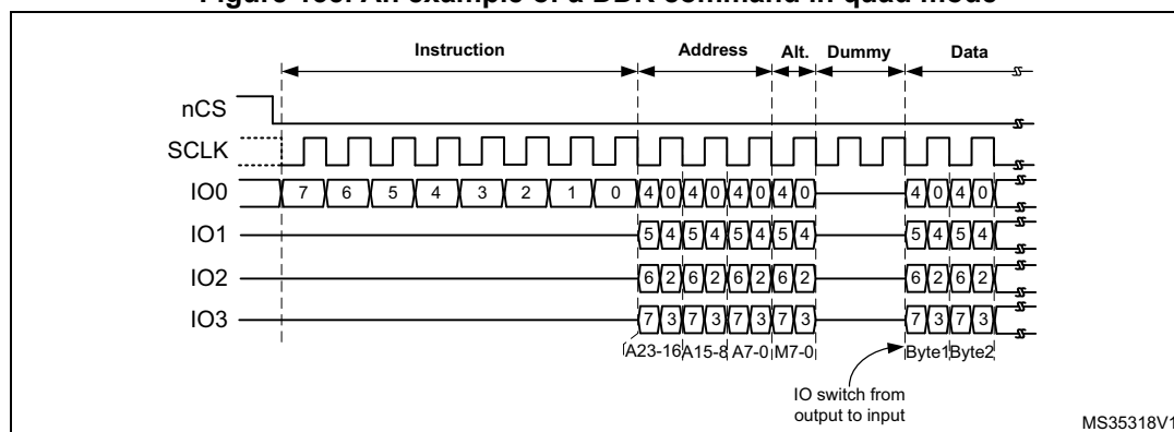
Figure 135. An example of a DDR command in quad mode
