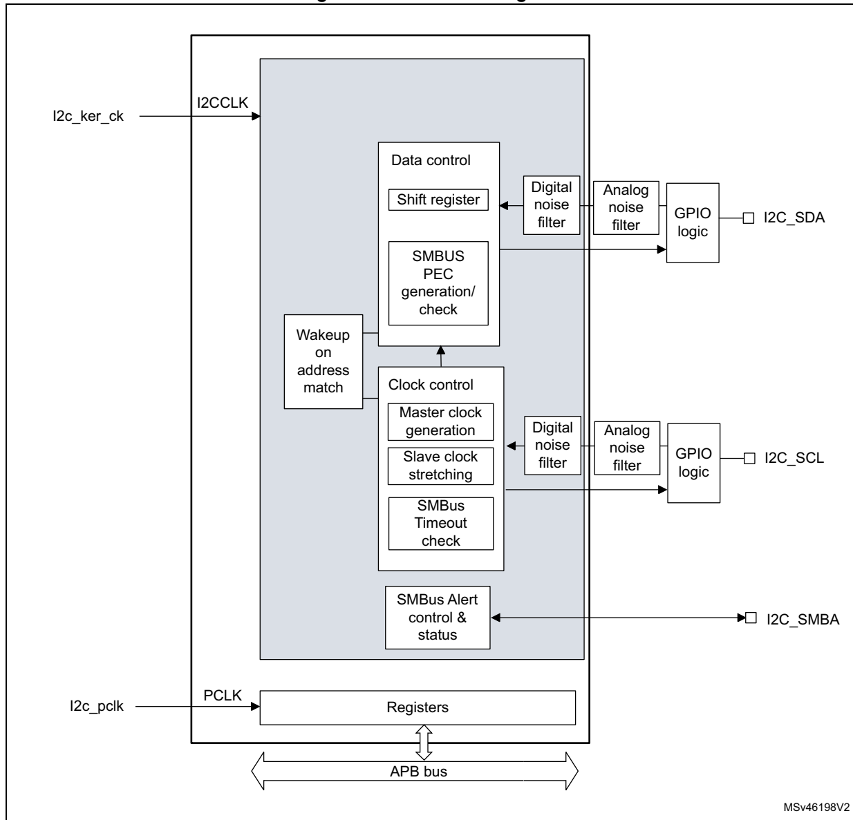
Figure 580. I2C block diagram
