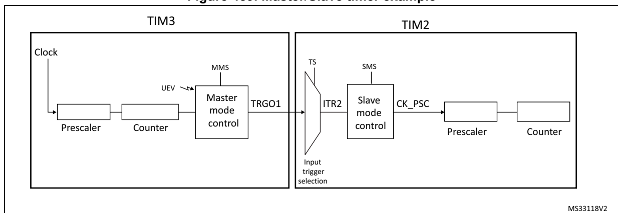
Figure 489. Master/Slave timer example
