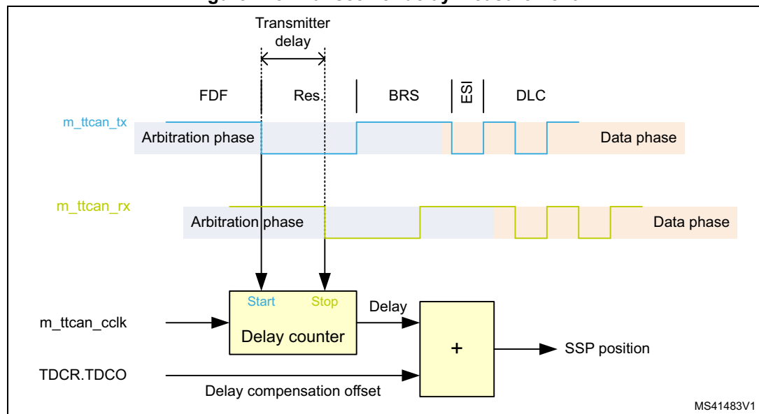
Figure 775. Transceiver delay measurement
