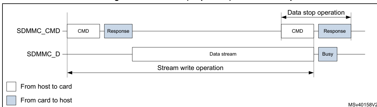
Figure 743. SDMMC (sequential) stream write operation
