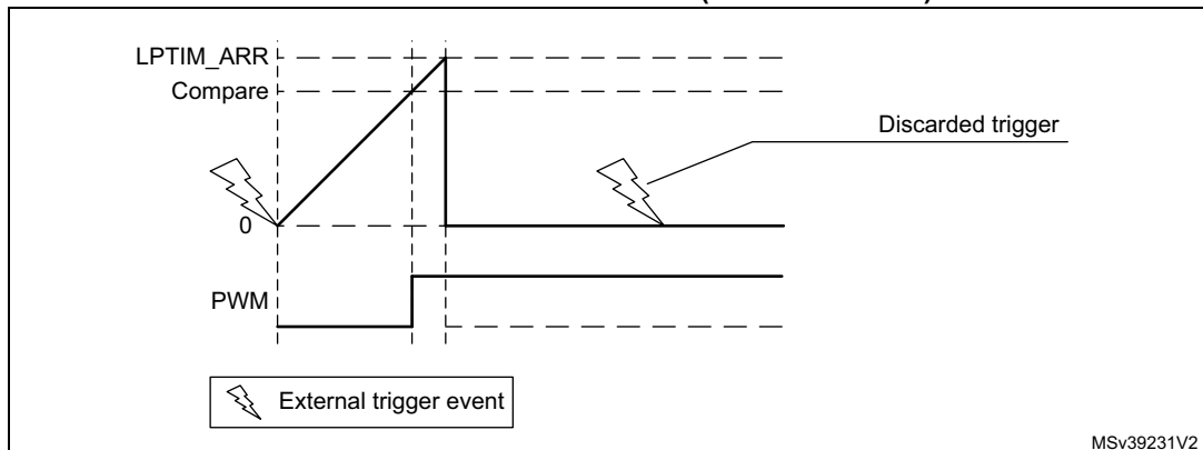
Figure 569. LPTIM output waveform, Single counting mode configuration and Set-once mode activated (WAVE bit is set)
