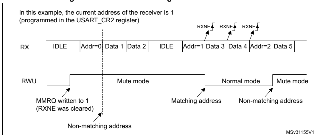
Figure 620. Mute mode using address mark detection
