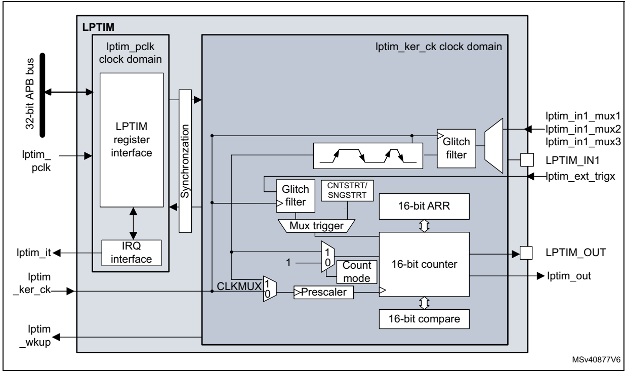
Figure 565. Low-power timer block diagram (LPTIM3)
