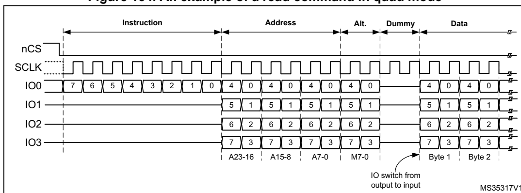
Figure 134. An example of a read command in quad mode
