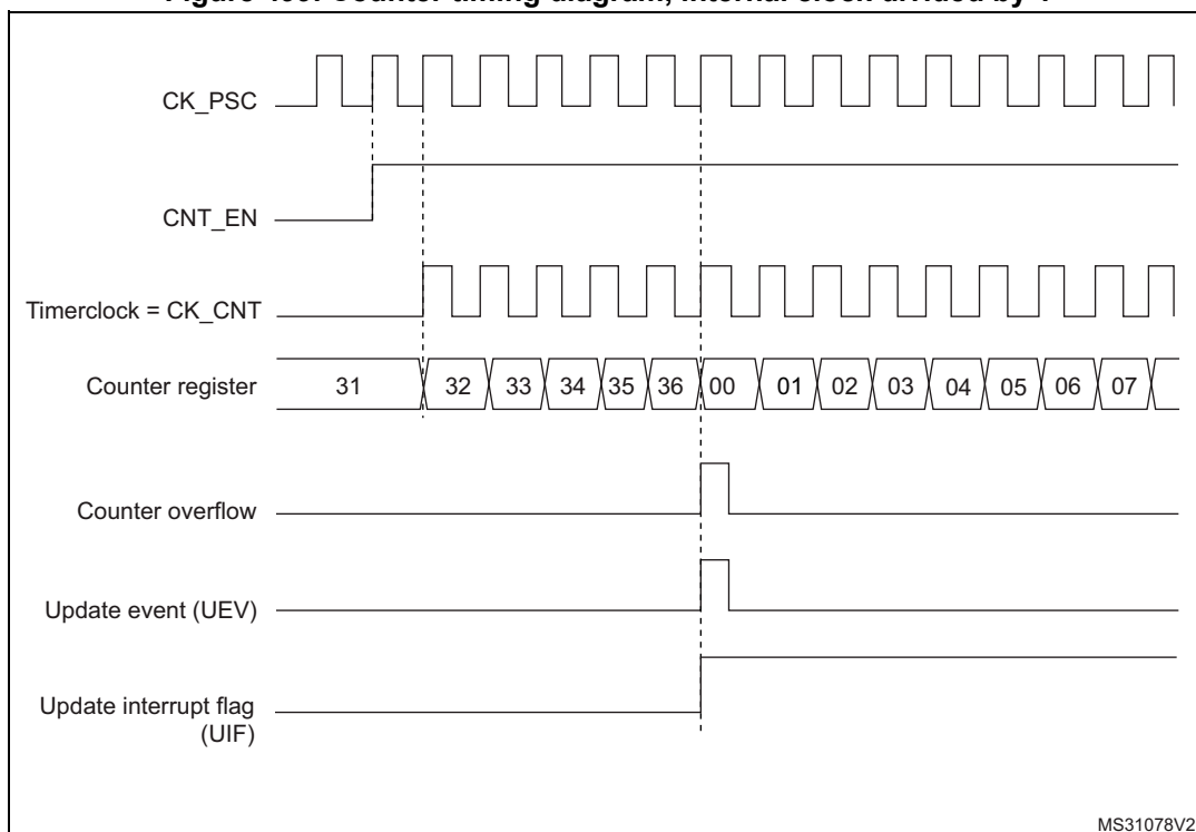
Figure 499. Counter timing diagram, internal clock divided by 1
