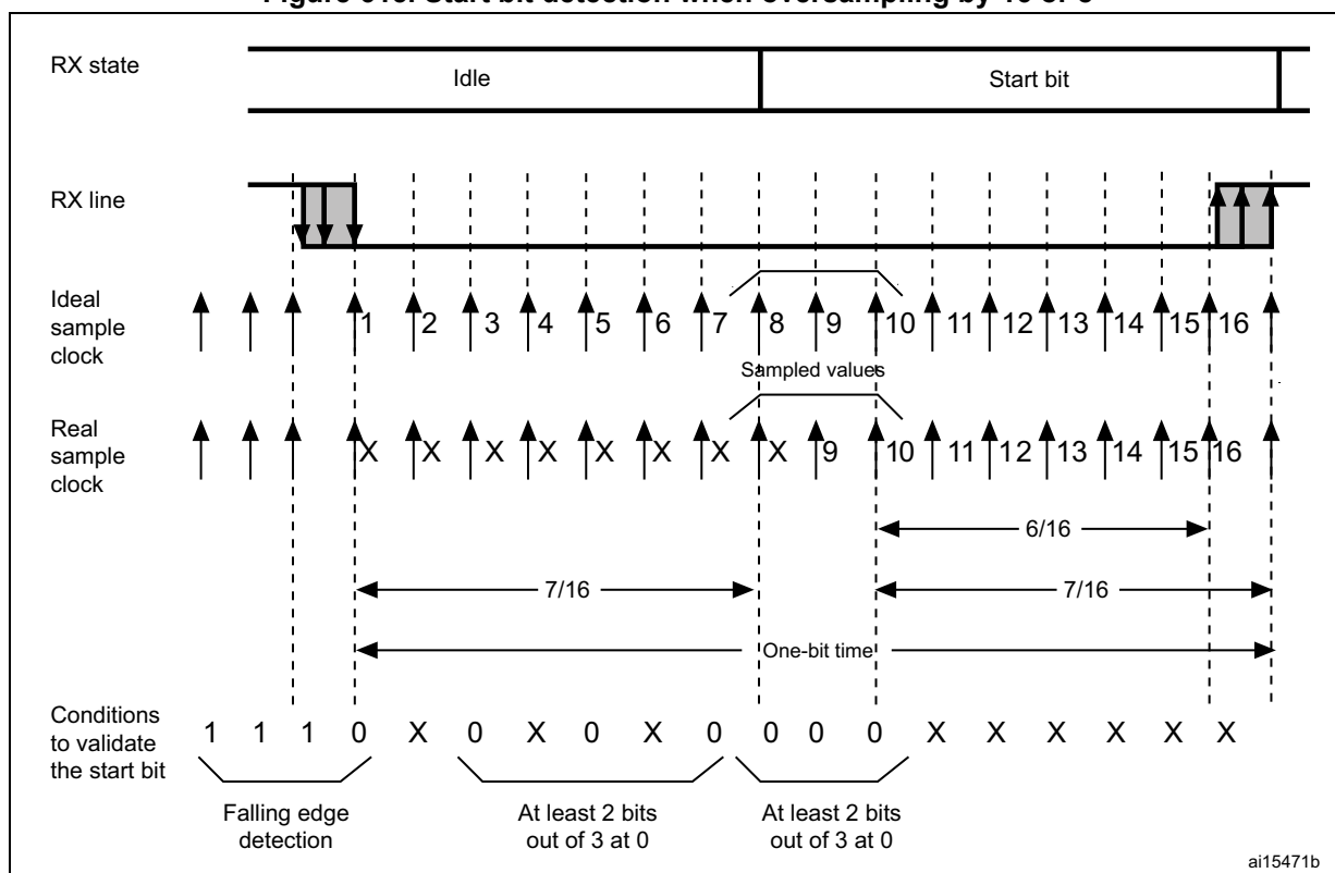
Figure 615. Start bit detection when oversampling by 16 or 8
