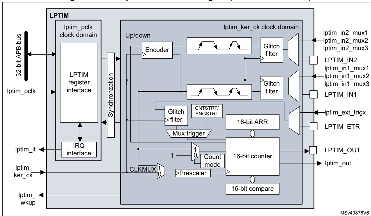
Figure 564. Low-power timer block diagram (LPTIM1 and LPTIM2)
