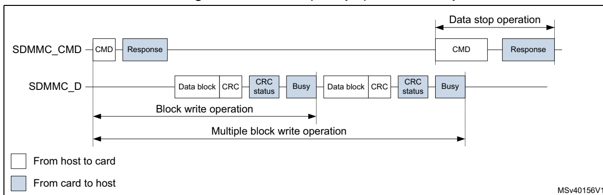
Figure 741. SDMMC (multiple) block write operation
