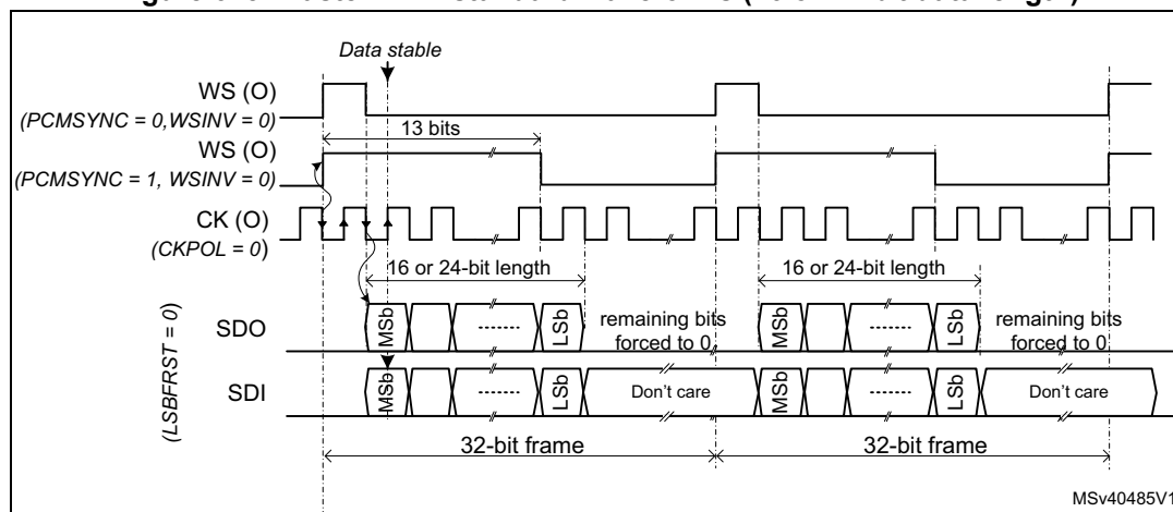
Figure 675. Master PCM standard waveforms (16 or 24-bit data length)
