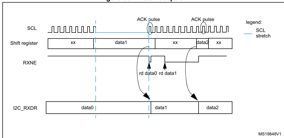
Figure 584. Data reception
