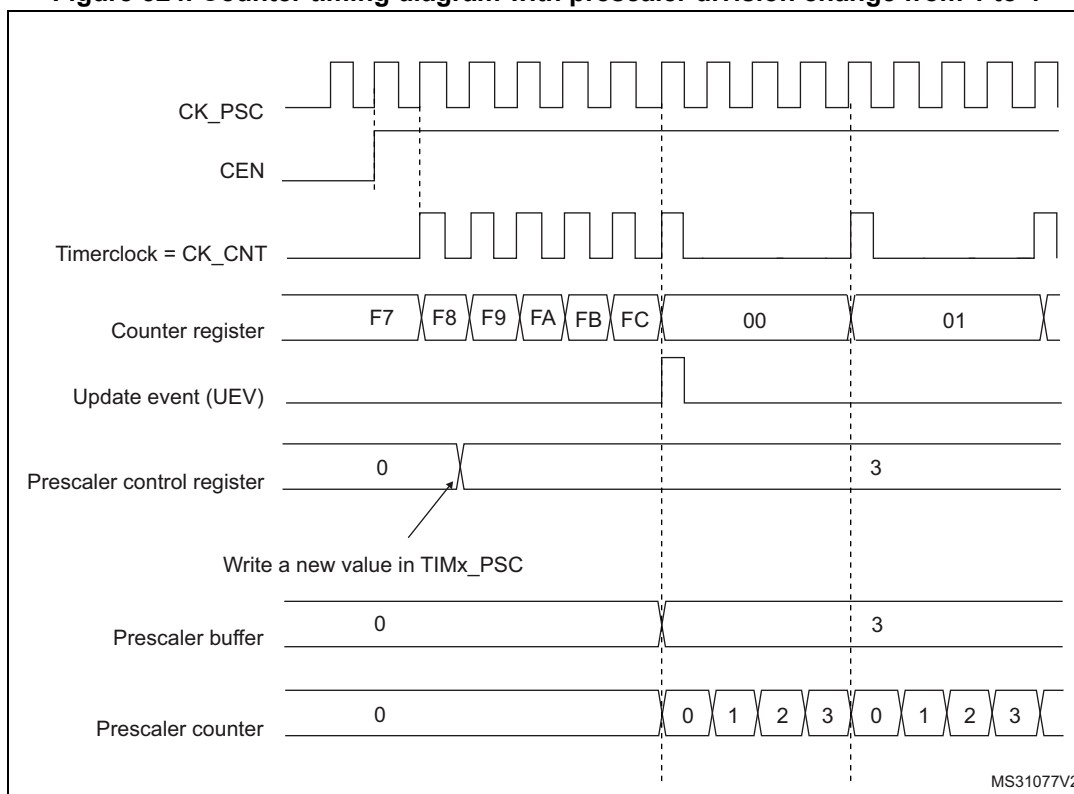
Figure 524. Counter timing diagram with prescaler division change from 1 to 4
