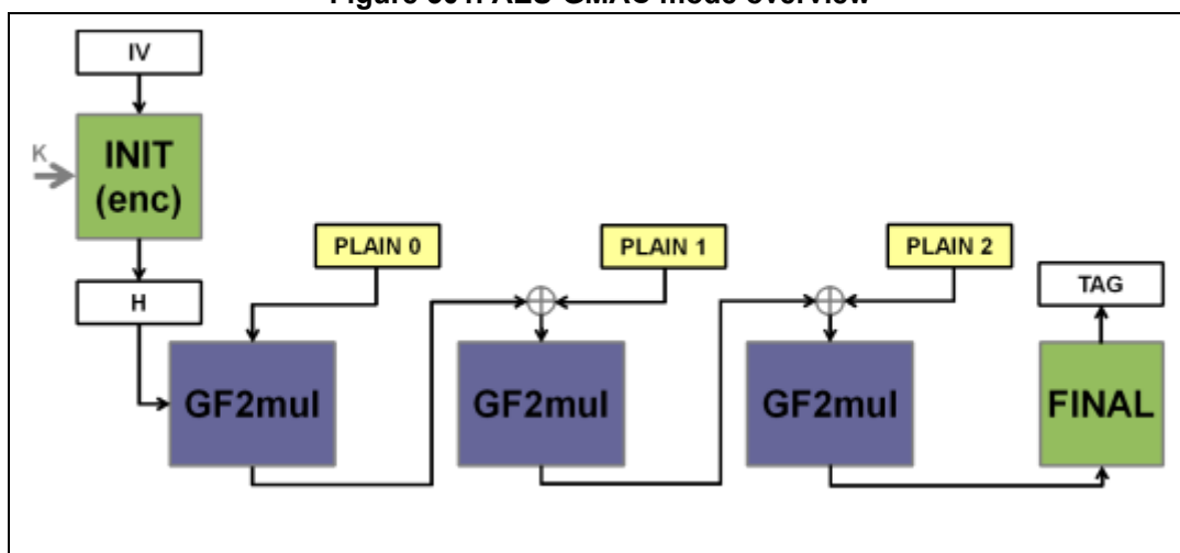
Figure 301. AES-GMAC mode overview
