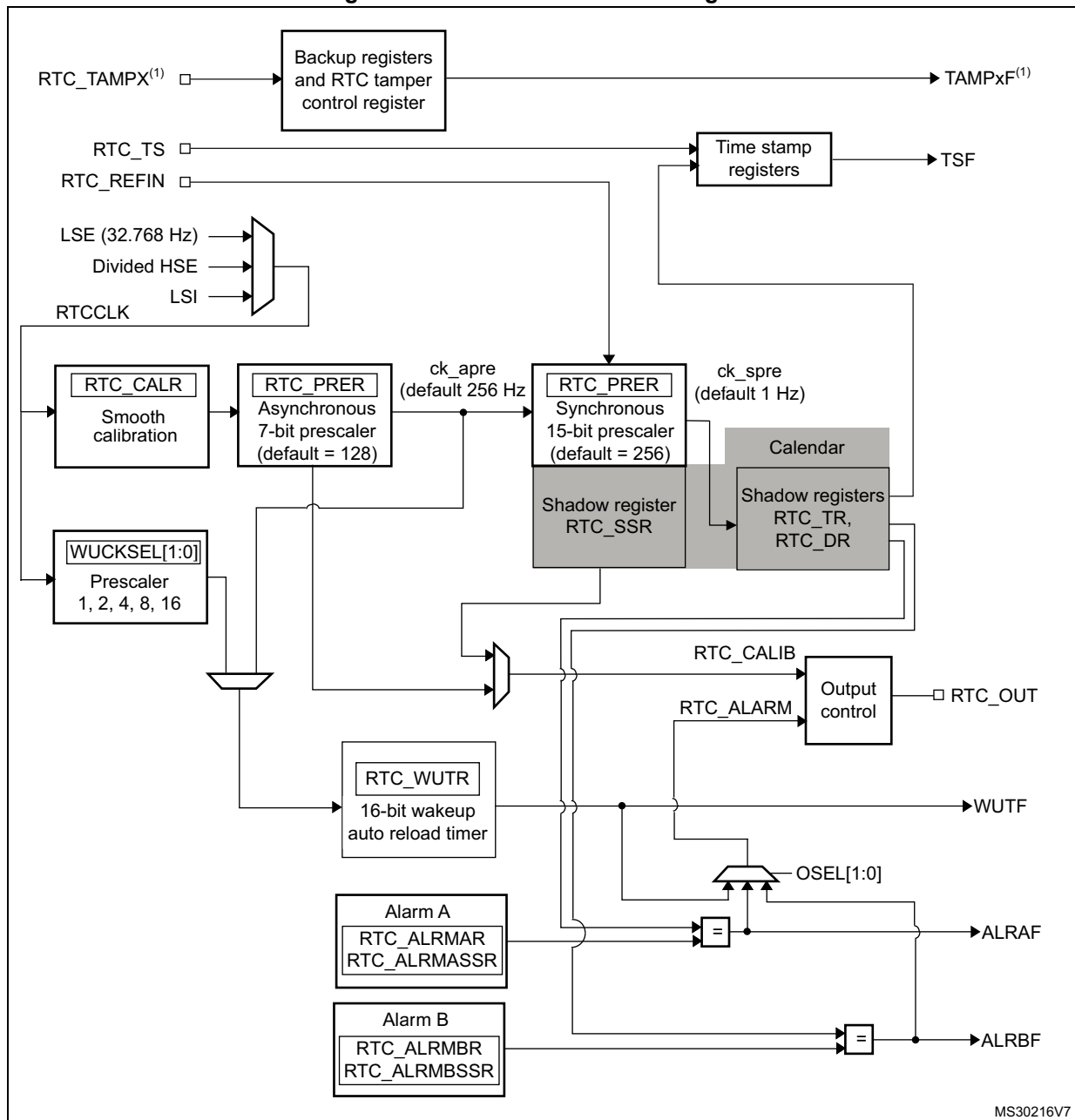
Figure 578. Detailed RTC block diagram
