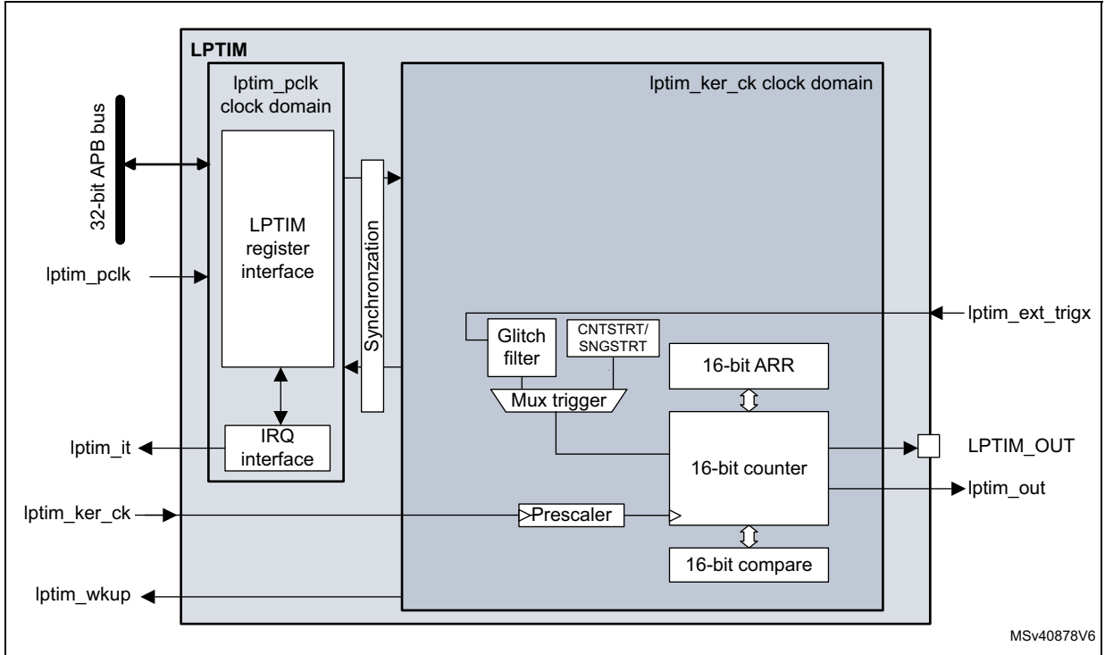
Figure 566. Low-power timer block diagram (LPTIM4 and LPTIM5)
