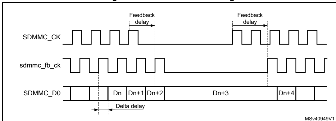
Figure 754. Hardware flow timing
