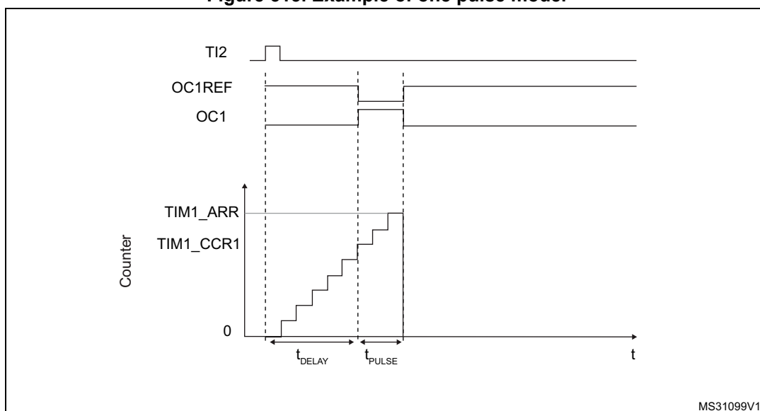
Figure 515. Example of one pulse mode.
