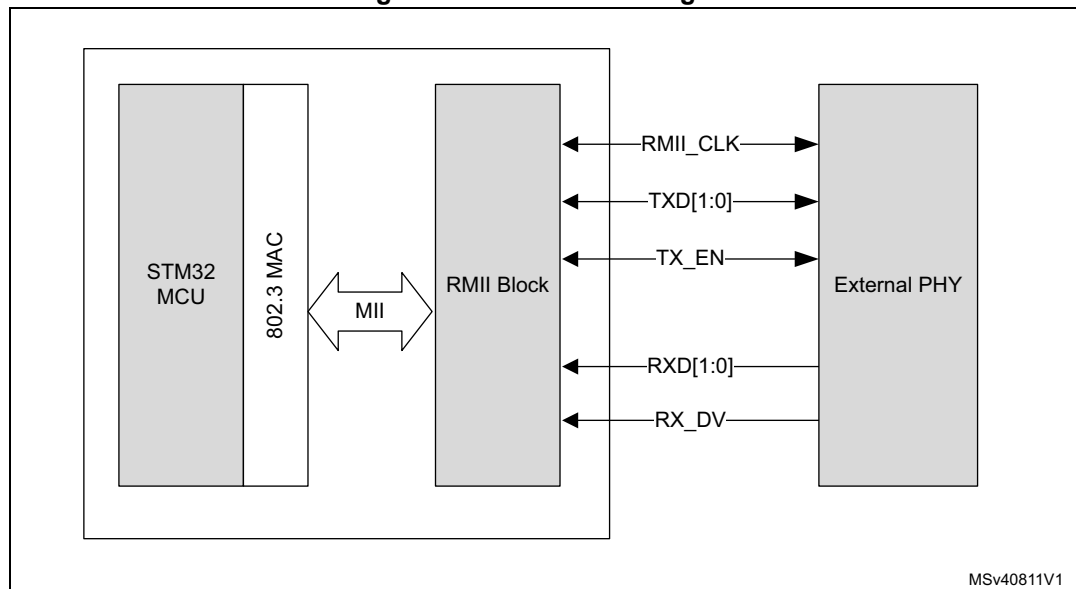
Figure 837. RMII block diagram
