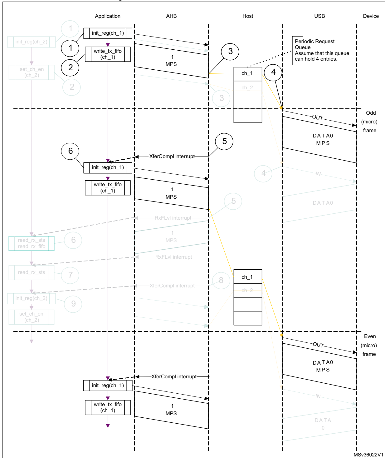
Figure 803. Isochronous OUT transactions
