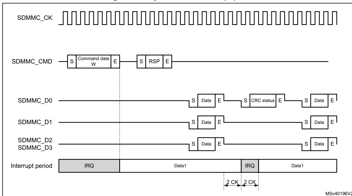
Figure 757. Synchronous interrupt period data write
