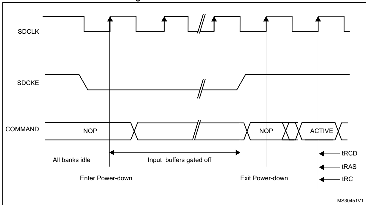
Figure 131. Power-down mode
