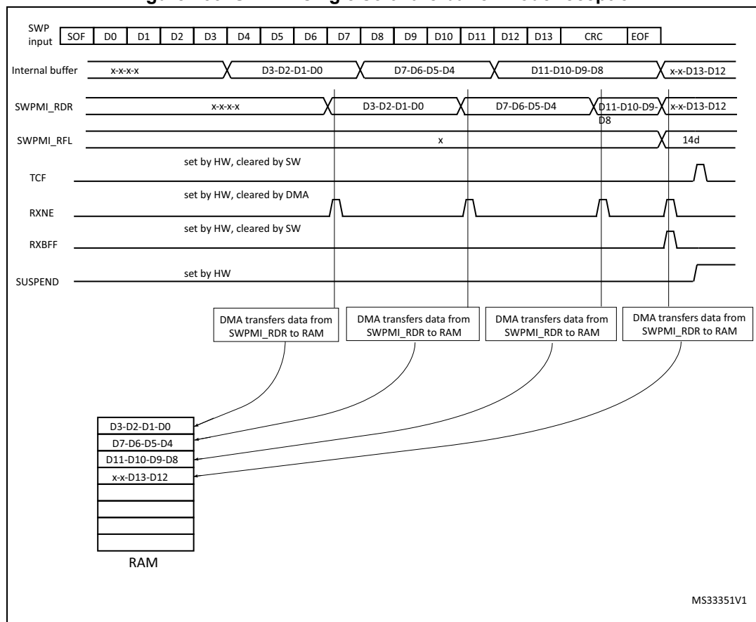
Figure 733. SWPMI single software buffer mode reception
