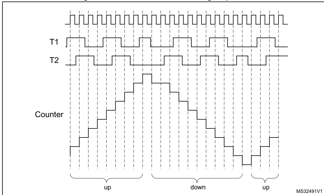
Figure 572. Encoder mode counting sequence
