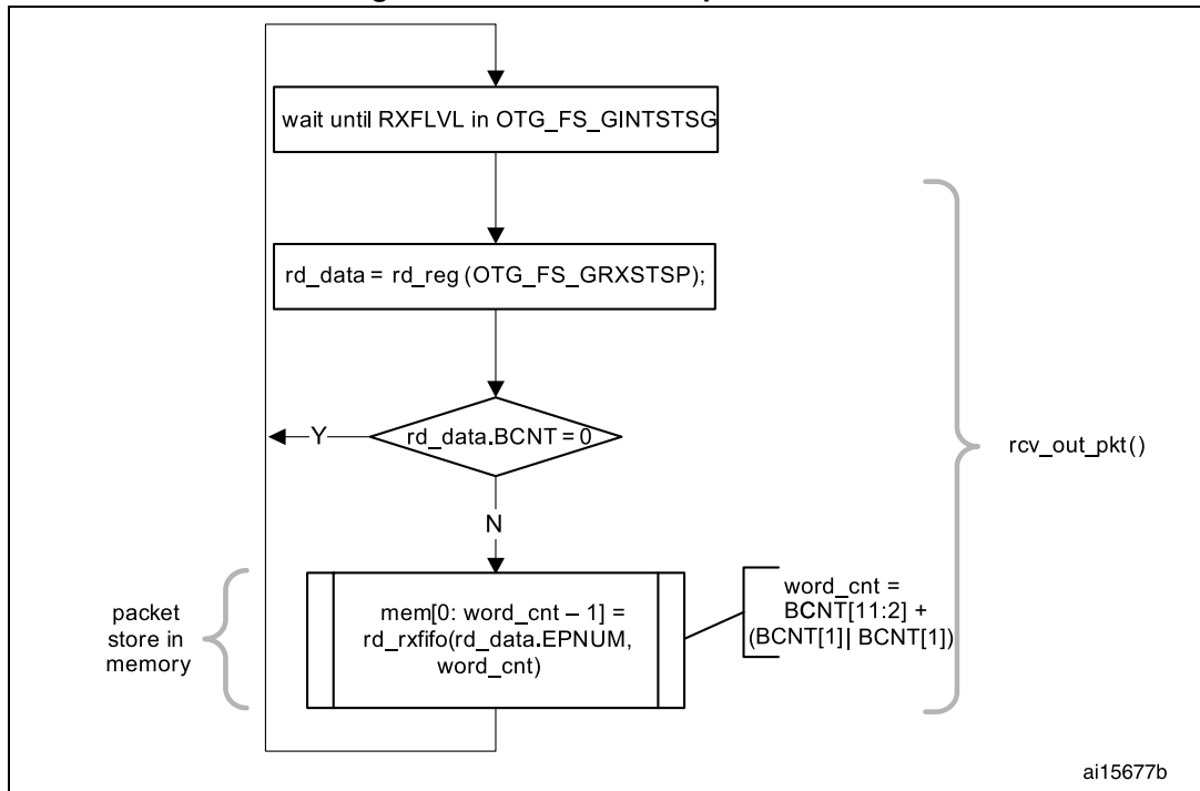
Figure 811. Receive FIFO packet read
