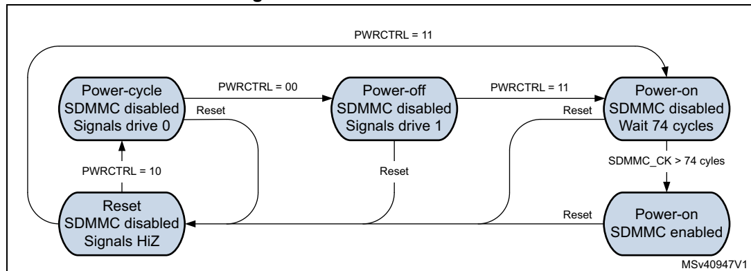
Figure 769. SDMMC state control
