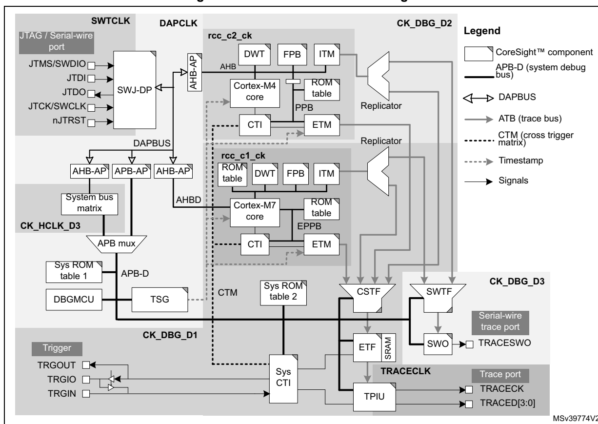
Figure 861. Clock domains of debug infrastructure
