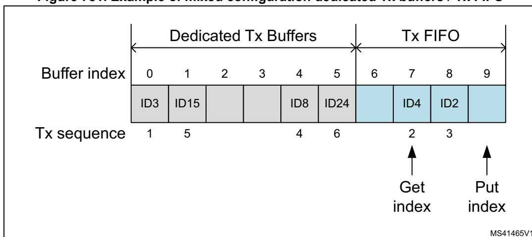
Figure 781. Example of mixed configuration dedicated Tx buffers / Tx FIFO
