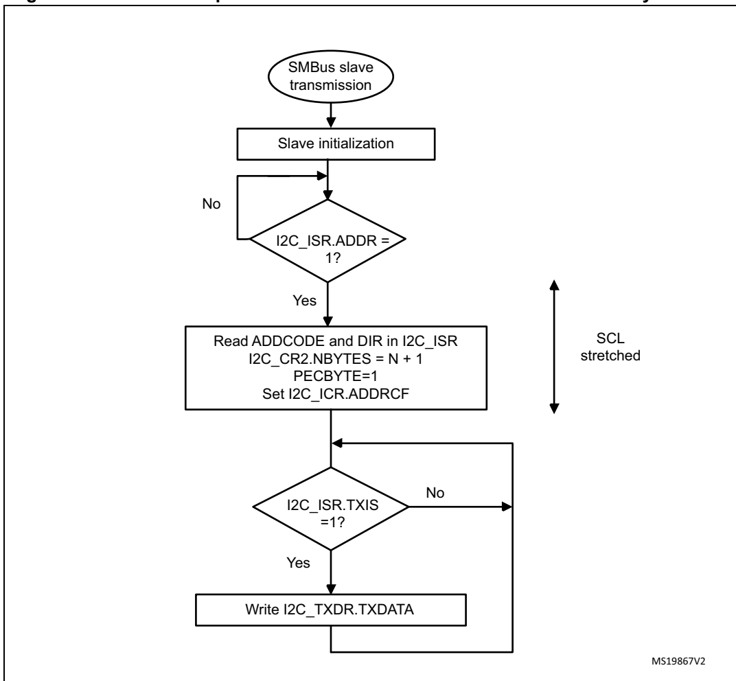
Figure 604. Transfer sequence flowchart for SMBus slave transmitter N bytes + PEC
