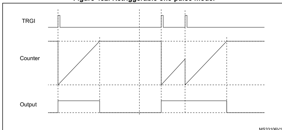
Figure 482. Retriggerable one-pulse mode.
