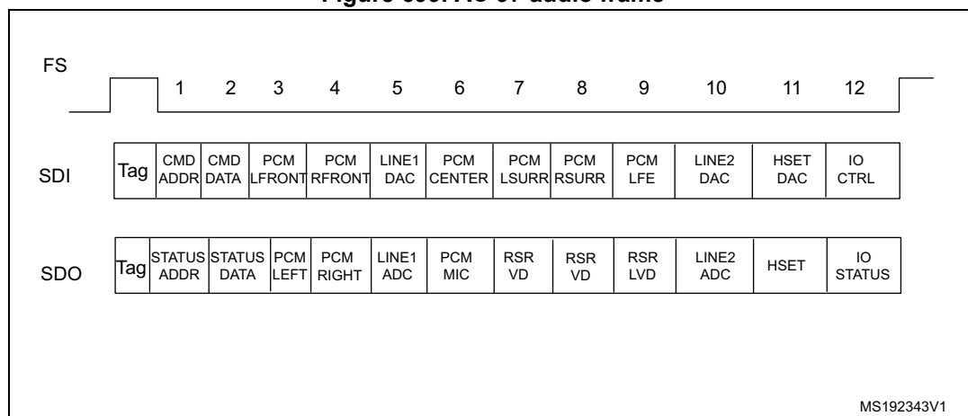
Figure 699. AC'97 audio frame
