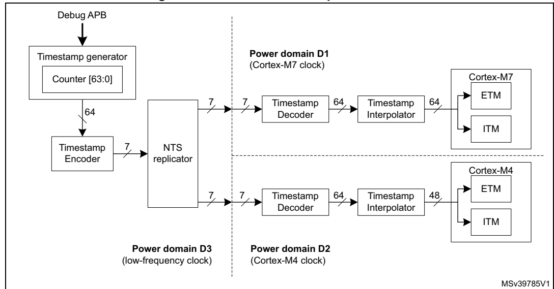
Figure 866. Global timestamp distribution
