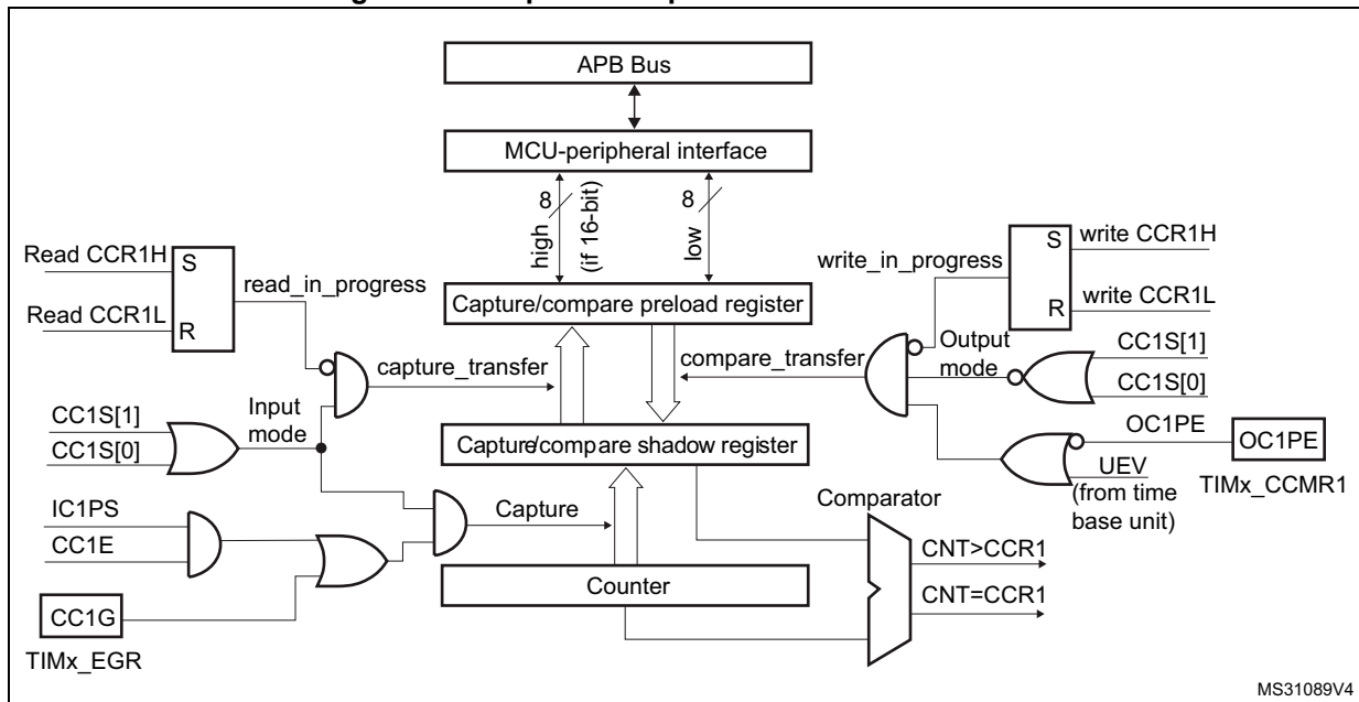
Figure 536. Capture/compare channel 1 main circuit
