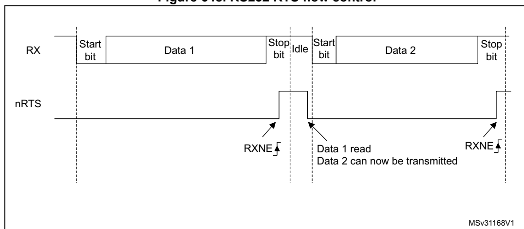
Figure 648. RS232 RTS flow control
