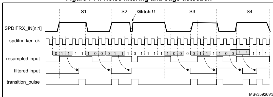
Figure 714. Noise filtering and edge detection
