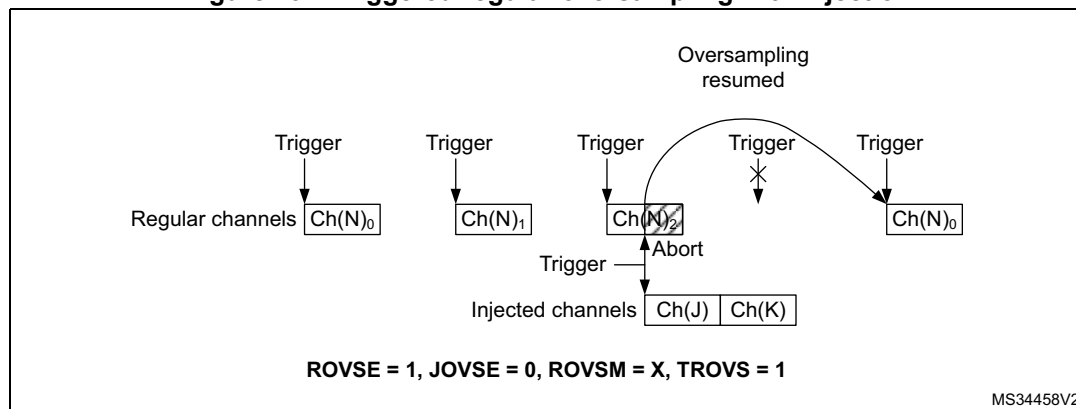
Figure 191. Triggered regular oversampling with injection
