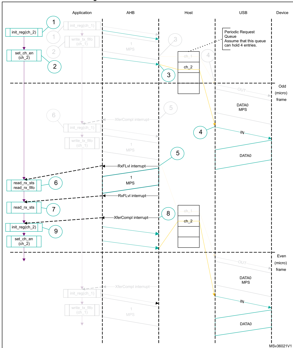
Figure 804. Isochronous IN transactions
