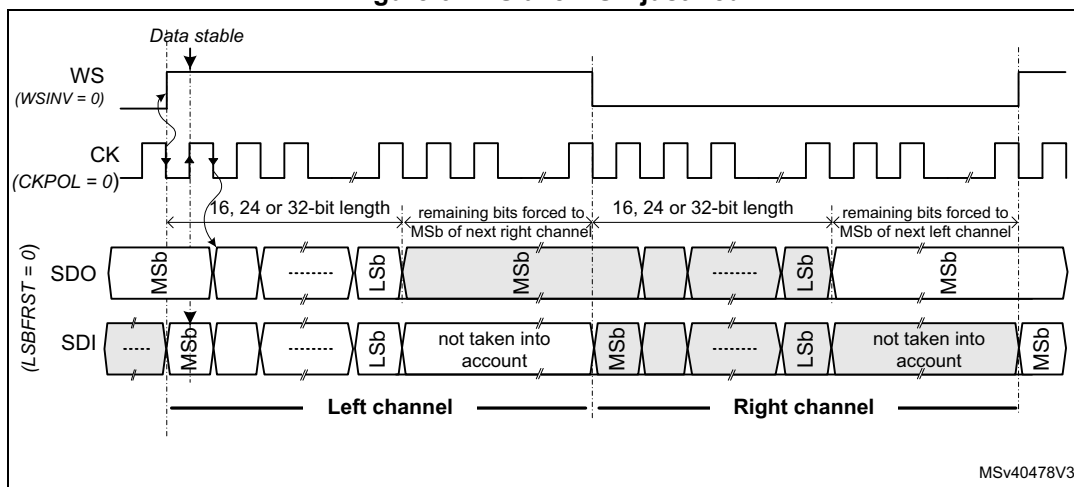
Figure 672. Slave MSB justified
