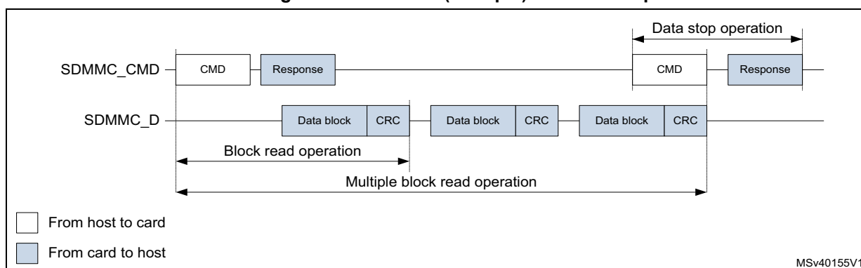
Figure 740. SDMMC (multiple) block read operation
