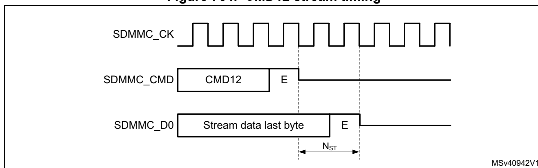
Figure 764. CMD12 stream timing
