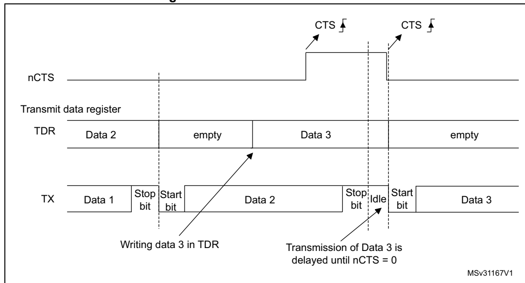
Figure 649. RS232 CTS flow control
