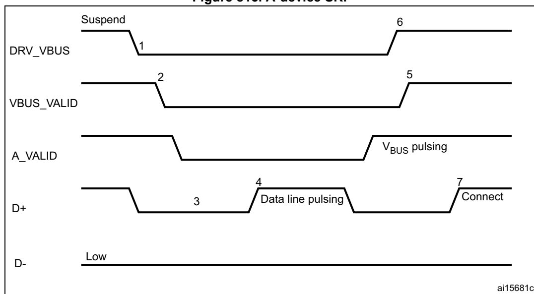
Figure 815. A-device SRP
