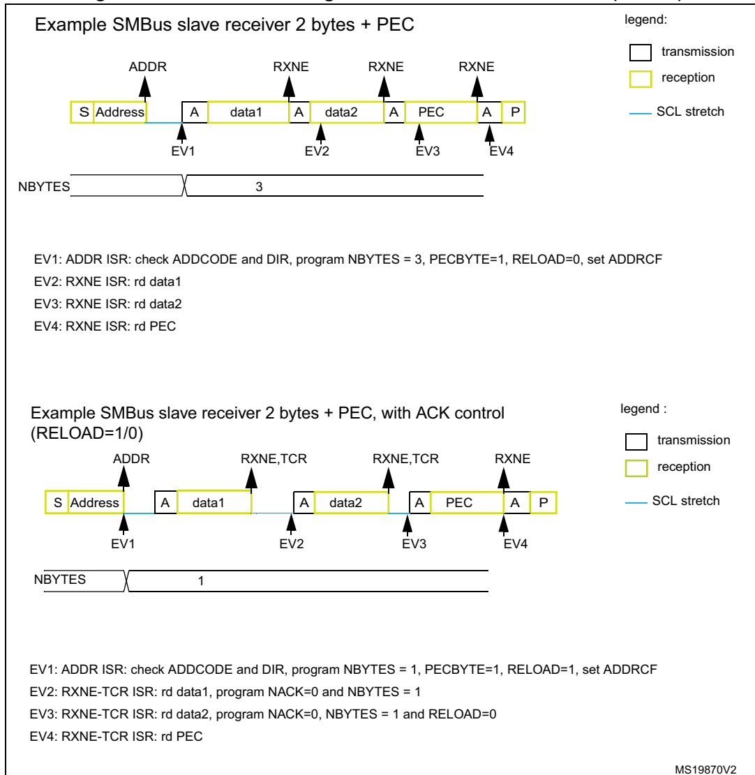
Figure 607. Bus transfer diagrams for SMBus slave receiver (SBC=1)
