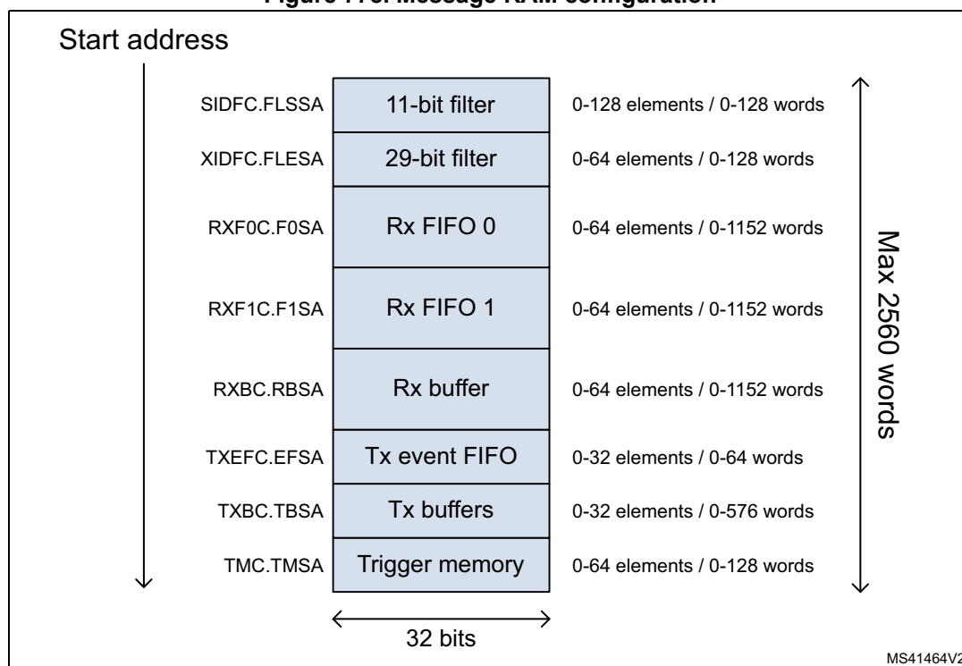
Figure 778. Message RAM configuration
