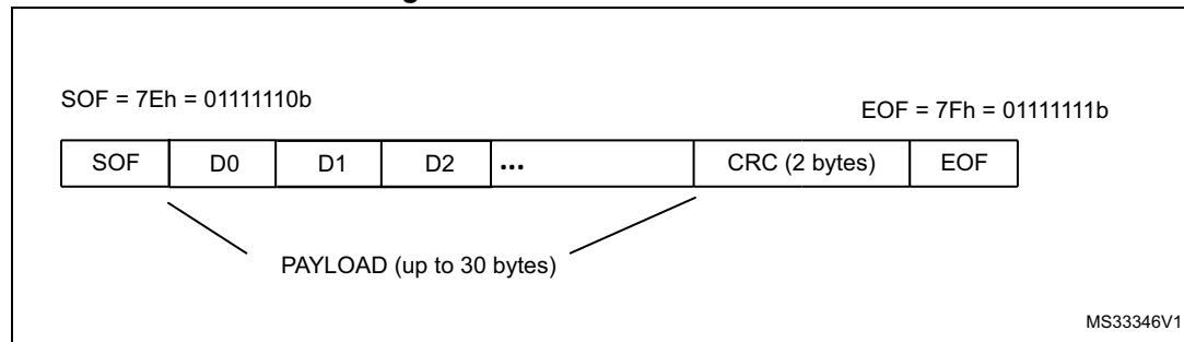
Figure 728. SWP frame structure
