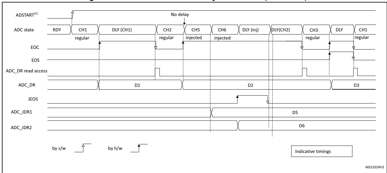
Figure 181. AUTDLY=1 in auto-injected mode (JAUTO=1)
