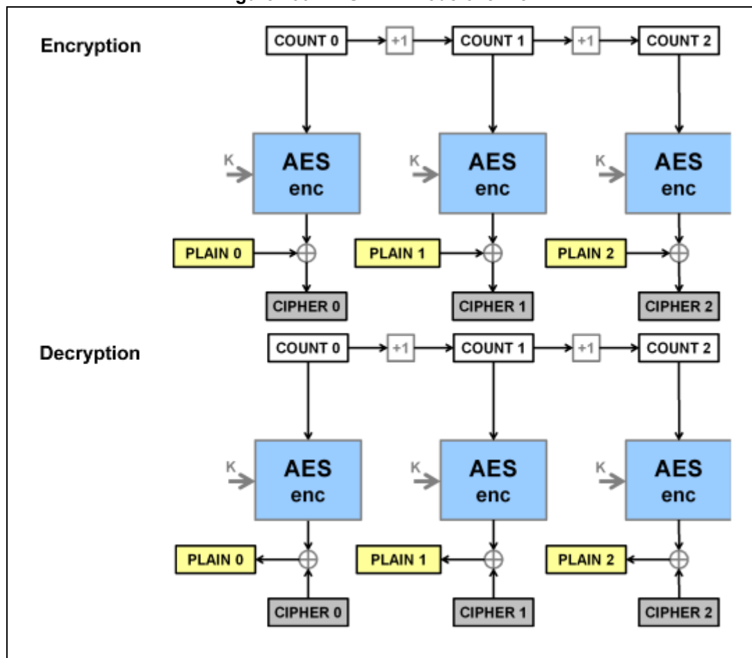
Figure 299. AES-CTR mode overview
