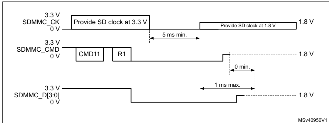
Figure 771. CMD11 signal voltage switch sequence
