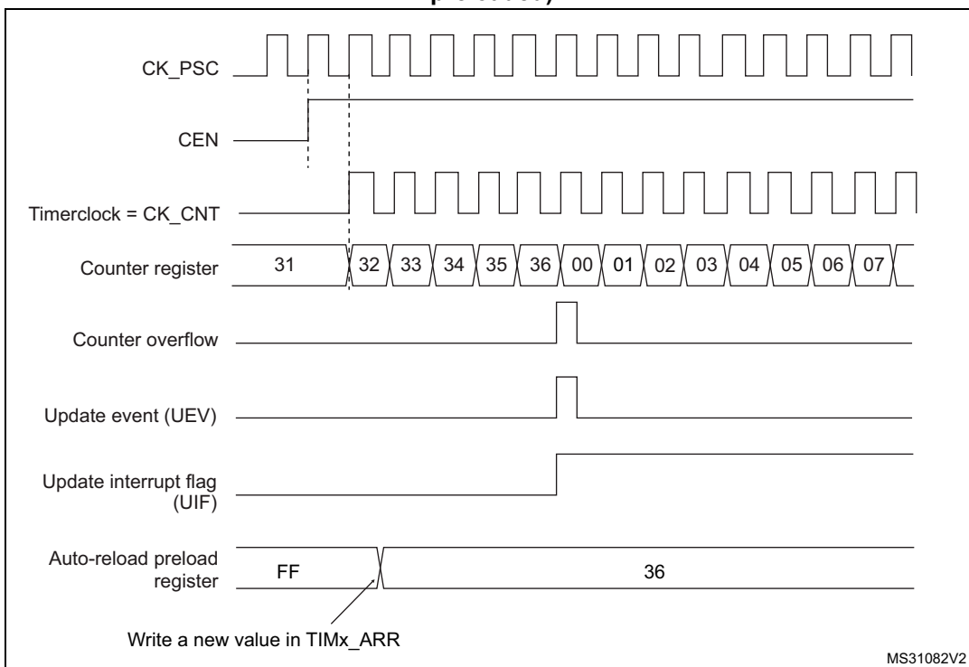
Figure 503. Counter timing diagram, update event when ARPE=0 (TIMx_ARR not preloaded)
