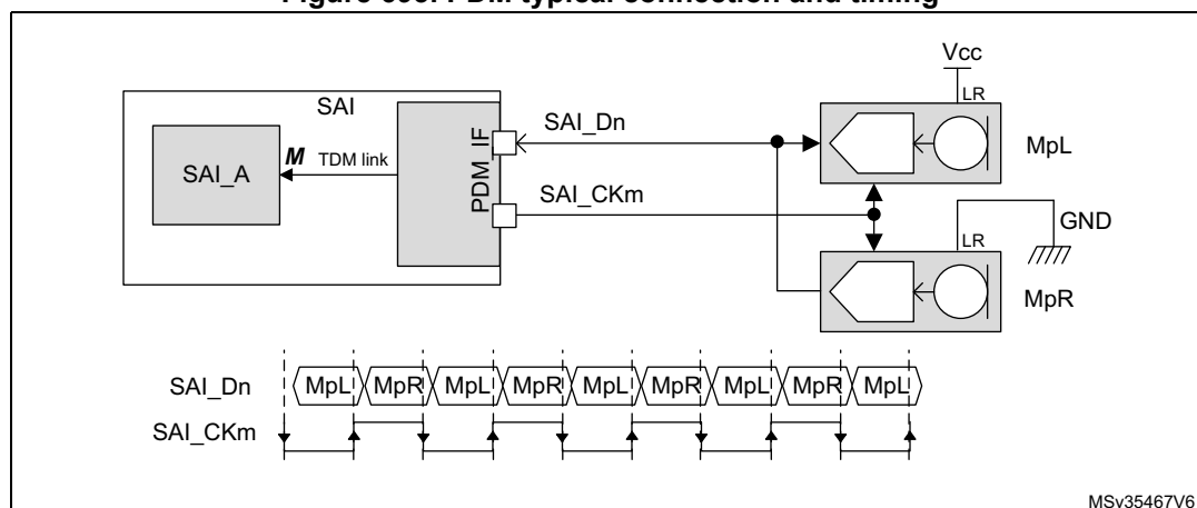
Figure 693. PDM typical connection and timing
