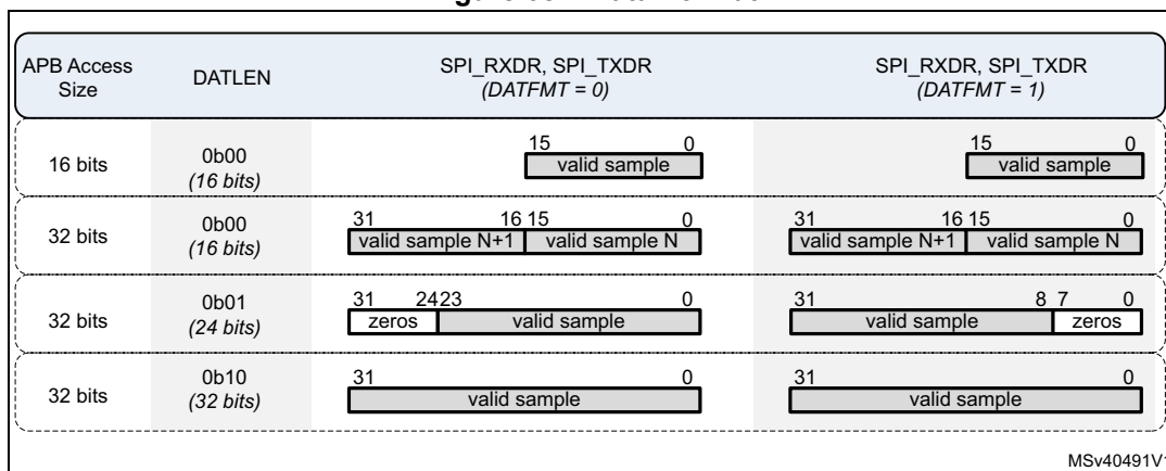
Figure 681. Data Format
