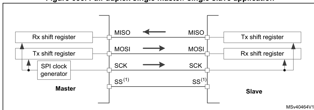
Figure 653. Full-duplex single master/ single slave application
