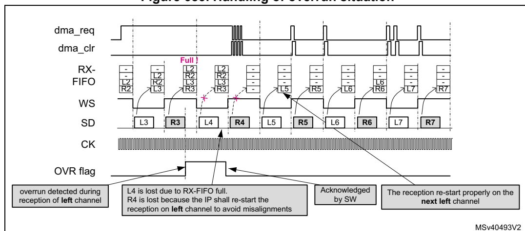
Figure 683. Handling of overrun situation
