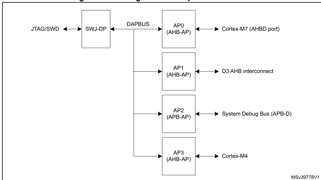
Figure 864. Debug and access port connections
