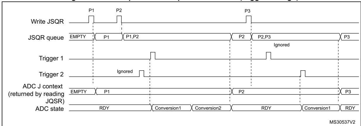
Figure 156. Example of JSQR queue of context (trigger change)
