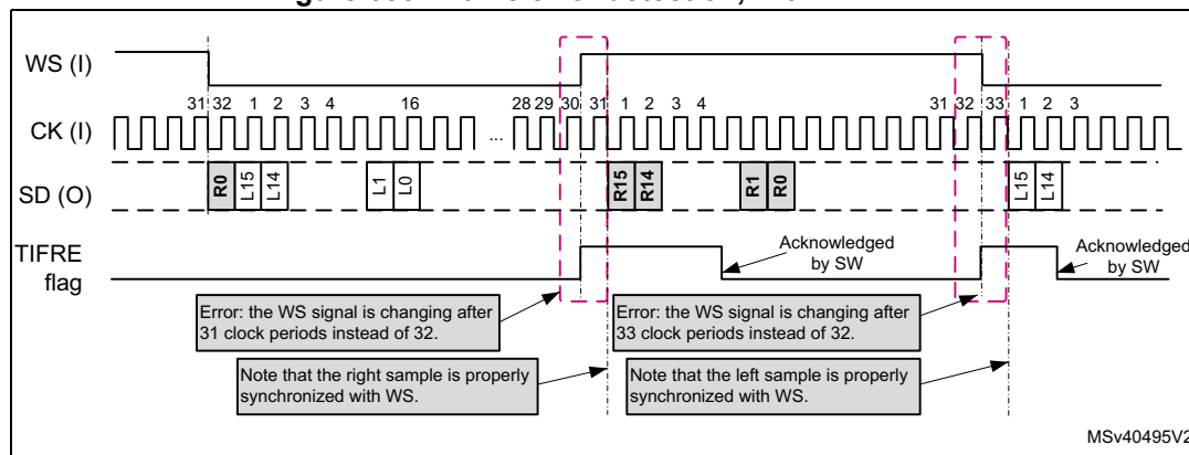
Figure 685. Frame error detection, with FIXCH=1
