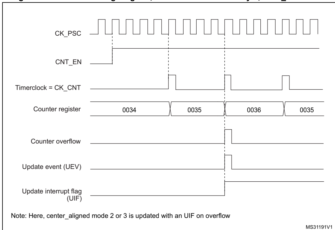
Figure 462. Counter timing diagram, internal clock divided by 4, TIMx_ARR=0x36
