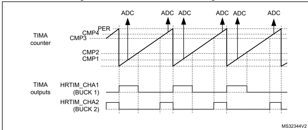
Figure 379. Dual Buck converter management
