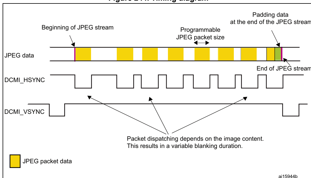
Figure 244. Timing diagram
