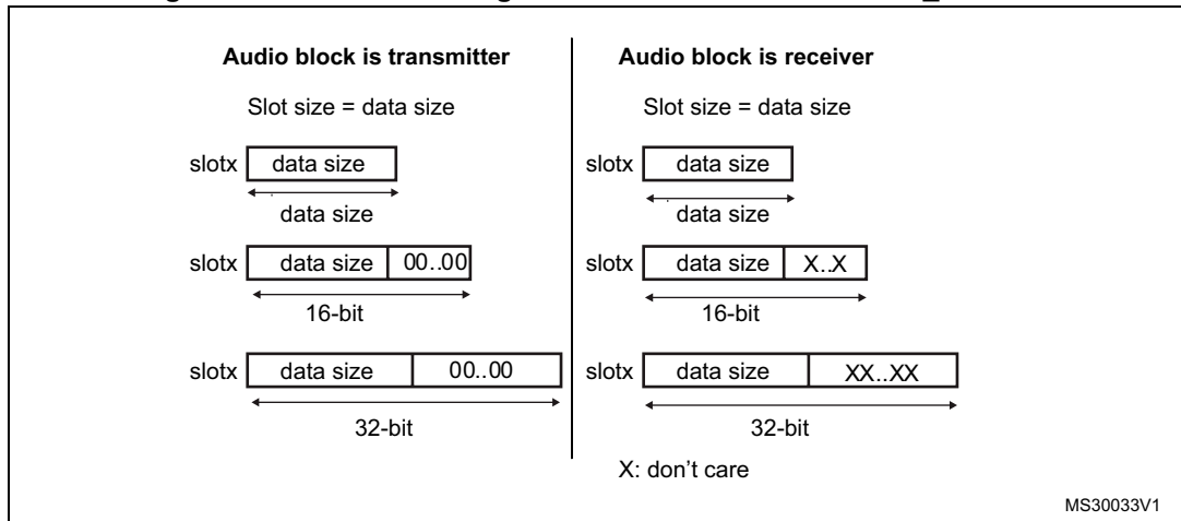
Figure 690. Slot size configuration with FBOFF = 0 in SAI_xSLOTR
