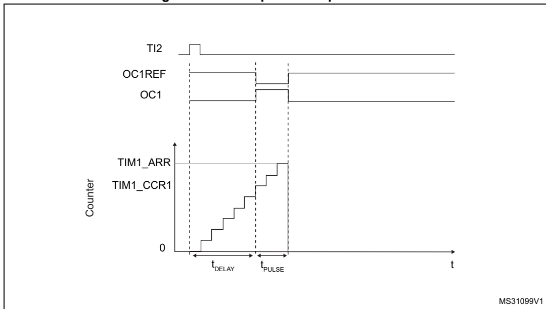
Figure 548. Example of one pulse mode
