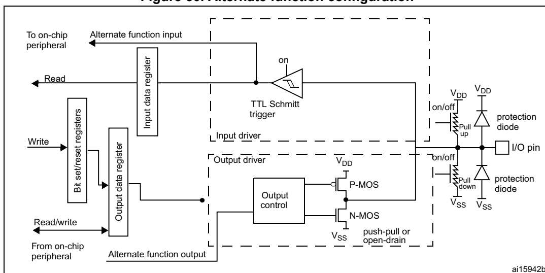
Figure 80. Alternate function configuration
