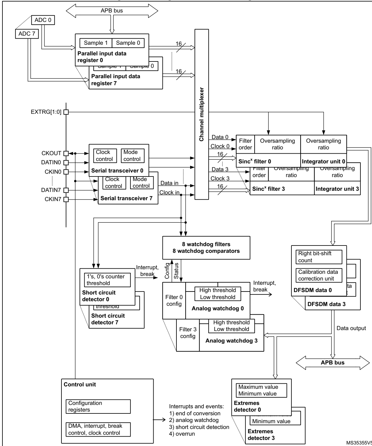
Figure 234. Single DFSDM block diagram
