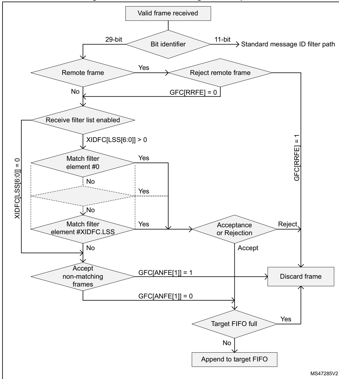
Figure 780. Extended message ID filter path
