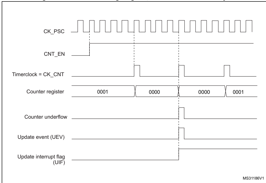
Figure 458. Counter timing diagram, internal clock divided by N
