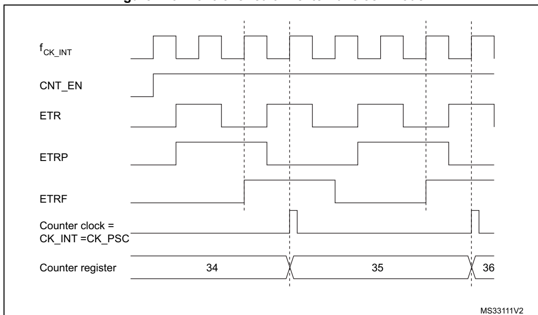
Figure 470. Control circuit in external clock mode 2
