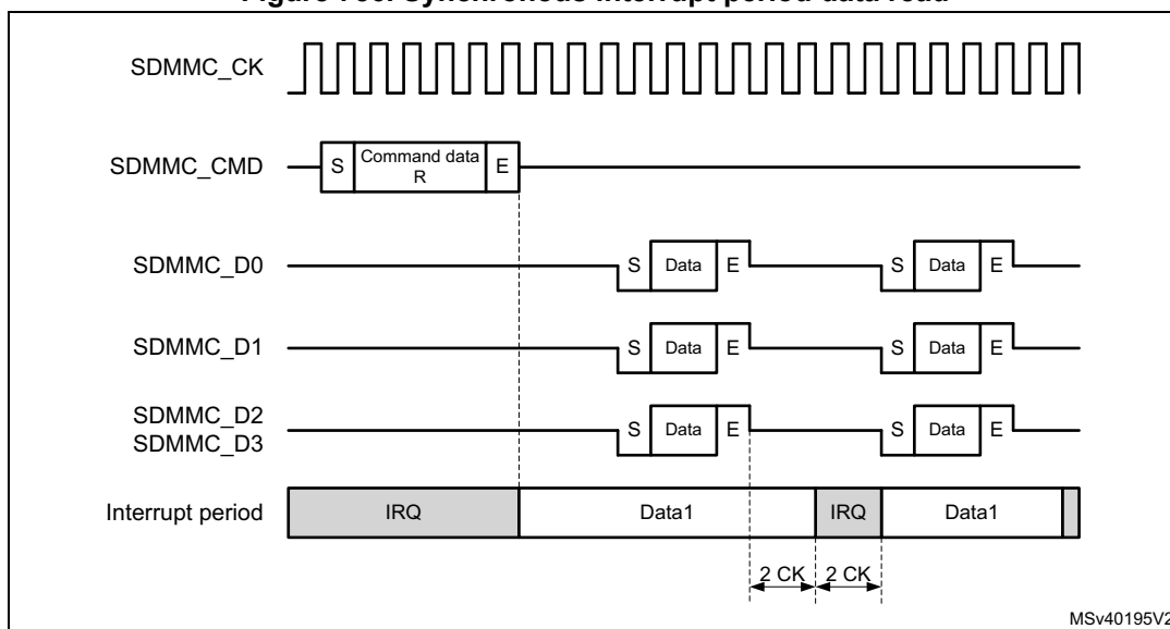
Figure 756. Synchronous interrupt period data read
