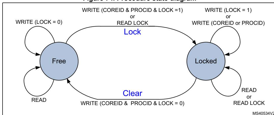
Figure 74. Procedure state diagram
