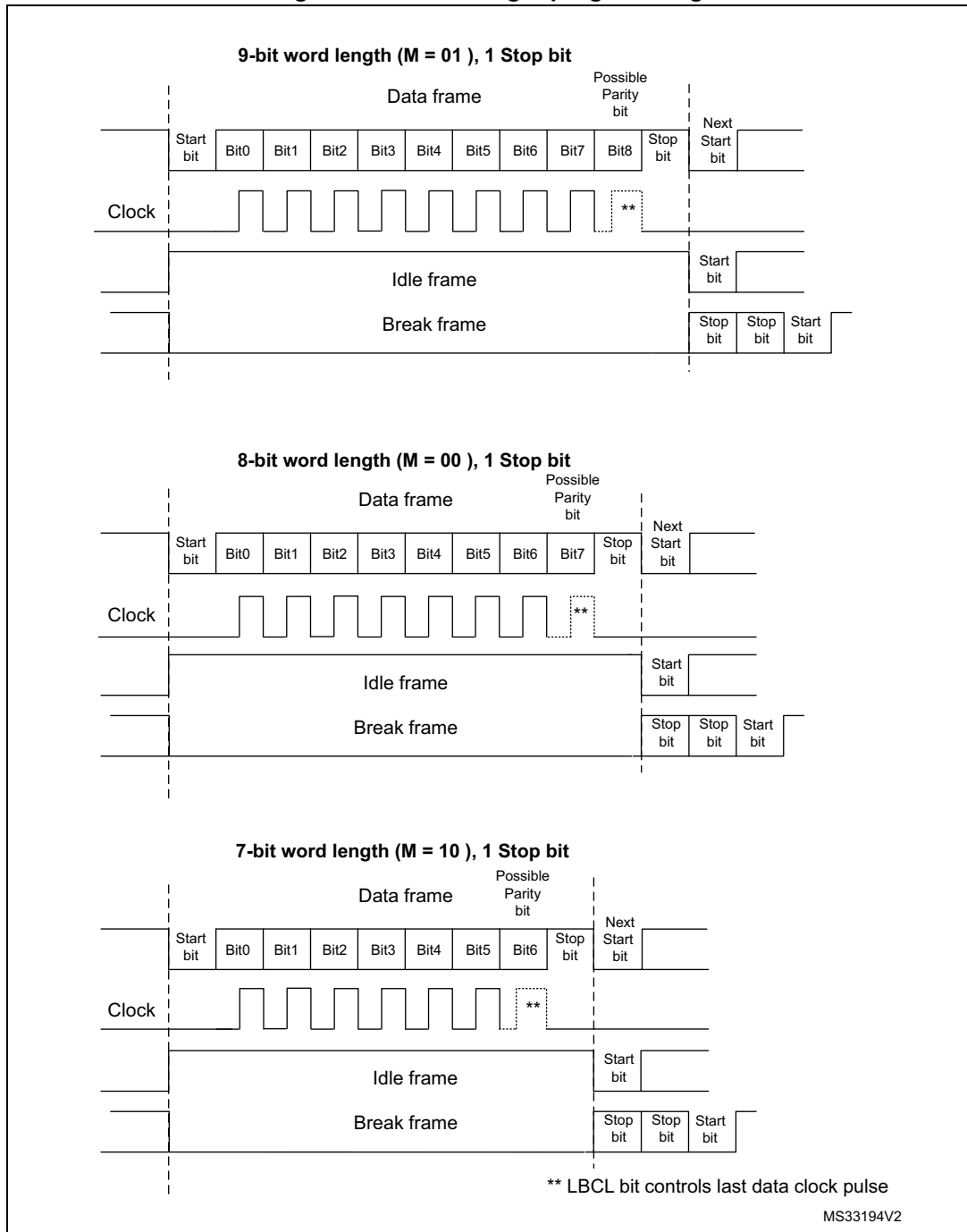
Figure 612. Word length programming
