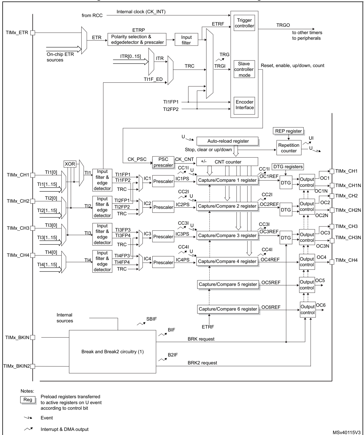
Figure 386. Advanced-control timer block diagram
