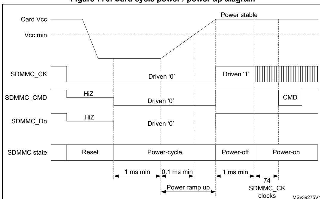
Figure 770. Card cycle power / power up diagram
