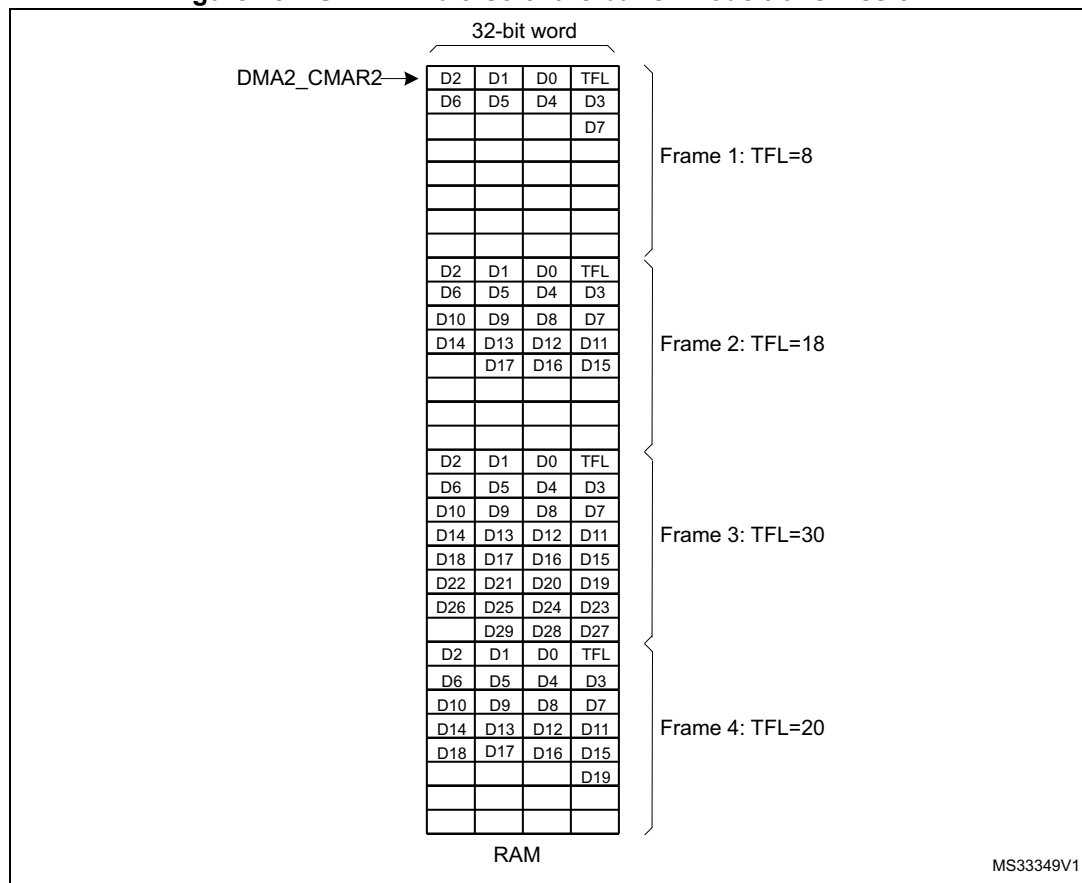
Figure 731. SWPMI Multi software buffer mode transmission
