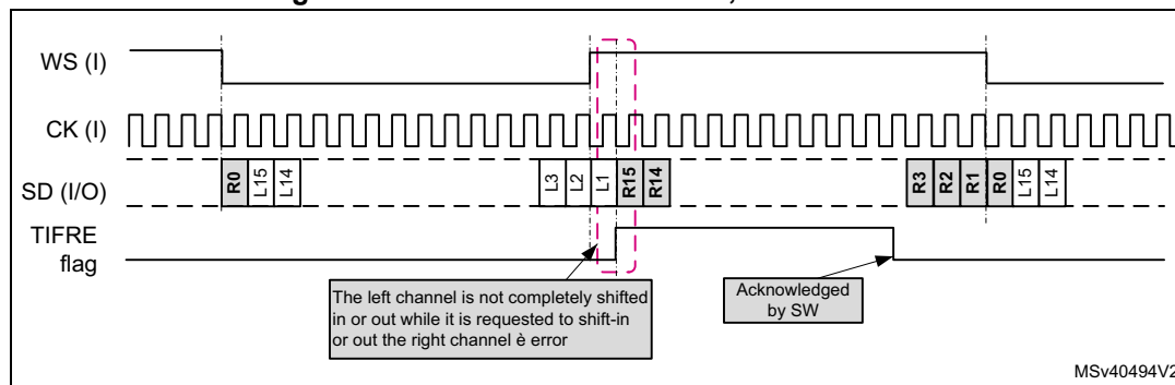
Figure 684. Frame error detection, with FIXCH=0
