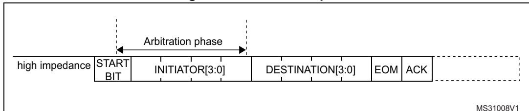
Figure 854. Arbitration phase
