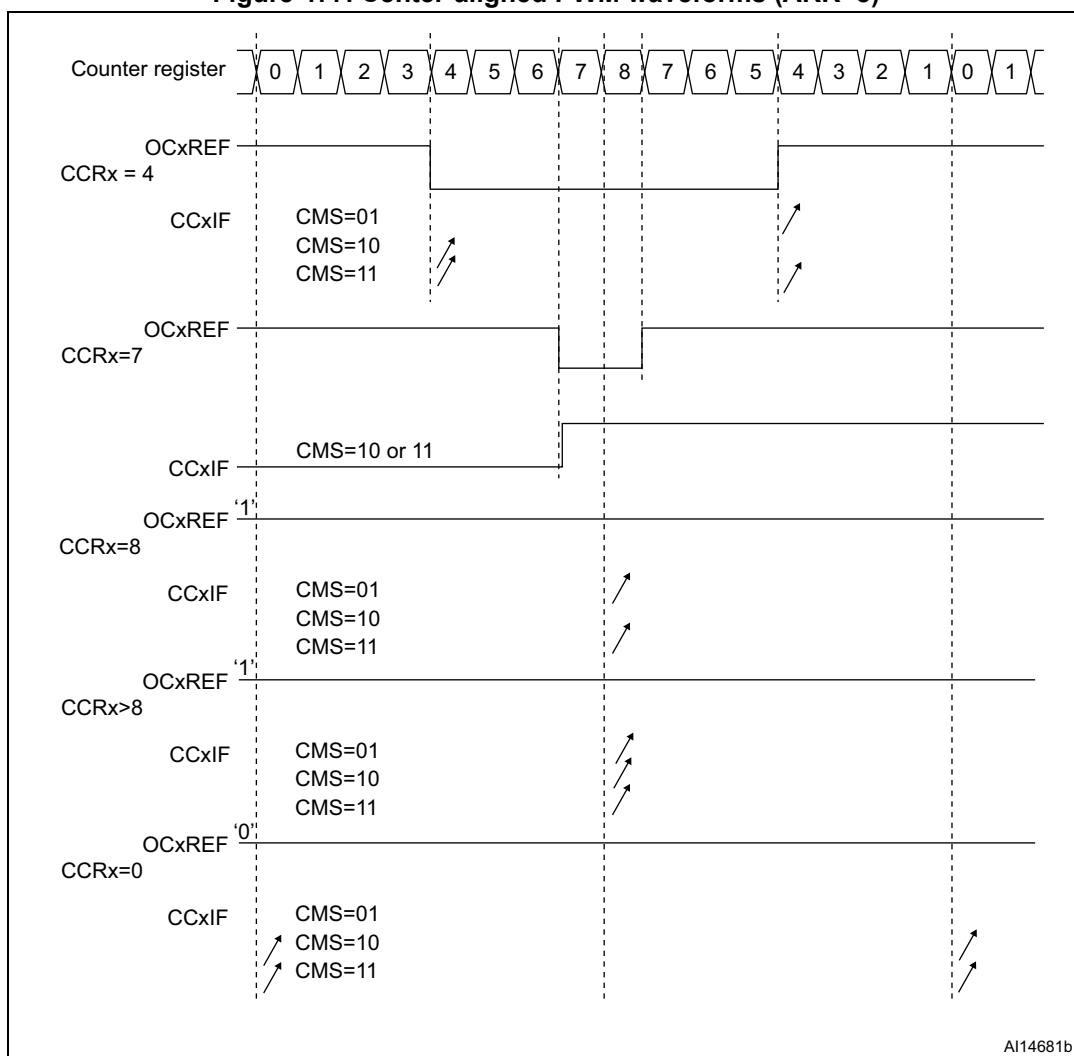
Figure 477. Center-aligned PWM waveforms (ARR=8)
