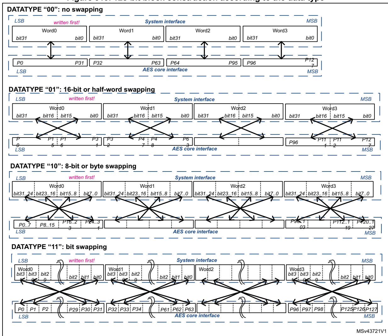
Figure 319. 128-bit block construction according to the data type
