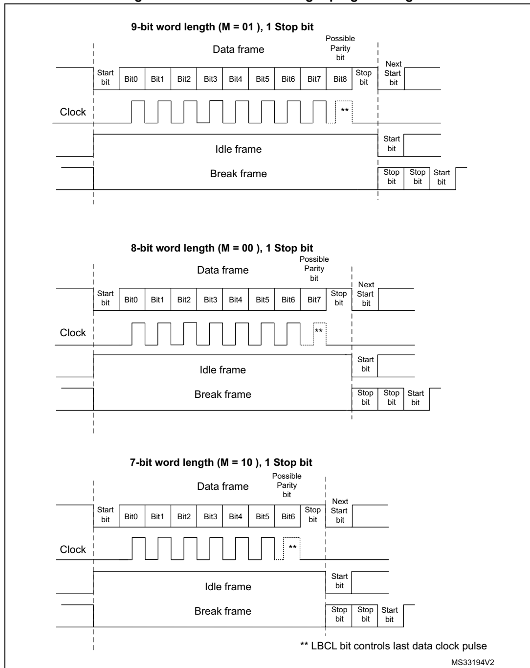
Figure 639. LPUART word length programming
