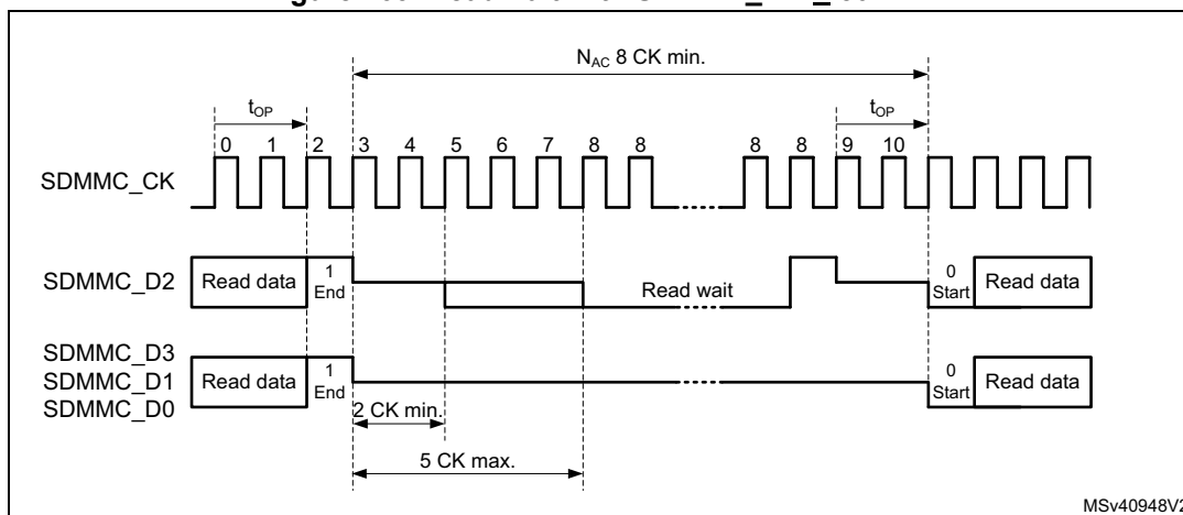
Figure 763. ReadWait with SDMMC_CK ≥ 50 MHz
