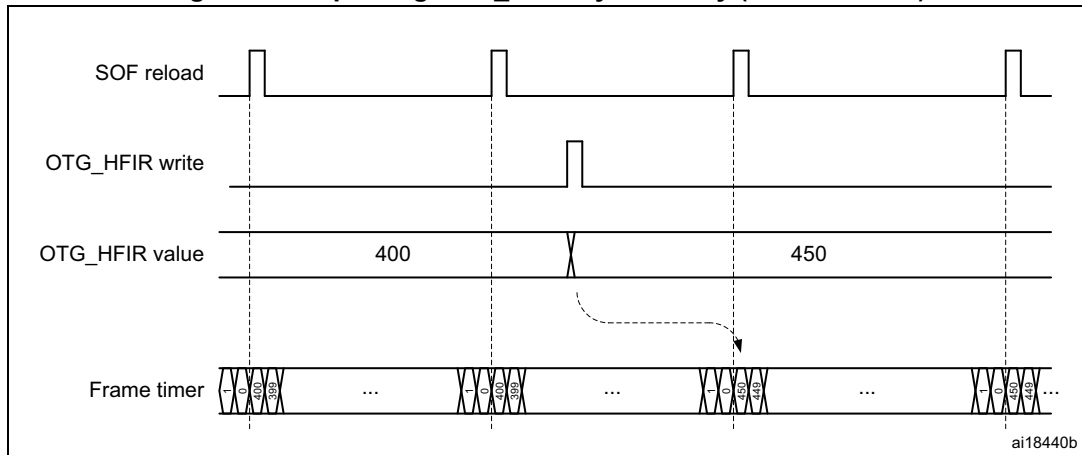
Figure 793. Updating OTG_HFIR dynamically (RLDCTRL = 1)
