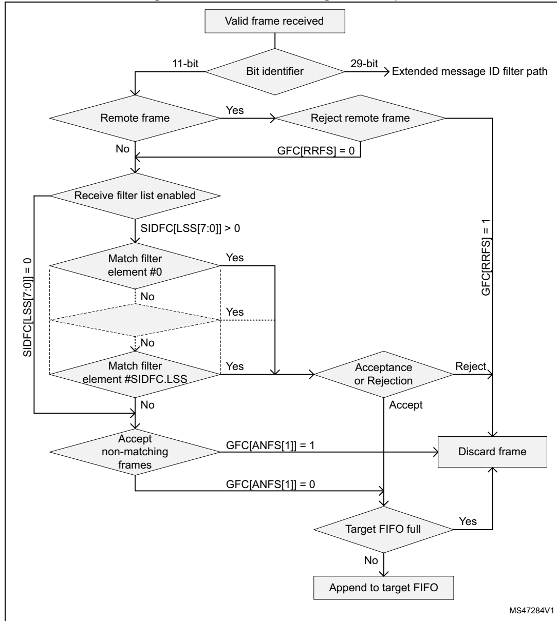
Figure 779. Standard message ID filter path
