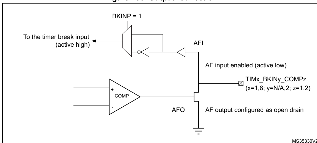
Figure 433. Output redirection
