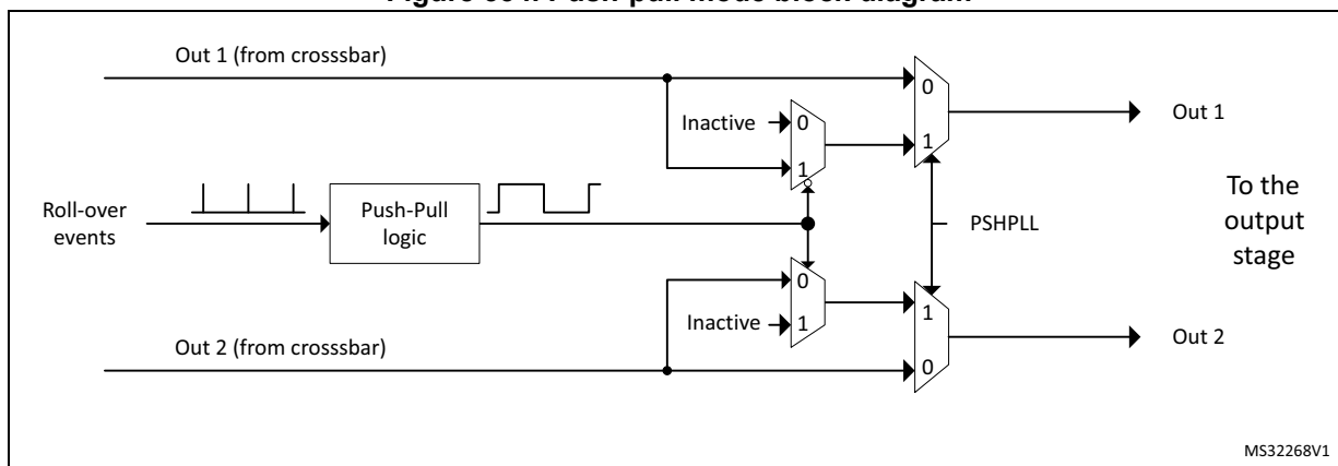
Figure 334. Push-pull mode block diagram
