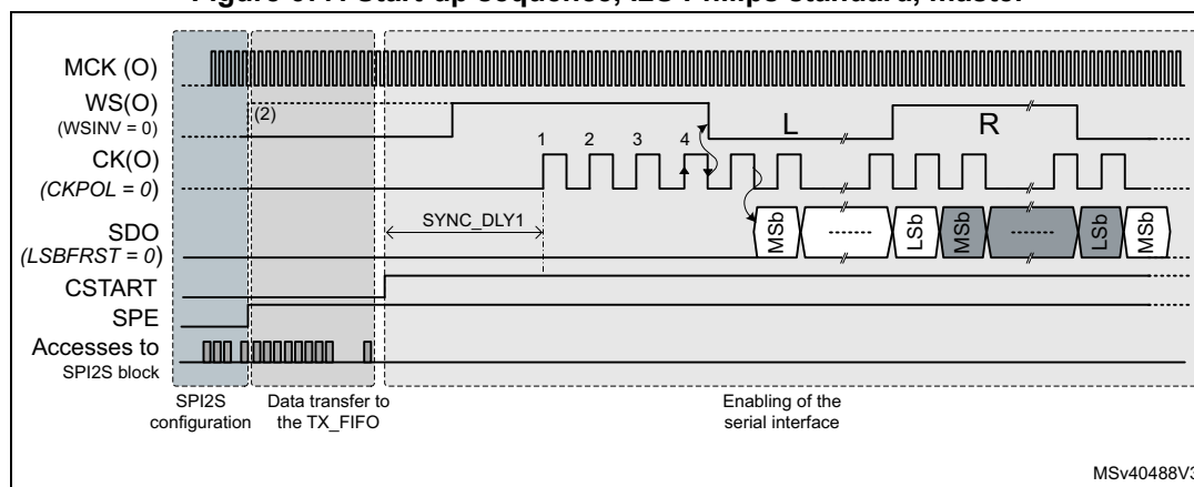
Figure 677. Start-up sequence, I2S Philips standard, master
