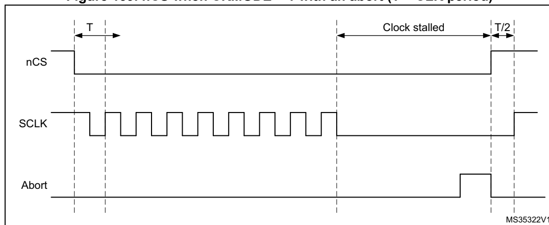
Figure 139. nCS when CKMODE = 1 with an abort (T = CLK period)
