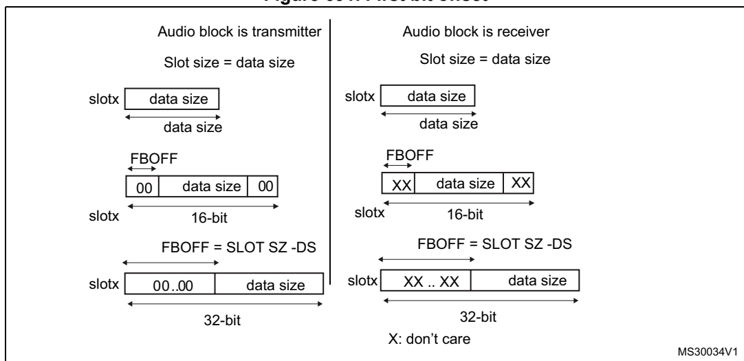
Figure 691. First bit offset
