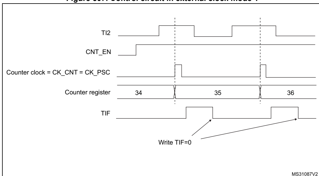
Figure 507. Control circuit in external clock mode 1
