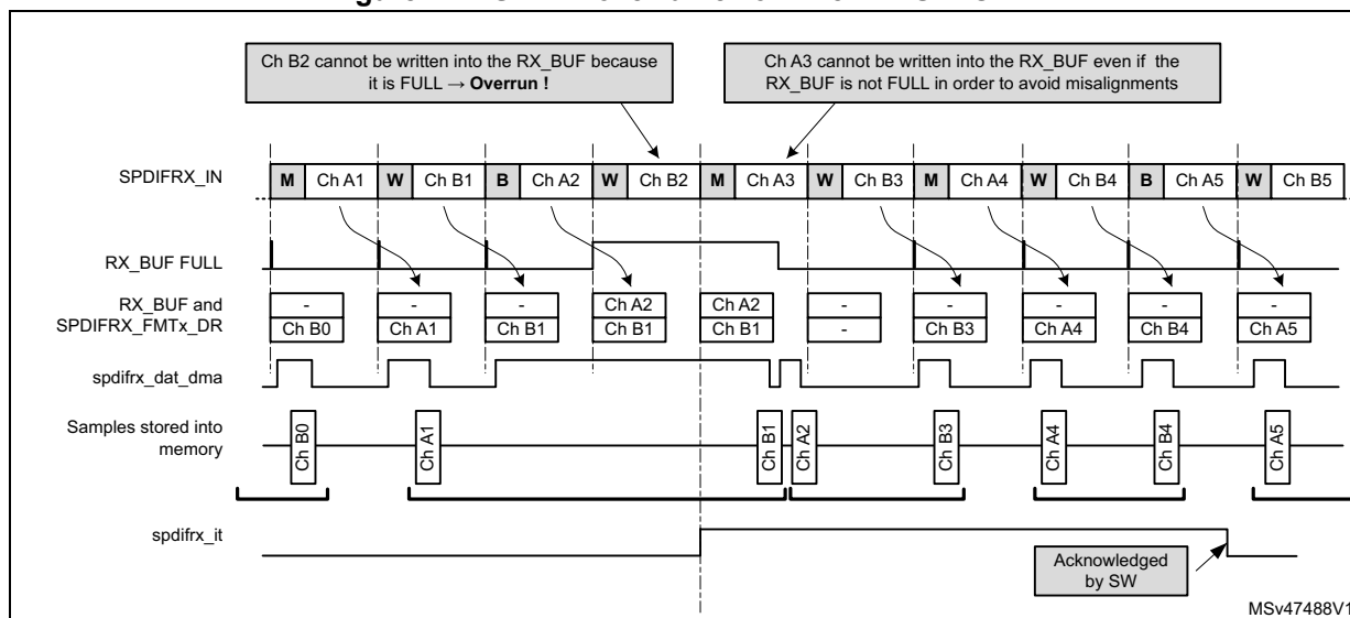
Figure 722. S/PDIF overrun error when RXSTEO = 1
