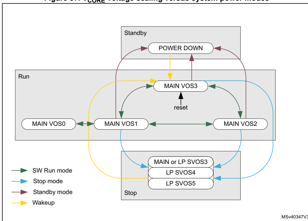
Figure 37. V CORE voltage scaling versus system power modes
