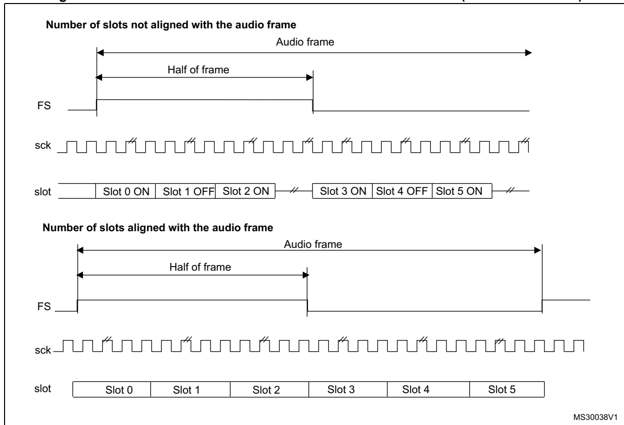
Figure 688. FS role is start of frame + channel side identification (FSDEF = TRIS = 1)
