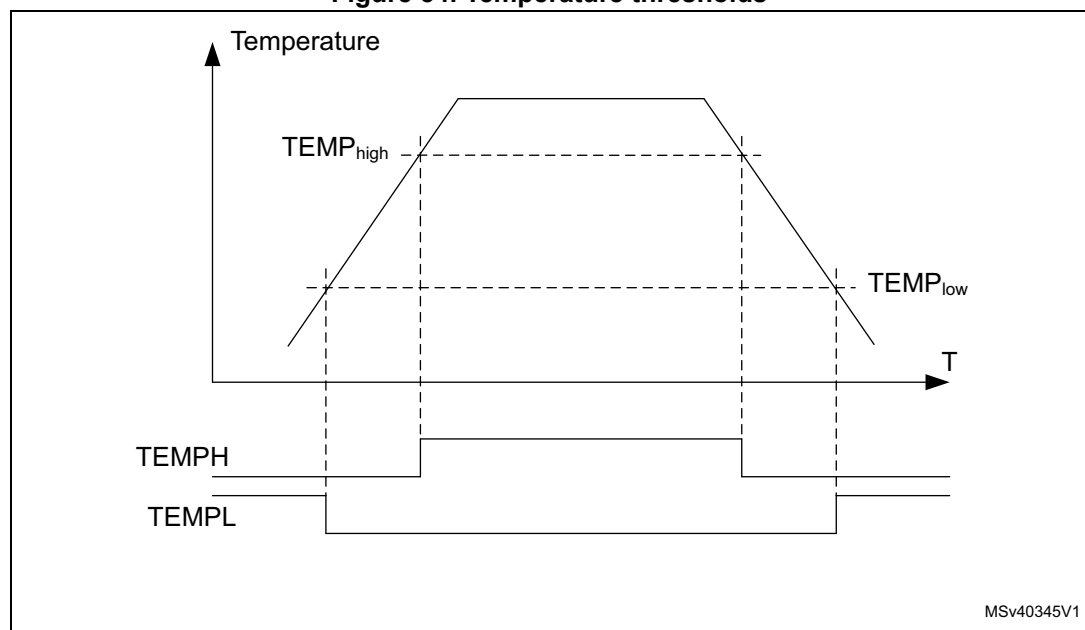
Figure 34. Temperature thresholds
