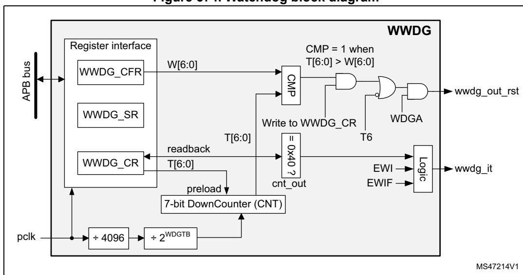
Figure 574. Watchdog block diagram
