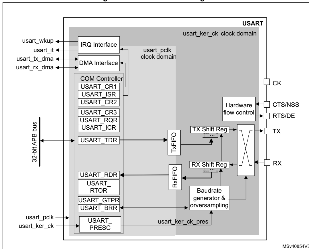
Figure 611. USART block diagram
