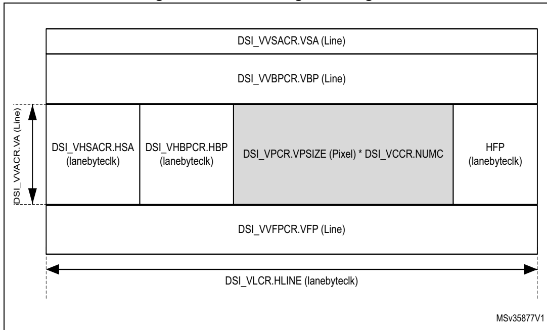
Figure 291. Frame configuration registers
