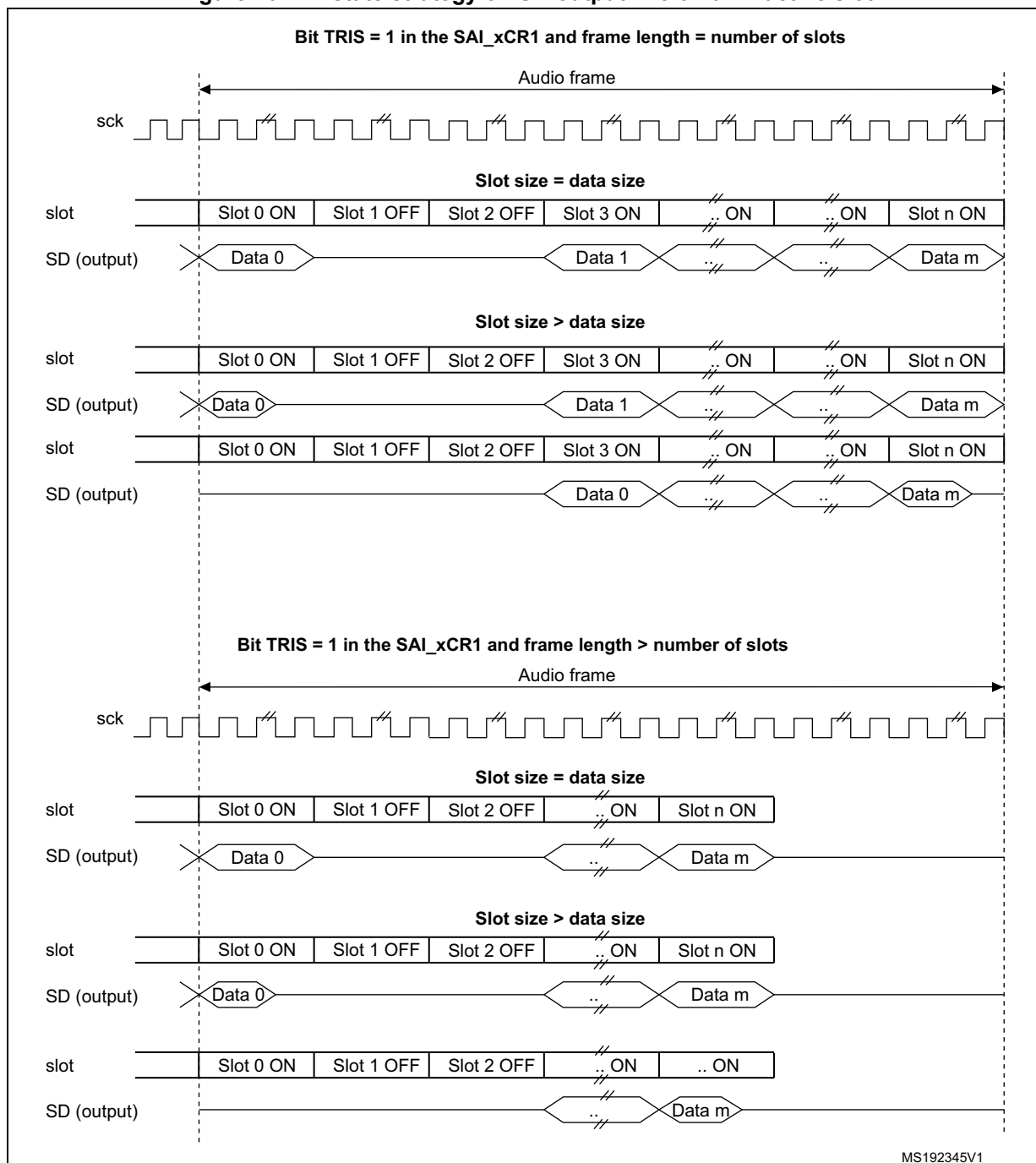
Figure 704. Tristate strategy on SD output line on an inactive slot
