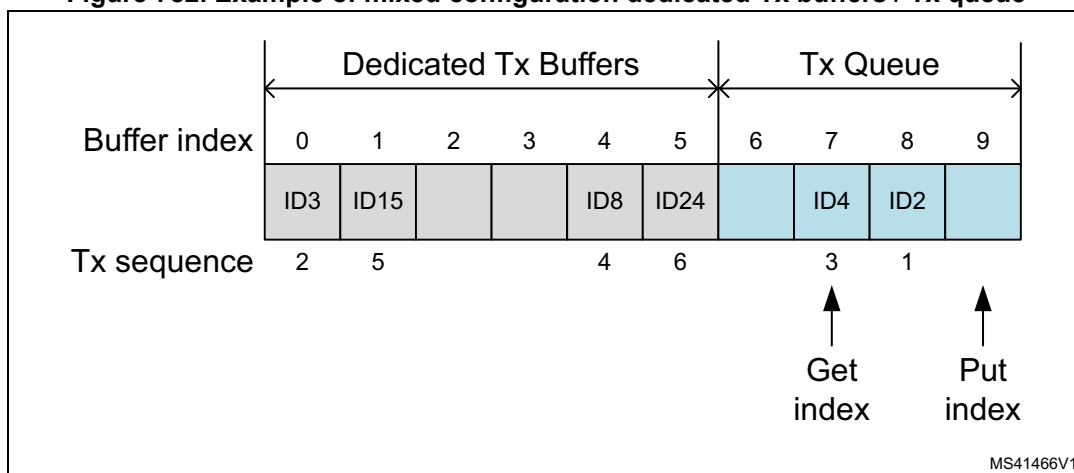
Figure 782. Example of mixed configuration dedicated Tx buffers / Tx queue
