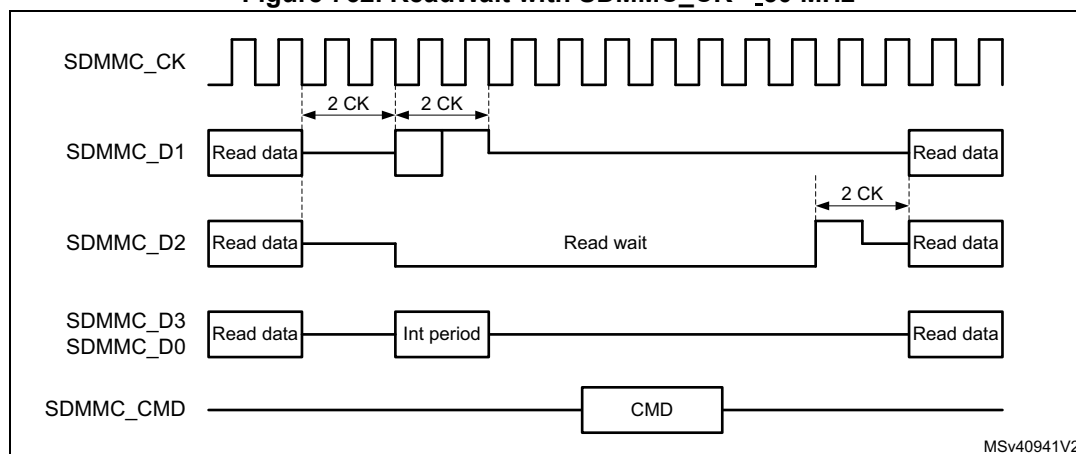
Figure 762. ReadWait with SDMMC_CK <_50 MHz
