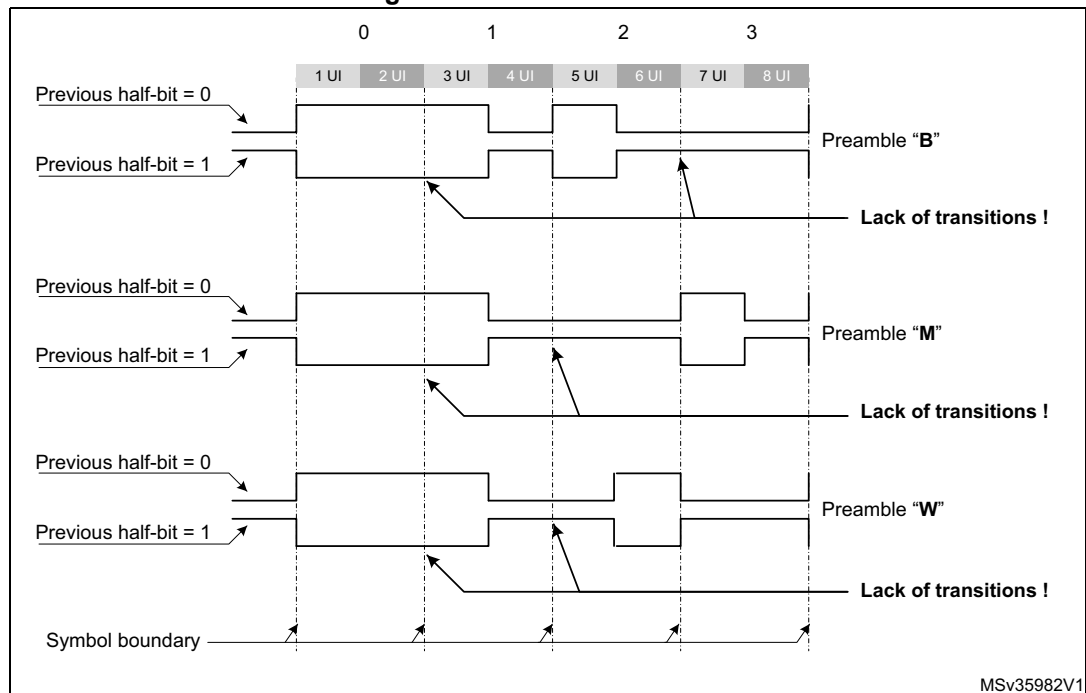
Figure 711. S/PDIF Preambles
