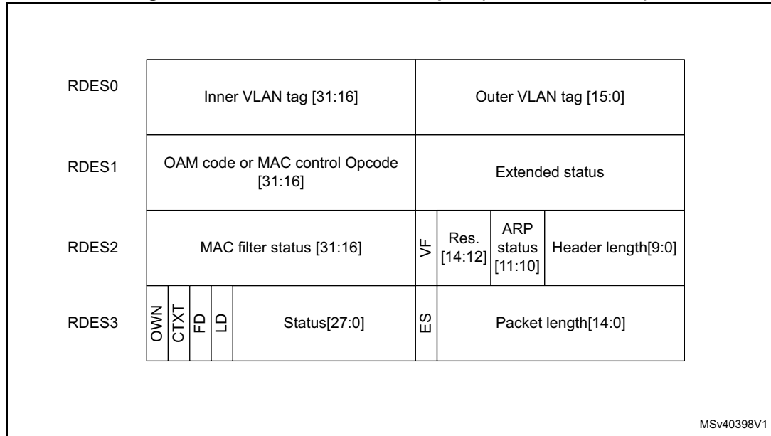
Figure 846. Receive normal descriptor (write-back format)
