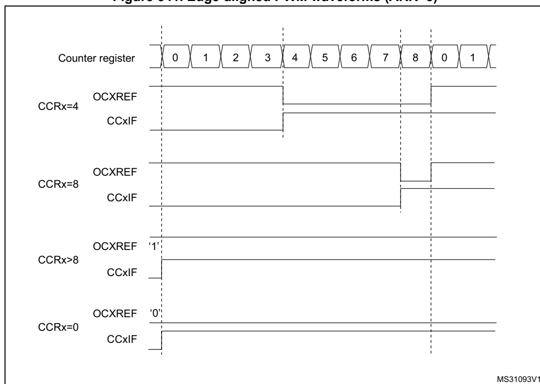
Figure 541. Edge-aligned PWM waveforms (ARR=8)
