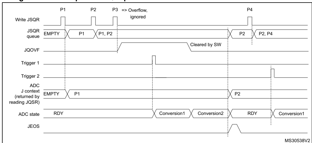
Figure 157. Example of JSQR queue of context with overflow before conversion
