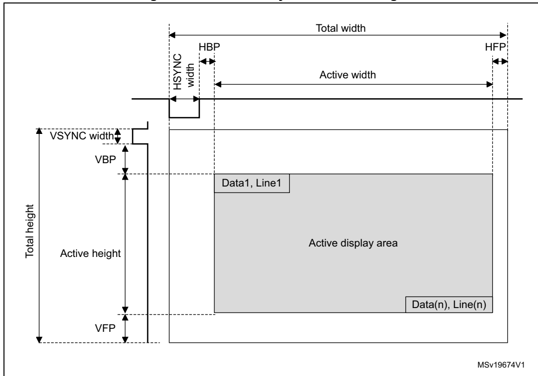
Figure 251. LCD-TFT synchronous timings
