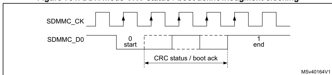
Figure 751. DDR mode CRC status / boot acknowledgment clocking
