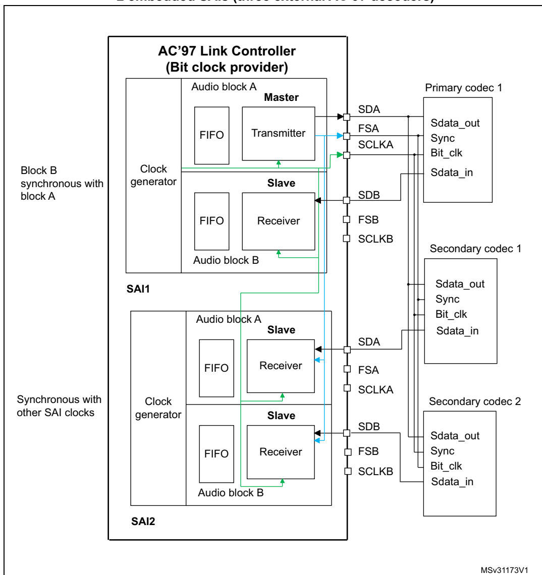
Figure 700. Example of typical AC'97 configuration on devices featuring at least 2 embedded SAIs (three external AC'97 decoders)
