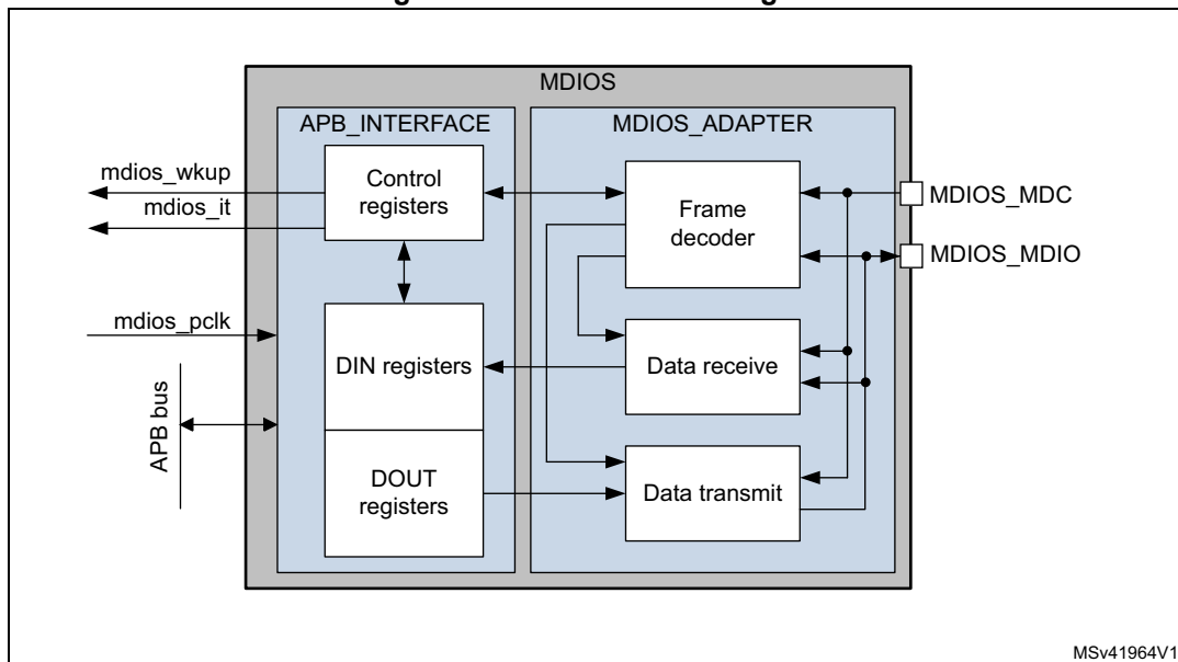
Figure 736. MDIOS block diagram
