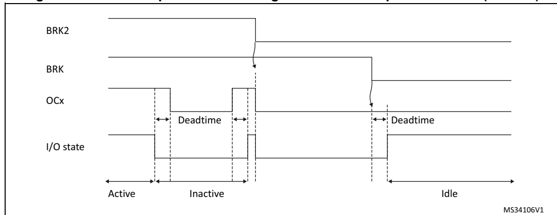
Figure 431. PWM output state following BRK and BRK2 pins assertion (OSSI=1)
