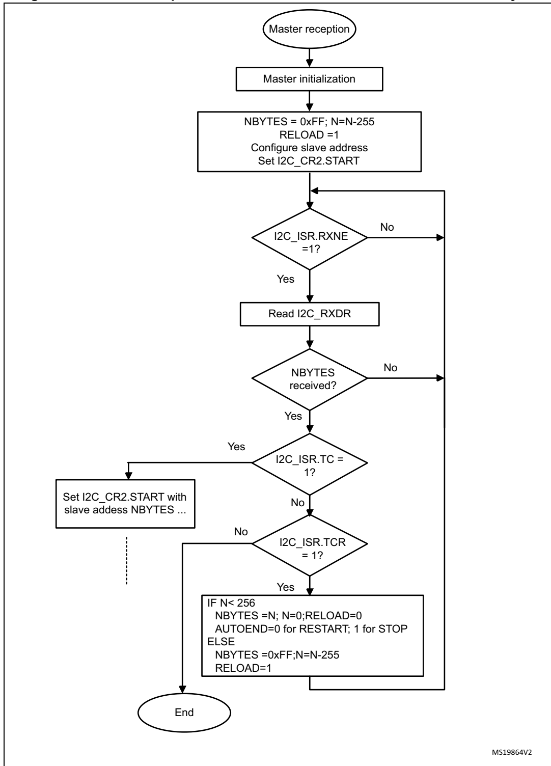
Figure 601. Transfer sequence flowchart for I2C master receiver for N >255 bytes
