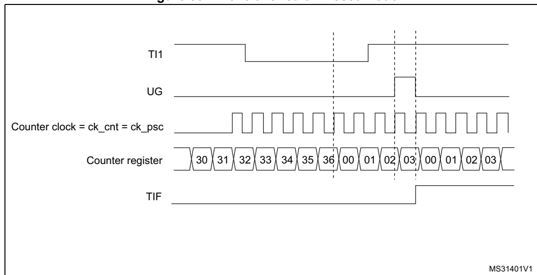
Figure 551. Control circuit in reset mode
