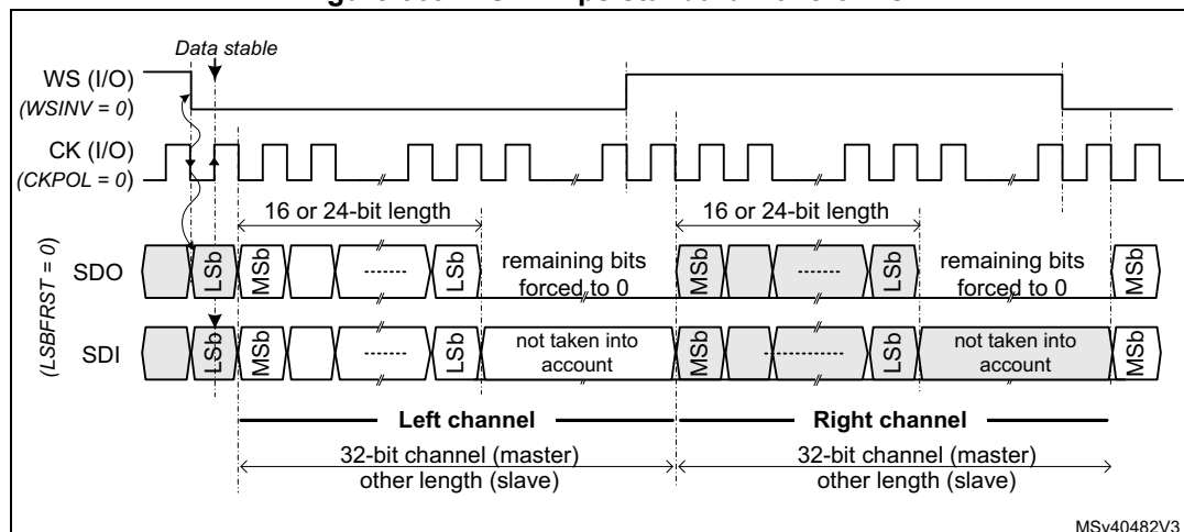
Figure 669. I2S Philips standard waveforms
