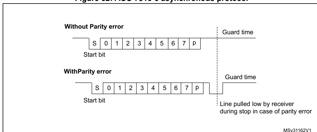
Figure 627. ISO 7816-3 asynchronous protocol
