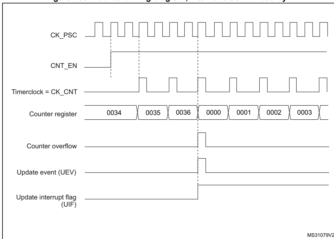
Figure 450. Counter timing diagram, internal clock divided by 2
