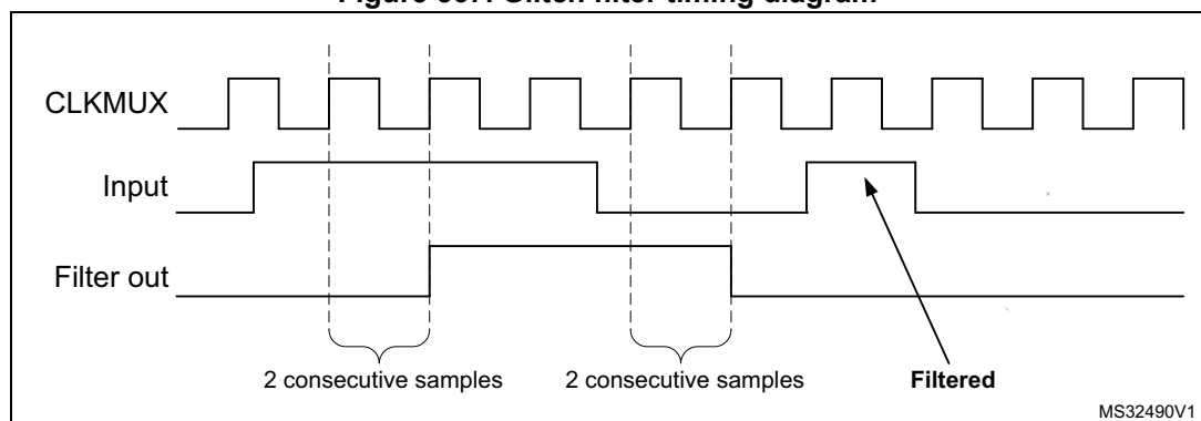
Figure 567. Glitch filter timing diagram
