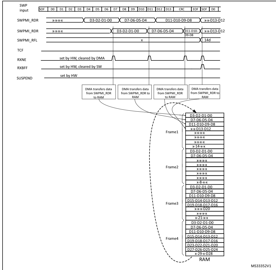
Figure 734. SWPMI Multi software buffer mode reception
