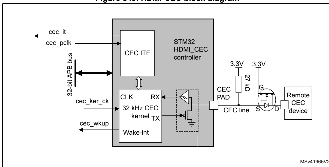
Figure 849. HDMI-CEC block diagram
