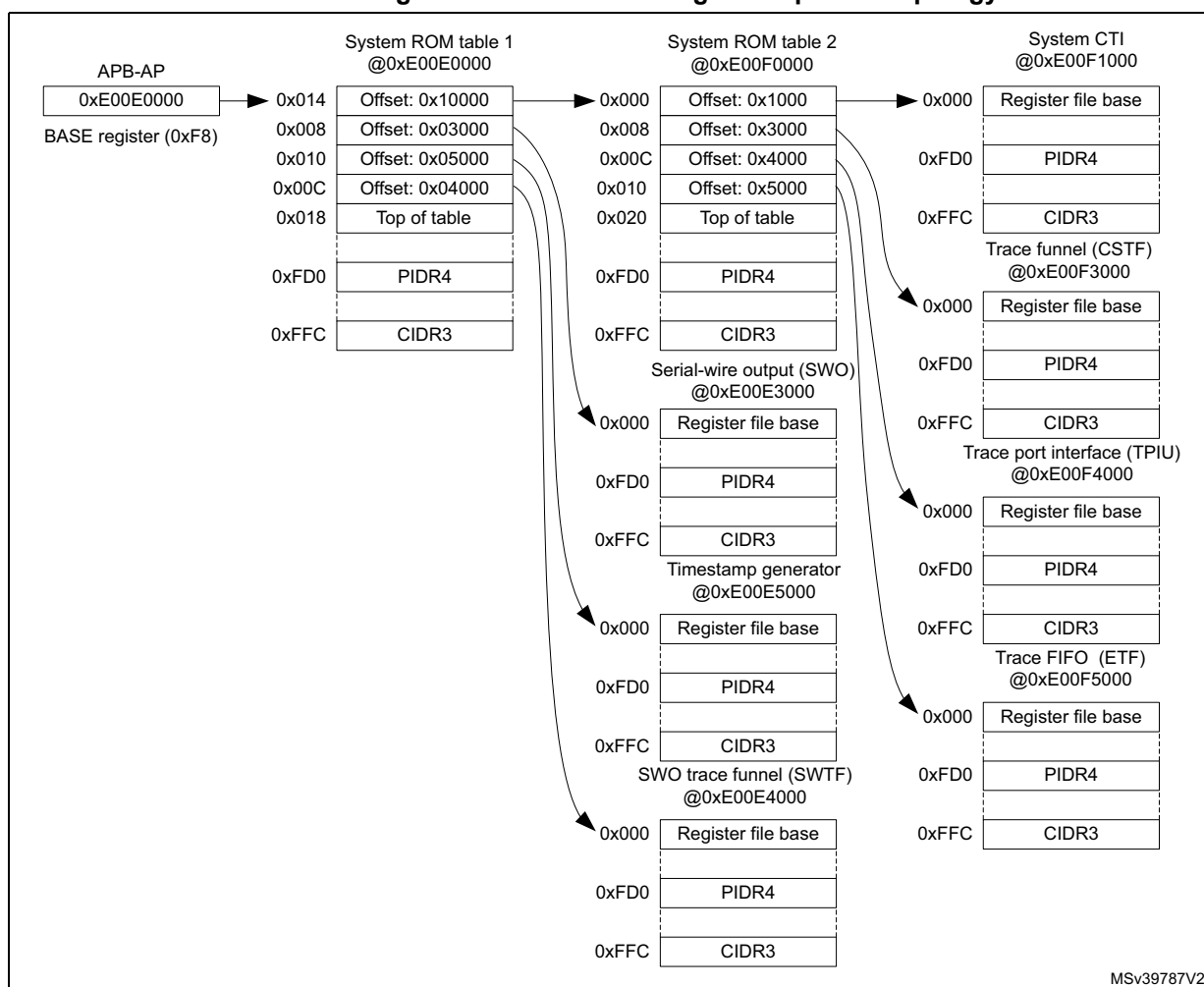
Figure 865. APB-D CoreSight component topology
