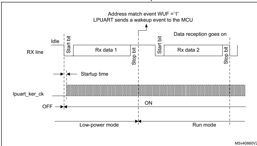
Figure 650. Wakeup event verified (wakeup event = address match, FIFO disabled)
