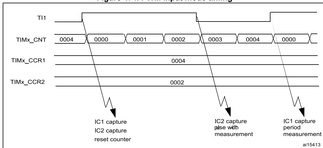
Figure 474. PWM input mode timing
