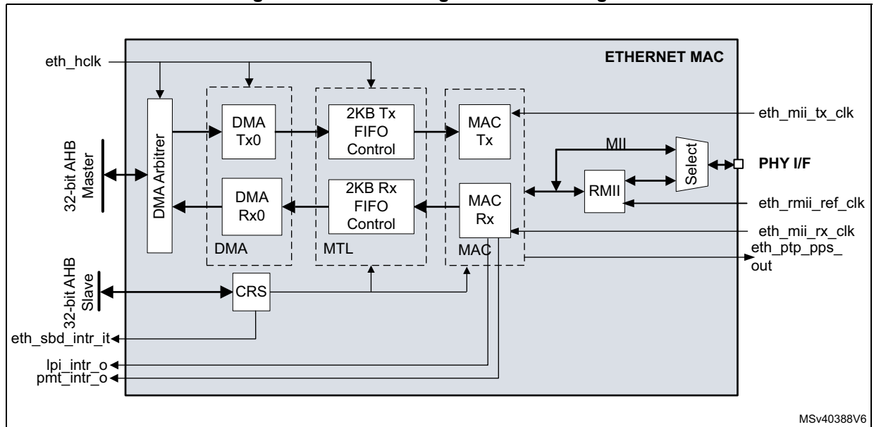
Figure 819. Ethernet high-level block diagram
