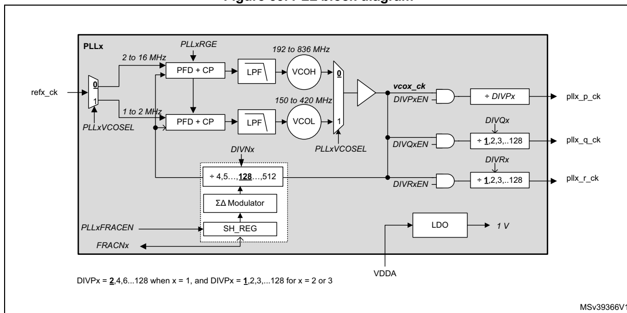
Figure 53. PLL block diagram
