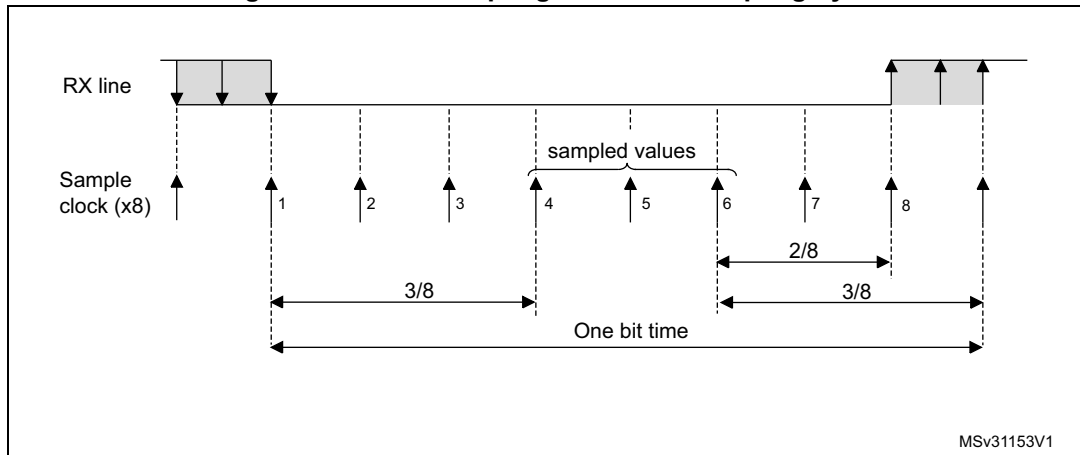
Figure 618. Data sampling when oversampling by 8
