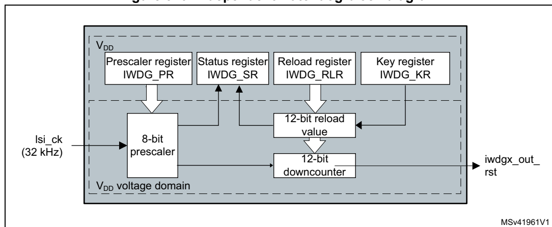
Figure 576. Independent watchdog block diagram
