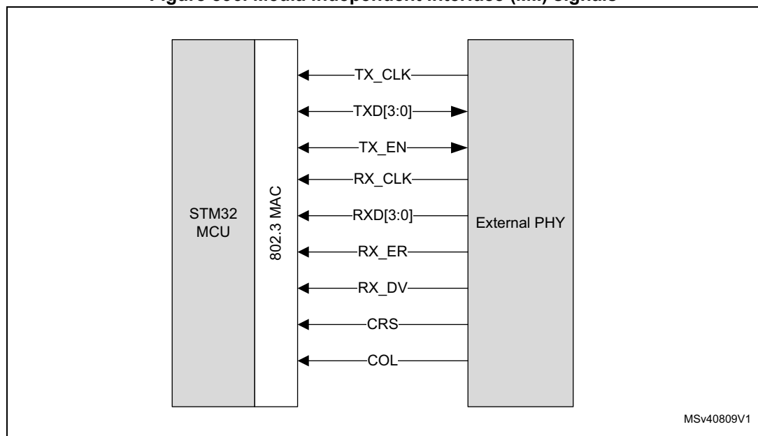
Figure 836. Media independent interface (MII) signals
