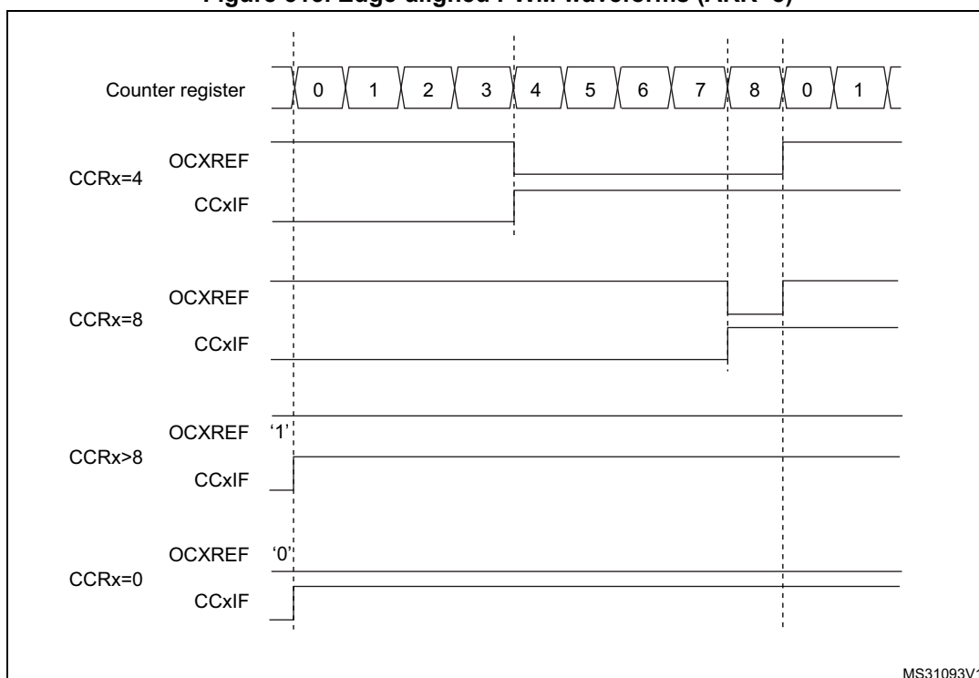
Figure 513. Edge-aligned PWM waveforms (ARR=8)
