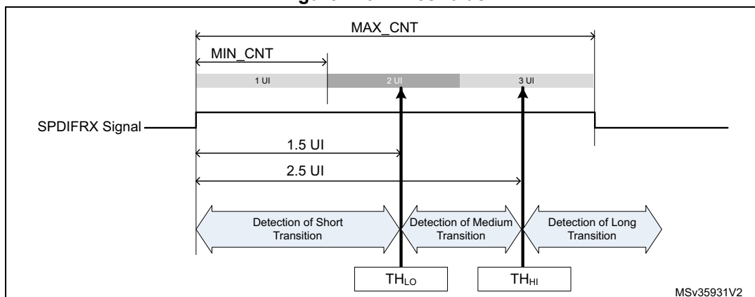
Figure 715. Thresholds
