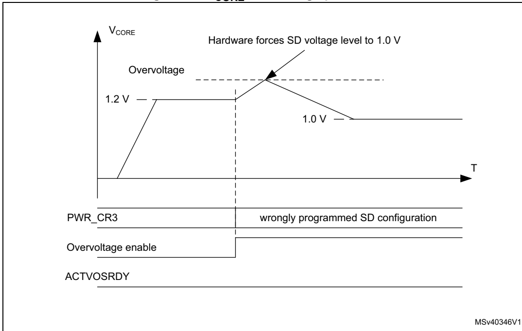
Figure 35. V CORE overvoltage protection
