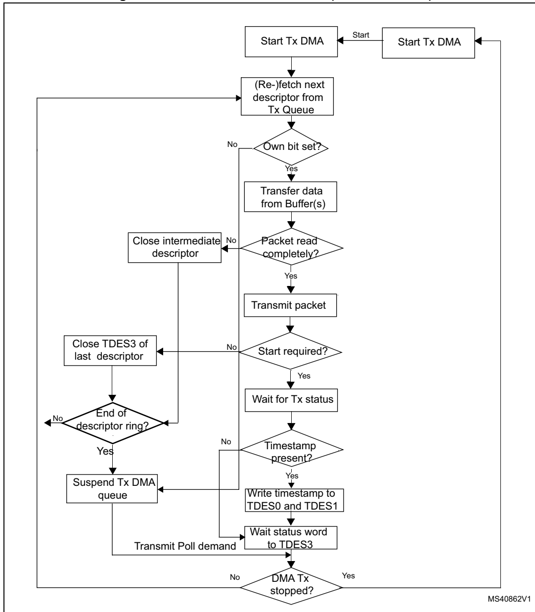
Figure 820. DMA transmission flow (standard mode)
