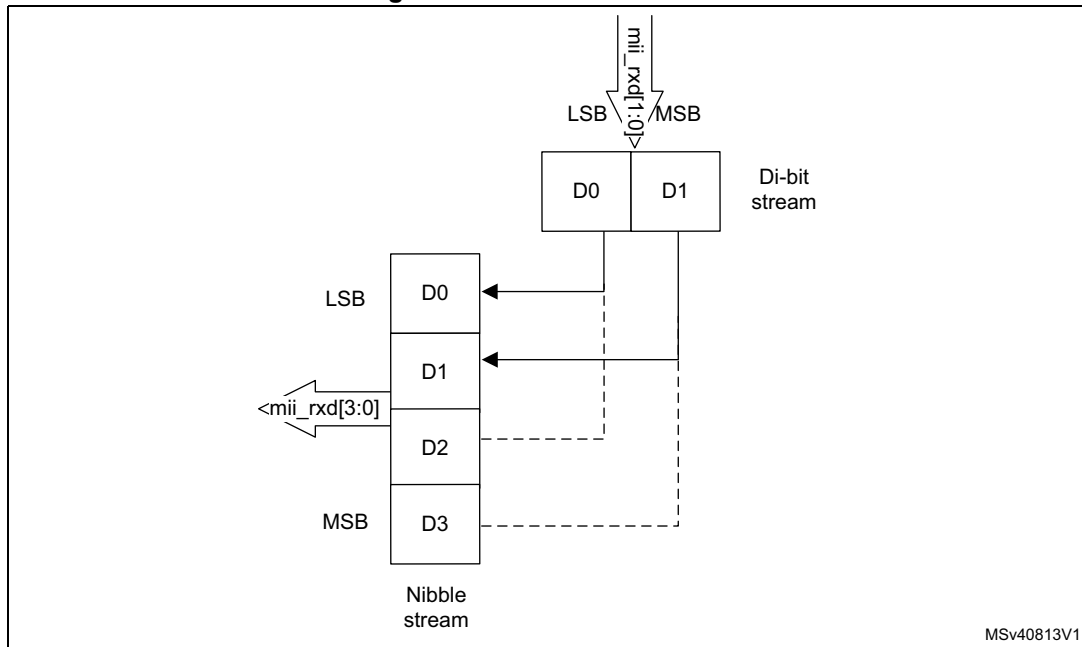
Figure 839. Receive bit order
