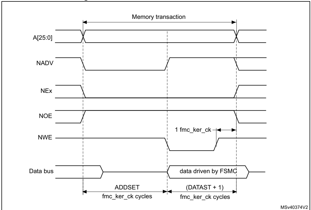
Figure 110. Mode 2 write access waveforms
