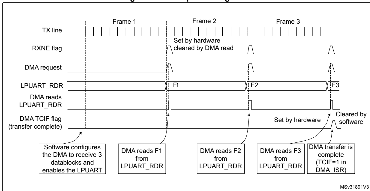
Figure 646. Reception using DMA
