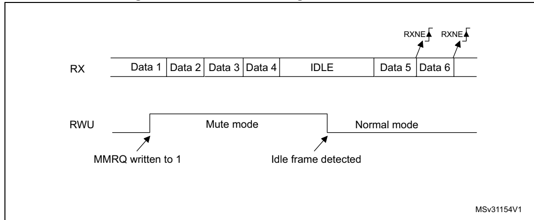
Figure 643. Mute mode using Idle line detection
