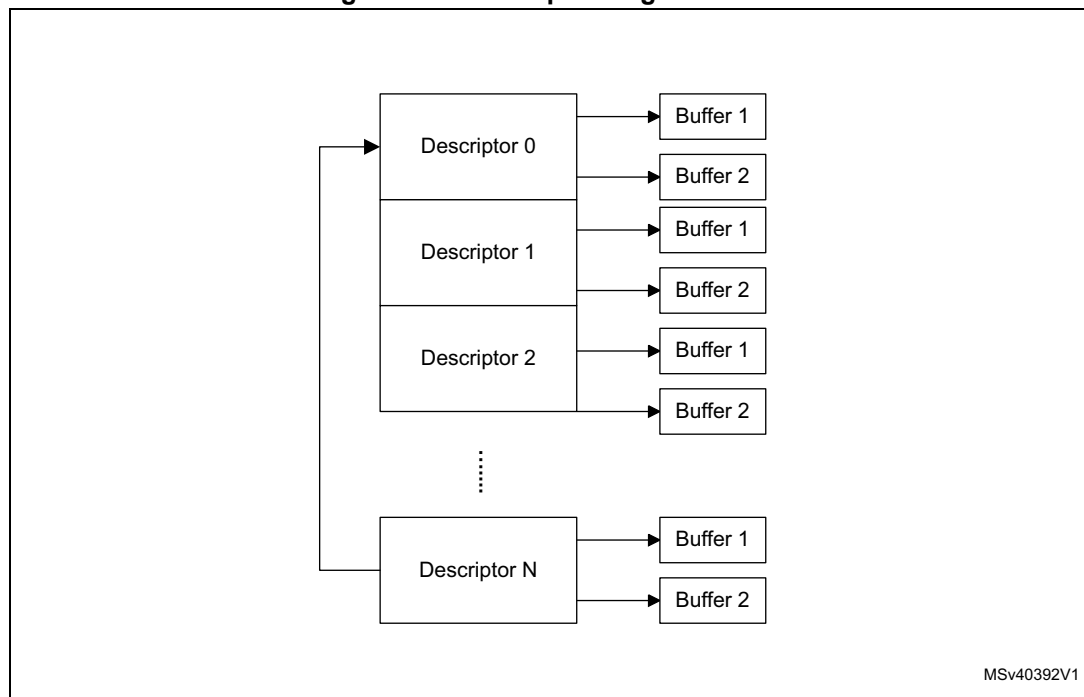
Figure 840. Descriptor ring structure
