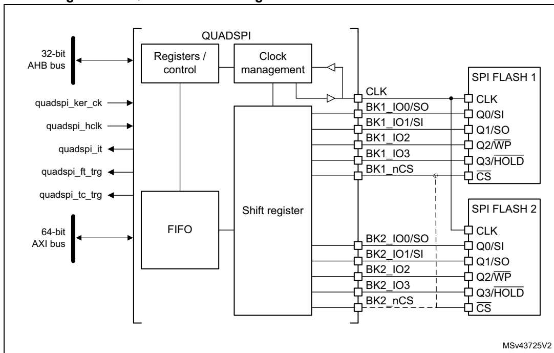
Figure 133. QUADSPI block diagram when dual-flash mode is enabled
