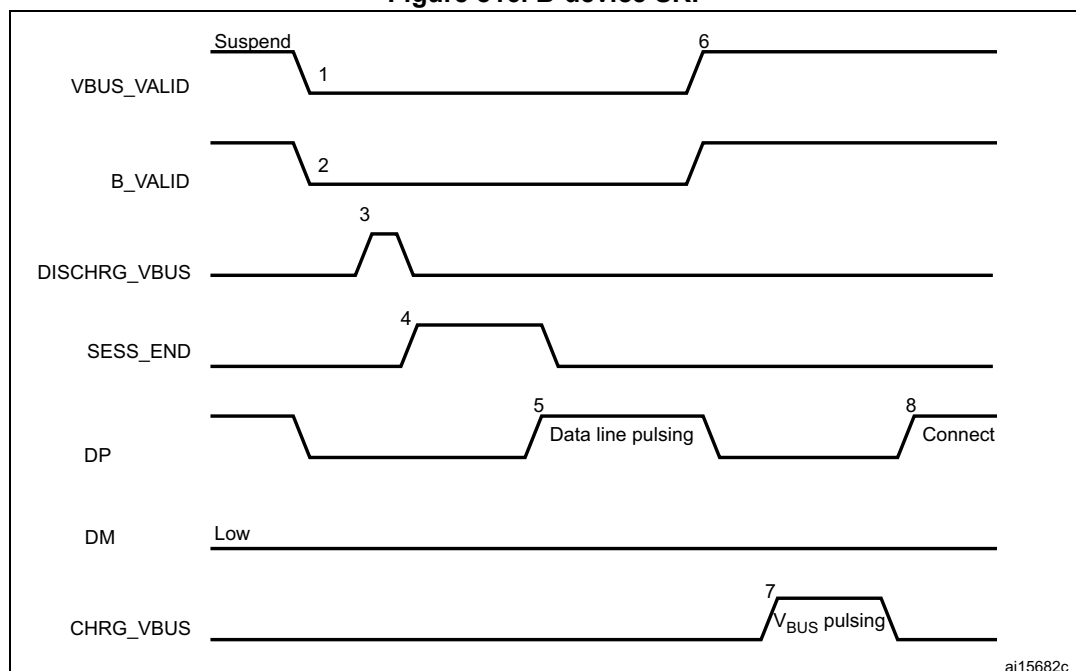
Figure 816. B-device SRP
