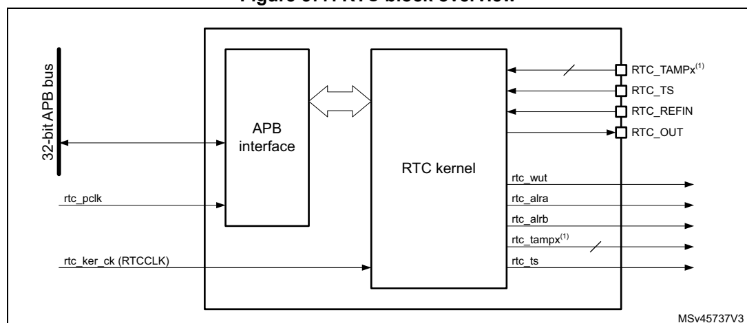
Figure 577. RTC block overview
