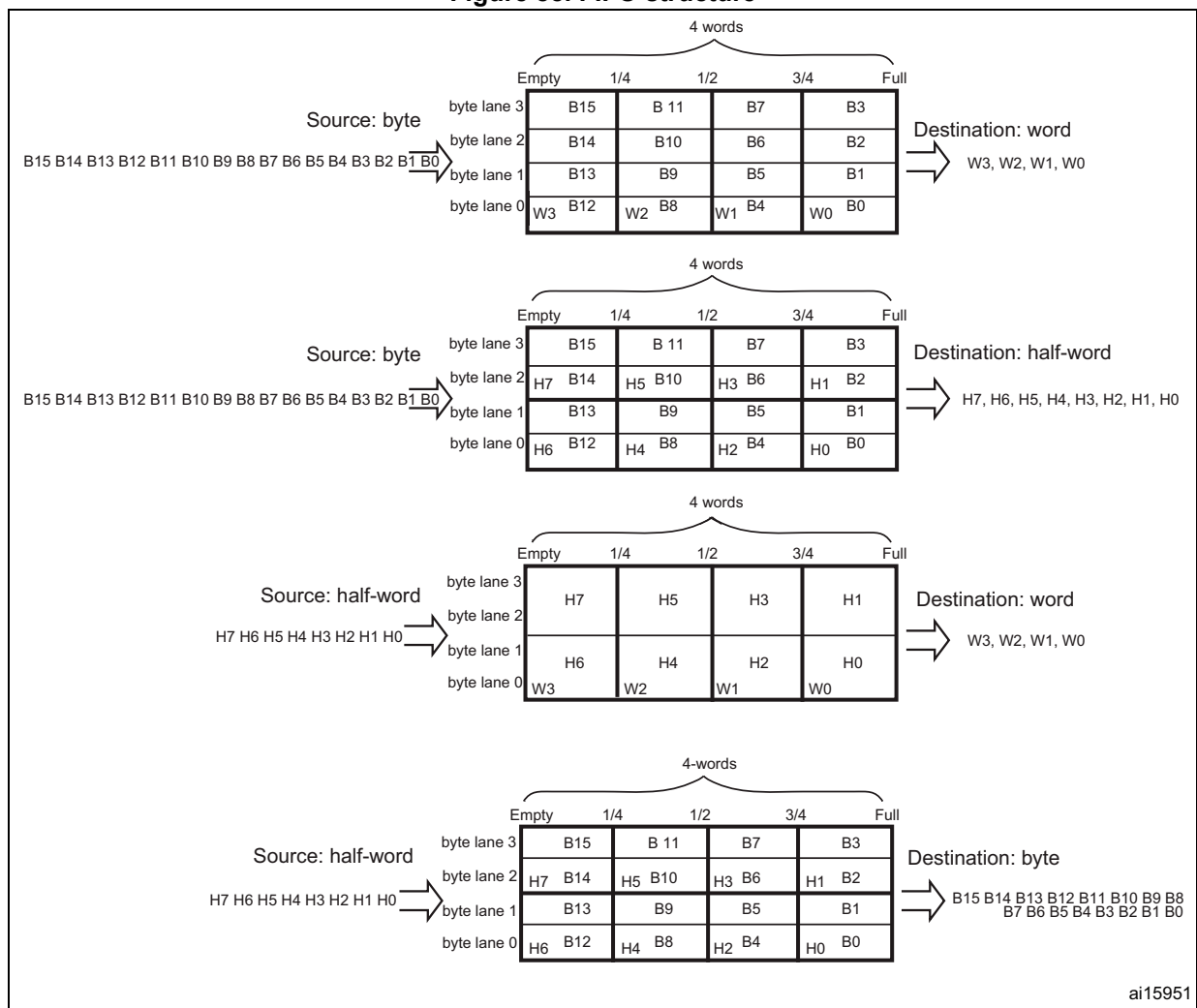
Figure 88. FIFO structure
