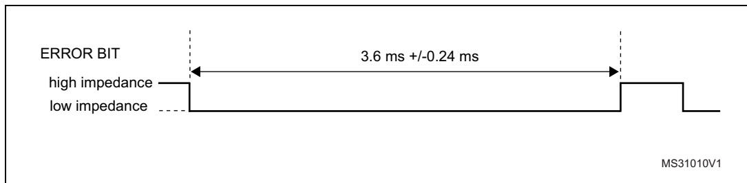
Figure 856. Error bit timing
