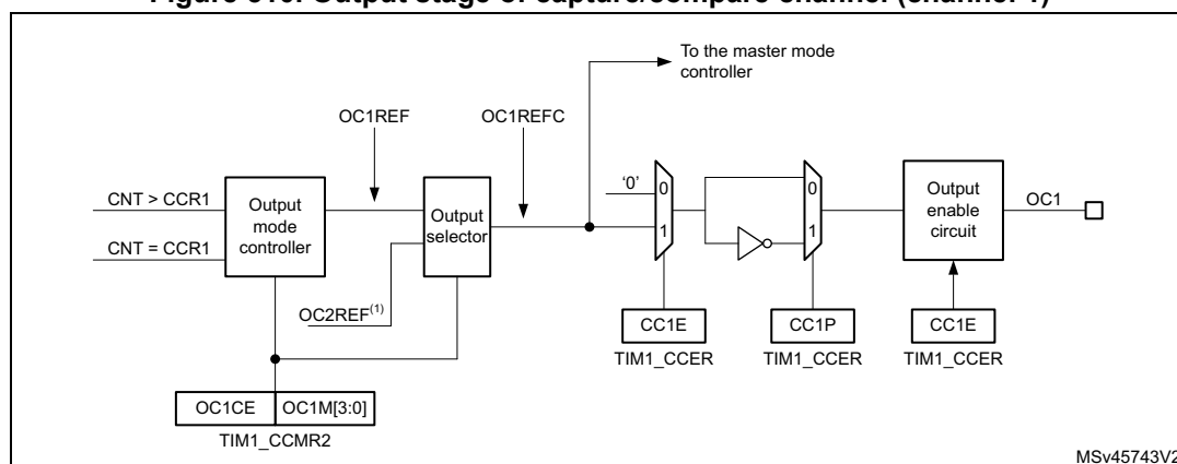
Figure 510. Output stage of capture/compare channel (channel 1)
