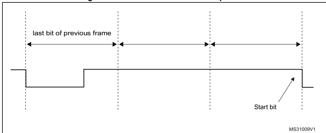
Figure 855. SFT of three nominal bit periods
