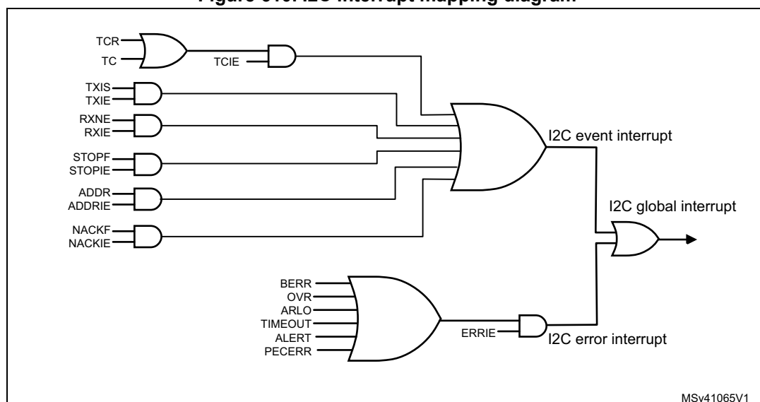
Figure 610. I2C interrupt mapping diagram
