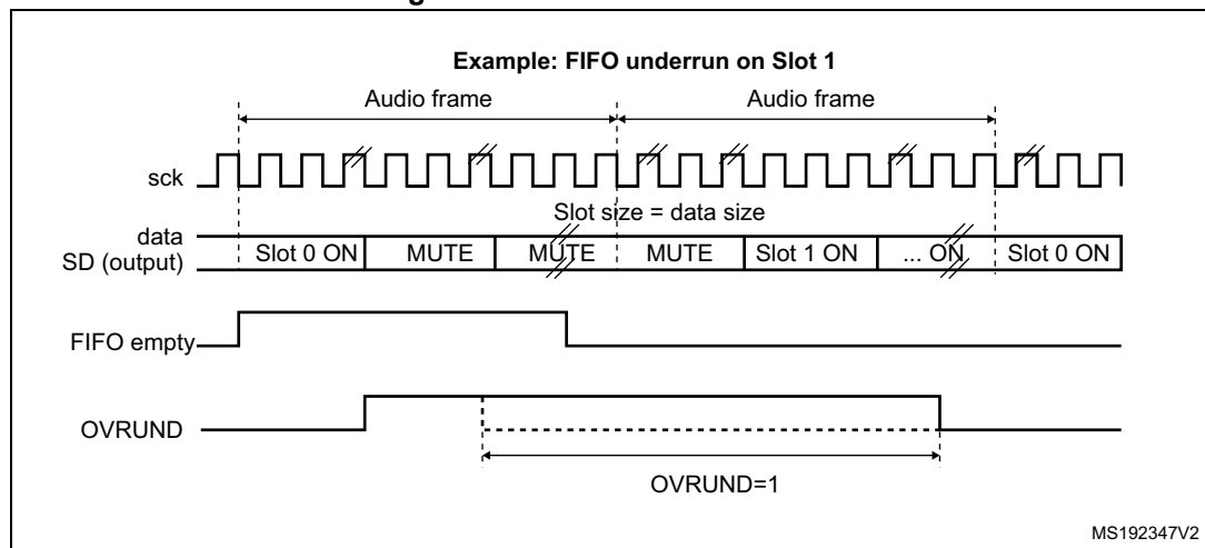
Figure 707. FIFO underrun event
