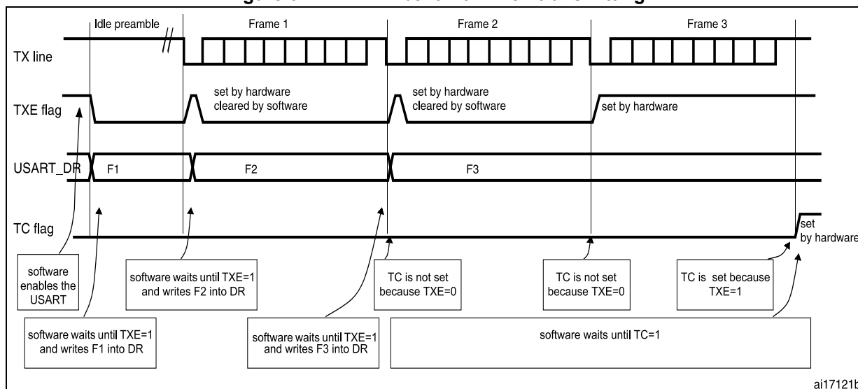
Figure 614. TC/TXE behavior when transmitting
