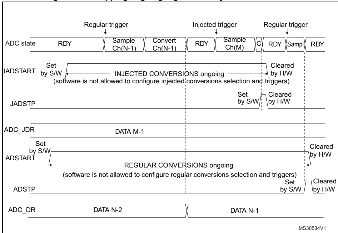
Figure 152. Stopping ongoing regular and injected conversions
