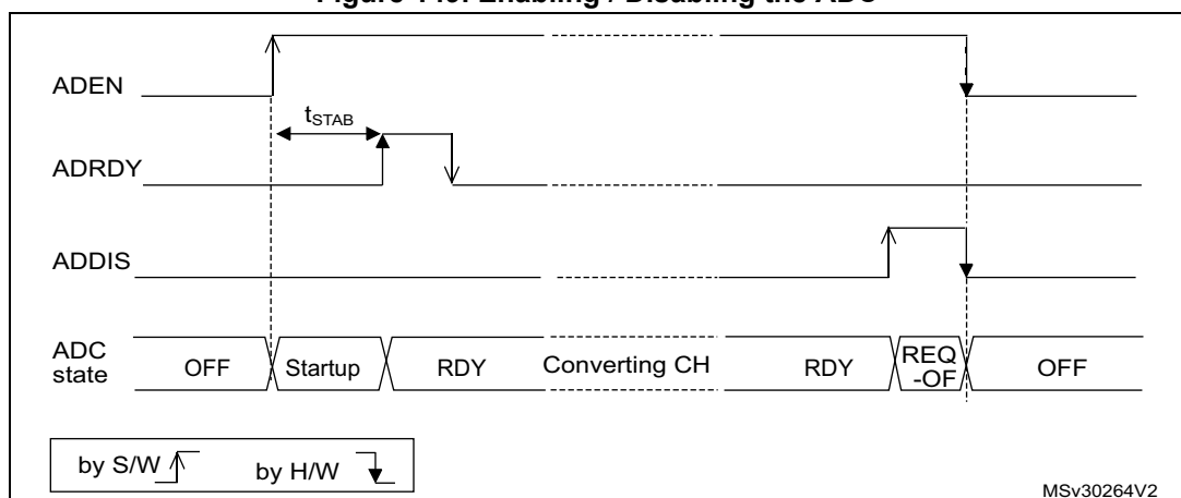
Figure 149. Enabling / Disabling the ADC
