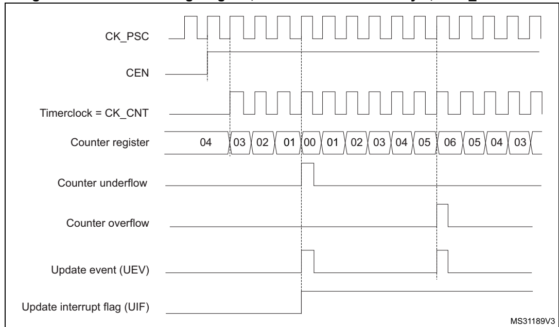
Figure 400. Counter timing diagram, internal clock divided by 1, TIMx_ARR = 0x6
