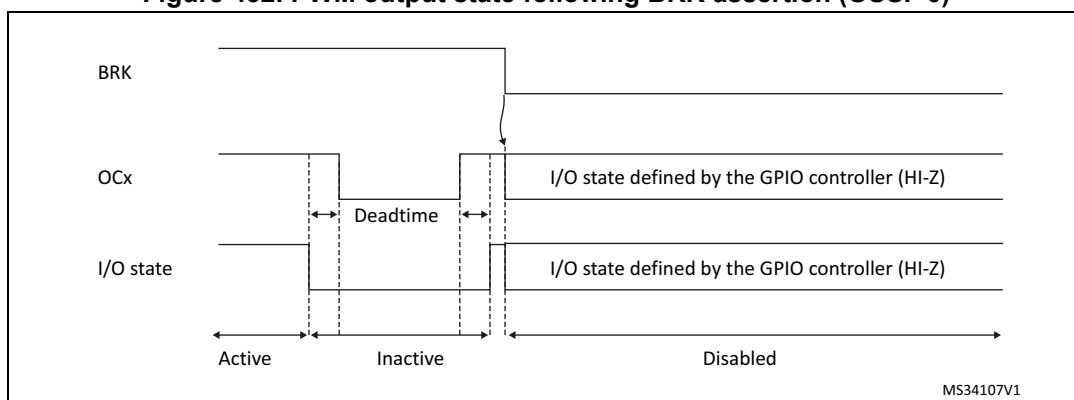
Figure 432. PWM output state following BRK assertion (OSSI=0)
