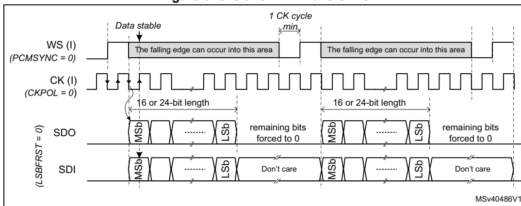
Figure 676. Slave PCM waveforms
