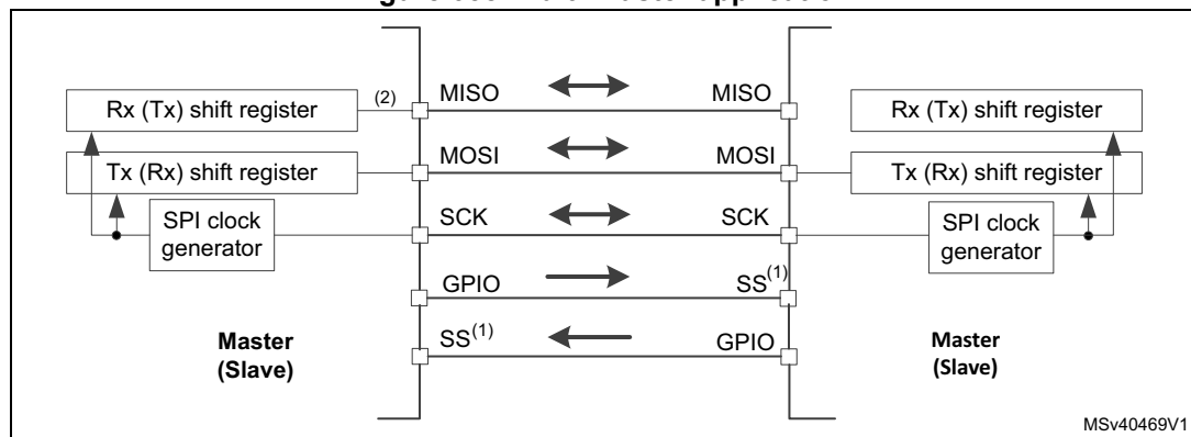
Figure 658. Multi-master application
