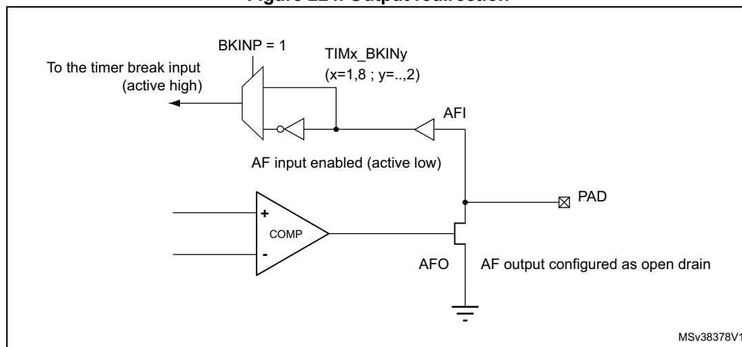
Figure 224. Output redirection
