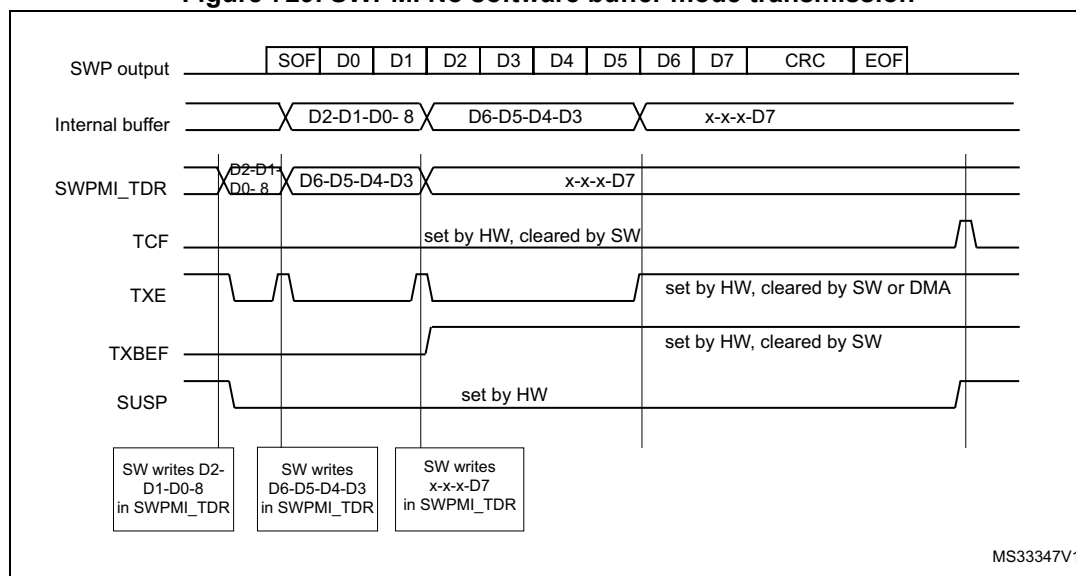
Figure 729. SWPMI No software buffer mode transmission
