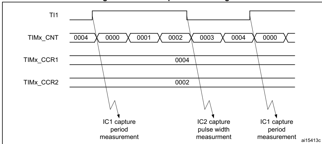
Figure 511. PWM input mode timing
