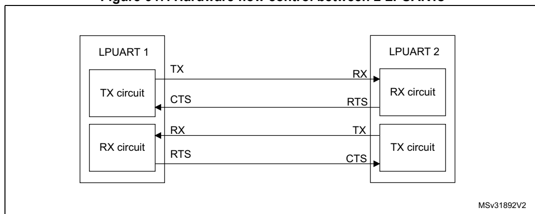
Figure 647. Hardware flow control between 2 LPUARTs
