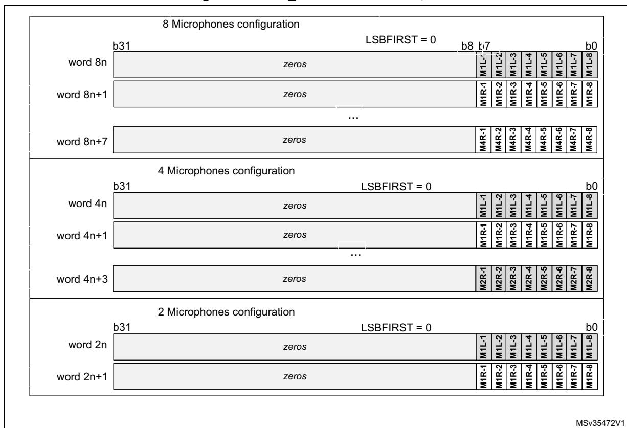
Figure 698. SAI_ADR format in TDM, 8-bit slot width
