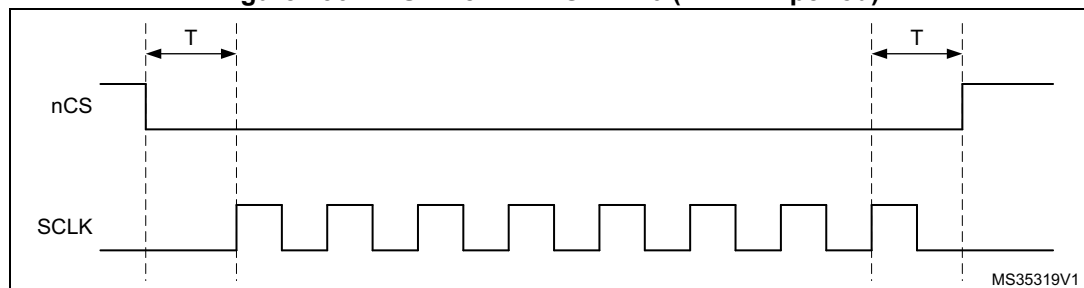
Figure 136. nCS when CKMODE = 0 (T = CLK period)
