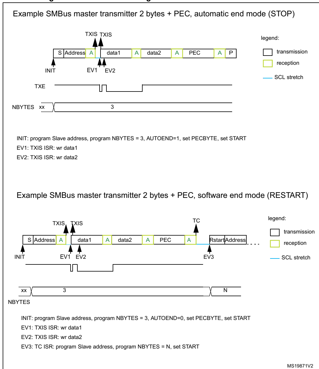
Figure 608. Bus transfer diagrams for SMBus master transmitter
