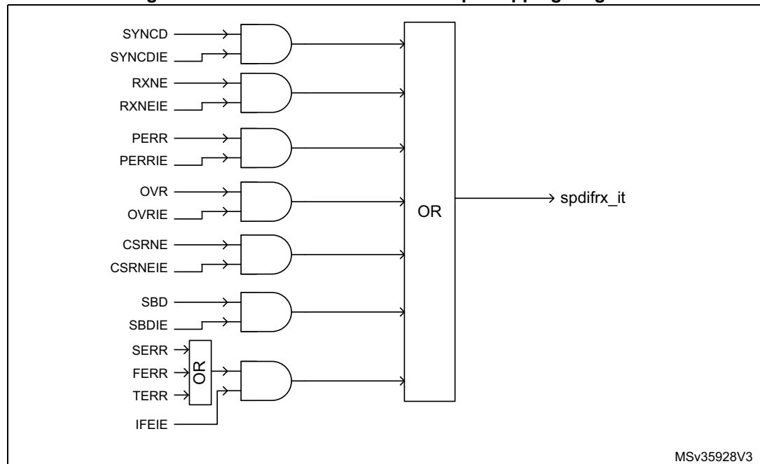
Figure 723. SPDIFRX interface interrupt mapping diagram
