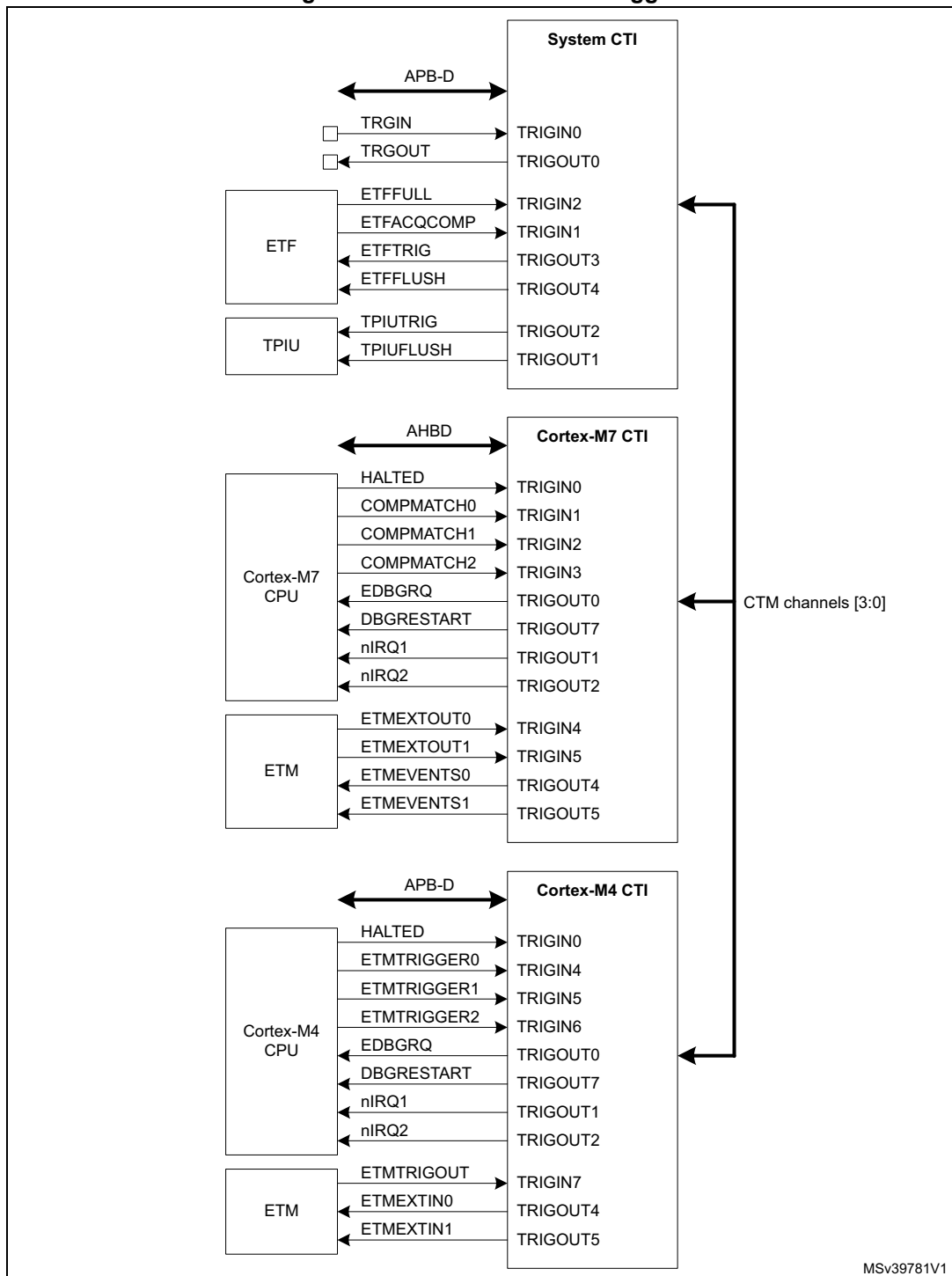
Figure 867. Embedded cross trigger
