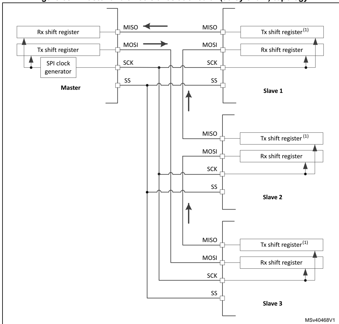
Figure 657. Master and three slaves at circular (daisy chain) topology
