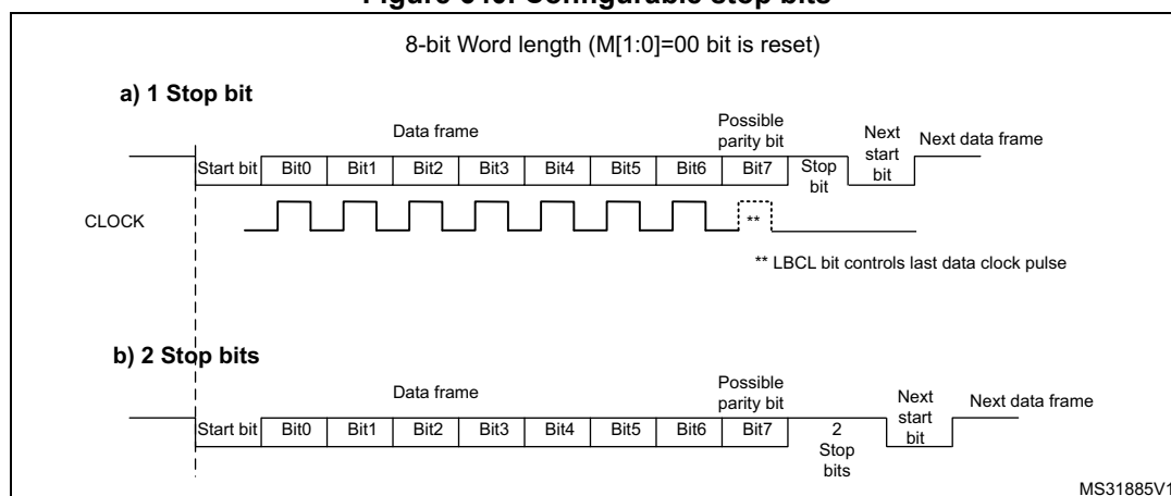
Figure 640. Configurable stop bits
