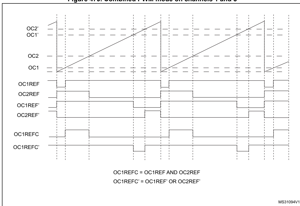
Figure 479. Combined PWM mode on channels 1 and 3
