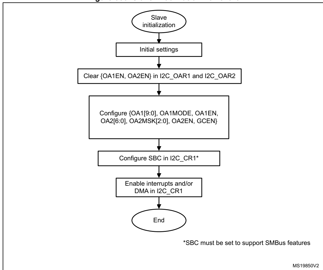
Figure 586. Slave initialization flowchart
