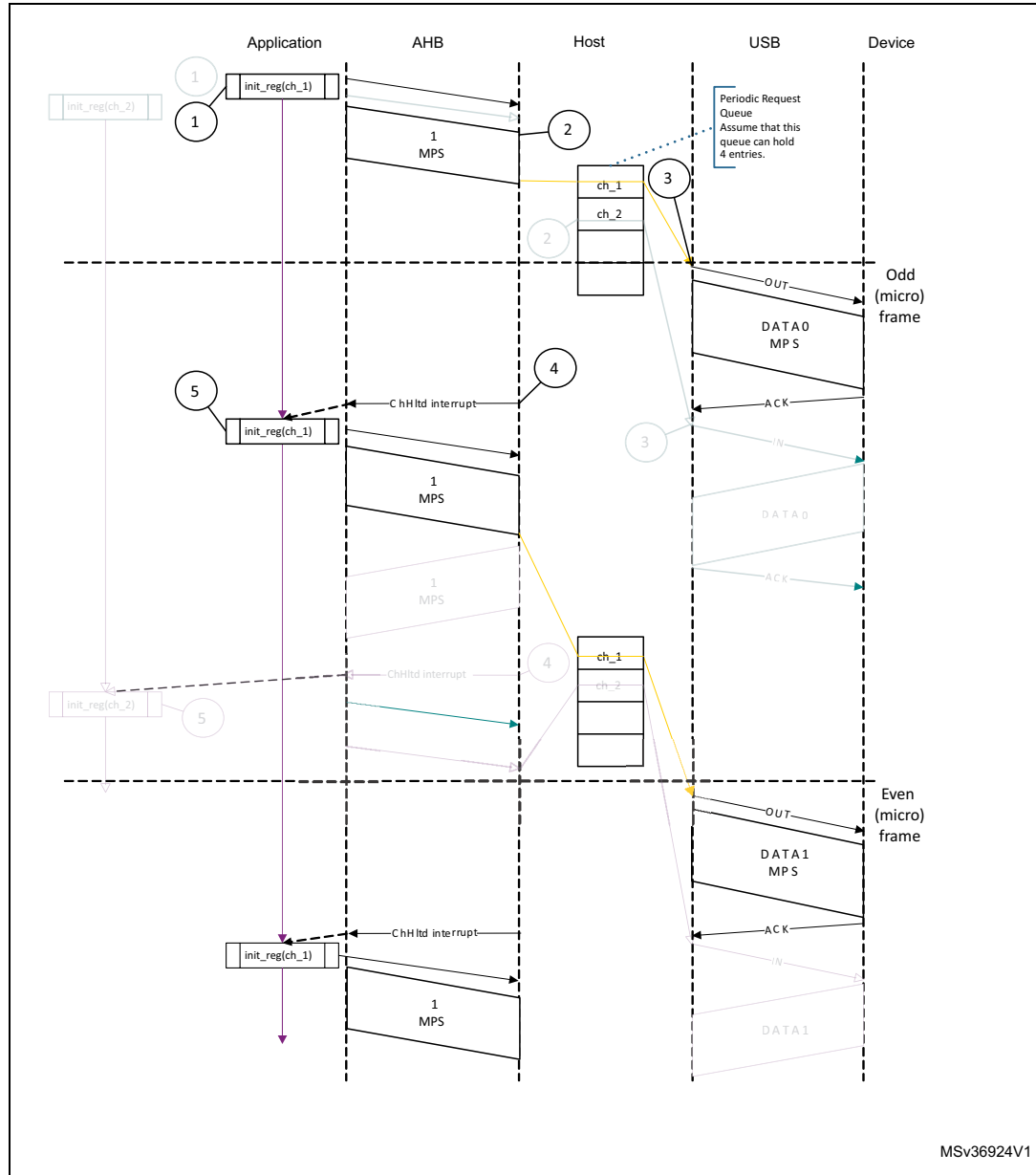
Figure 807. Normal interrupt OUT transactions - DMA mode
