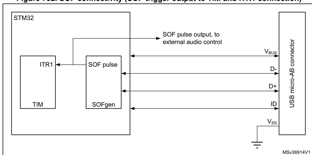
Figure 792. SOF connectivity (SOF trigger output to TIM and ITR1 connection)
