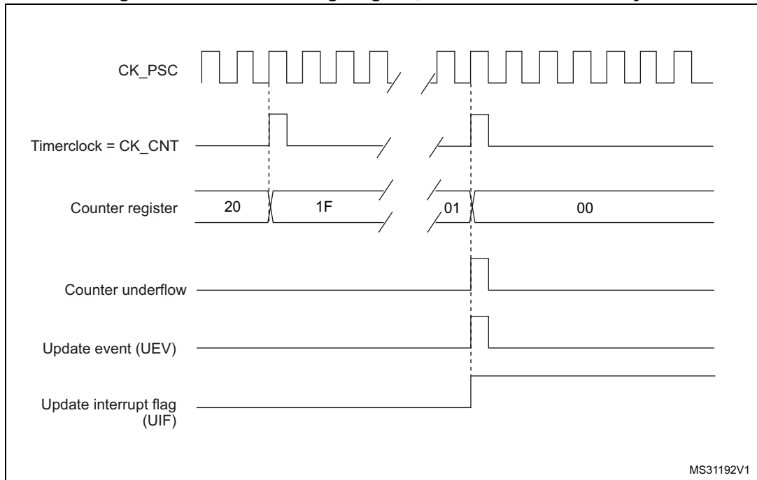
Figure 404. Counter timing diagram, update event with ARPE=1 (counter underflow)
