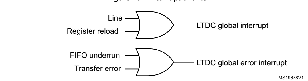
Figure 254. Interrupt events
