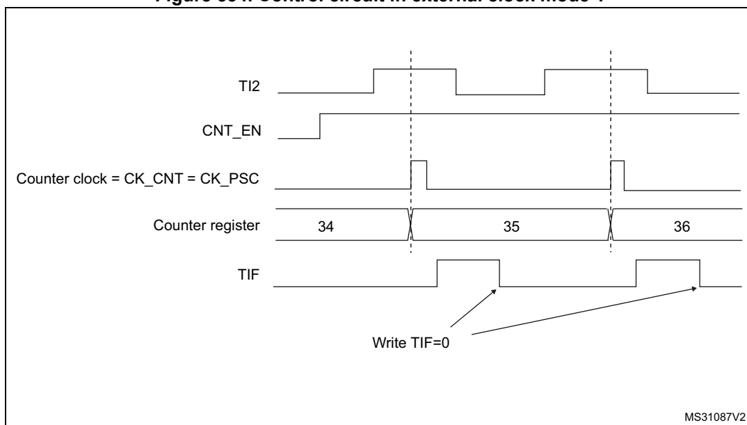
Figure 534. Control circuit in external clock mode 1
