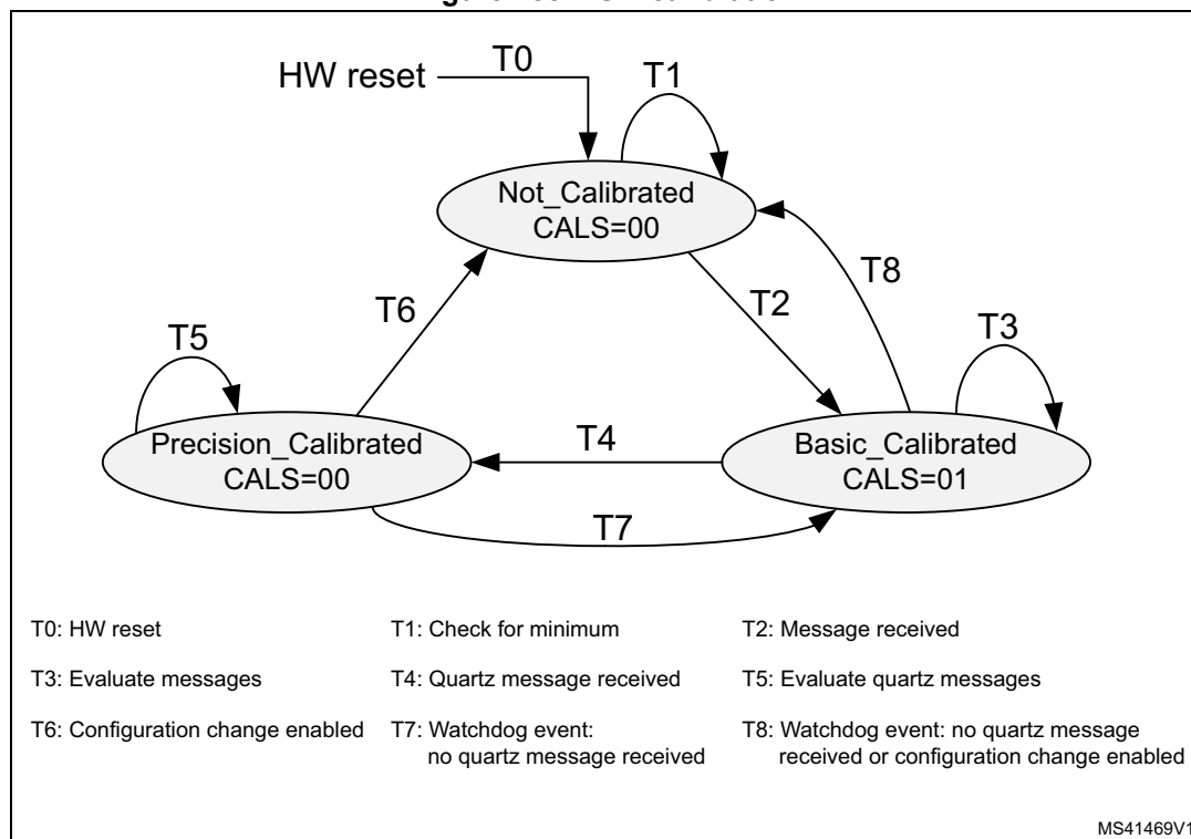
Figure 785. FSM calibration
