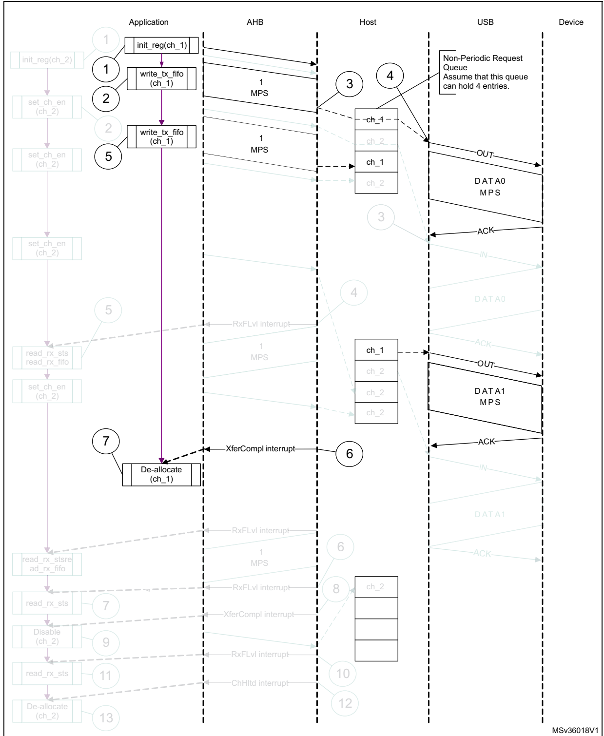
Figure 799. Normal bulk/control OUT/SETUP
