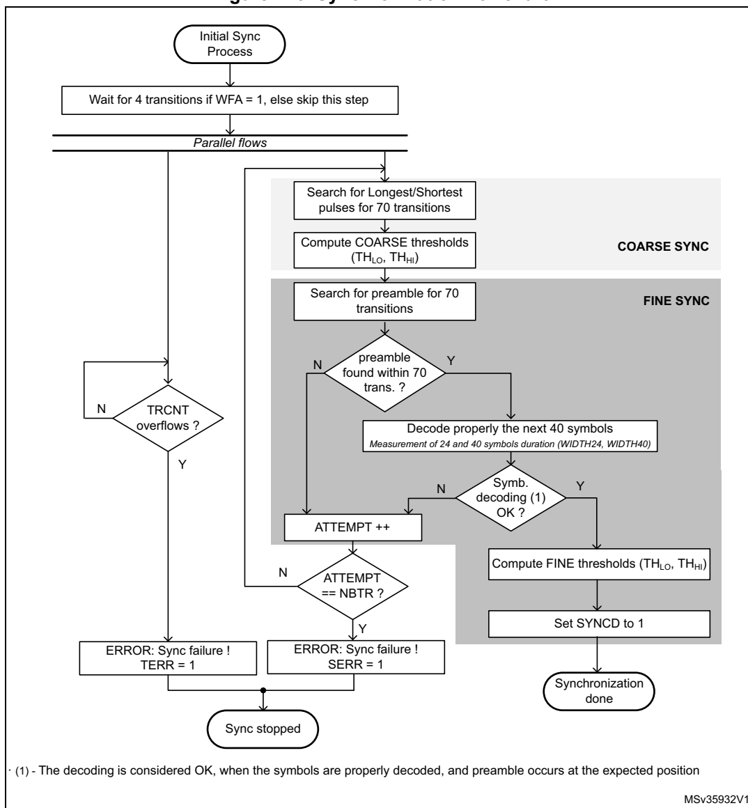
Figure 716. Synchronization flowchart
