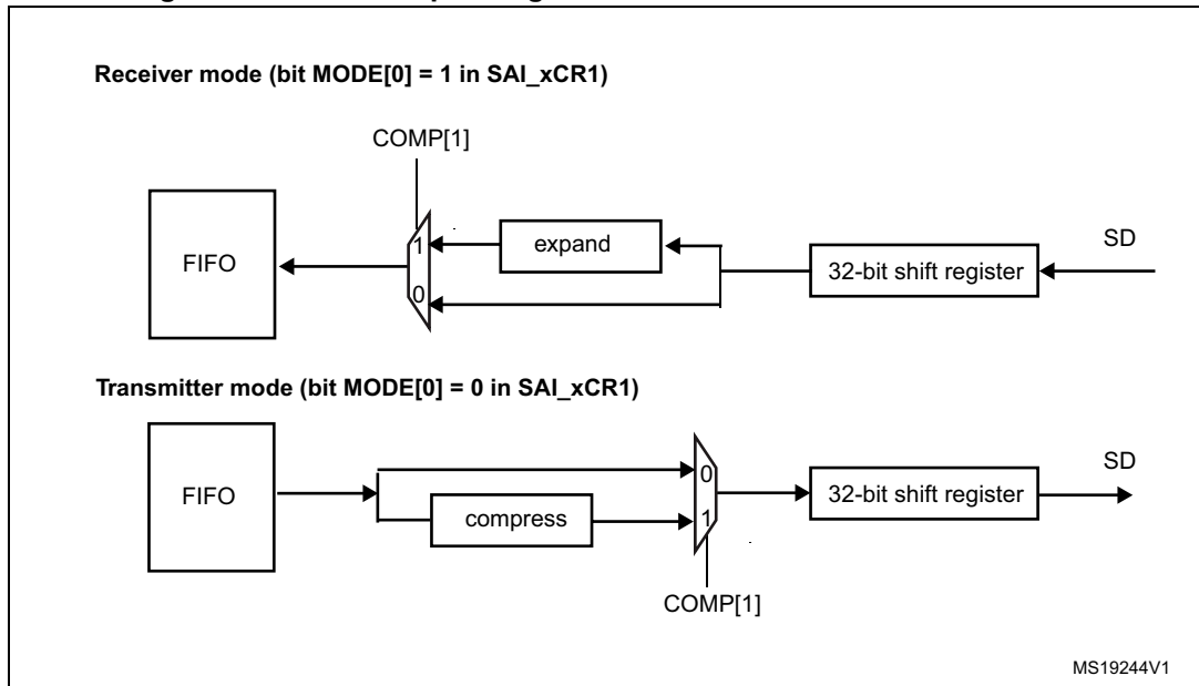
Figure 703. Data companding hardware in an audio block in the SAI
