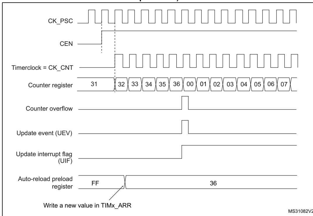
Figure 529. Counter timing diagram, update event when ARPE=0 (TIMx_ARR not preloaded)
