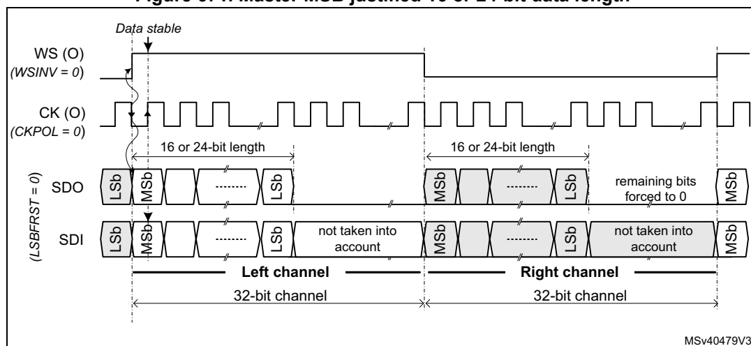
Figure 671. Master MSB justified 16 or 24-bit data length
