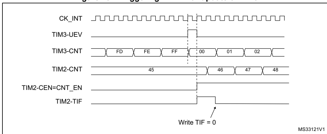
Figure 492. Triggering TIM2 with update of TIM3
