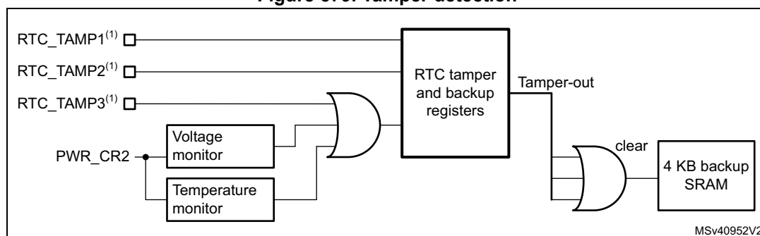
Figure 579. Tamper detection
