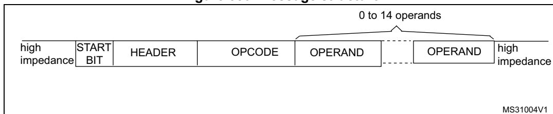
Figure 850. Message structure
