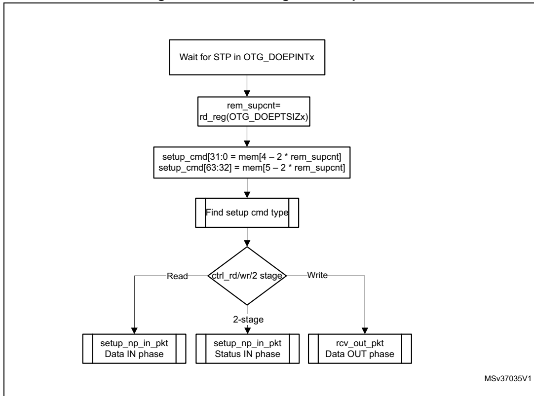
Figure 812. Processing a SETUP packet
