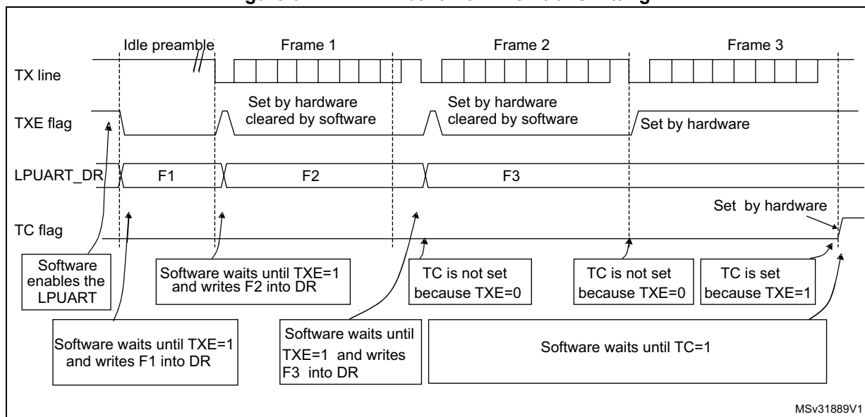
Figure 641. TC/TXE behavior when transmitting
