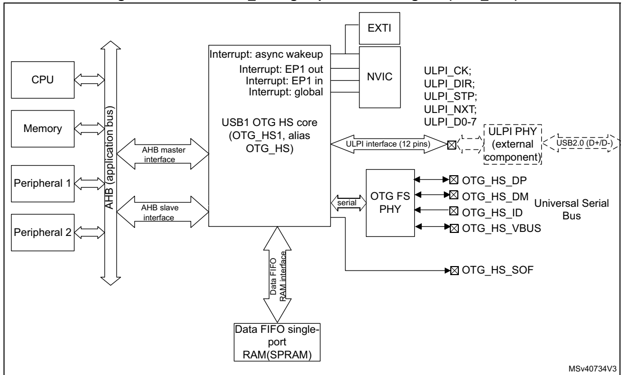
Figure 790. USB1 OTG_HS high-speed block diagram (OTG_HS1)
