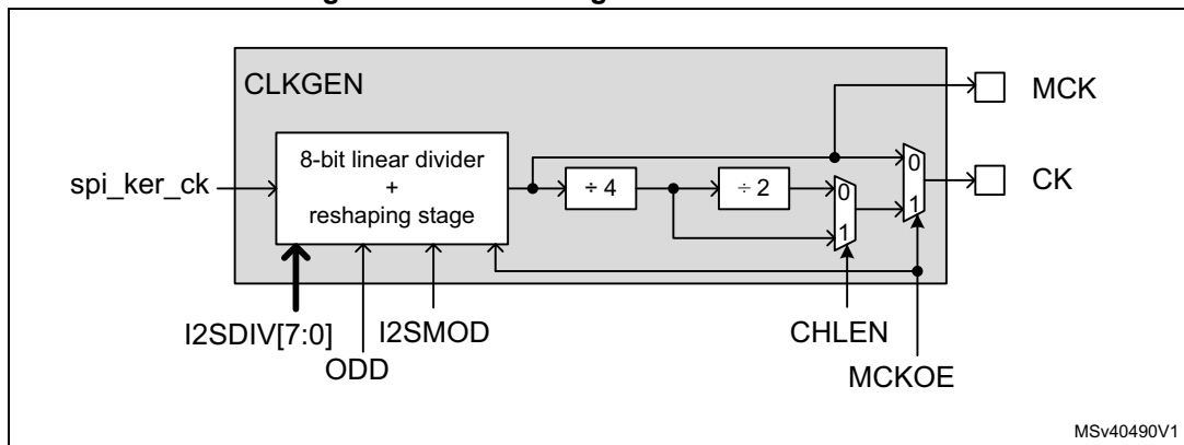
Figure 680. I 2 S clock generator architecture
