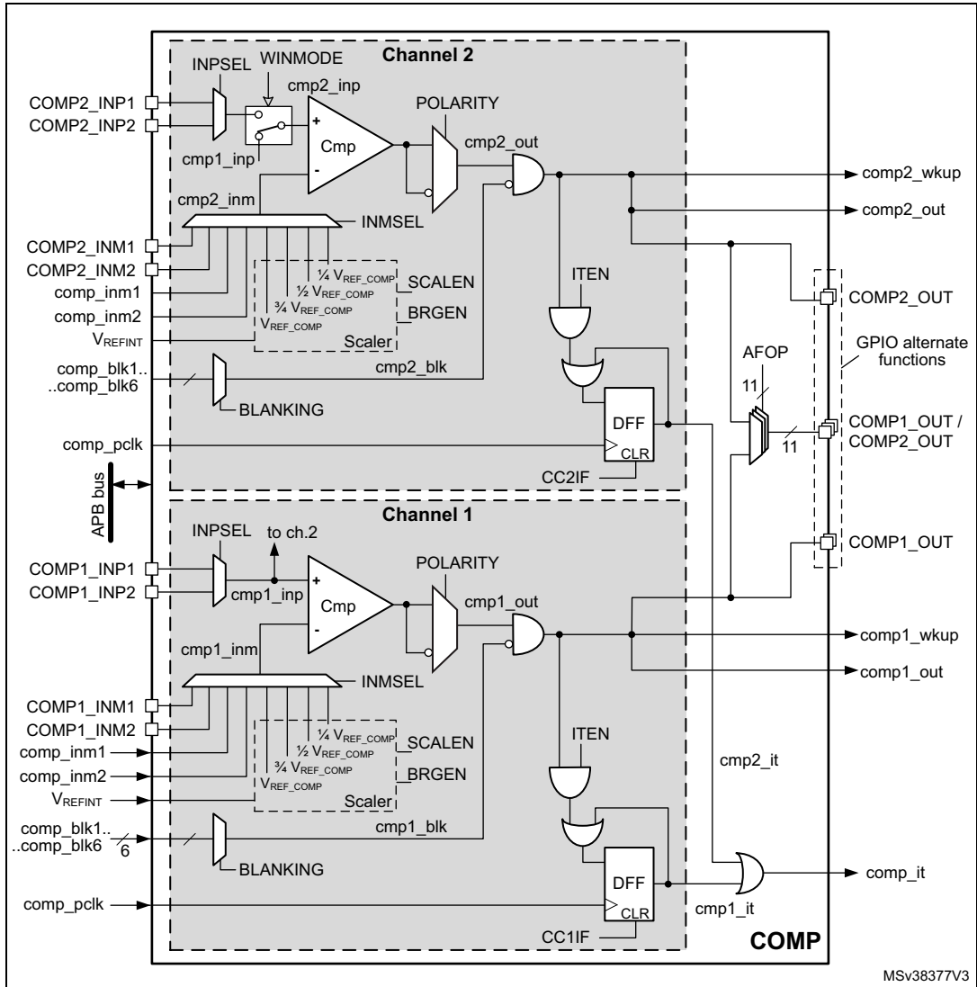
Figure 221. Comparator functional block diagram
