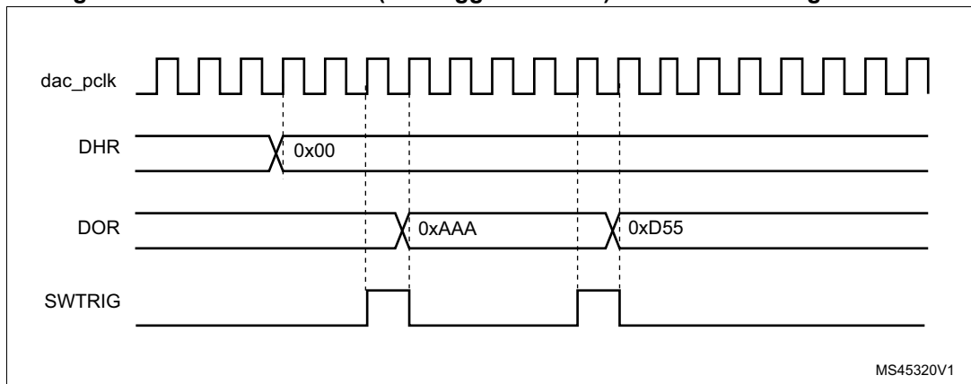
Figure 217. DAC conversion (SW trigger enabled) with LFSR wave generation
