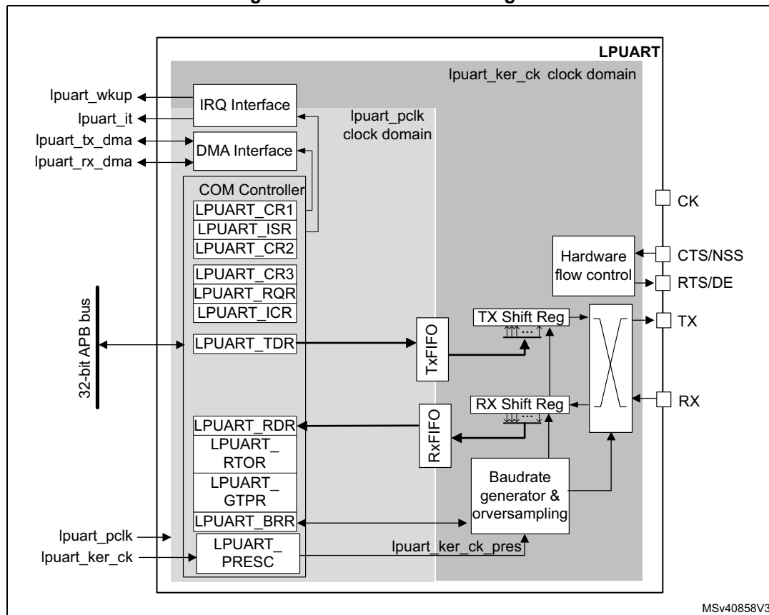
Figure 638. LPUART block diagram
