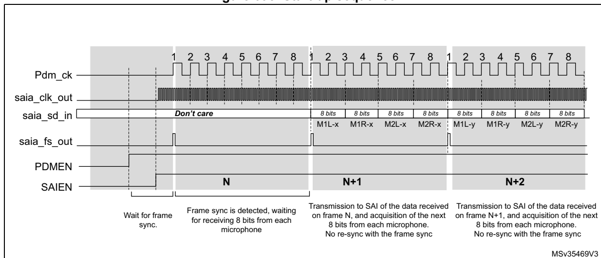
Figure 695. Start-up sequence
