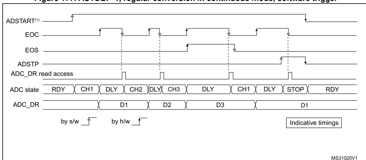
Figure 177. AUTDLY=1, regular conversion in continuous mode, software trigger
