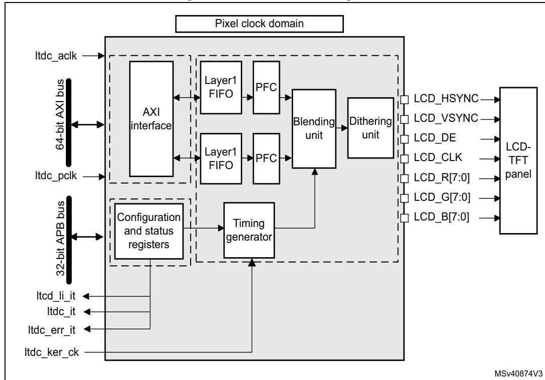
Figure 250. LTDC block diagram
