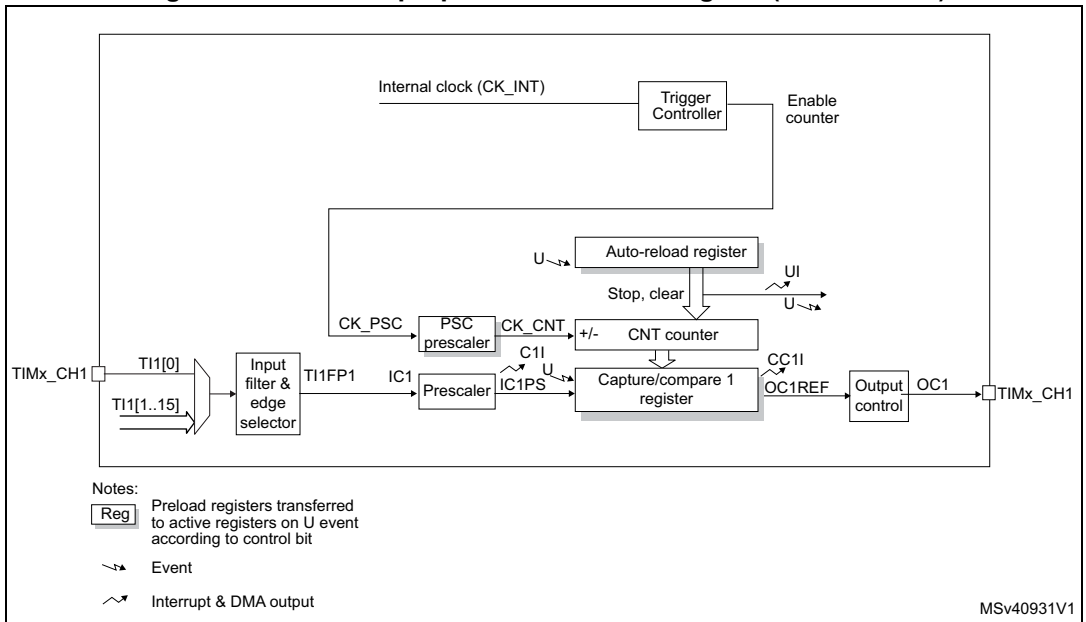
Figure 496. General-purpose timer block diagram (TIM13/TIM14)
