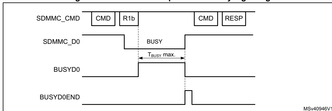
Figure 768. Command response R1b busy signaling
