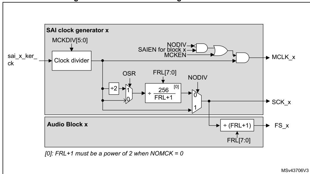
Figure 692. Audio block clock generator overview
