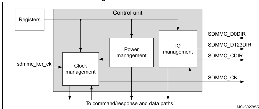
Figure 746. Control unit
