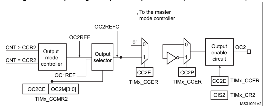
Figure 538. Output stage of capture/compare channel (channel 2 for TIM15)
