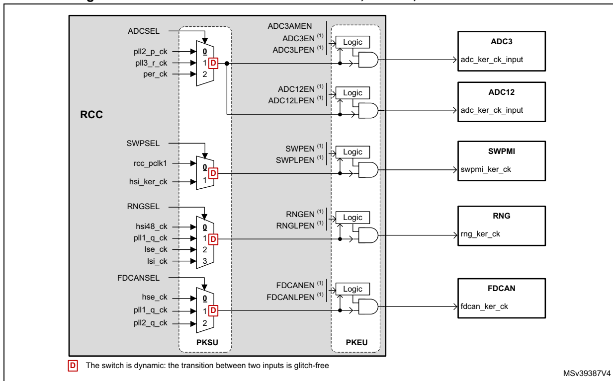
Figure 64. Kernel clock distribution For ADCs, SWPMI, RNG and FDCAN (2)
