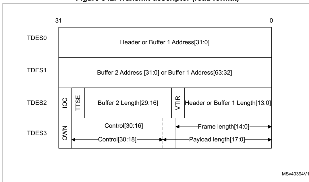
Figure 842. Transmit descriptor (read format)
