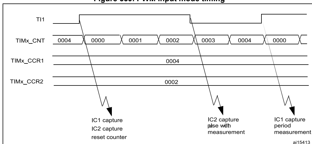
Figure 539. PWM input mode timing
