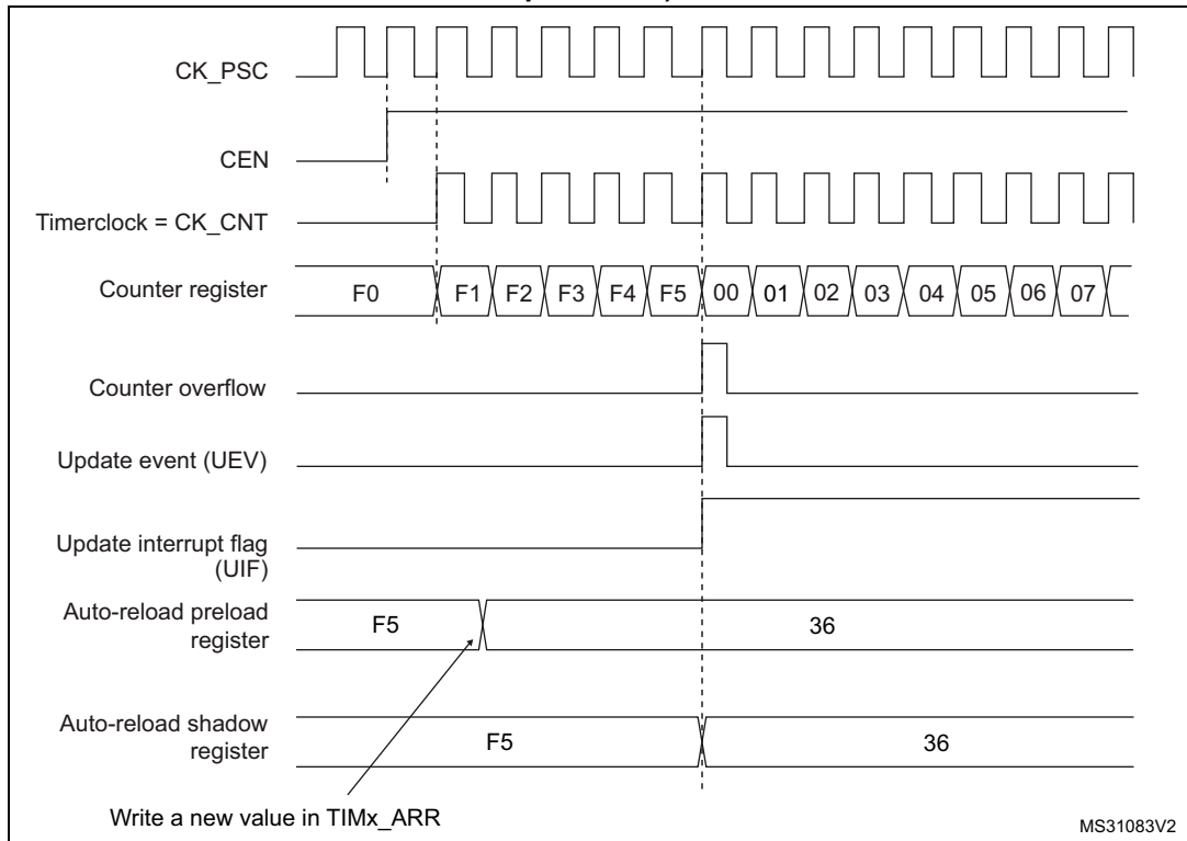
Figure 504. Counter timing diagram, update event when ARPE=1 (TIMx_ARR preloaded)
