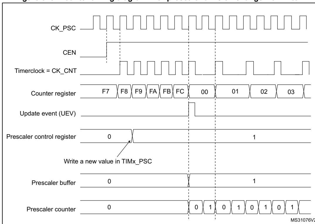
Figure 523. Counter timing diagram with prescaler division change from 1 to 2
