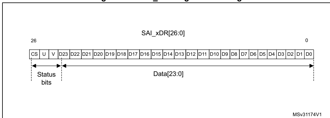
Figure 702. SAI_xDR register ordering
