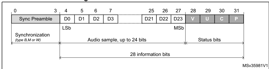
Figure 709. S/PDIF Sub-frame format
