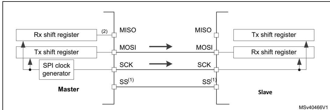
Figure 655. Simplex single master/single slave application (master in transmit-only/ slave in receive-only mode)
