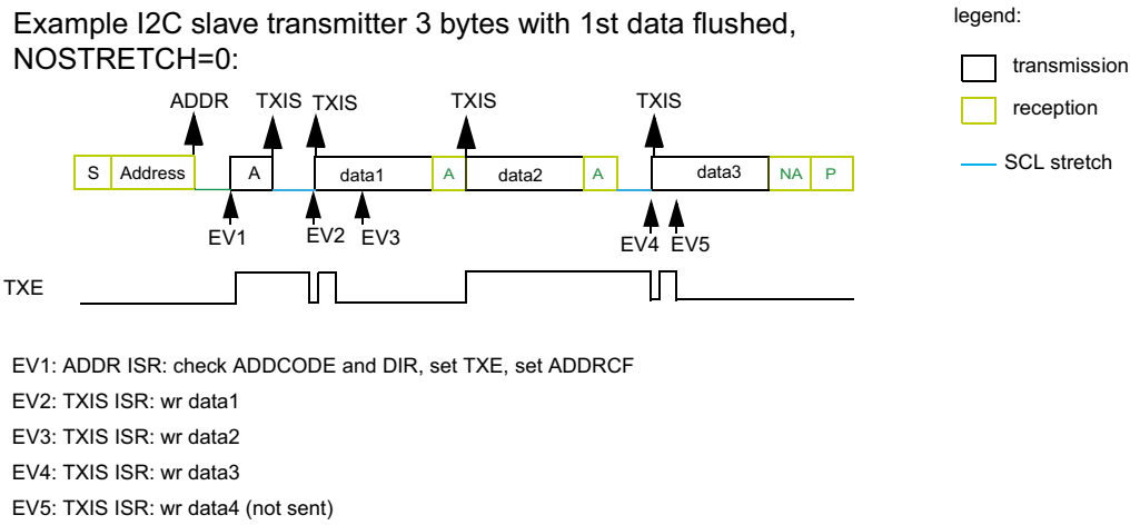
Figure 589. Transfer bus diagrams for I2C slave transmitter
