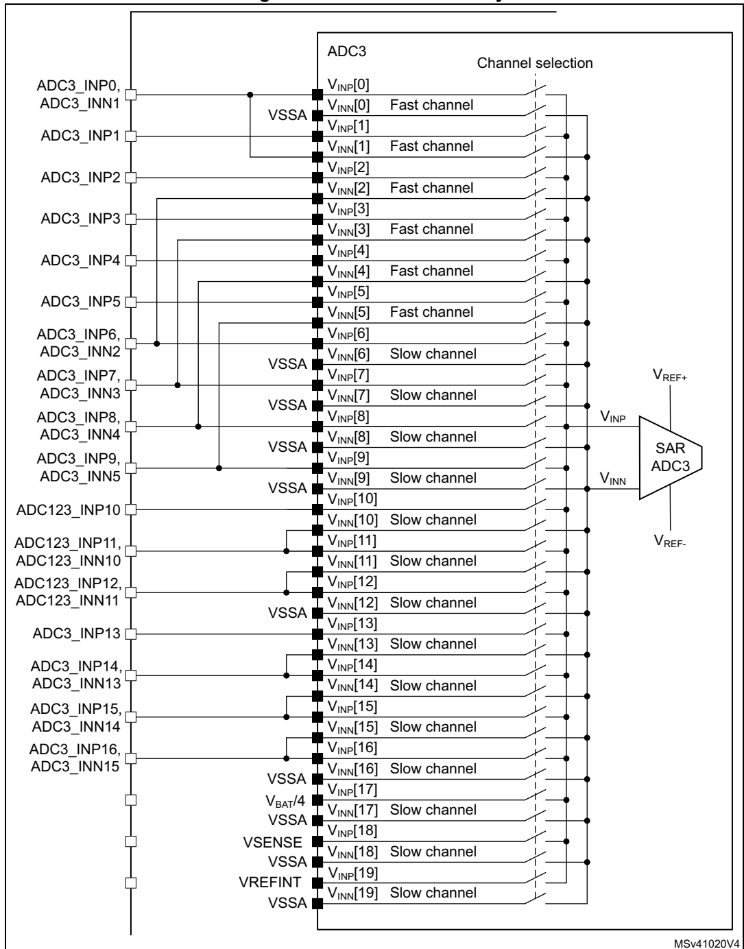
Figure 145. ADC3 connectivity
