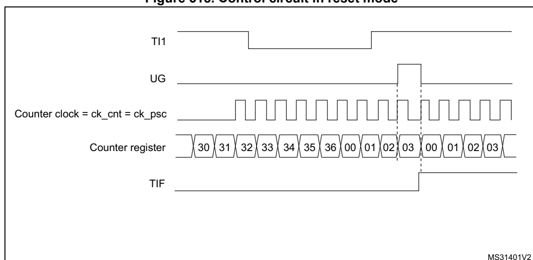
Figure 518. Control circuit in reset mode
