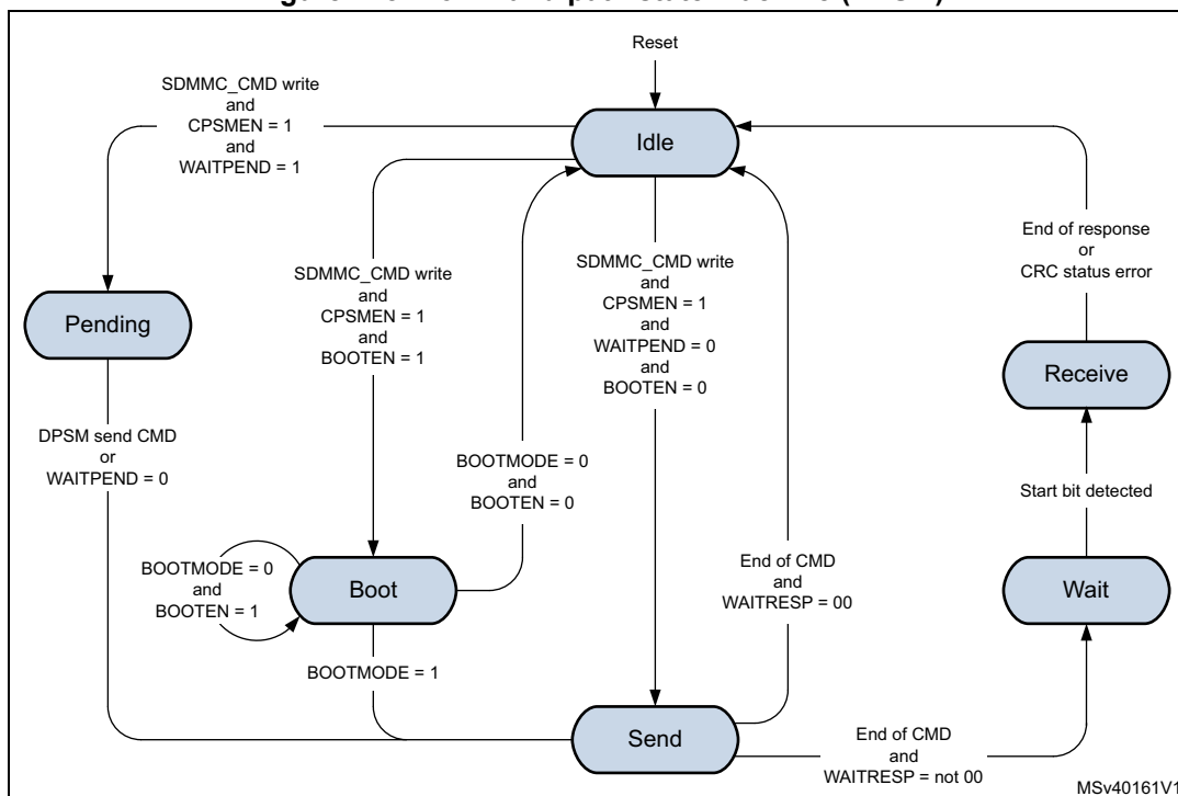
Figure 748. Command path state machine (CPSM)
