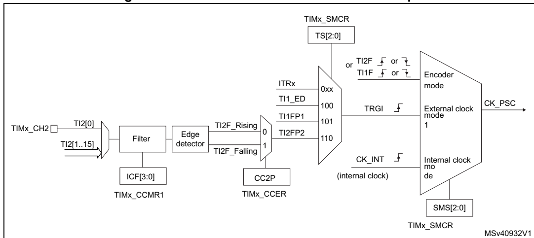
Figure 506. TI2 external clock connection example
