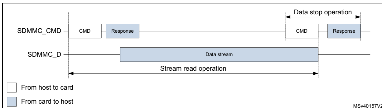
Figure 742. SDMMC (sequential) stream read operation
