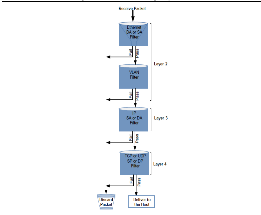
Figure 825. Packet filtering sequence
