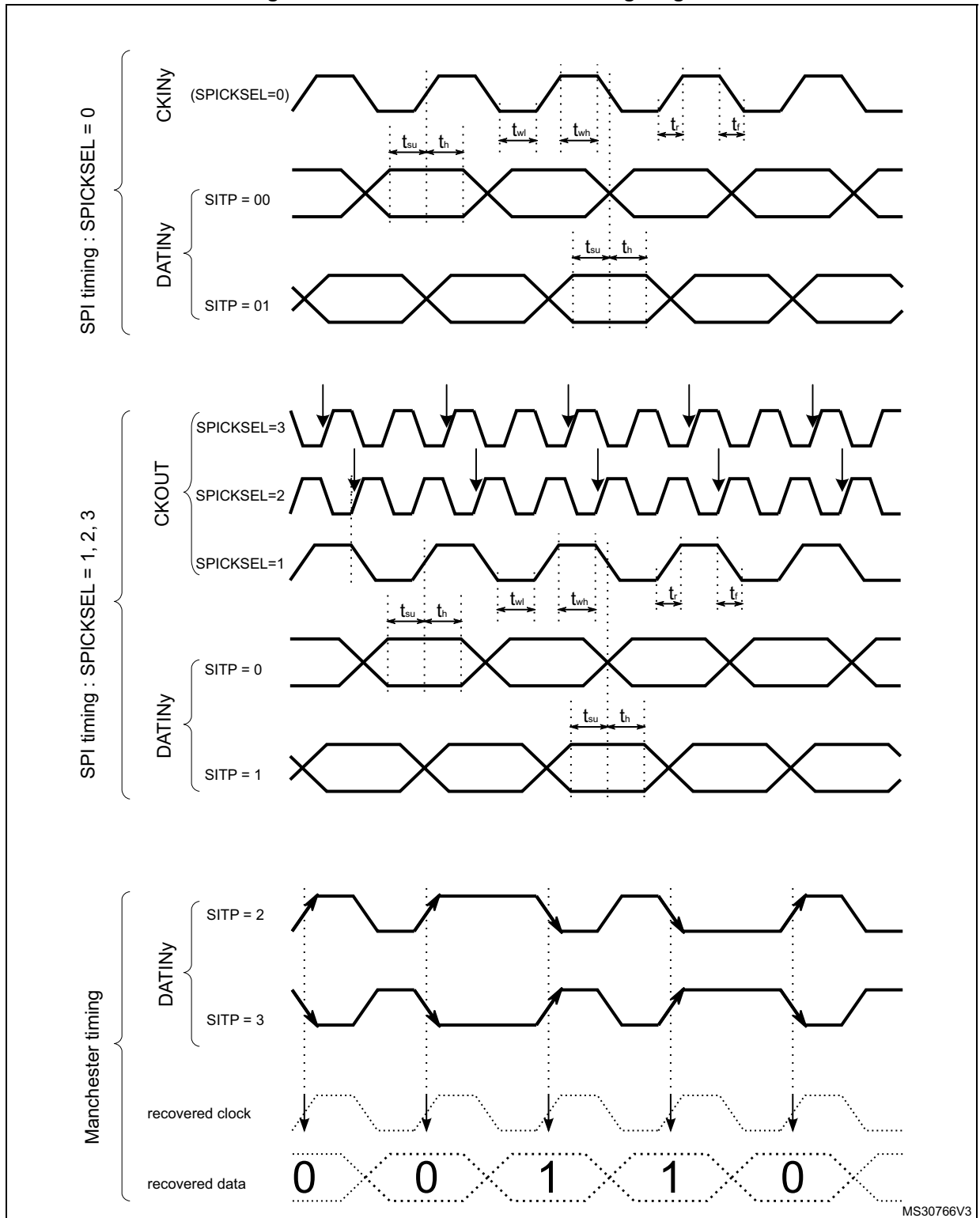
Figure 236. Channel transceiver timing diagrams
