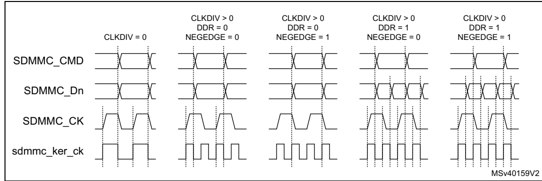
Figure 745. SDMMC Command and data phase relation
