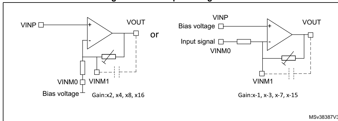
Figure 233. Example configuration
