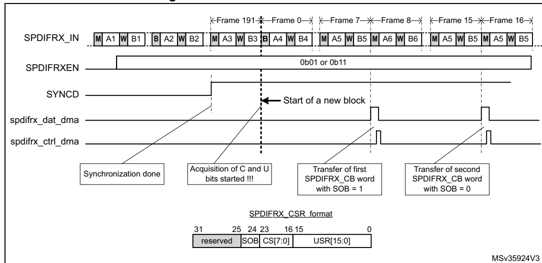
Figure 720. Channel/user data format
