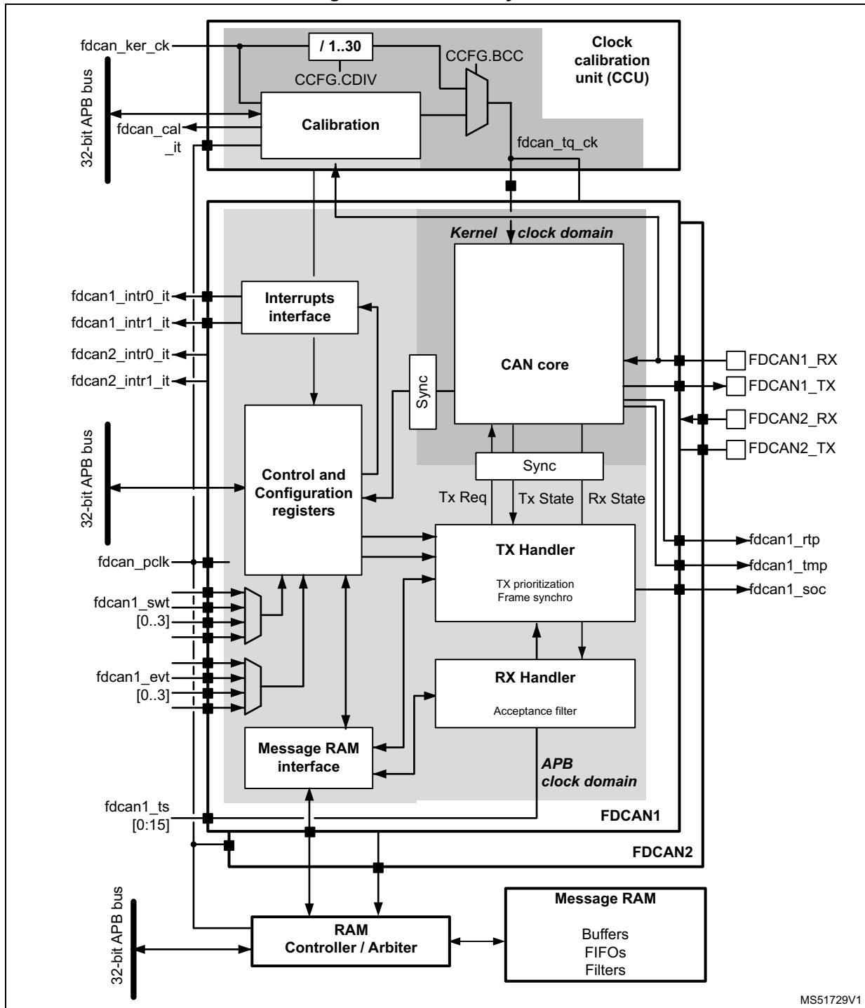
Figure 773. CAN subsystem
