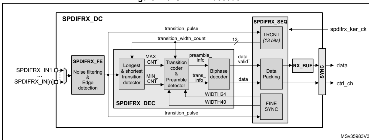
Figure 713. SPDIFRX decoder
