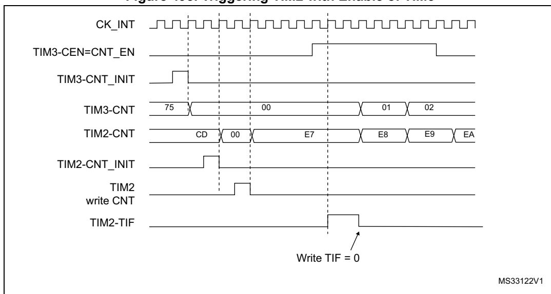
Figure 493. Triggering TIM2 with Enable of TIM3
