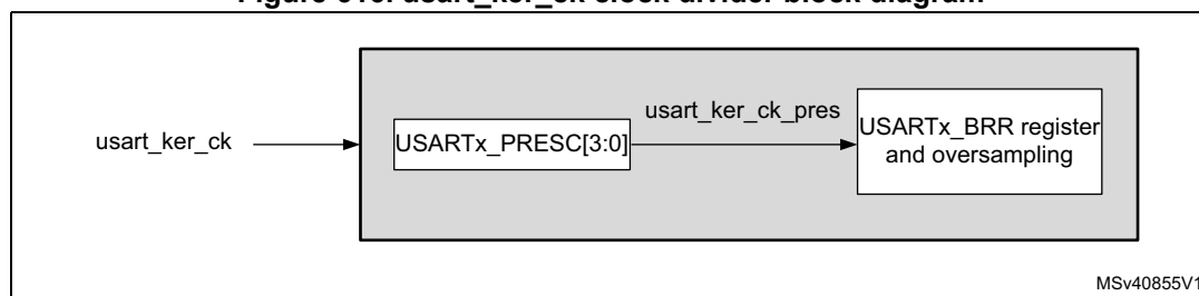
Figure 616. usart_ker_ck clock divider block diagram
