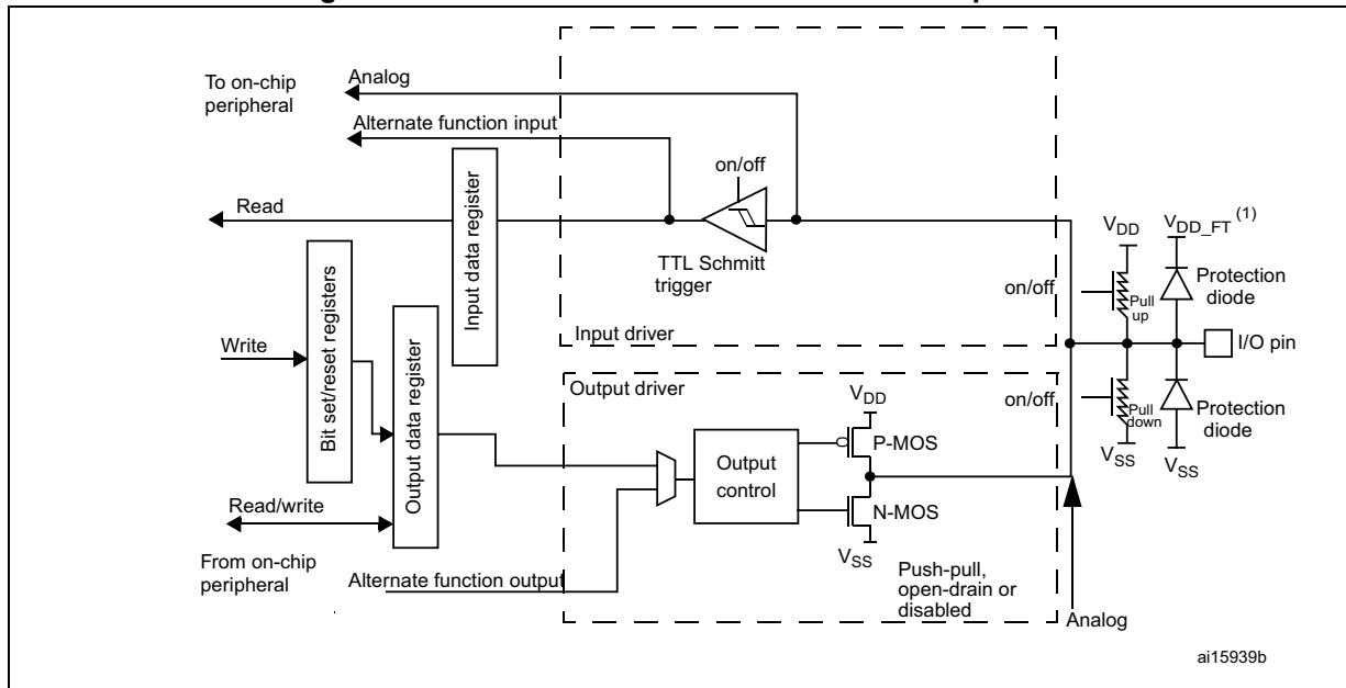
Figure 77. Basic structure of a 5-Volt tolerant I/O port bit
