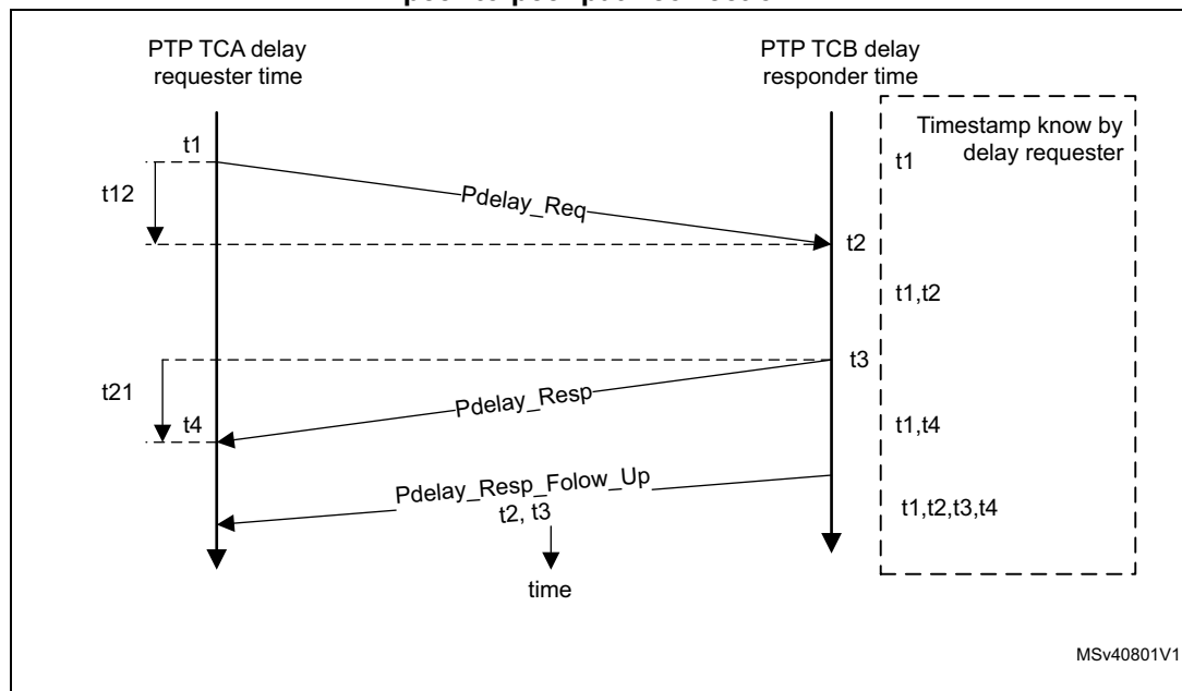
Figure 827. Propagation delay calculation in clocks supporting peer-to-peer path correction
