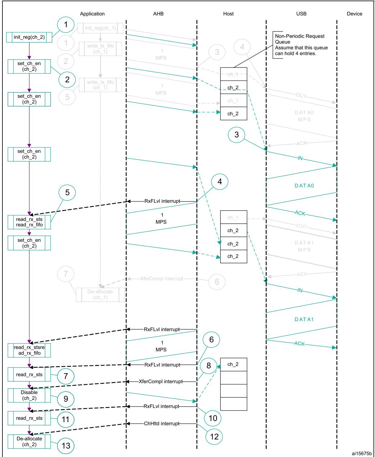
Figure 800. Bulk/control IN transactions
