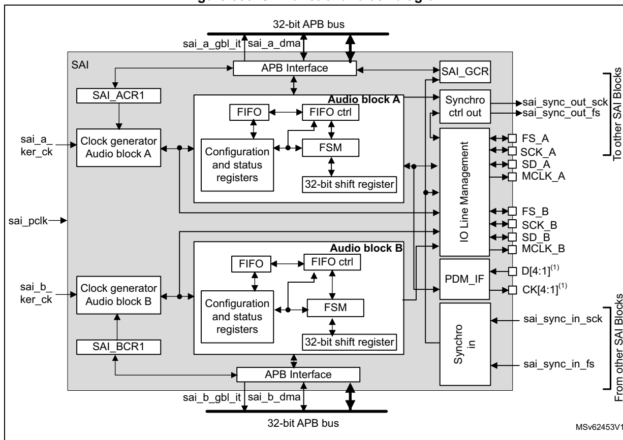
Figure 686. SAI functional block diagram
