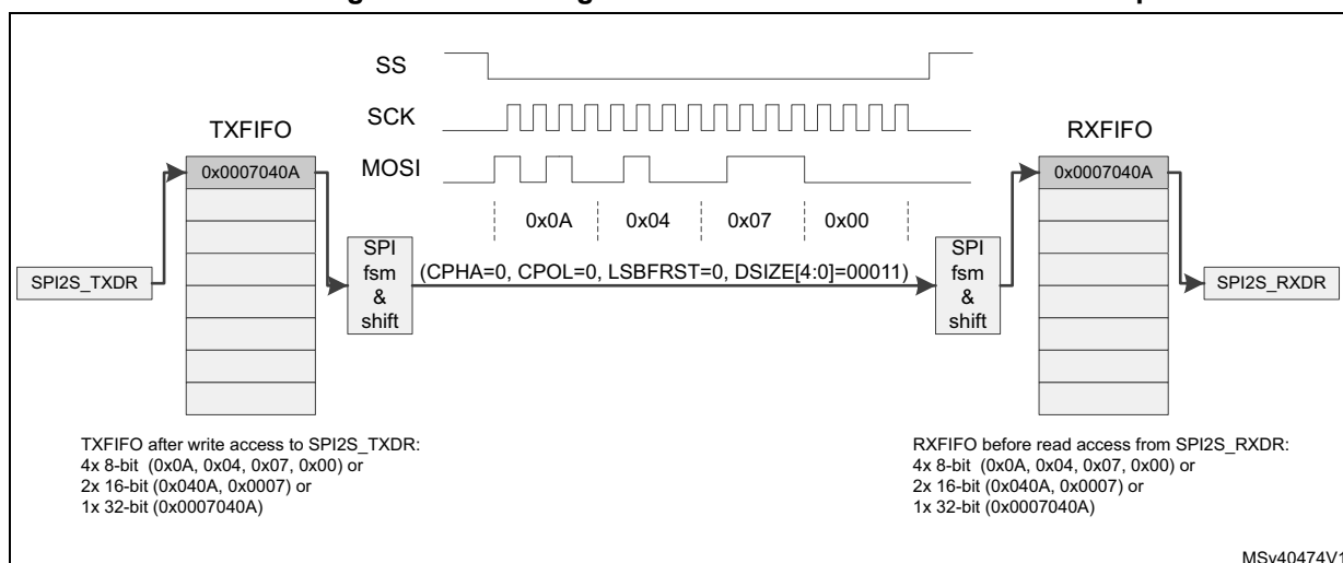
Figure 664. Packing data in FIFO for transmission and reception
