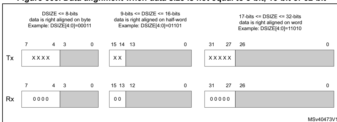
Figure 663. Data alignment when data size is not equal to 8-bit, 16-bit or 32-bit
