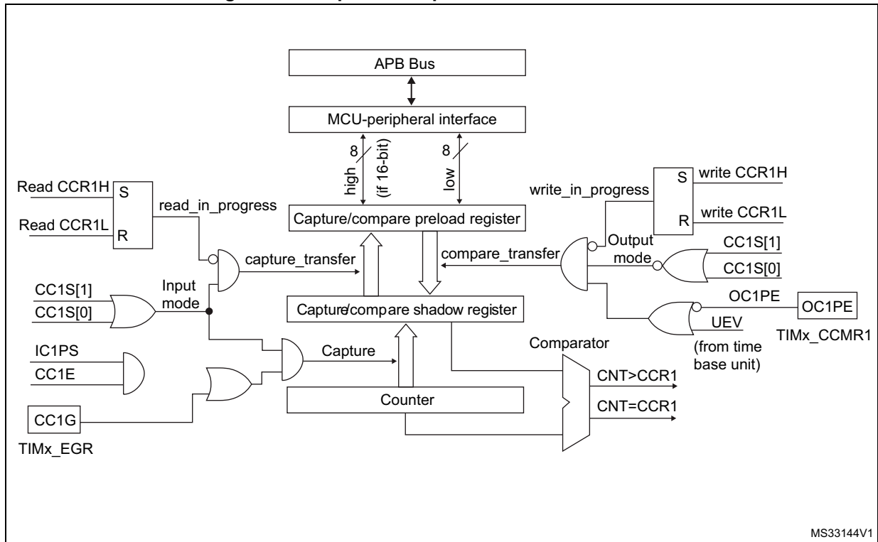
Figure 472. Capture/Compare channel 1 main circuit
