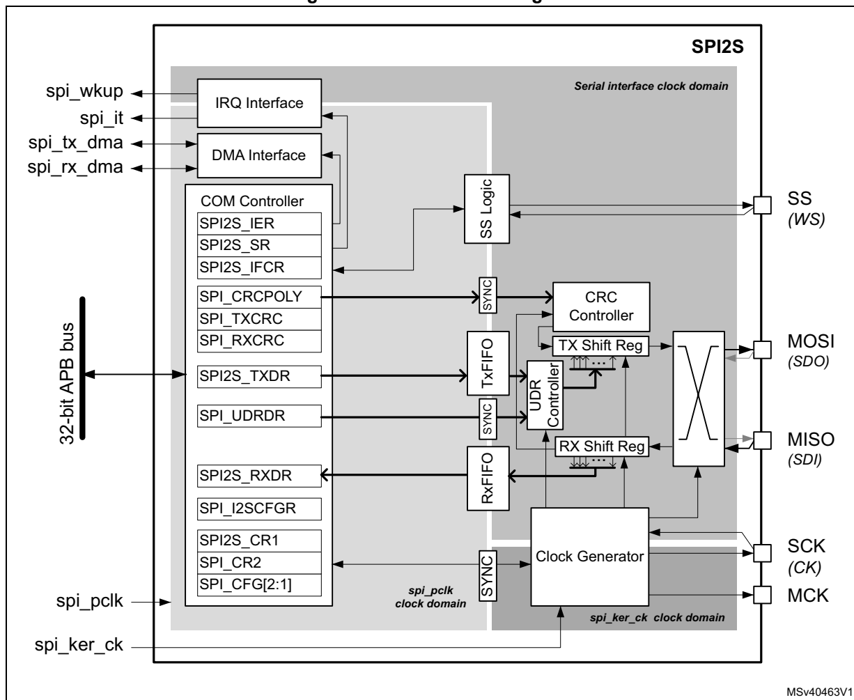
Figure 652. SPI2S block diagram
