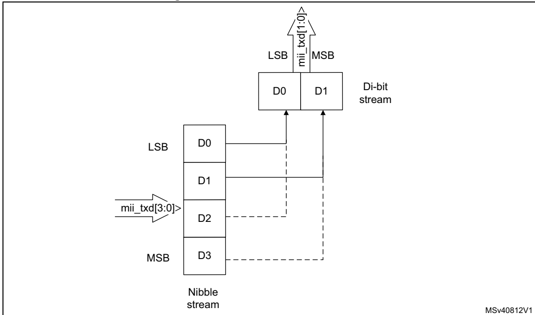
Figure 838. Transmission bit order
