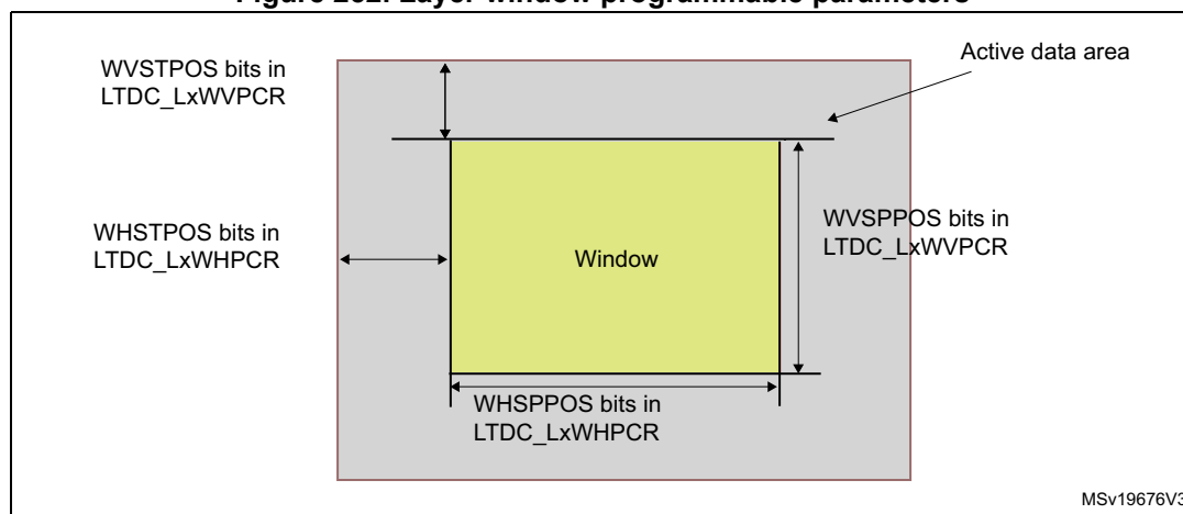
Figure 252. Layer window programmable parameters
