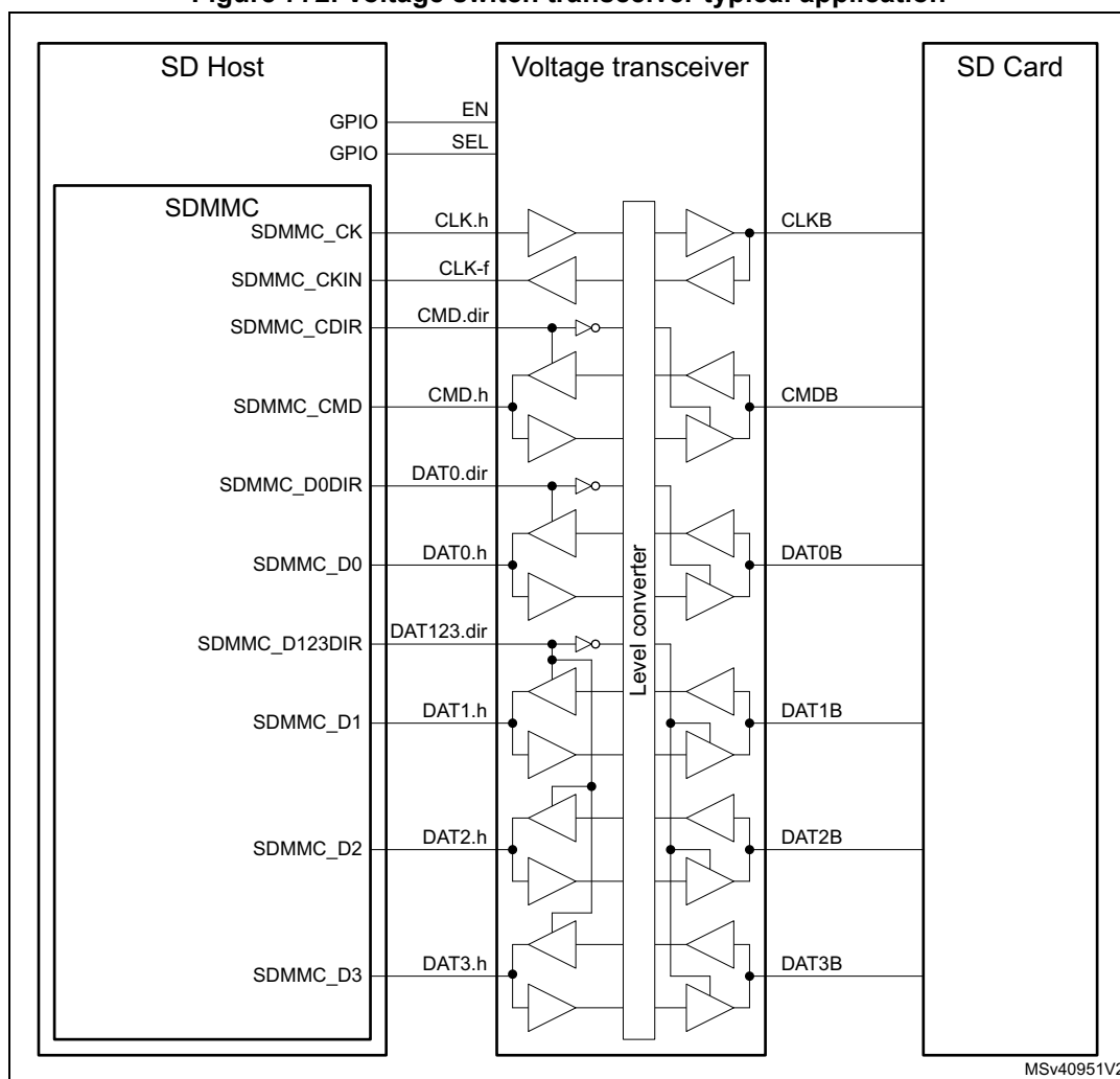
Figure 772. Voltage switch transceiver typical application
