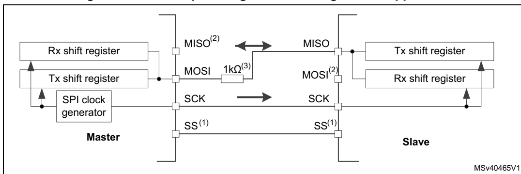
Figure 654. Half-duplex single master/ single slave application
