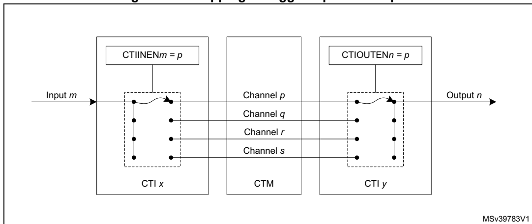
Figure 868. Mapping of trigger inputs to outputs
