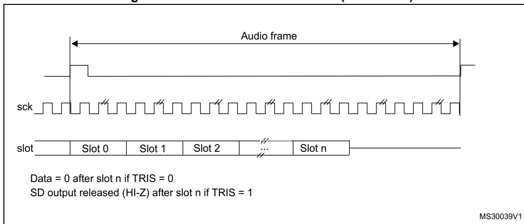
Figure 689. FS role is start of frame (FSDEF = 0)
