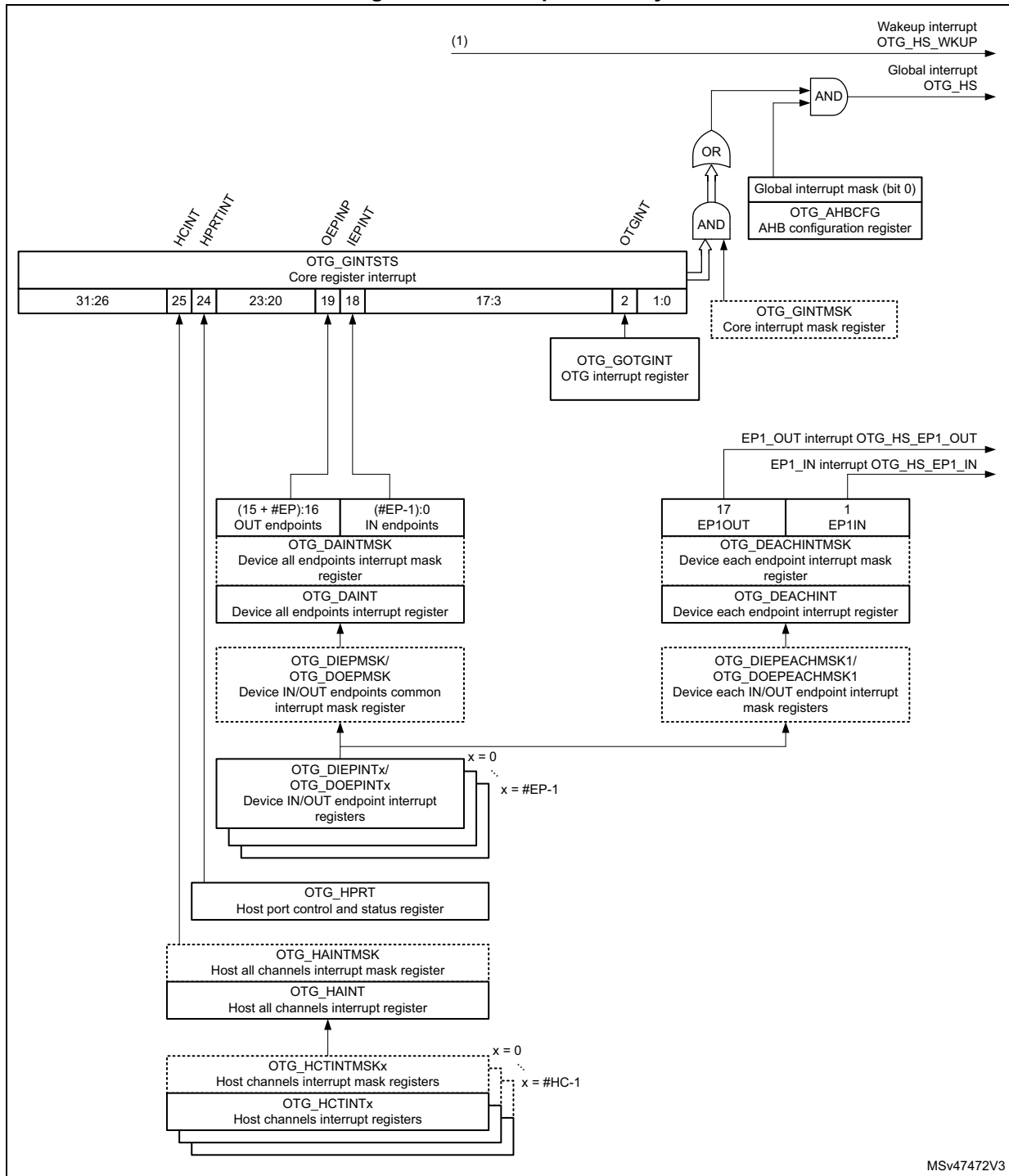
Figure 796. Interrupt hierarchy
