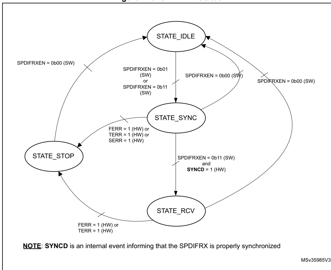
Figure 718. SPDIFRX States
