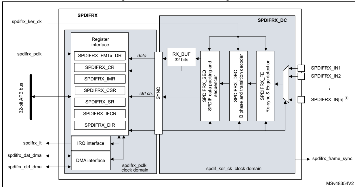
Figure 708. SPDIFRX block diagram
