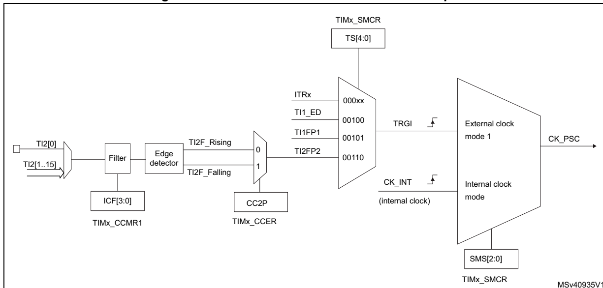
Figure 533. TI2 external clock connection example
