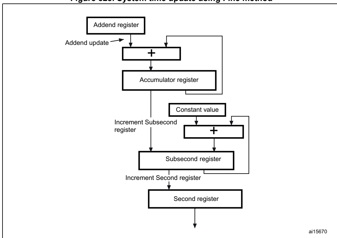
Figure 828. System time update using Fine method
