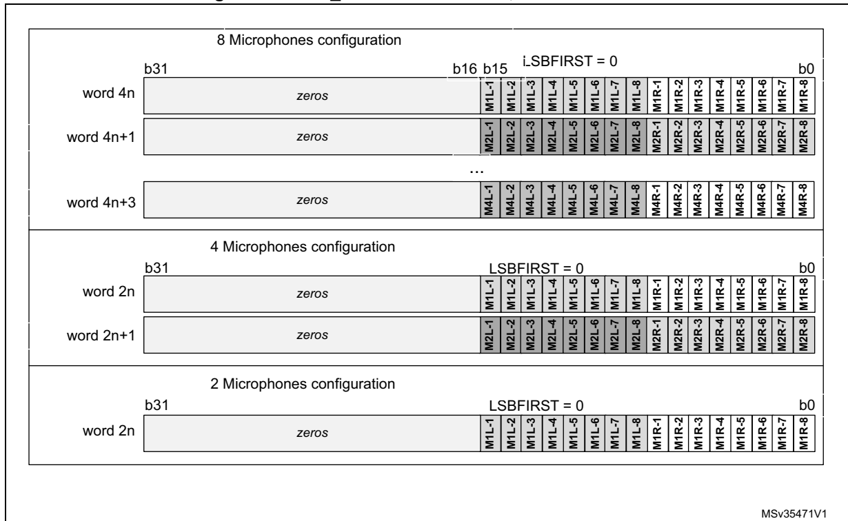
Figure 697. SAI_ADR format in TDM, 16-bit slot width
