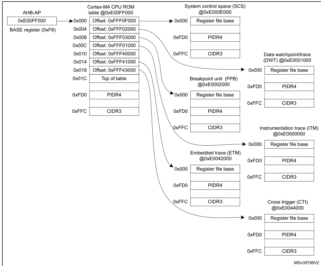
Figure 872. Cortex-M4 CoreSight Topology
