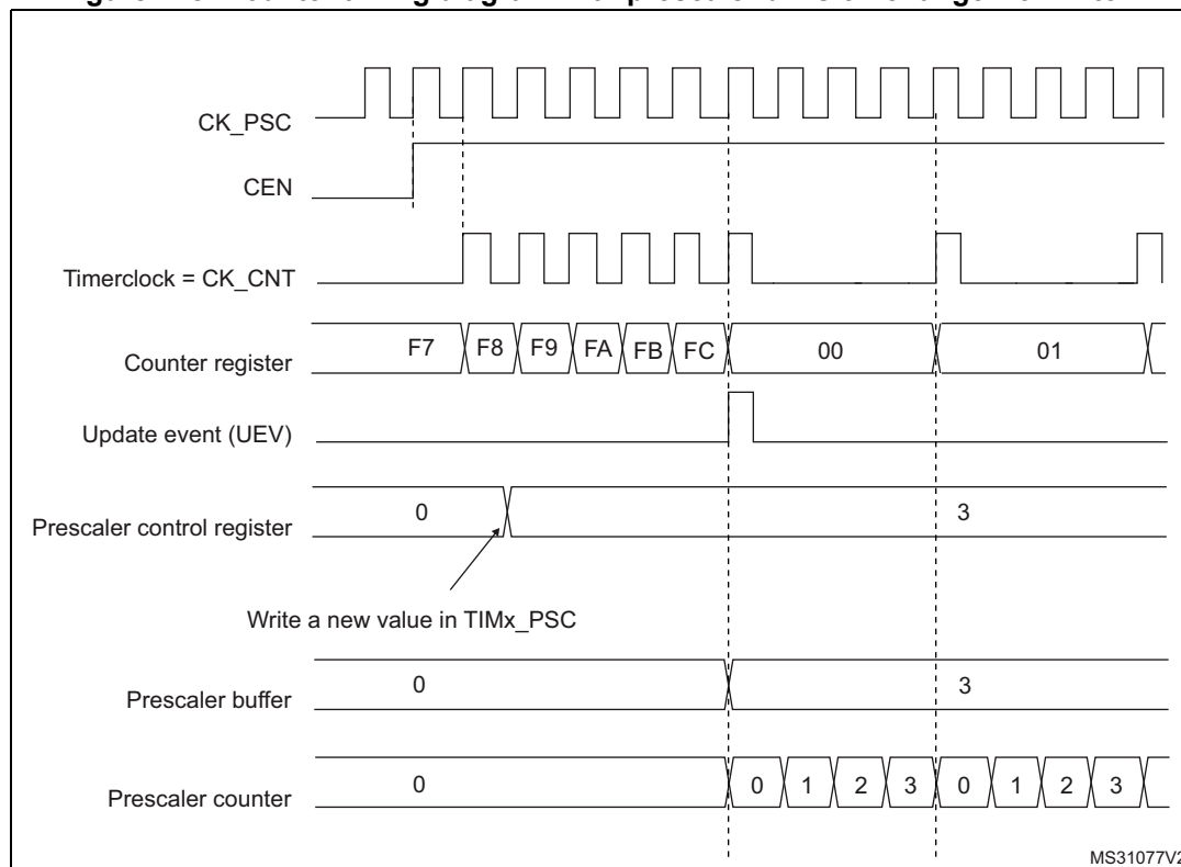
Figure 448. Counter timing diagram with prescaler division change from 1 to 4
