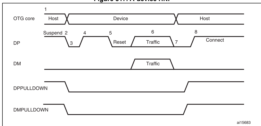
Figure 817. A-device HNP
