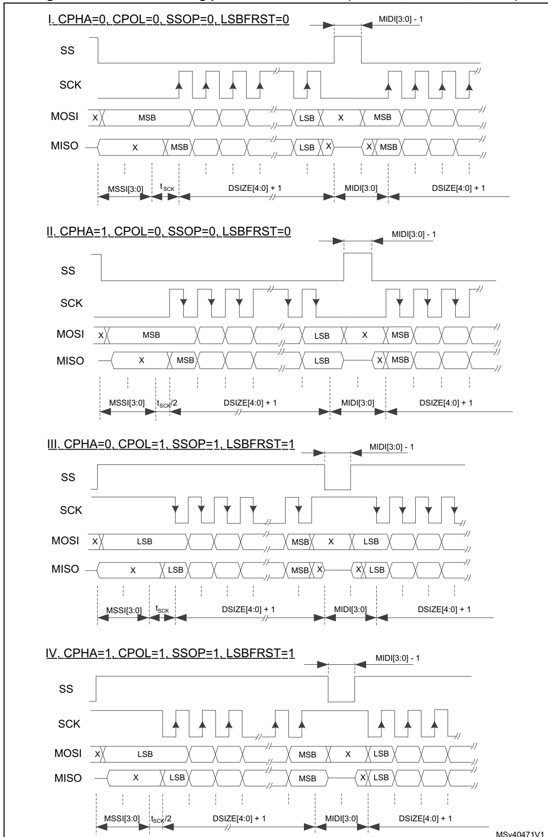
Figure 661. SS interleaving pulses between data (SSOE=1, SSOM=1,SSM=0)
