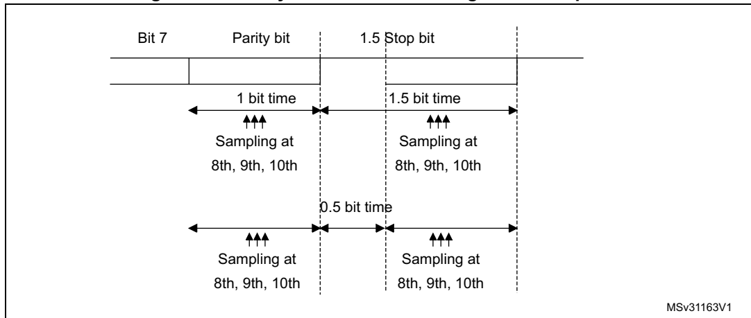
Figure 628. Parity error detection using the 1.5 stop bits
