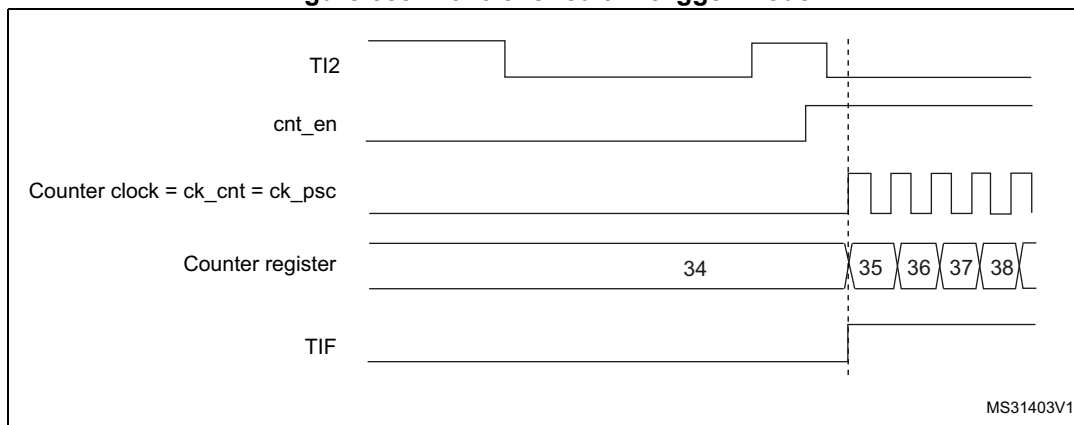
Figure 553. Control circuit in trigger mode
