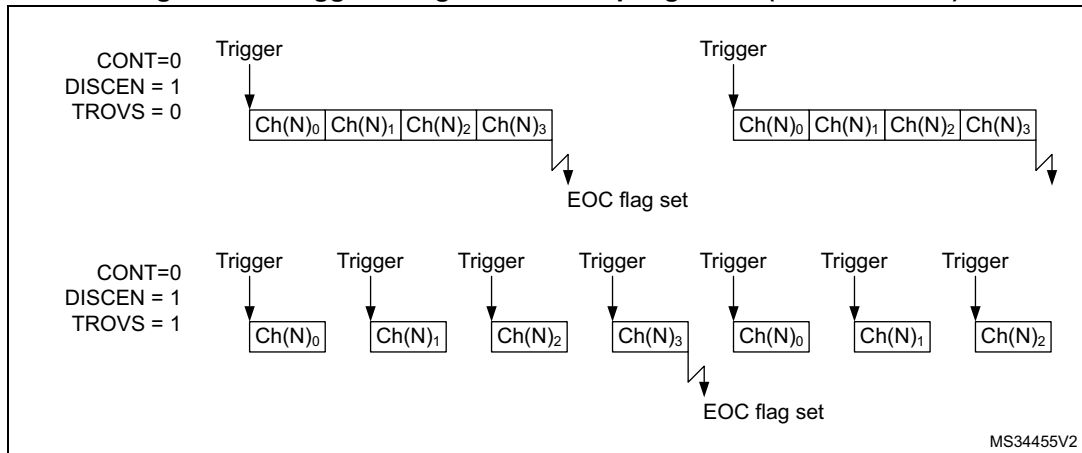
Figure 188. Triggered regular oversampling mode (TROVS bit = 1)
