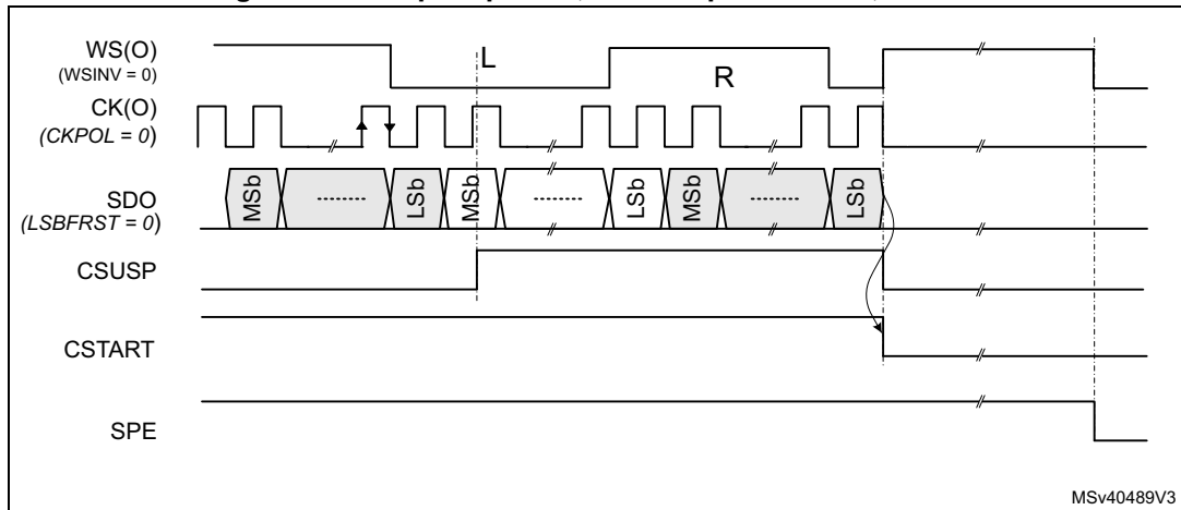
Figure 679. Stop sequence, I2S Philips standard, master
