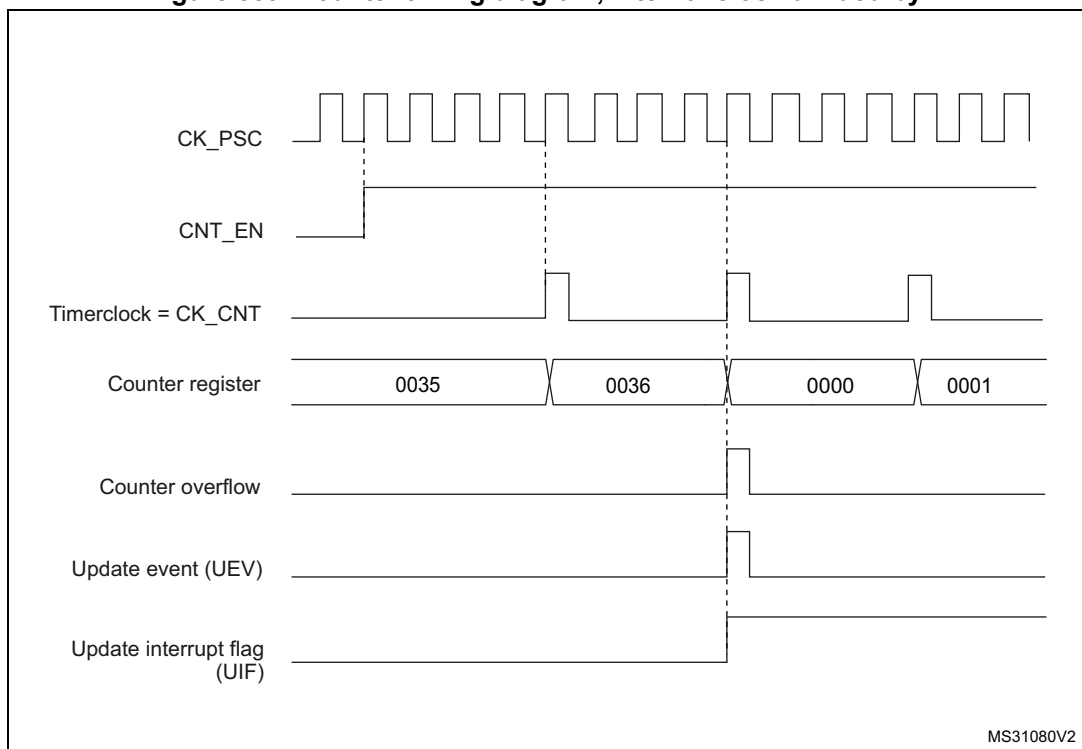
Figure 559. Counter timing diagram, internal clock divided by 4
