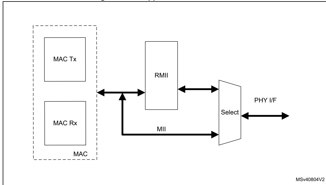
Figure 831. Supported PHY interfaces
