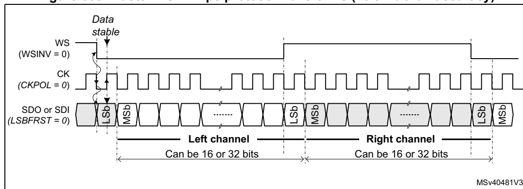
Figure 668. Master I2S Philips protocol waveforms (16/32-bit full accuracy)
