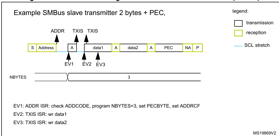
Figure 605. Transfer bus diagrams for SMBus slave transmitter (SBC=1)
