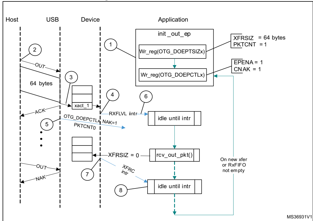
Figure 813. Bulk OUT transaction
