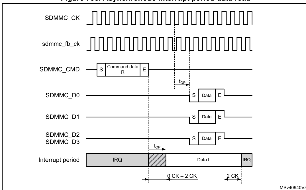
Figure 758. Asynchronous interrupt period data read
