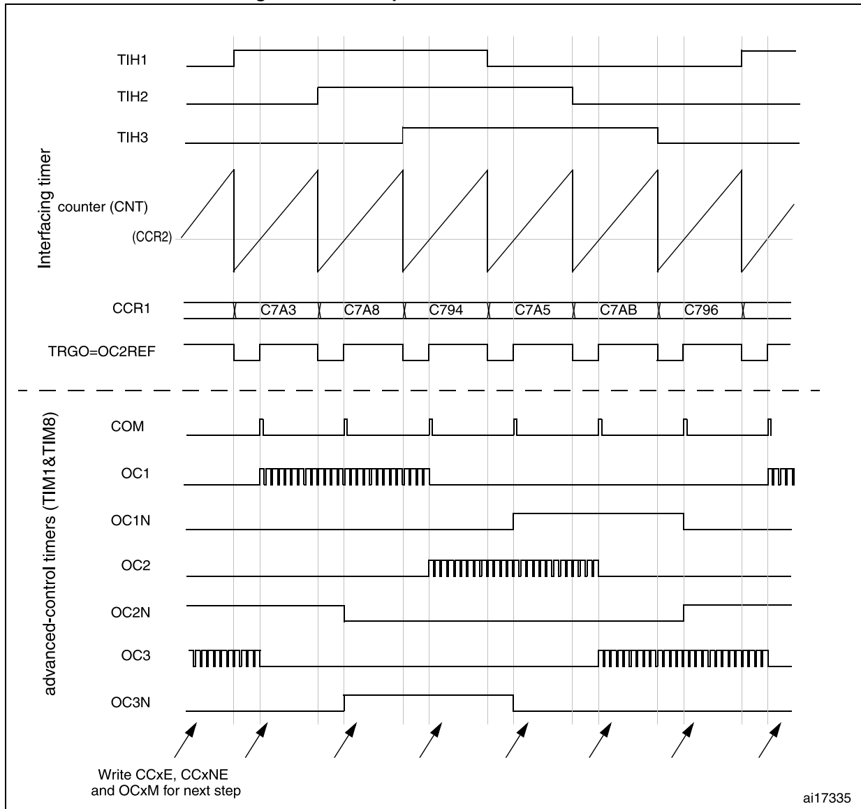
Figure 441. Example of Hall sensor interface
