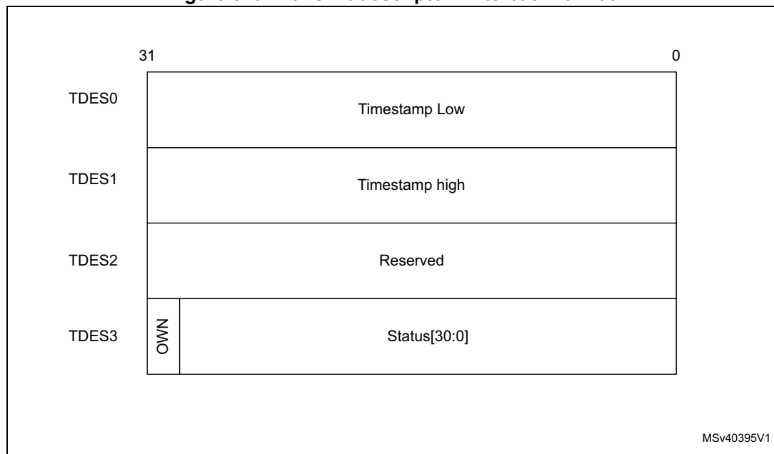
Figure 843. Transmit descriptor write-back format
