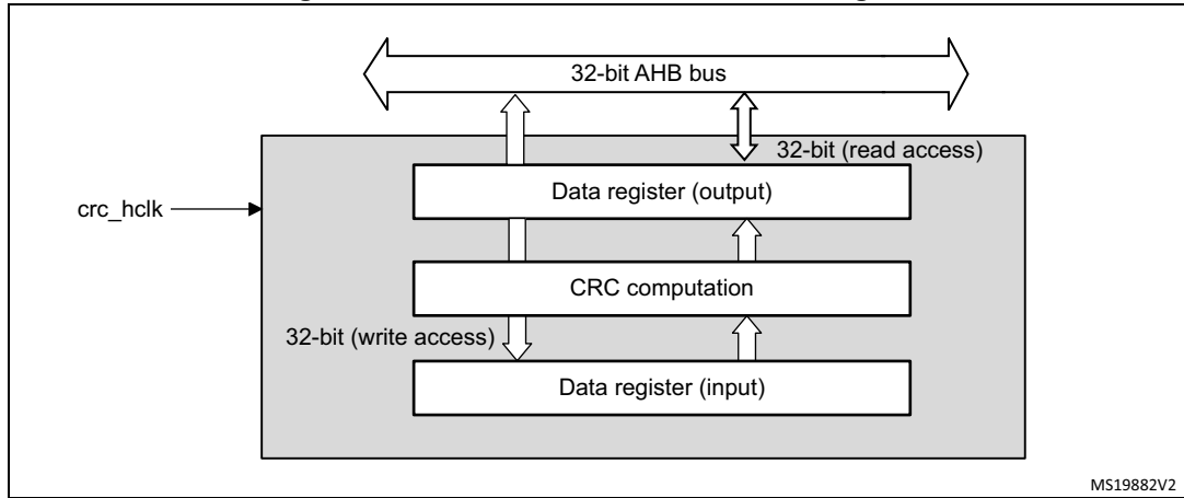
Figure 102. CRC calculation unit block diagram
