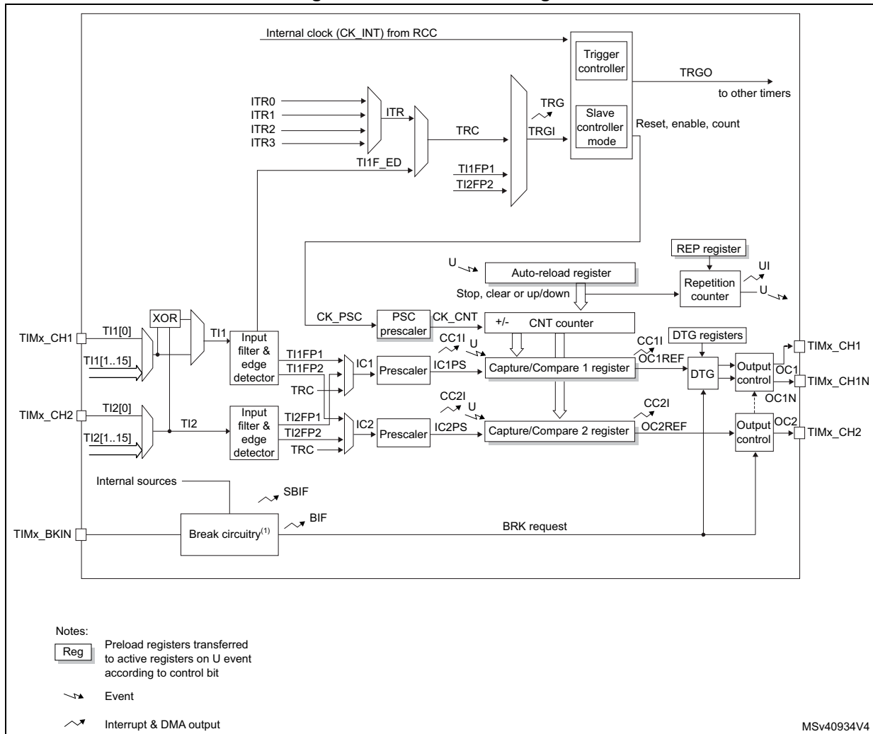
Figure 521. TIM15 block diagram
