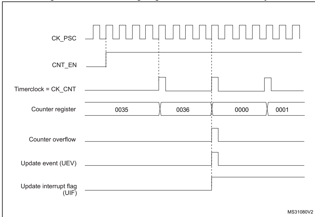
Figure 392. Counter timing diagram, internal clock divided by N
