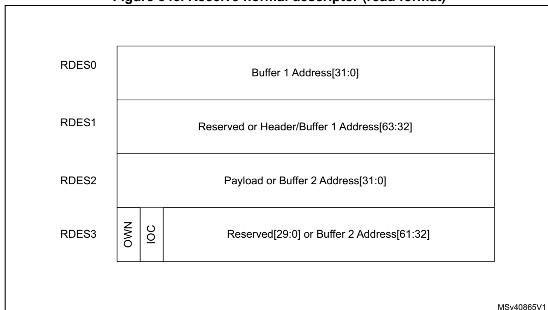
Figure 845. Receive normal descriptor (read format)
