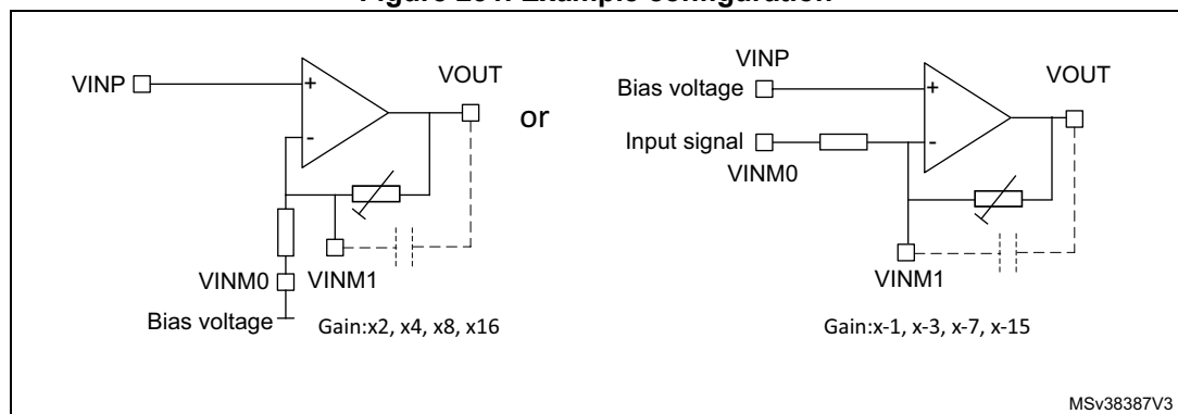
Figure 231. Example configuration
