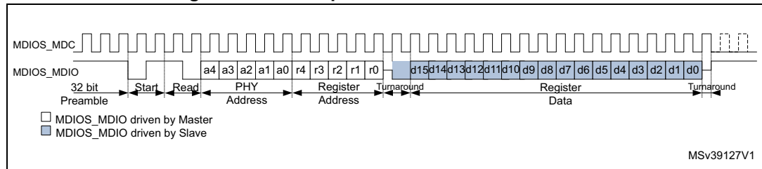
Figure 738. MDIO protocol read frame waveform
