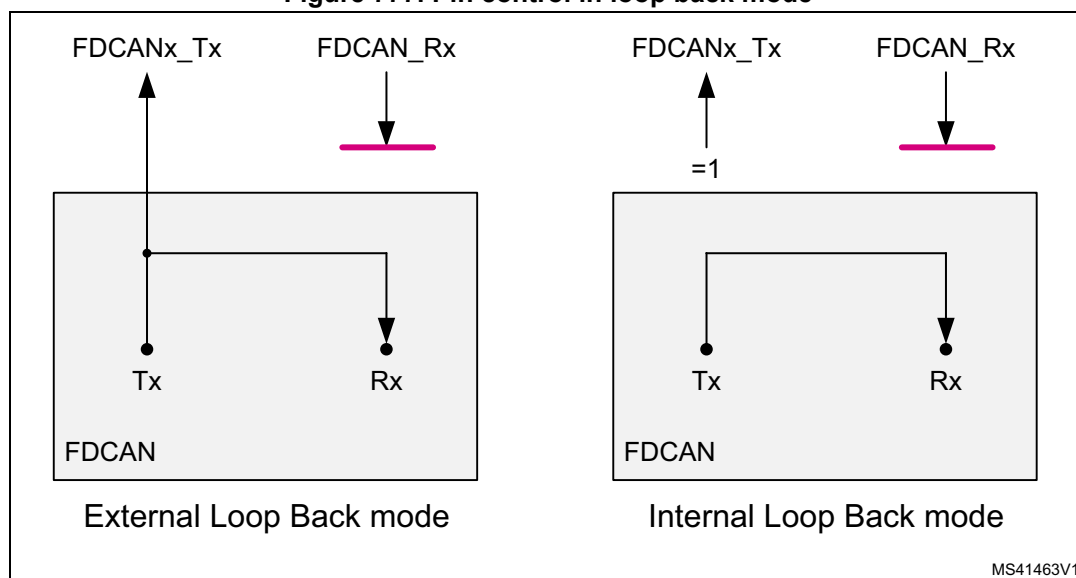
Figure 777. Pin control in loop back mode
