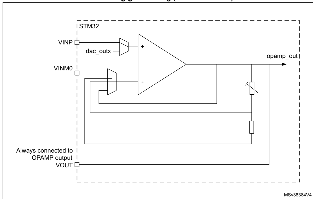
Figure 231. Example configuration
