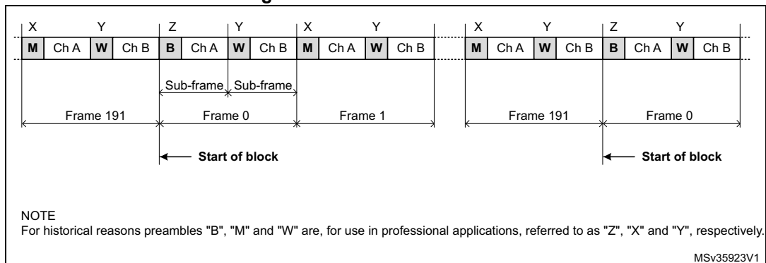
Figure 710. S/PDIF block format
