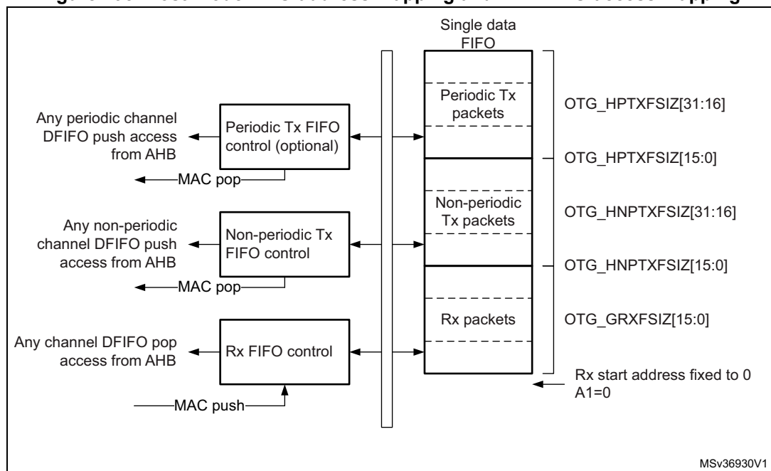
Figure 795. Host-mode FIFO address mapping and AHB FIFO access mapping
