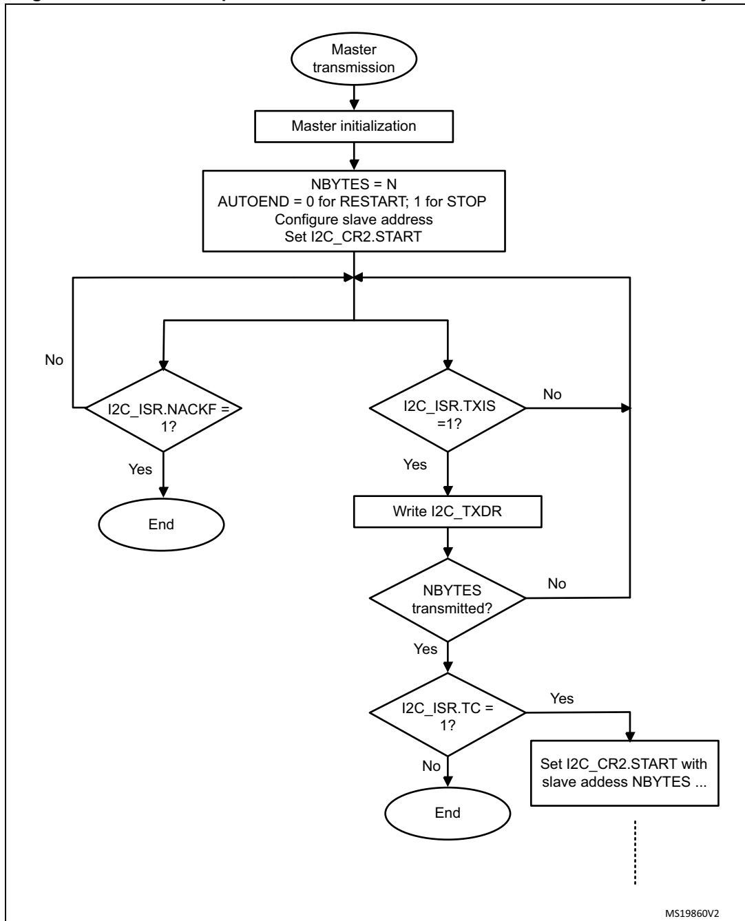
Figure 597. Transfer sequence flowchart for I2C master transmitter for N≤255 bytes
