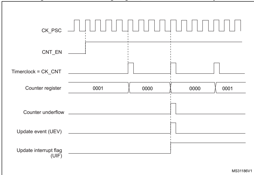
Figure 398. Counter timing diagram, internal clock divided by N
