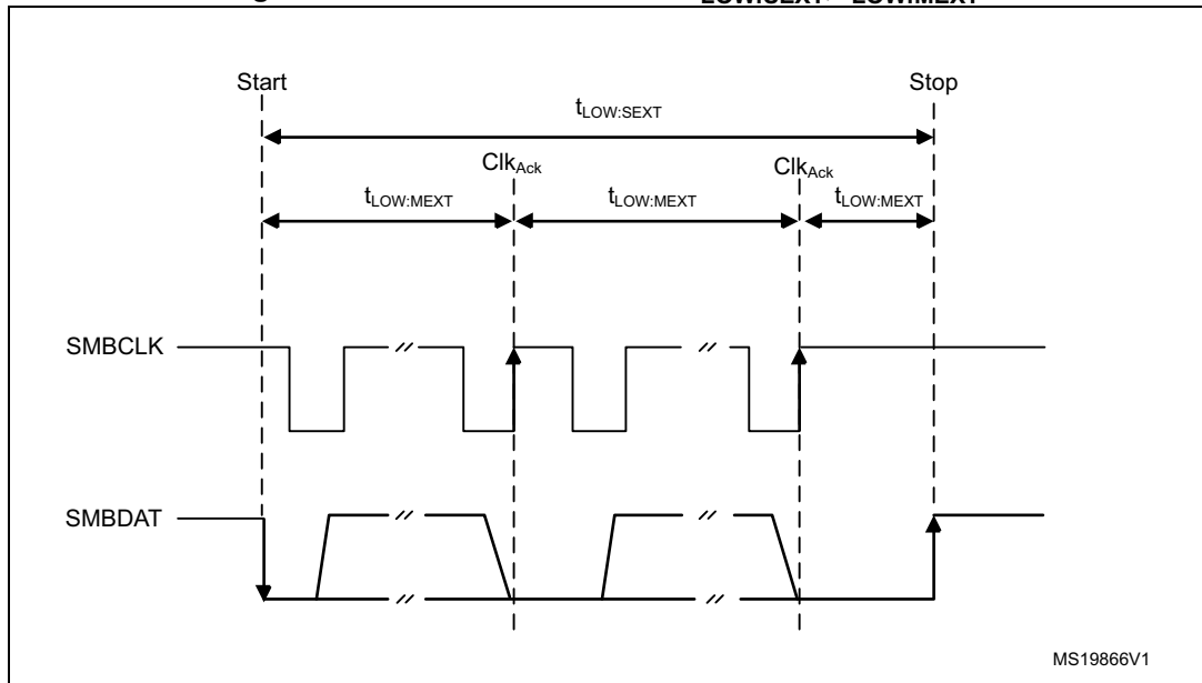
Figure 603. Timeout intervals for t_{LOW:SEXT} , t_{LOW:MEXT}
