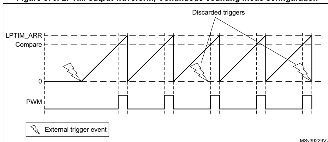
Figure 570. LPTIM output waveform, Continuous counting mode configuration
