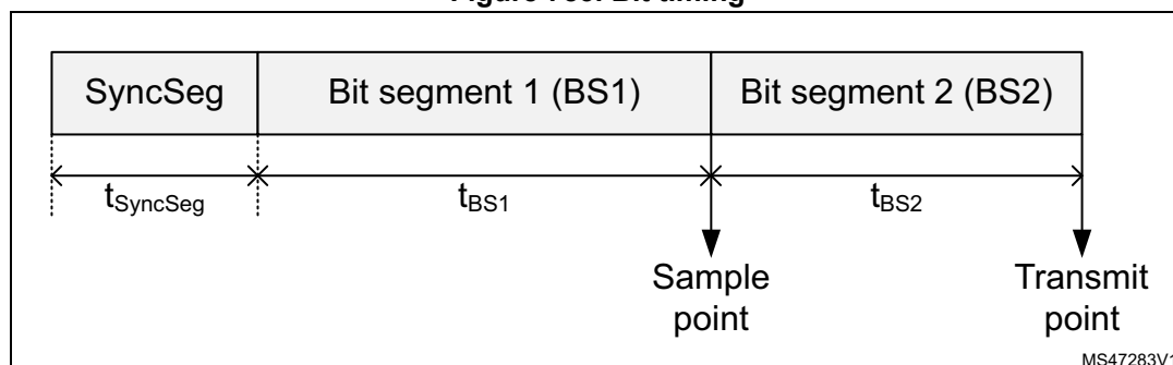
Figure 783. Bit timing
