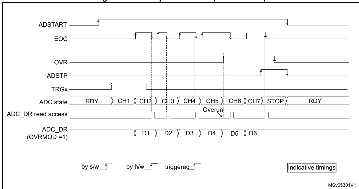
Figure 176. Example of overrun (OVRMOD = 1)
