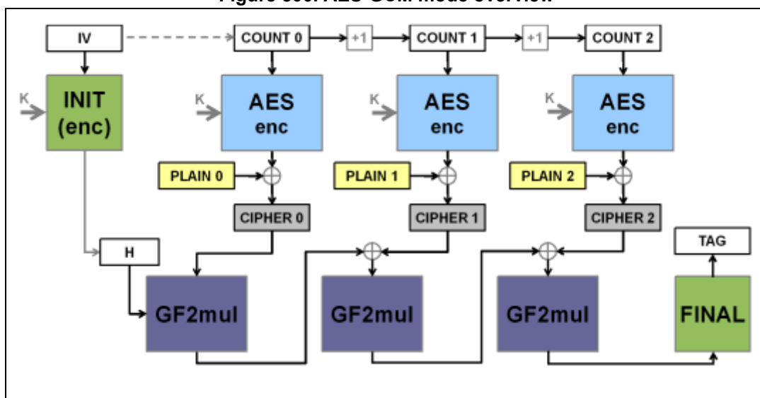
Figure 300. AES-GCM mode overview
