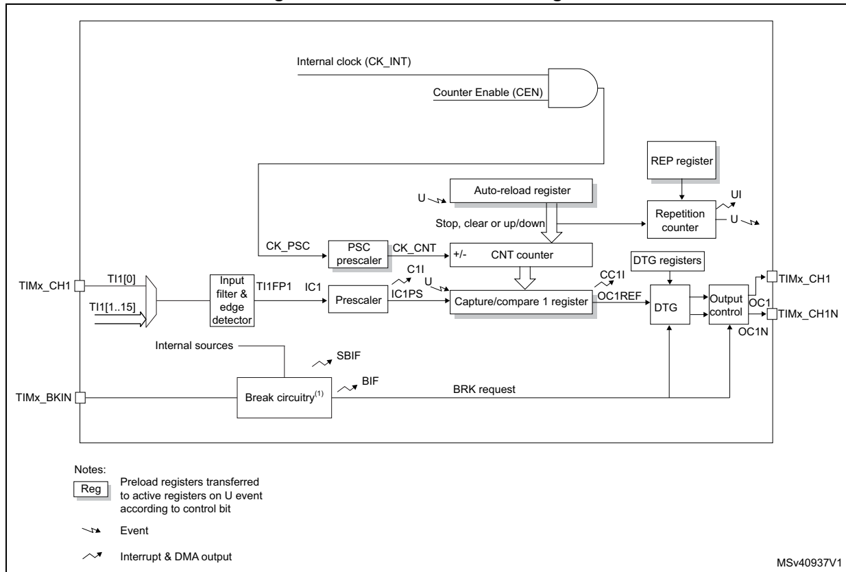
Figure 522. TIM16/TIM17 block diagram
