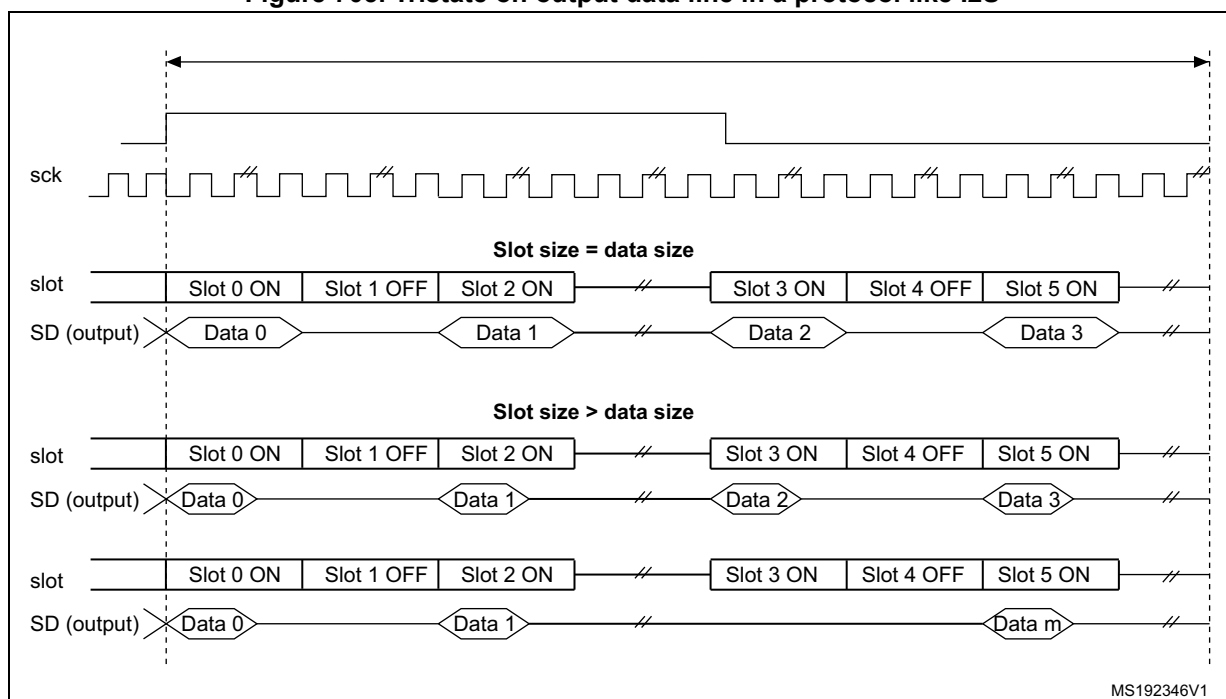
Figure 705. Tristate on output data line in a protocol like I2S
