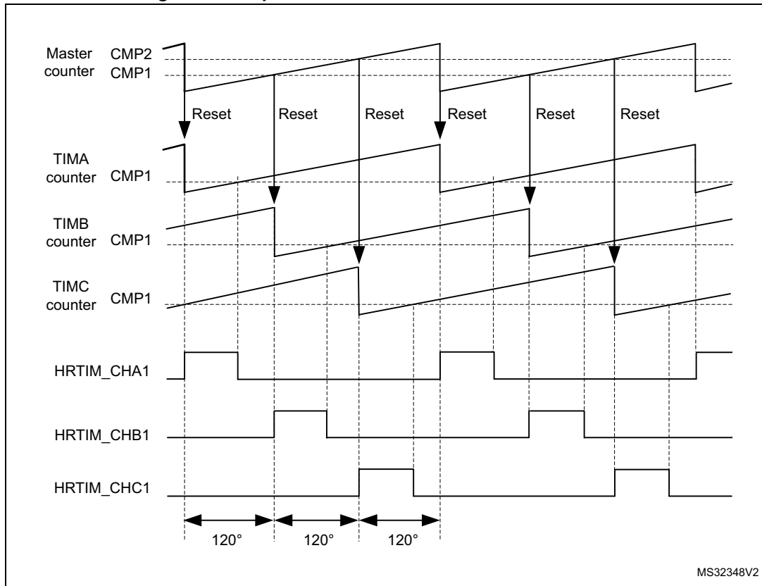
Figure 383. 3-phase interleaved buck converter control
