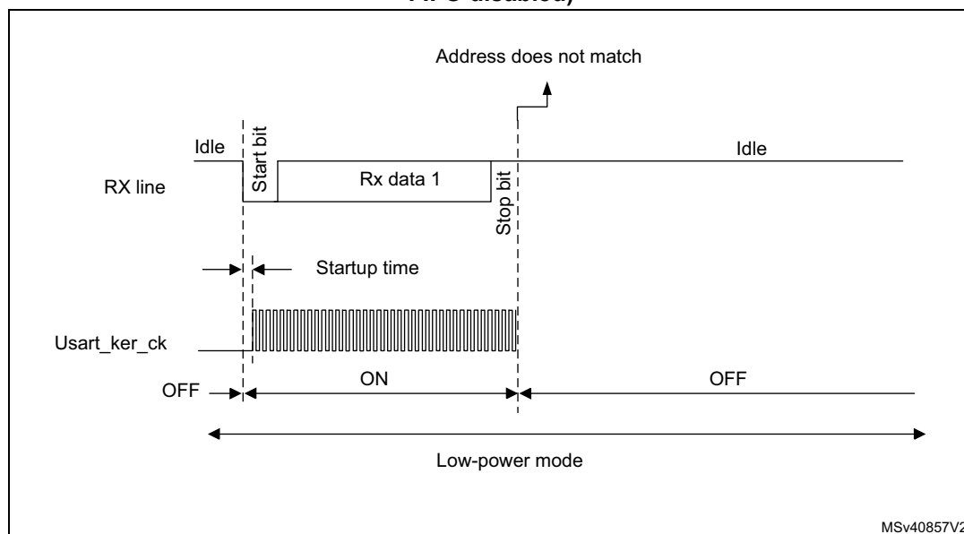
Figure 637. Wakeup event not verified (wakeup event = address match, FIFO disabled)
