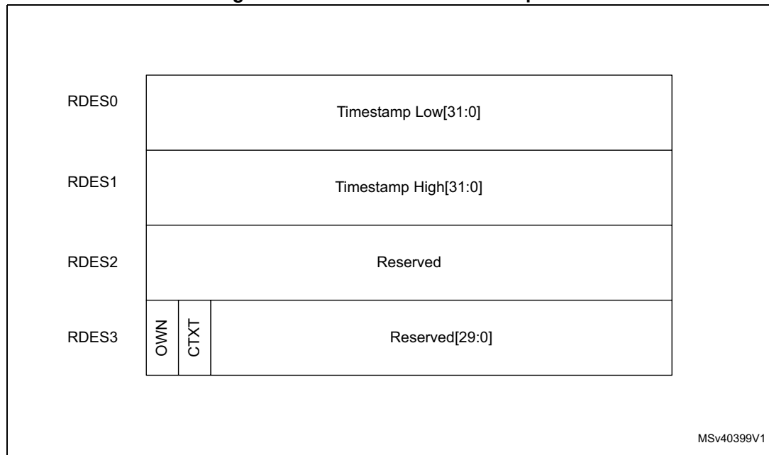
Figure 847. Receive context descriptor
