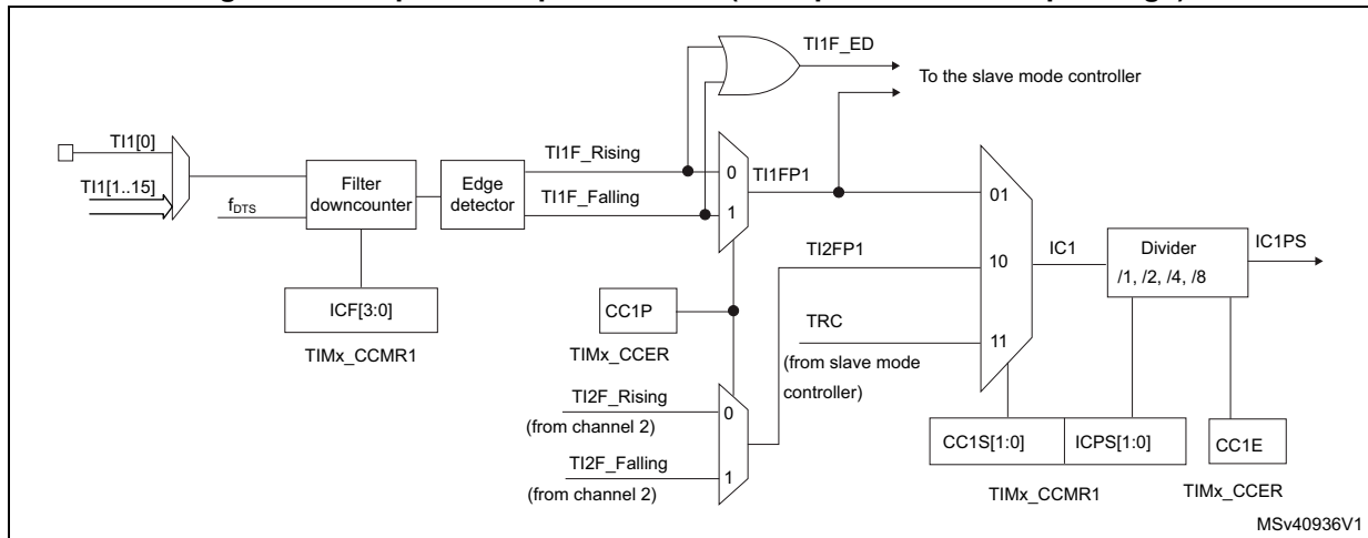
Figure 535. Capture/compare channel (example: channel 1 input stage)
