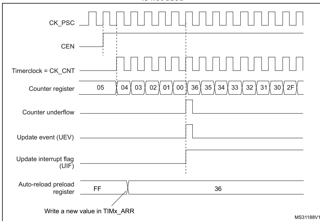
Figure 459. Counter timing diagram, Update event when repetition counter is not used
