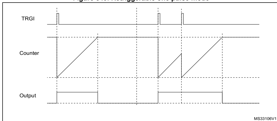
Figure 549. Retriggerable one pulse mode
