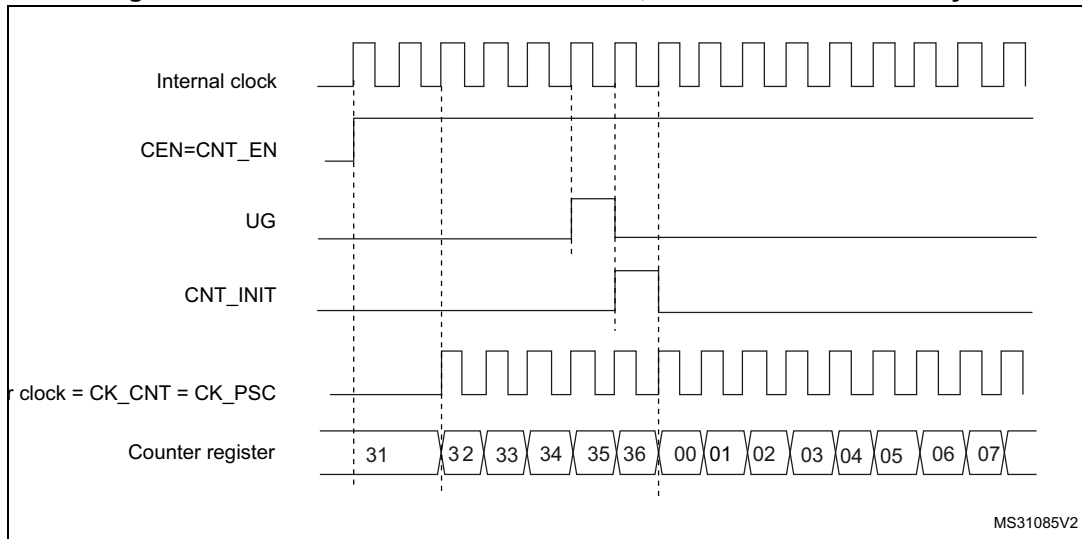
Figure 505. Control circuit in normal mode, internal clock divided by 1
