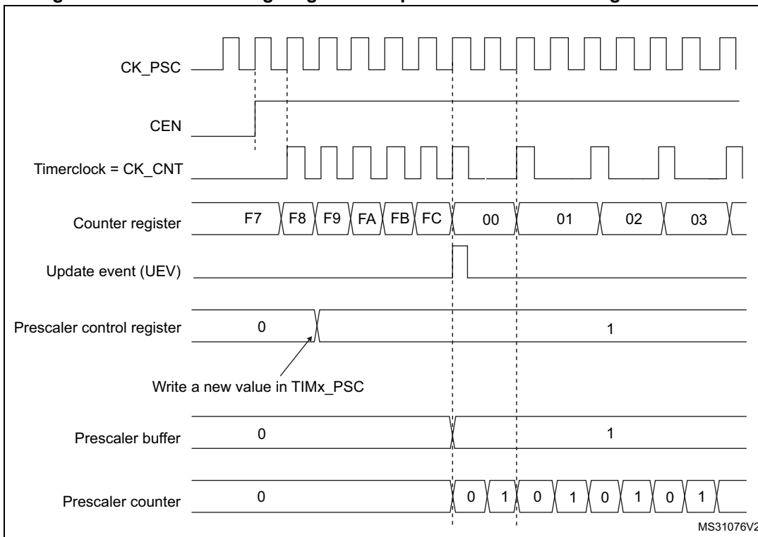
Figure 497. Counter timing diagram with prescaler division change from 1 to 2
