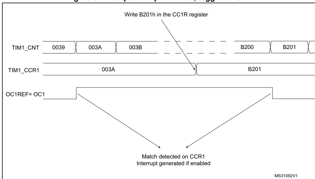
Figure 512. Output compare mode, toggle on OC1.
