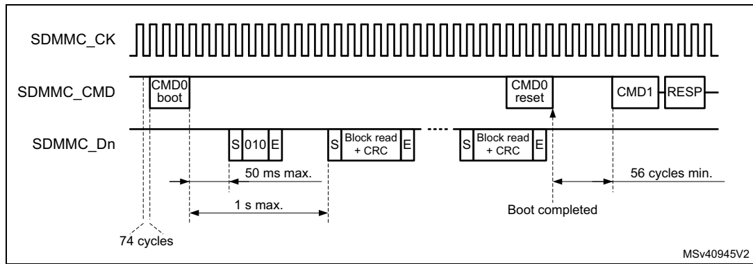
Figure 767. Alternative boot mode operation
