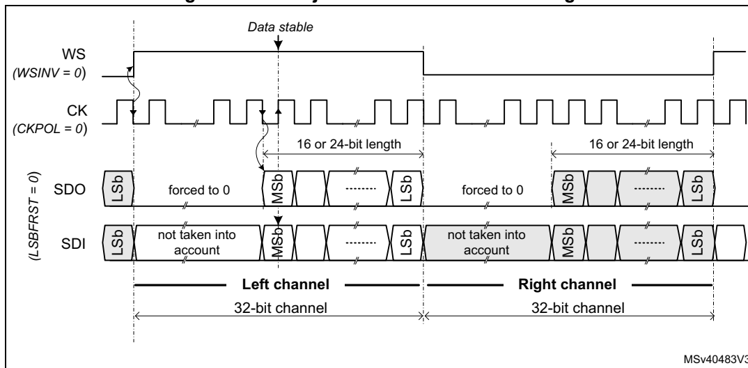
Figure 673. LSB justified 16 or 24-bit data length
