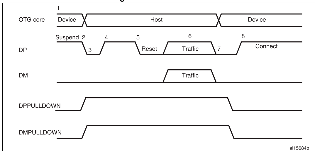
Figure 818. B-device HNP
