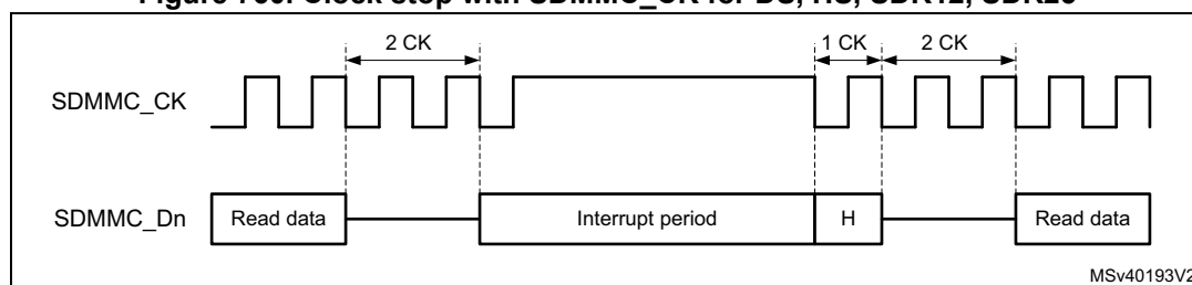
Figure 760. Clock stop with SDMMC_CK for DS, HS, SDR12, SDR25
