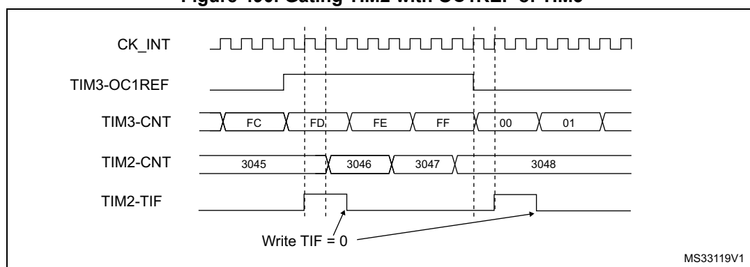
Figure 490. Gating TIM2 with OC1REF of TIM3
