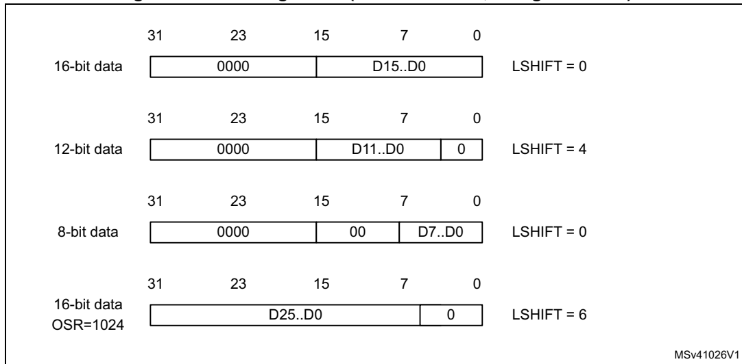
Figure 174. Left alignment (offset enabled, signed value)
