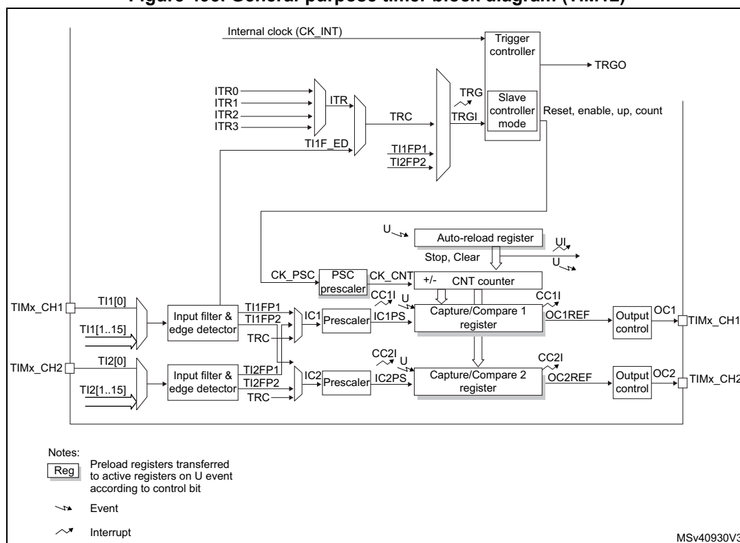
Figure 495. General-purpose timer block diagram (TIM12)
