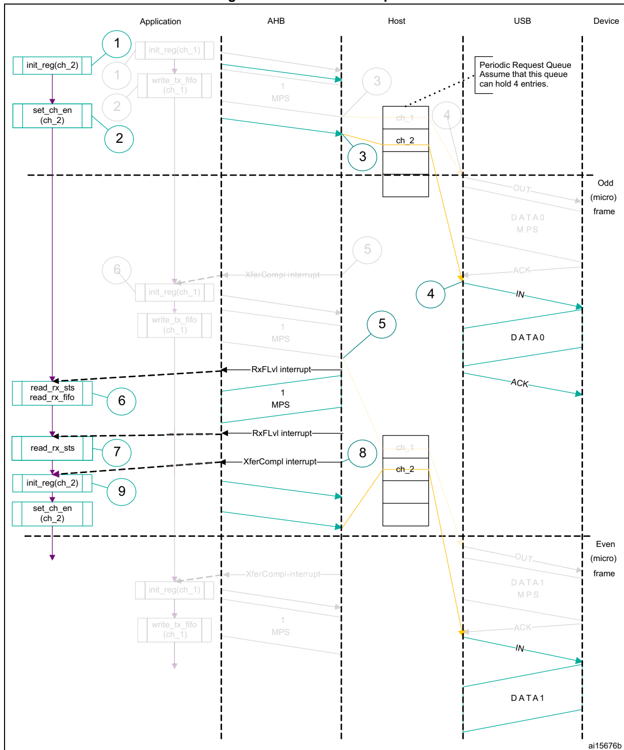
Figure 802. Normal interrupt IN
