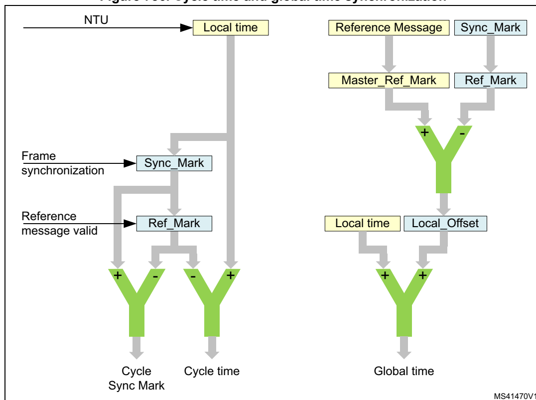
Figure 786. Cycle time and global time synchronization
