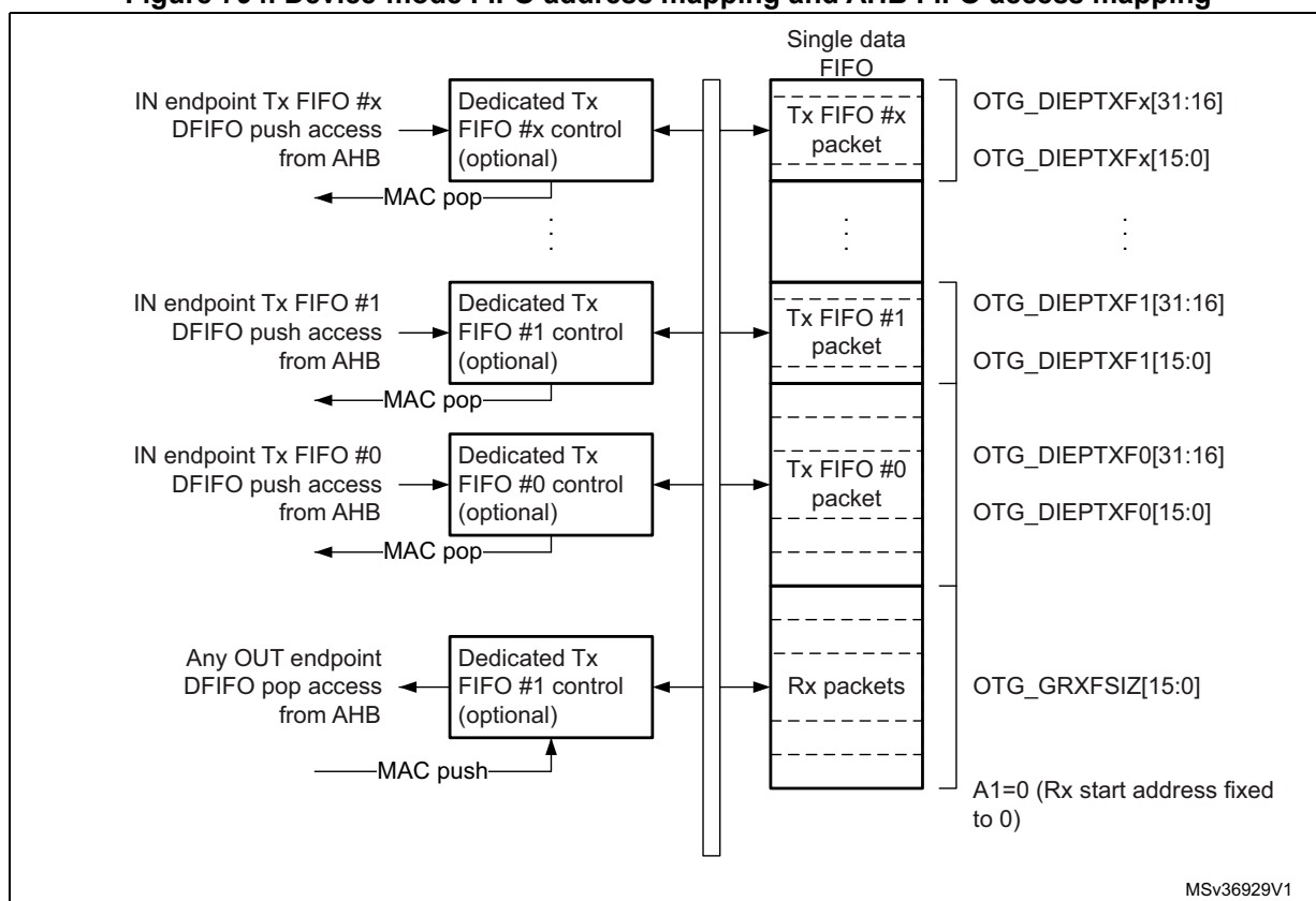
Figure 794. Device-mode FIFO address mapping and AHB FIFO access mapping
