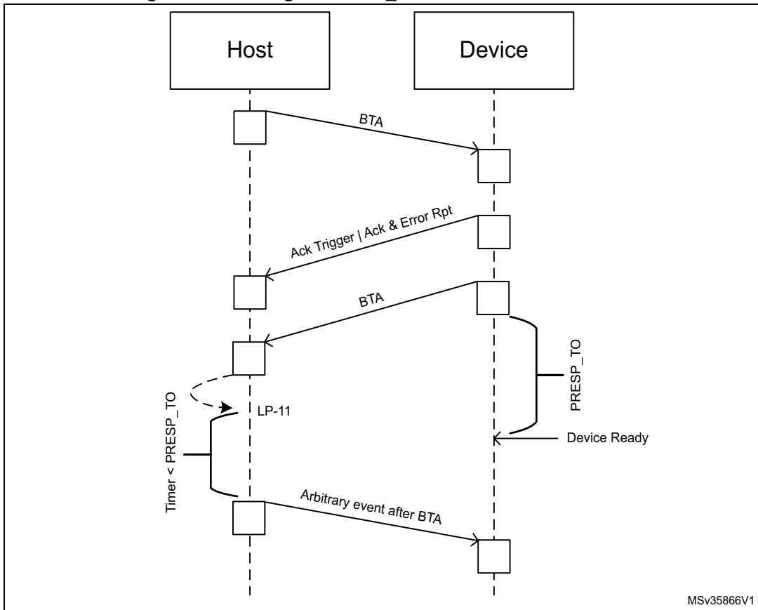
Figure 266. Timing of PRESP_TO after a bus-turn-around
