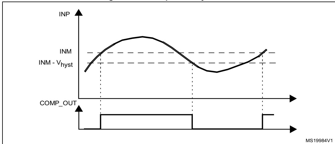
Figure 222. Comparator hysteresis
