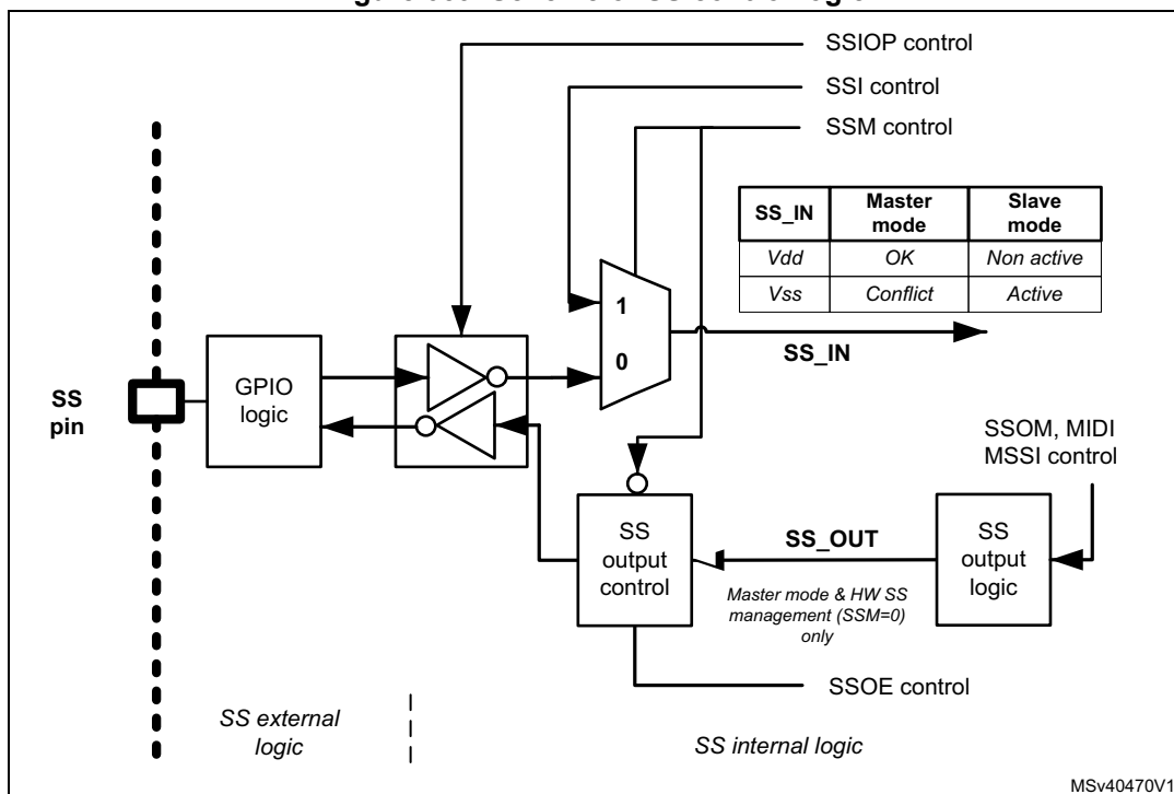
Figure 659. Scheme of SS control logic
