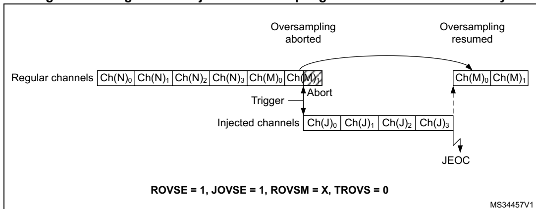
Figure 190. Regular and injected oversampling modes used simultaneously
