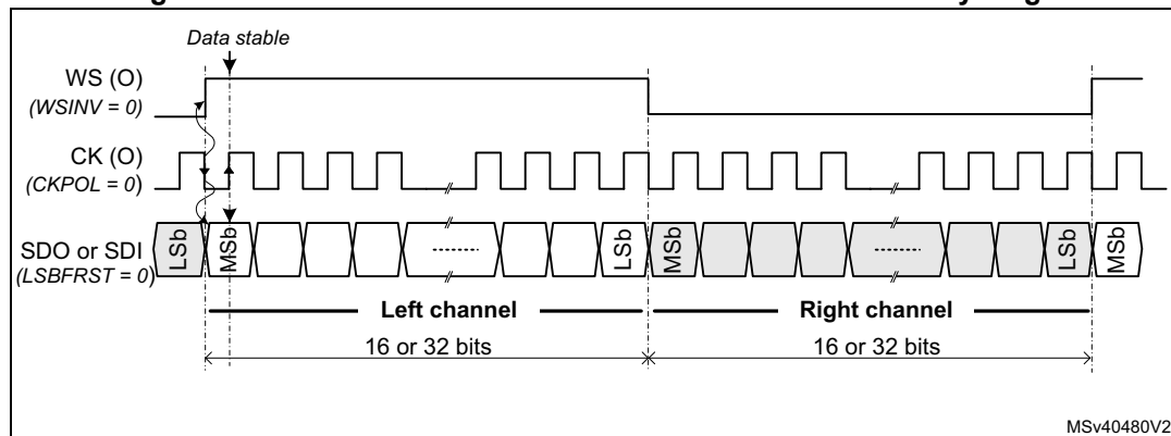
Figure 670. Master MSB Justified 16-bit or 32-bit full-accuracy length
