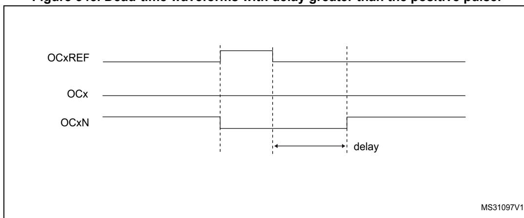
Figure 545. Dead-time waveforms with delay greater than the positive pulse.
