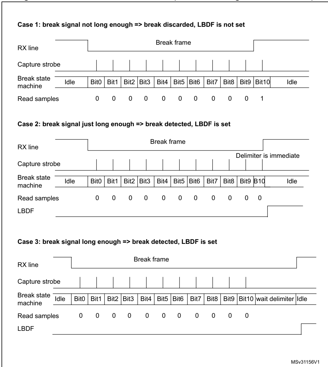
Figure 621. Break detection in LIN mode (11-bit break length - LBDL bit is set)
