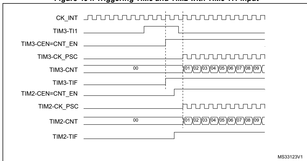
Figure 494. Triggering TIM3 and TIM2 with TIM3 TI1 input
