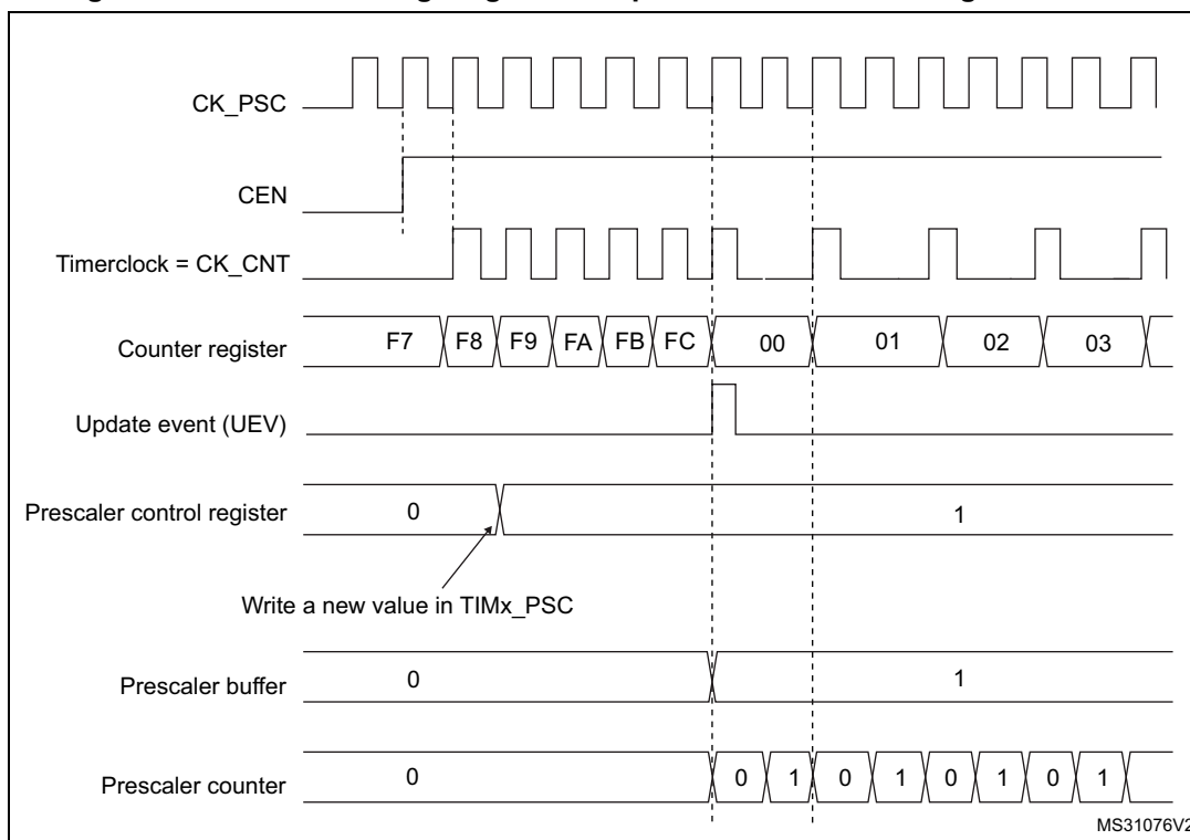
Figure 447. Counter timing diagram with prescaler division change from 1 to 2
