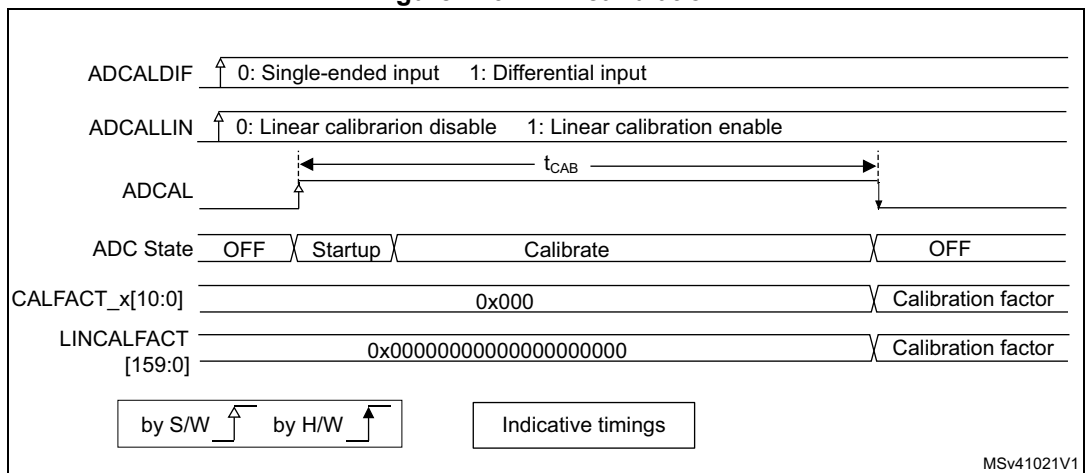
Figure 146. ADC calibration
