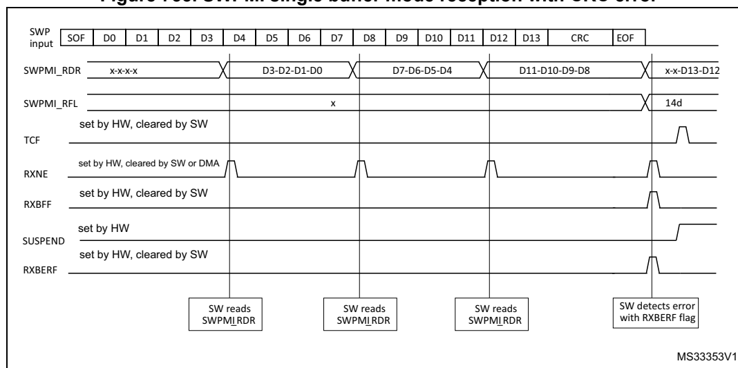
Figure 735. SWPMI single buffer mode reception with CRC error
