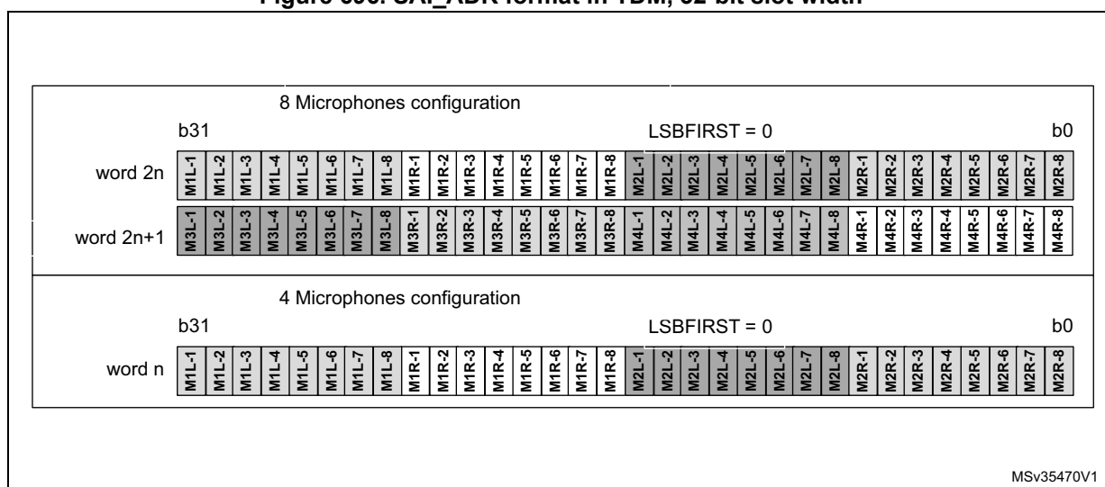
Figure 696. SAI_ADR format in TDM, 32-bit slot width
