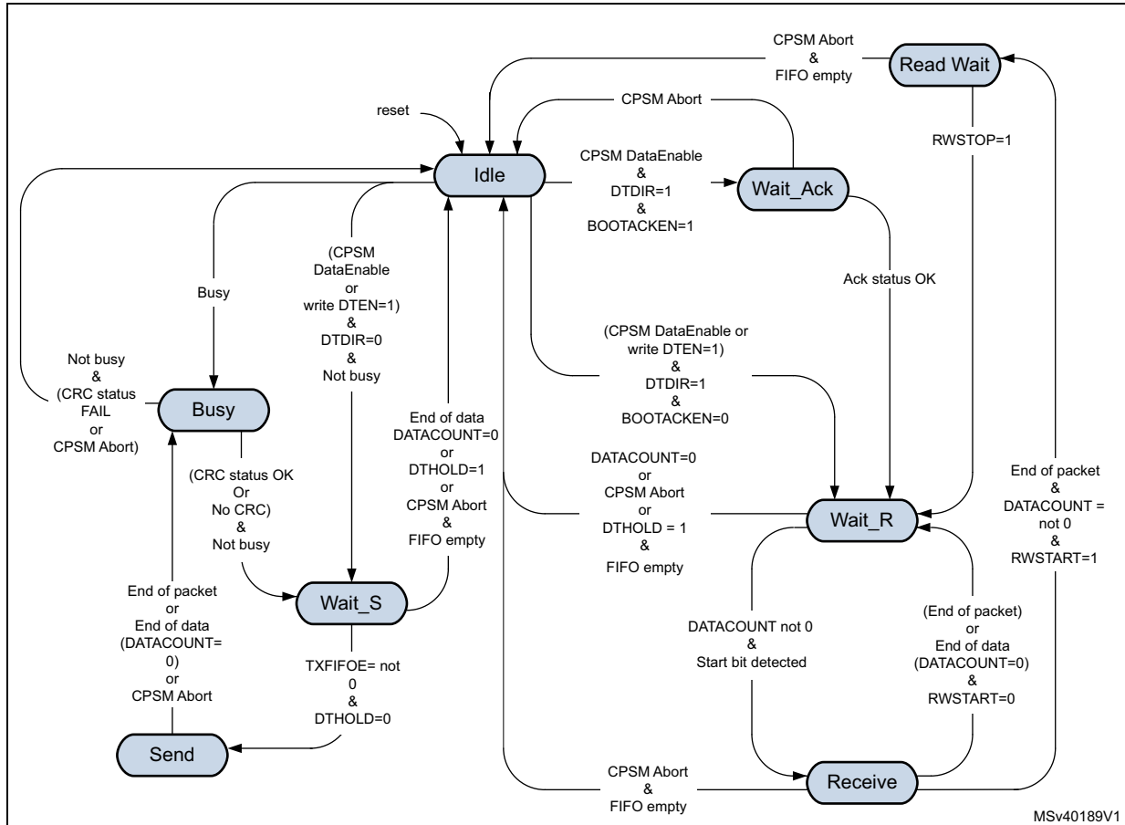
Figure 752. Data path state machine (DPSM)
