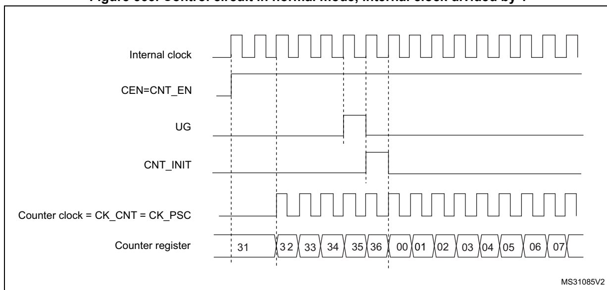
Figure 563. Control circuit in normal mode, internal clock divided by 1
