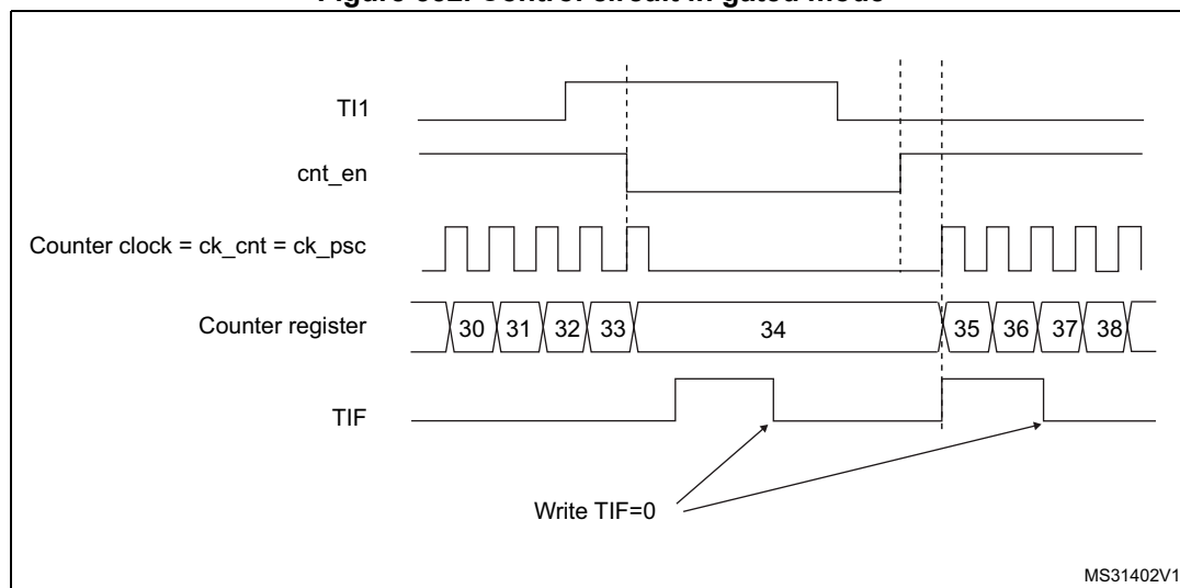
Figure 552. Control circuit in gated mode
