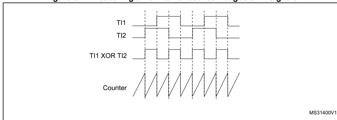
Figure 517. Measuring time interval between edges on 2 signals
