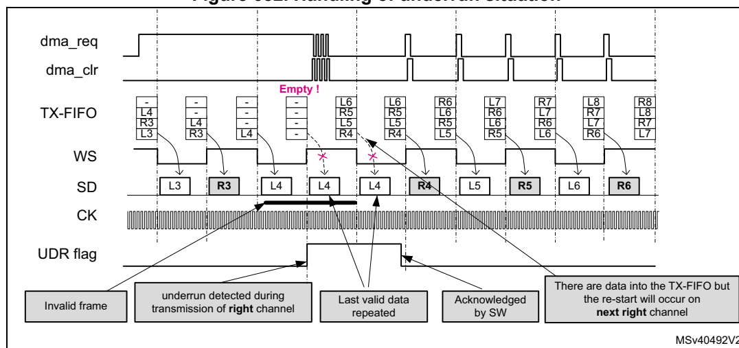
Figure 682. Handling of underrun situation
