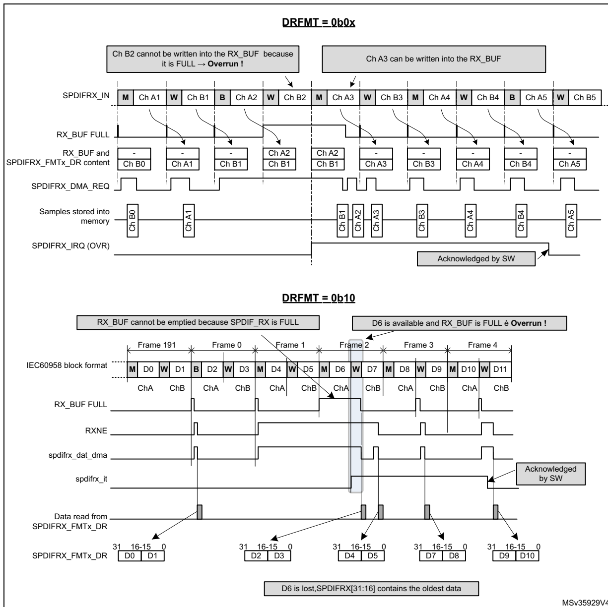
Figure 721. S/PDIF overrun error when RXSTEO = 0
