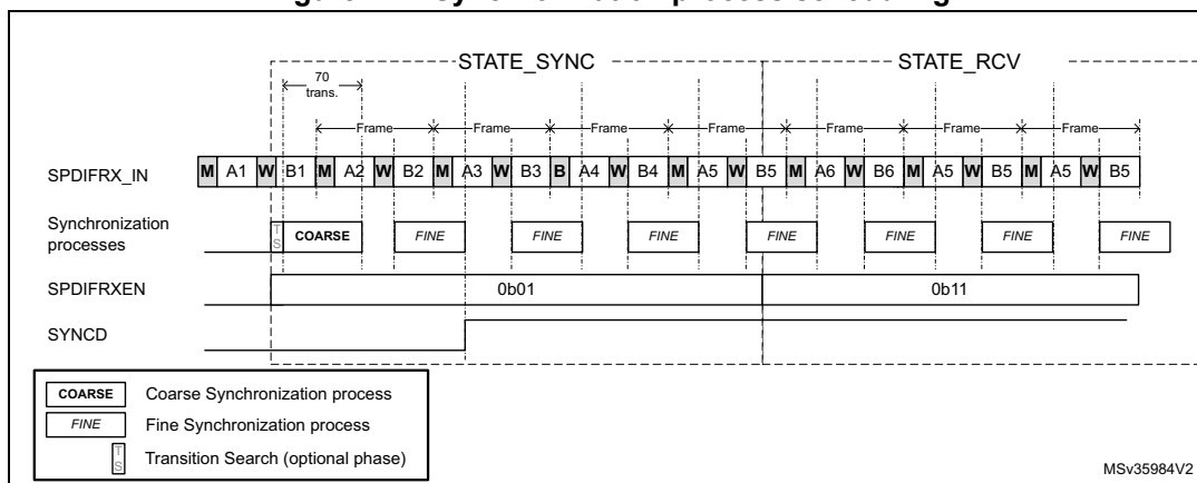
Figure 717. Synchronization process scheduling
