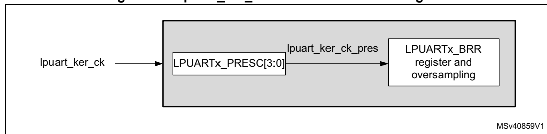
Figure 642. lpuart_ker_ck clock divider block diagram
