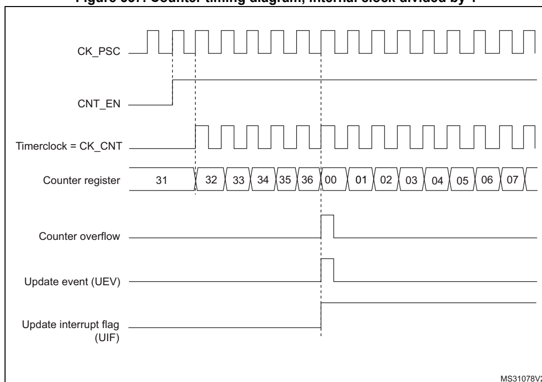
Figure 557. Counter timing diagram, internal clock divided by 1
