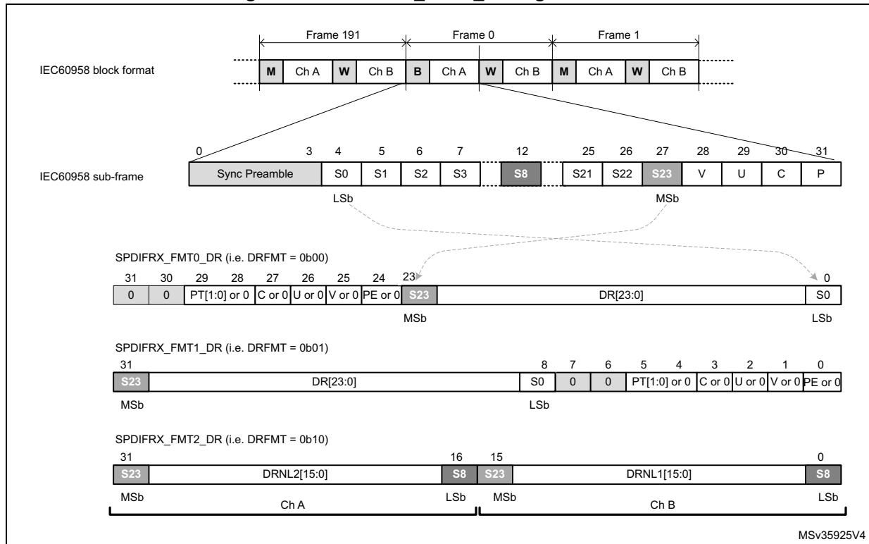
Figure 719. SPDIFRX_FMTx_DR register format
