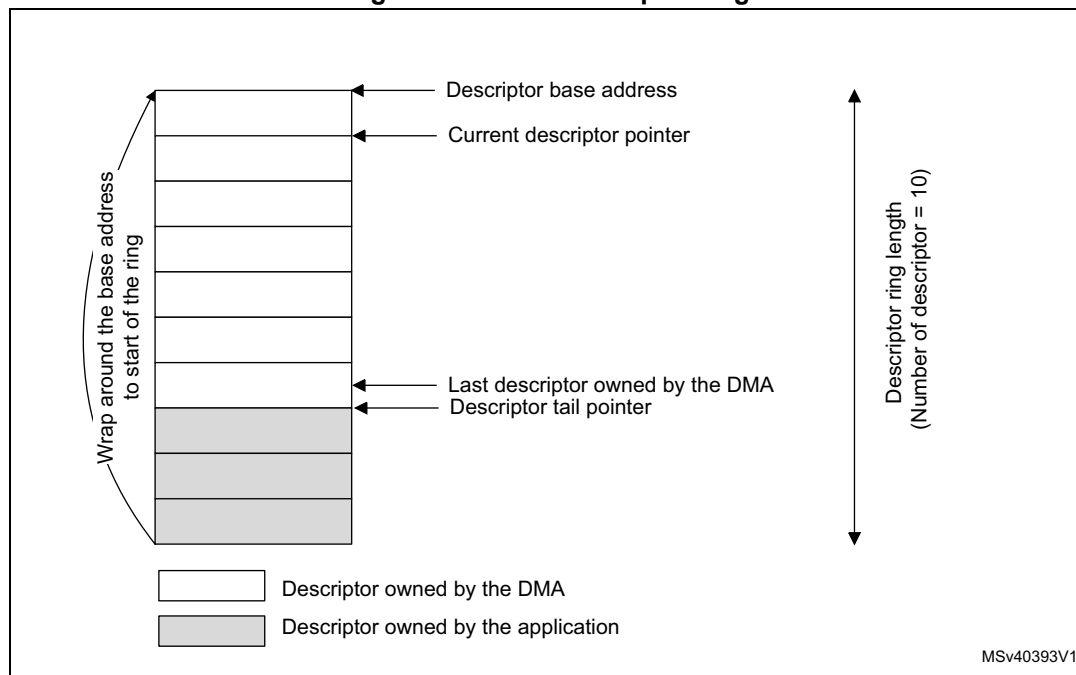
Figure 841. DMA descriptor ring
