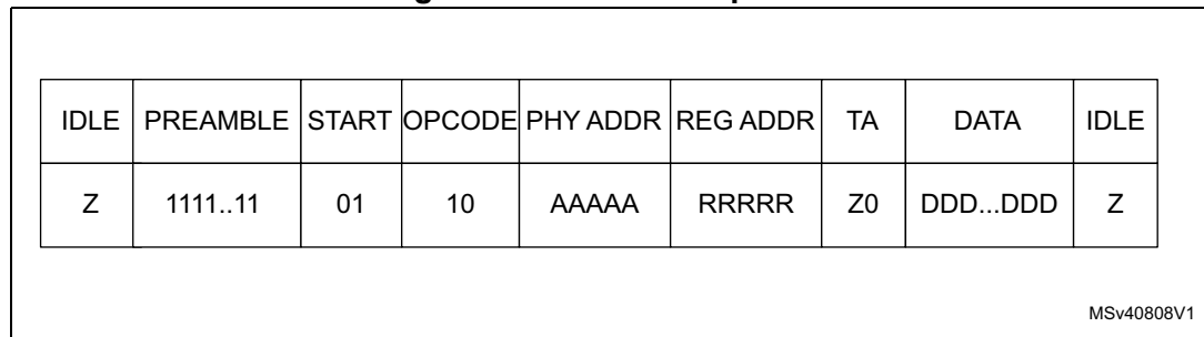
Figure 835. Read data packet
