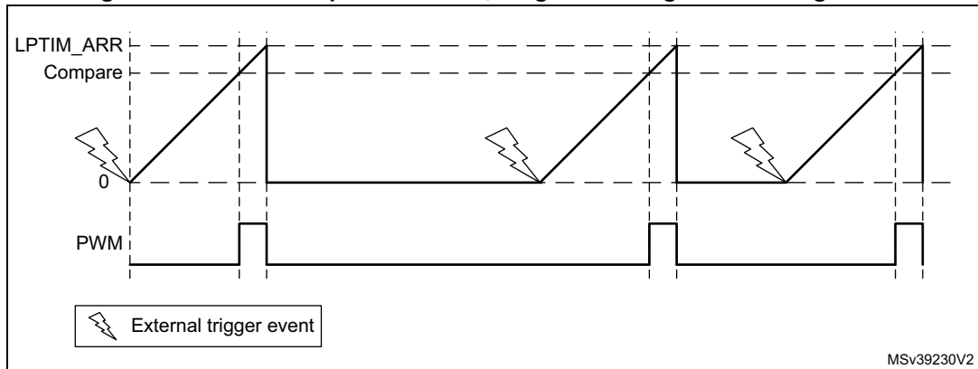
Figure 568. LPTIM output waveform, single counting mode configuration
