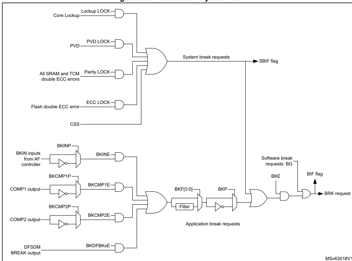
Figure 546. Break circuitry overview
