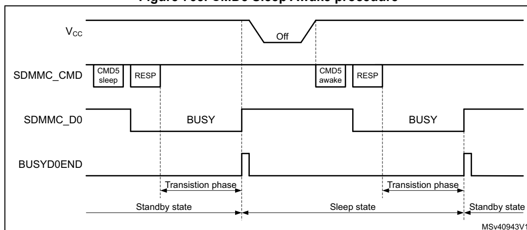
Figure 765. CMD5 Sleep Awake procedure
