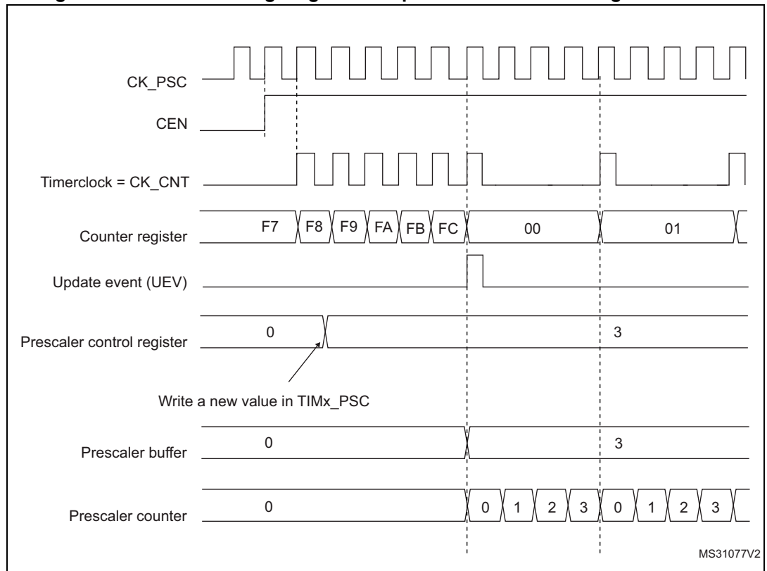
Figure 556. Counter timing diagram with prescaler division change from 1 to 4
