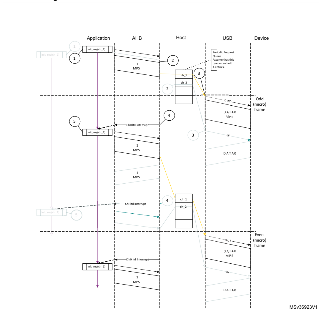
Figure 809. Normal isochronous OUT transaction - DMA mode
