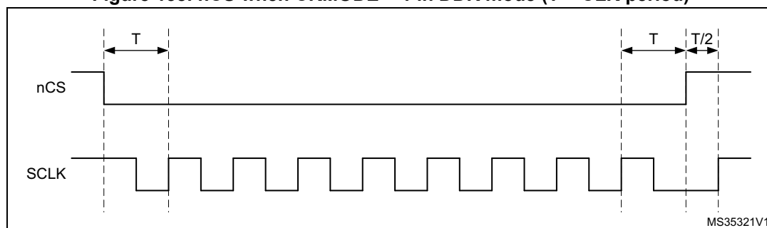
Figure 138. nCS when CKMODE = 1 in DDR mode (T = CLK period)
