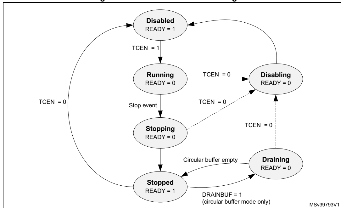
Figure 870. ETF state transition diagram
