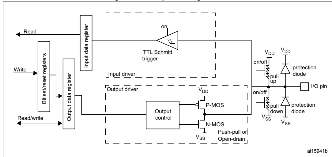
Figure 79. Output configuration
