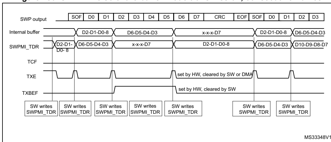
Figure 730. SWPMI No software buffer mode transmission, consecutive frames
