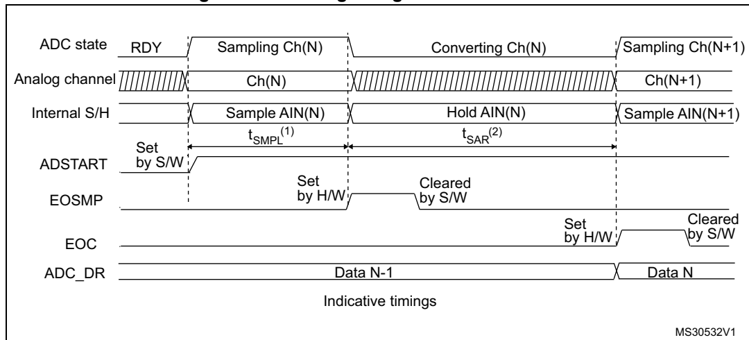
Figure 150. Analog to digital conversion time
