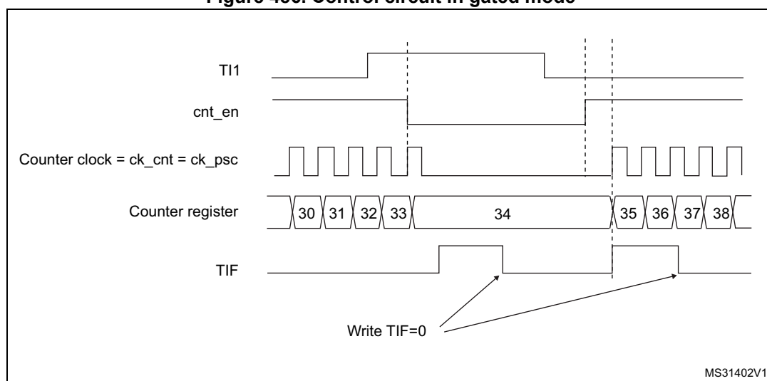
Figure 486. Control circuit in gated mode
