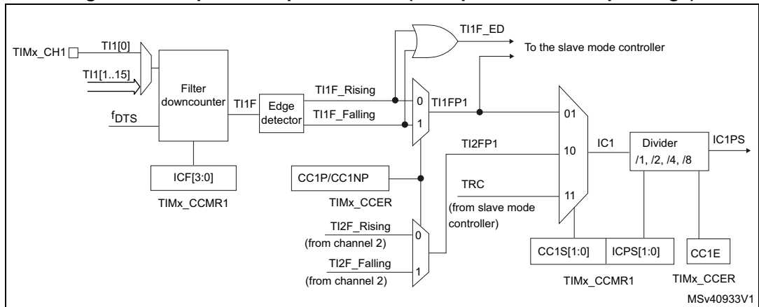
Figure 508. Capture/compare channel (example: channel 1 input stage)
