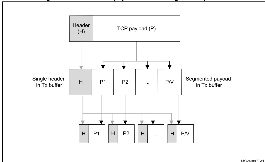
Figure 830. Header and payload fields of segmented packets
