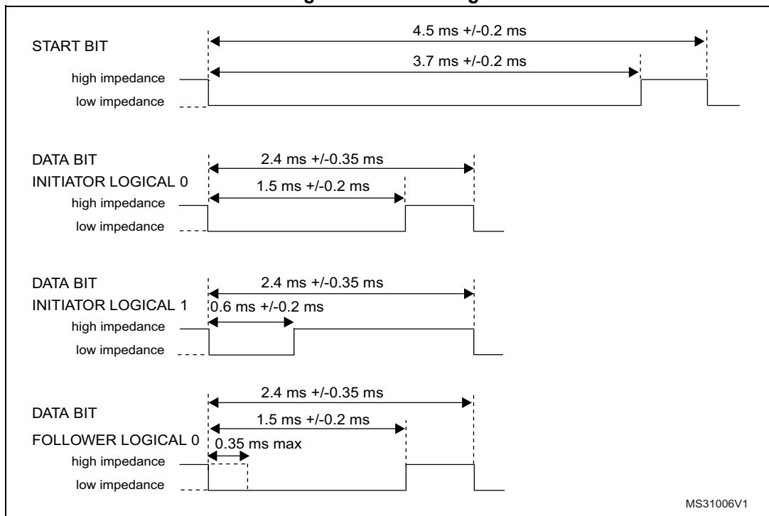
Figure 852. Bit timings
