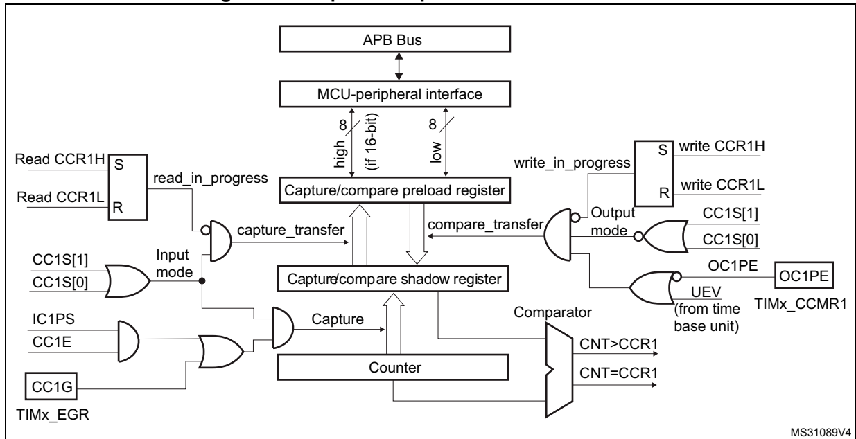
Figure 509. Capture/compare channel 1 main circuit
