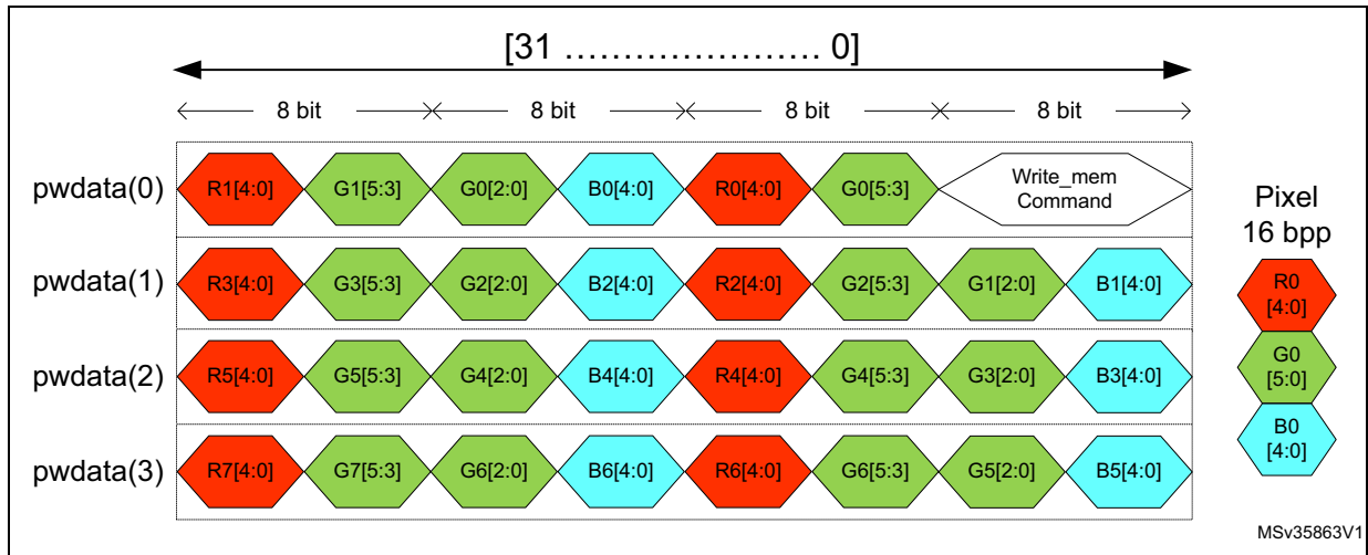
Figure 263. 16 bpp APB pixel to byte organization
