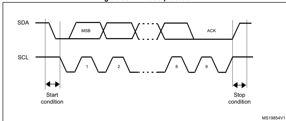
Figure 581. I 2 C bus protocol
