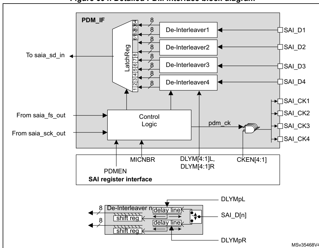
Figure 694. Detailed PDM interface block diagram
