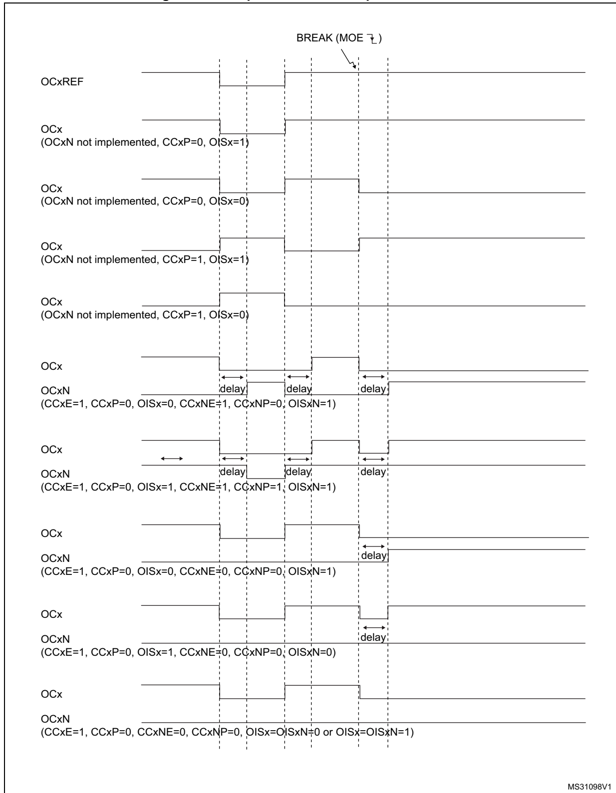
Figure 547. Output behavior in response to a break
