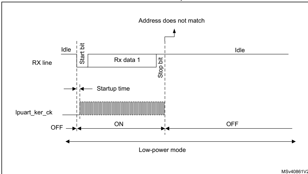
Figure 651. Wakeup event not verified (wakeup event = address match, FIFO disabled)
