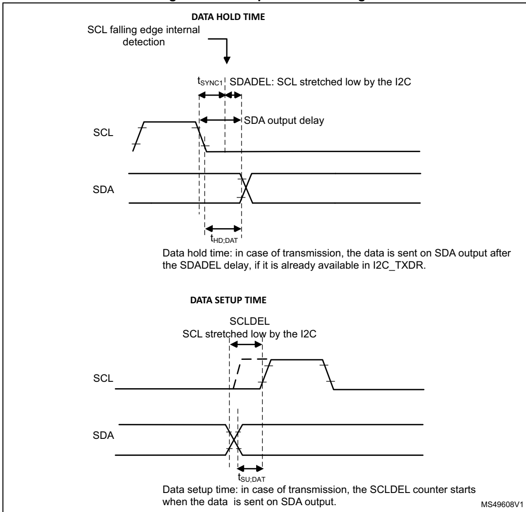
Figure 582. Setup and hold timings
