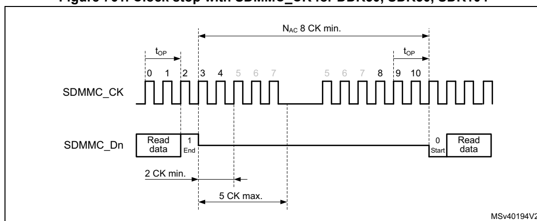
Figure 761. Clock stop with SDMMC_CK for DDR50, SDR50, SDR104
