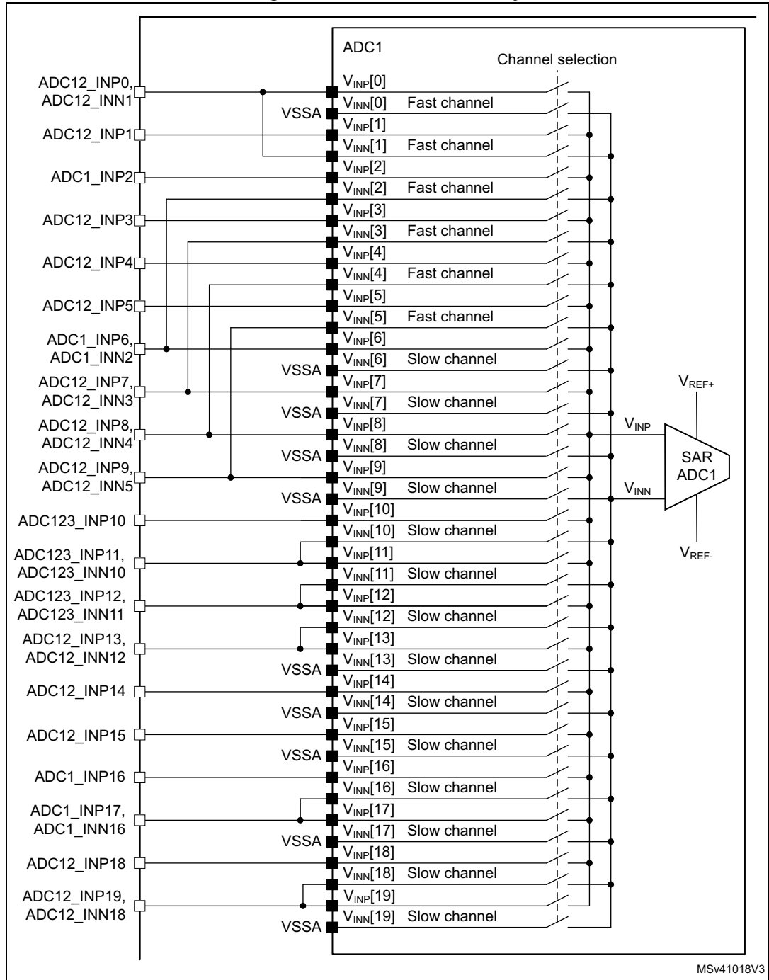
Figure 143. ADC1 connectivity
