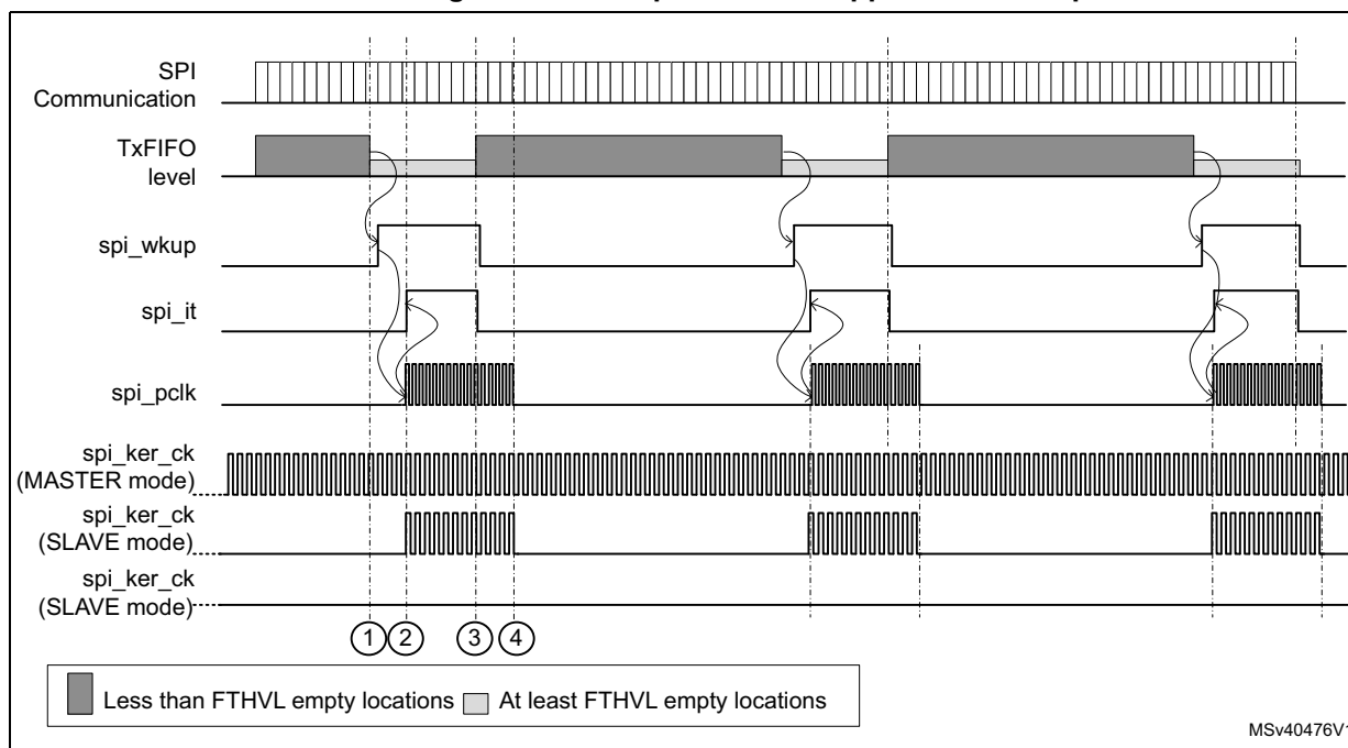
Figure 666. Low-power mode application example
