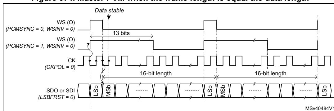
Figure 674. Master PCM when the frame length is equal the data length
