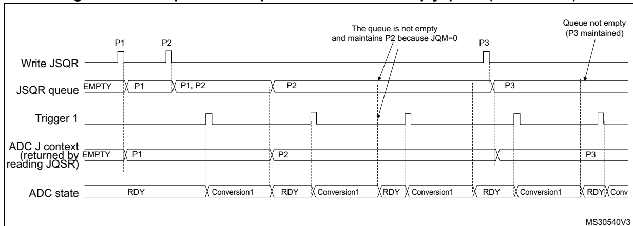
Figure 159. Example of JSQR queue of context with empty queue (case JQM=0)
