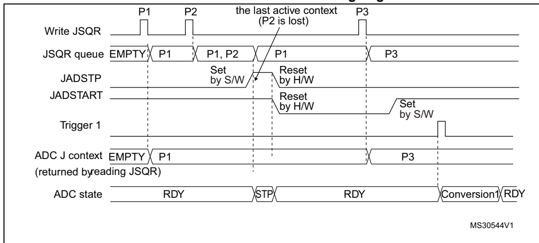
Figure 163. Flushing JSQR queue of context by setting JADSTP=1 (JQM=0). Case when JADSTP occurs outside an ongoing conversion
