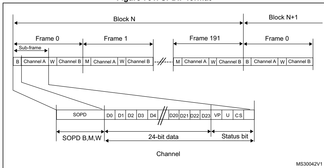
Figure 701. SPDIF format
