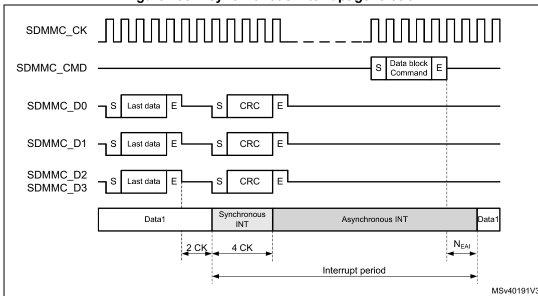
Figure 755. Asynchronous interrupt generation
