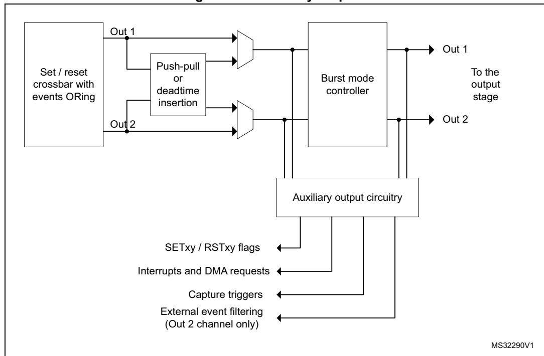
Figure 369. Auxiliary outputs
