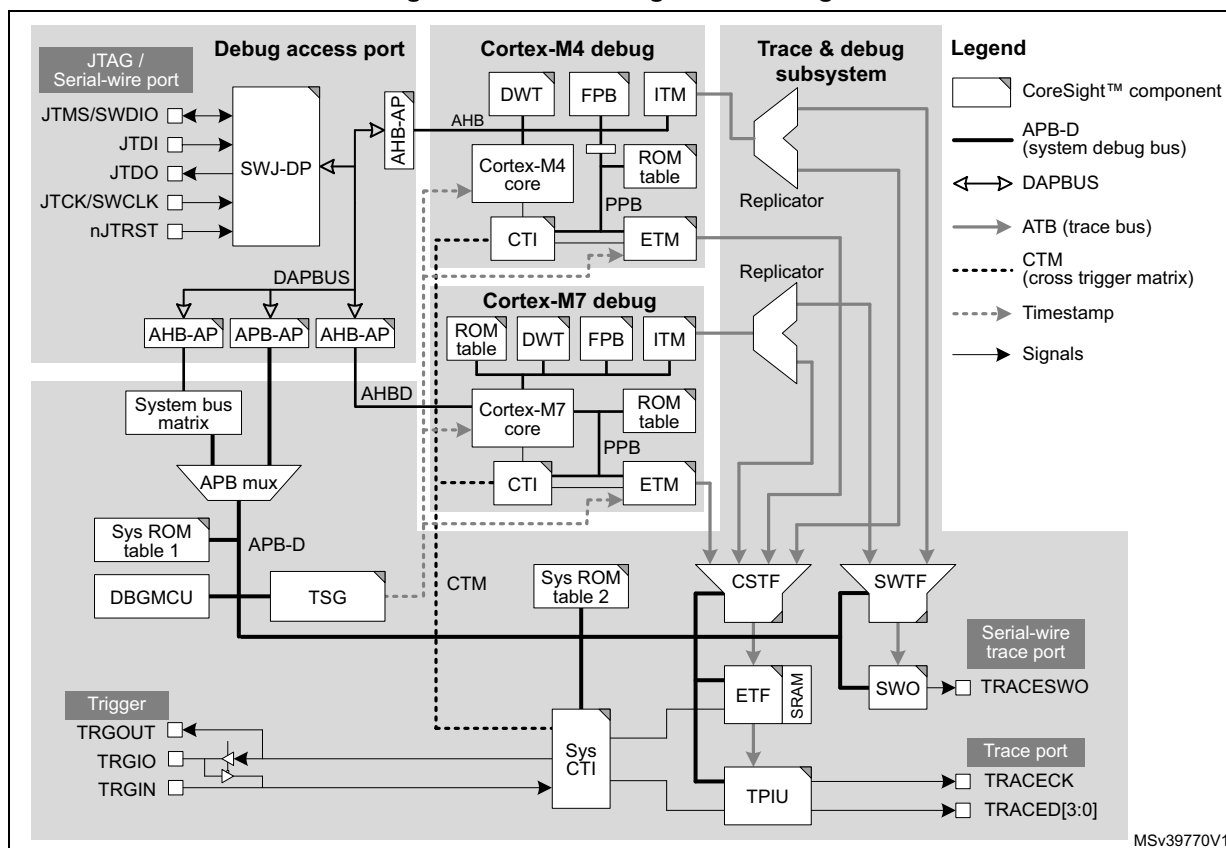
Figure 859. Block diagram of debug infrastructure
