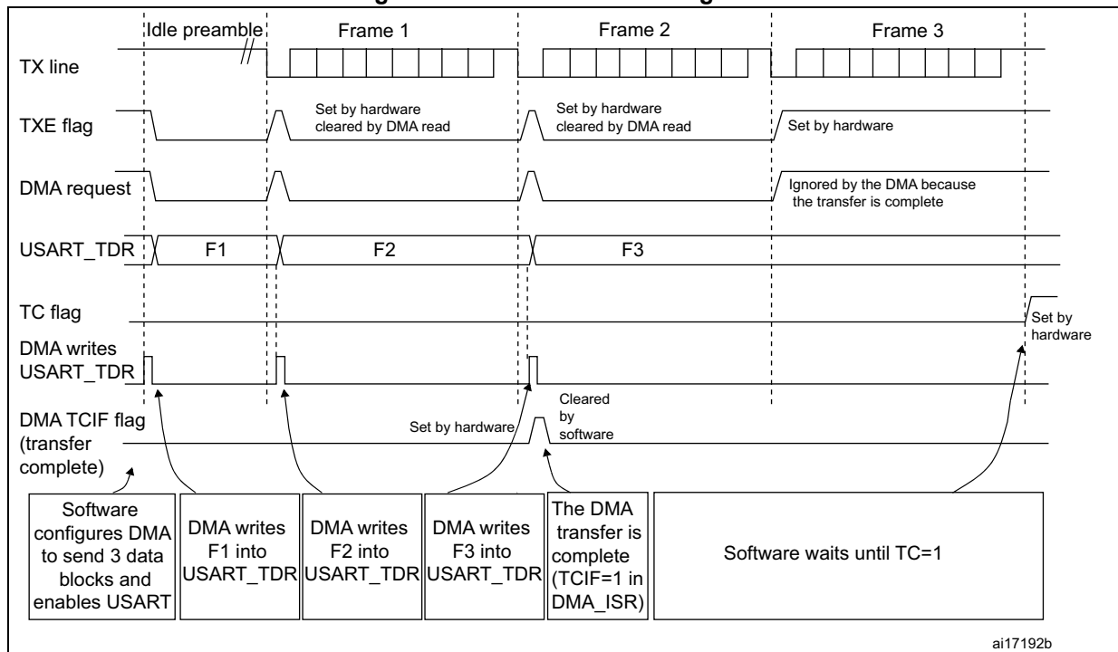
Figure 645. Transmission using DMA
