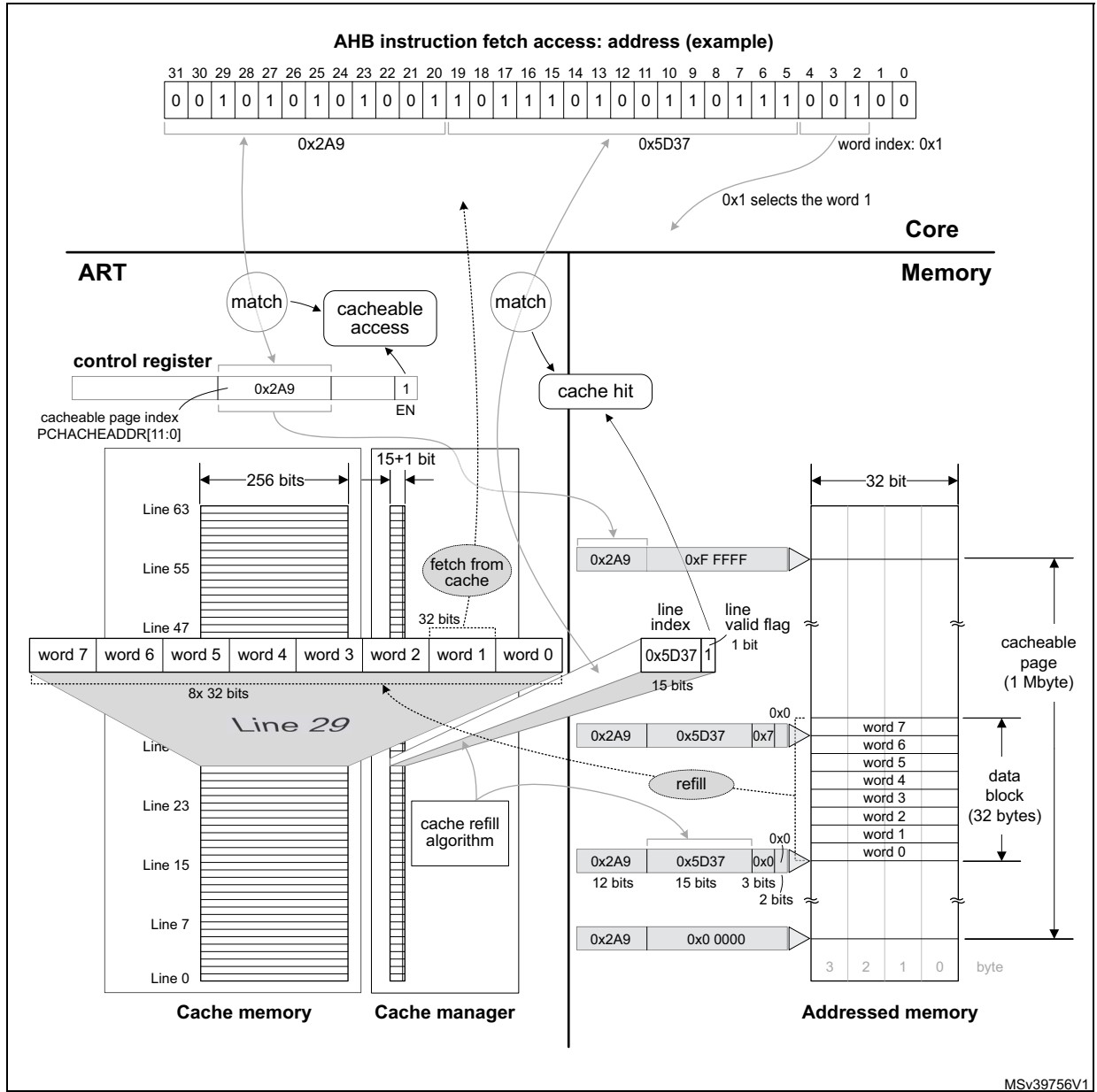
Figure 19. Instruction fetch from cache
