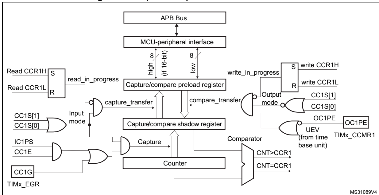
Figure 415. Capture/compare channel 1 main circuit
