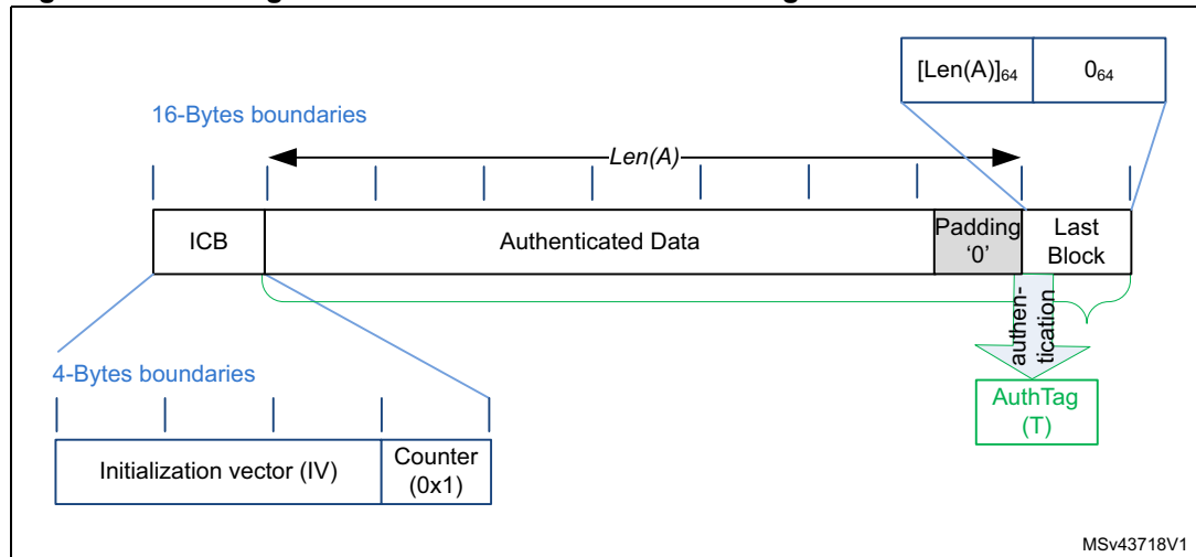
Figure 316. Message construction for the Galois Message Authentication Code mode
