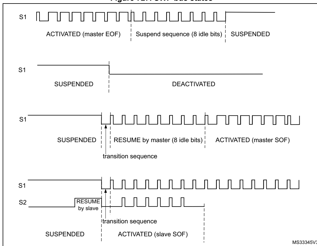
Figure 727. SWP bus states
