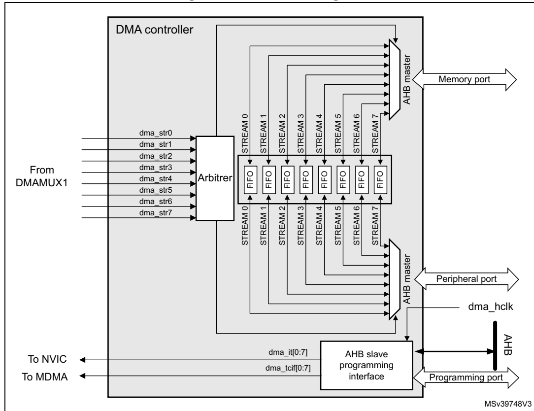
Figure 84. DMA block diagram
