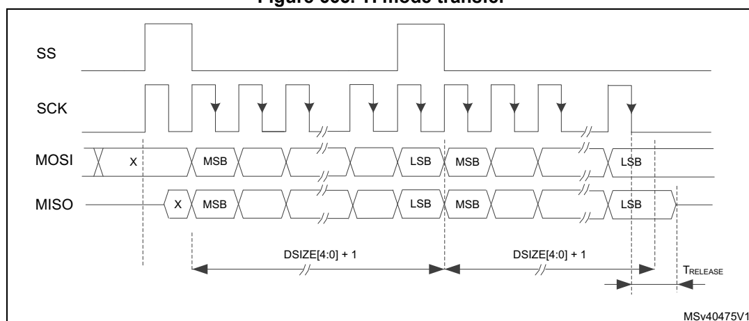
Figure 665. TI mode transfer
