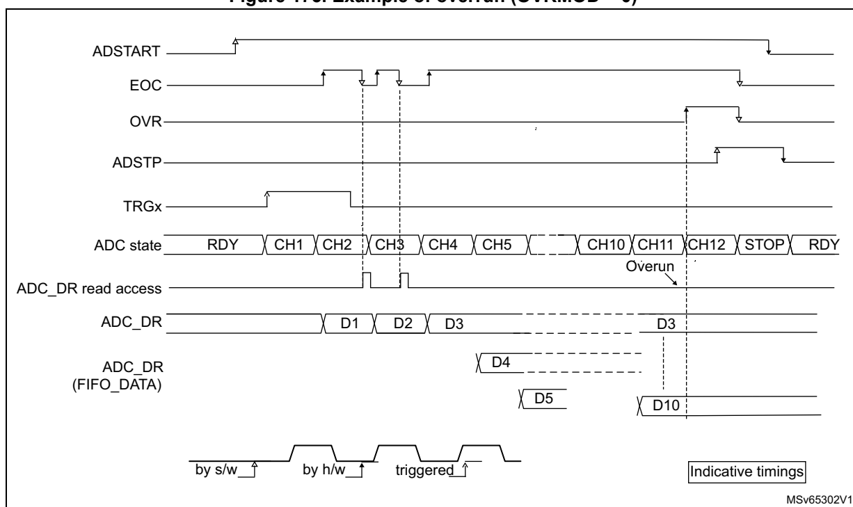
Figure 175. Example of overrun (OVRMOD = 0)
