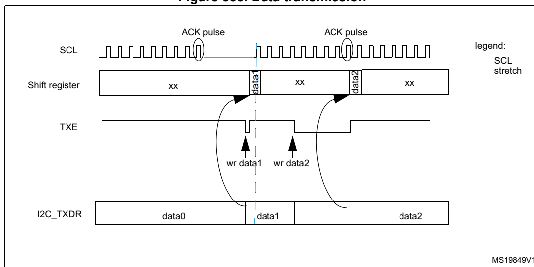
Figure 585. Data transmission
