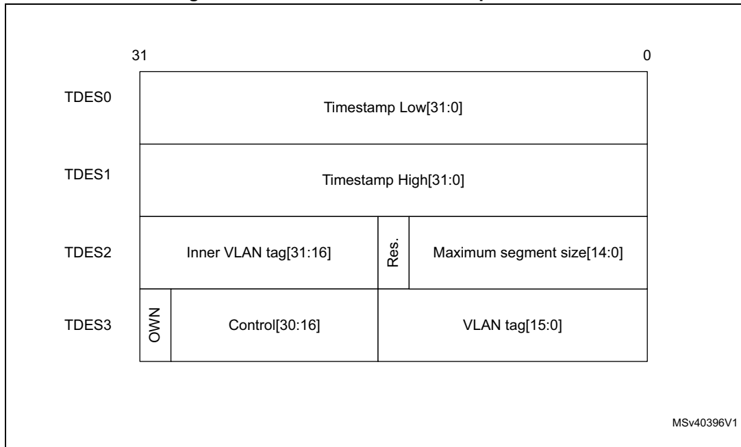
Figure 844. Transmit context descriptor format
