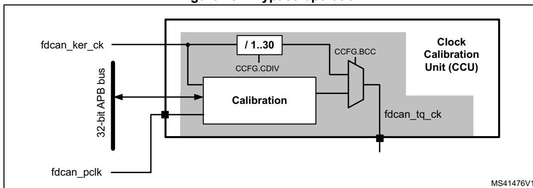
Figure 784. Bypass operation
