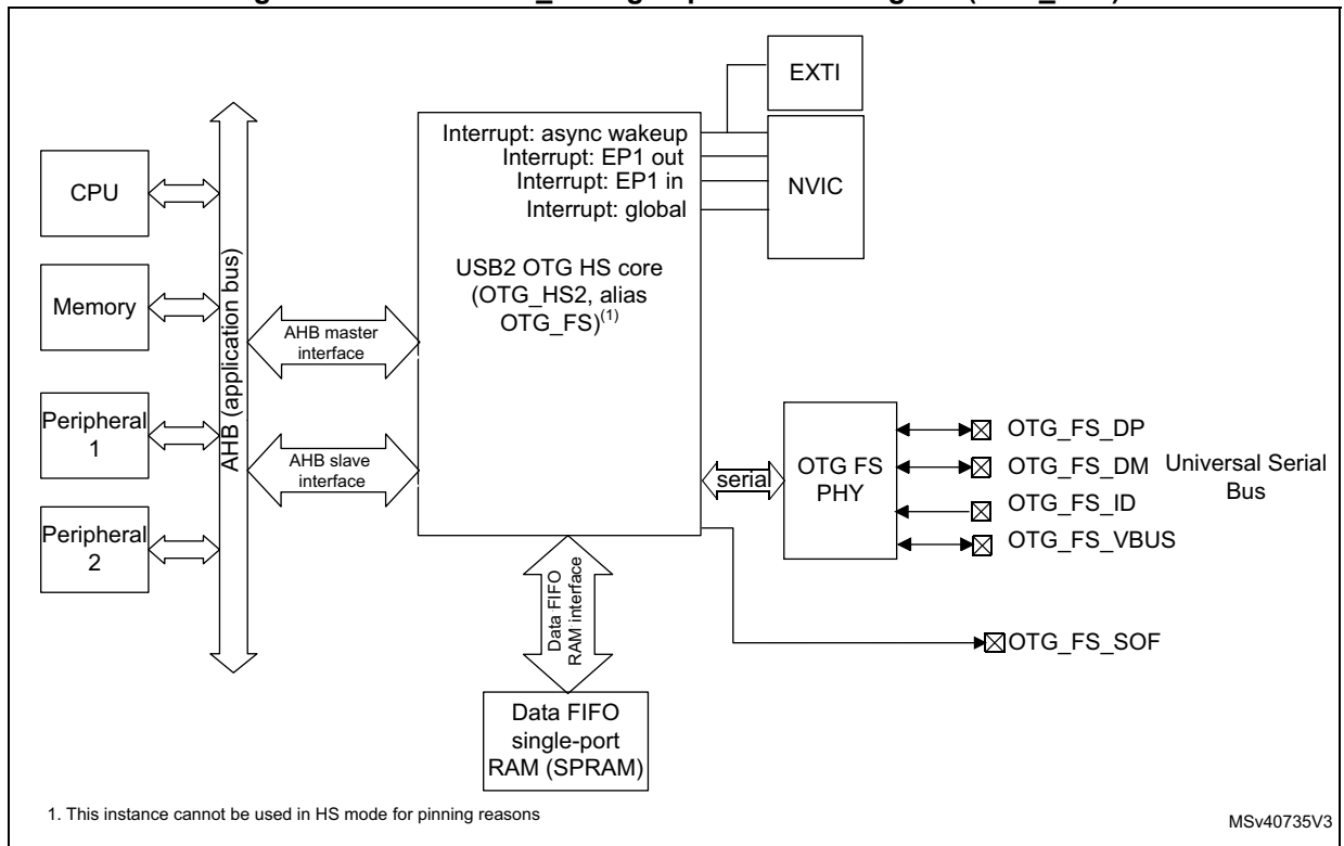
Figure 791. USB2 OTG_HS high-speed block diagram (OTG_HS2)
