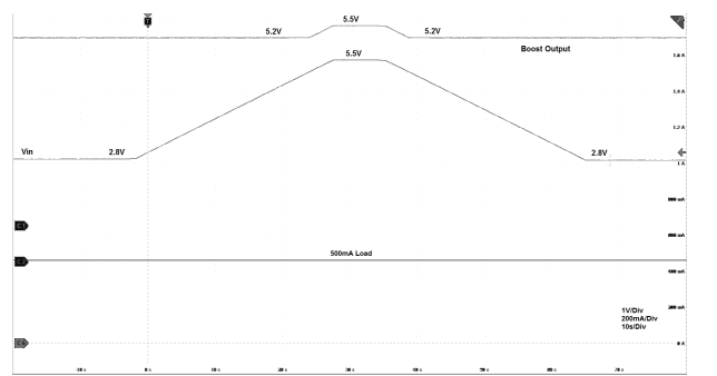
Figure 24. Boost output vs. input voltage
