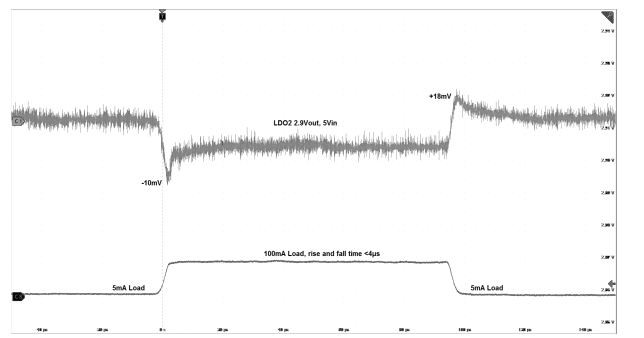
Figure 18. LDO2 load transient
