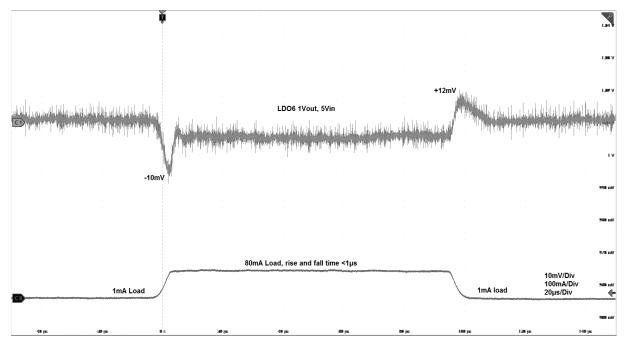
Figure 22. LDO6 load transient
