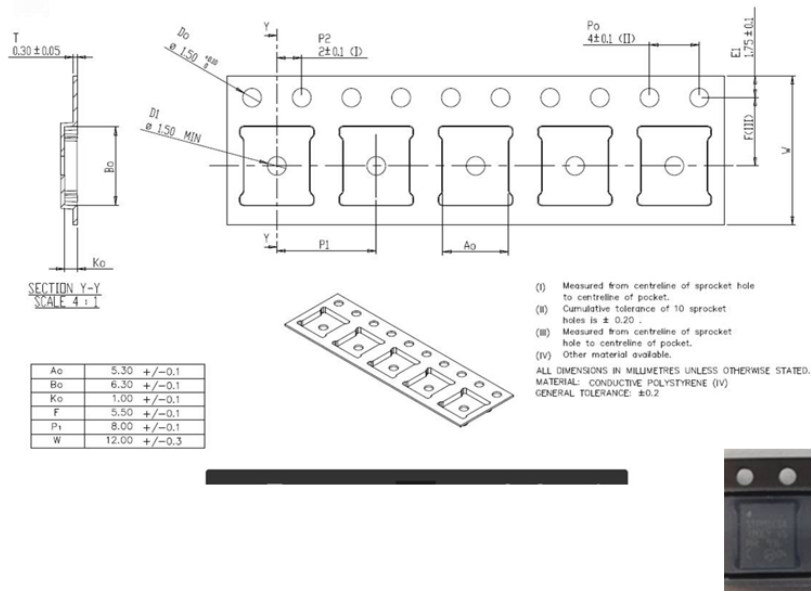
Figure 67. Reel outline
