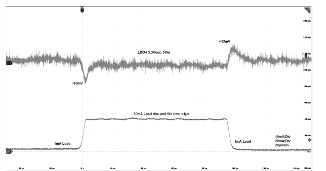
Figure 20. LDO4 load transient
