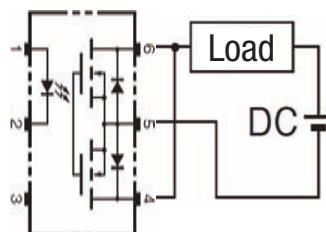
DIP/SOP 6-pin package
