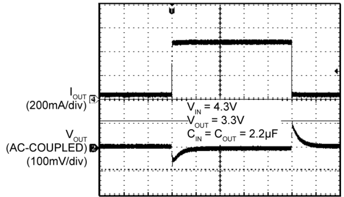
Time (20 \mu s/div)
