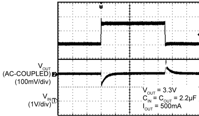
Time (20 \mu s/div)
