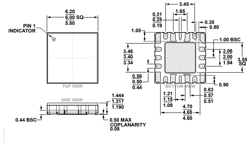
Figure 36. 16-Terminal Ceramic Leadless Chip with Heat Sink [LCC_HS] (EP-16-2) Dimensions shown in millimeters
