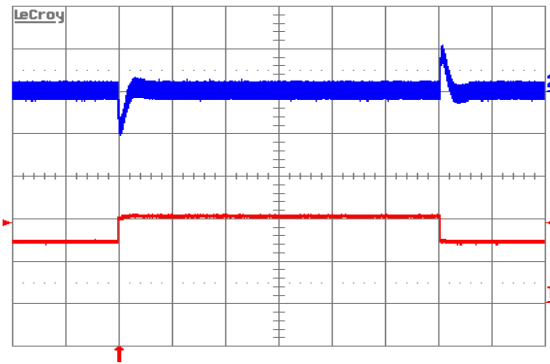
Figure 9. Output voltage response to load current step-change (6.5 A–9.75 A–6.5 A) at V_{in} = 48\text{ V} . Top trace: output voltage (100 mV/div.). Bottom trace: load current (5A/div.). Current slew rate: 5 A/ \mu\text{s} . C_o = 470\mu\text{F} POS + 1 \mu\text{F} ceramic. Time scale: 0.2 ms/div.
