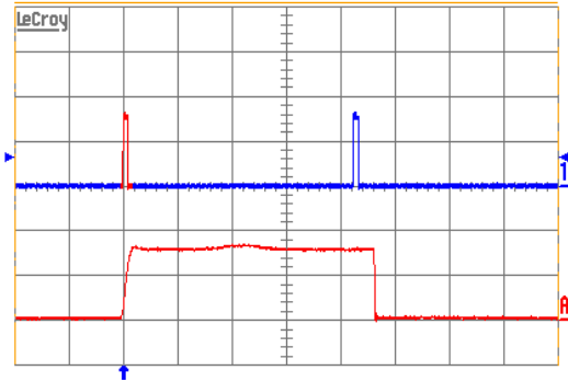
Figure 15. Load current (top trace, 10 A/div., 50 ms/div.) into a 10m \Omega short circuit during restart, at V_{in} = 48 V. Bottom trace (10A/div., 1.0ms/div.) is an expansion of the on-time portion of the top trace.
